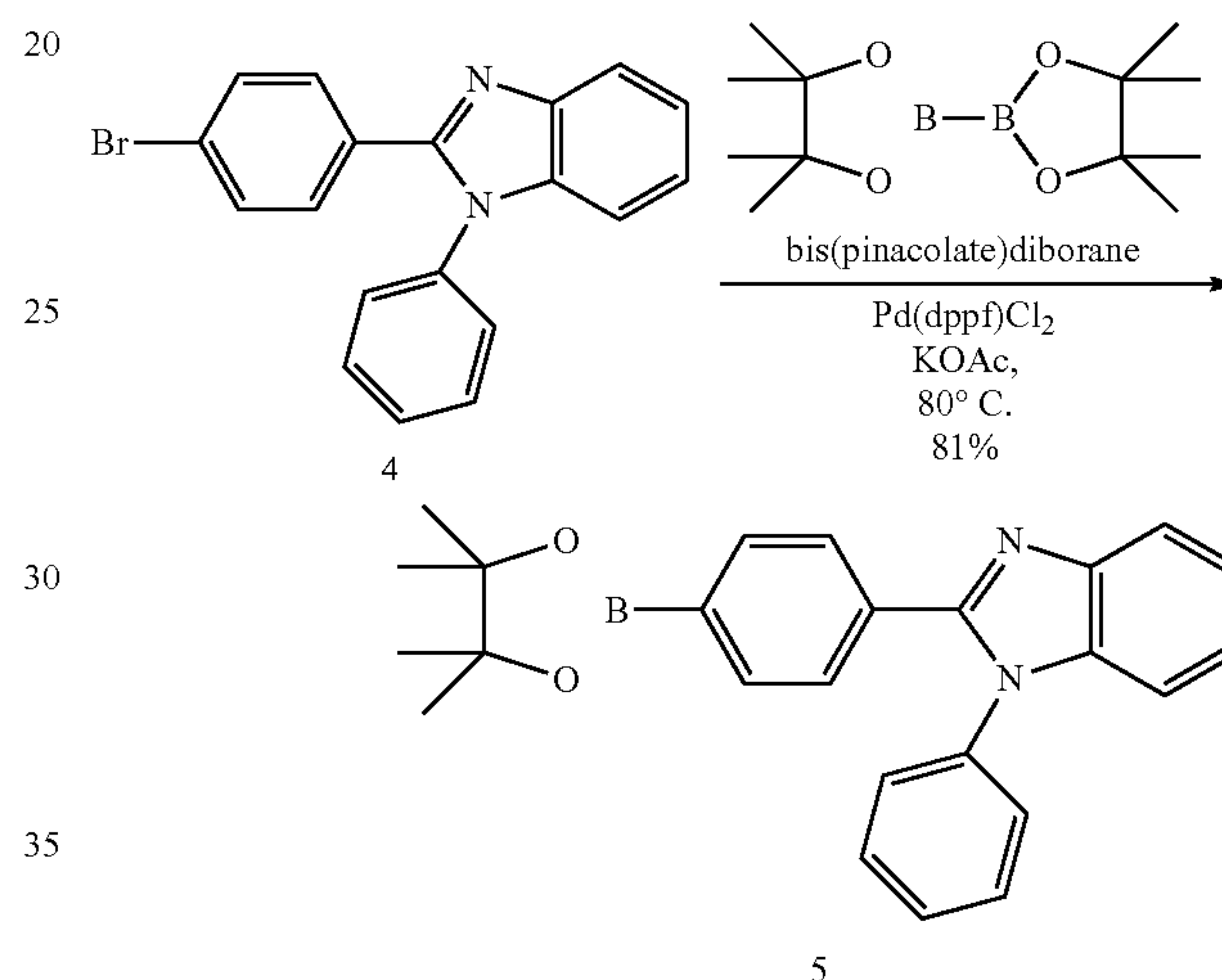
1-phenyl-2-(4-(4,4,5,5-tetramethyl-1,3,2-dioxaborolan-2-yl)phenyl)-1H-benzo[d]imidazole (5)
