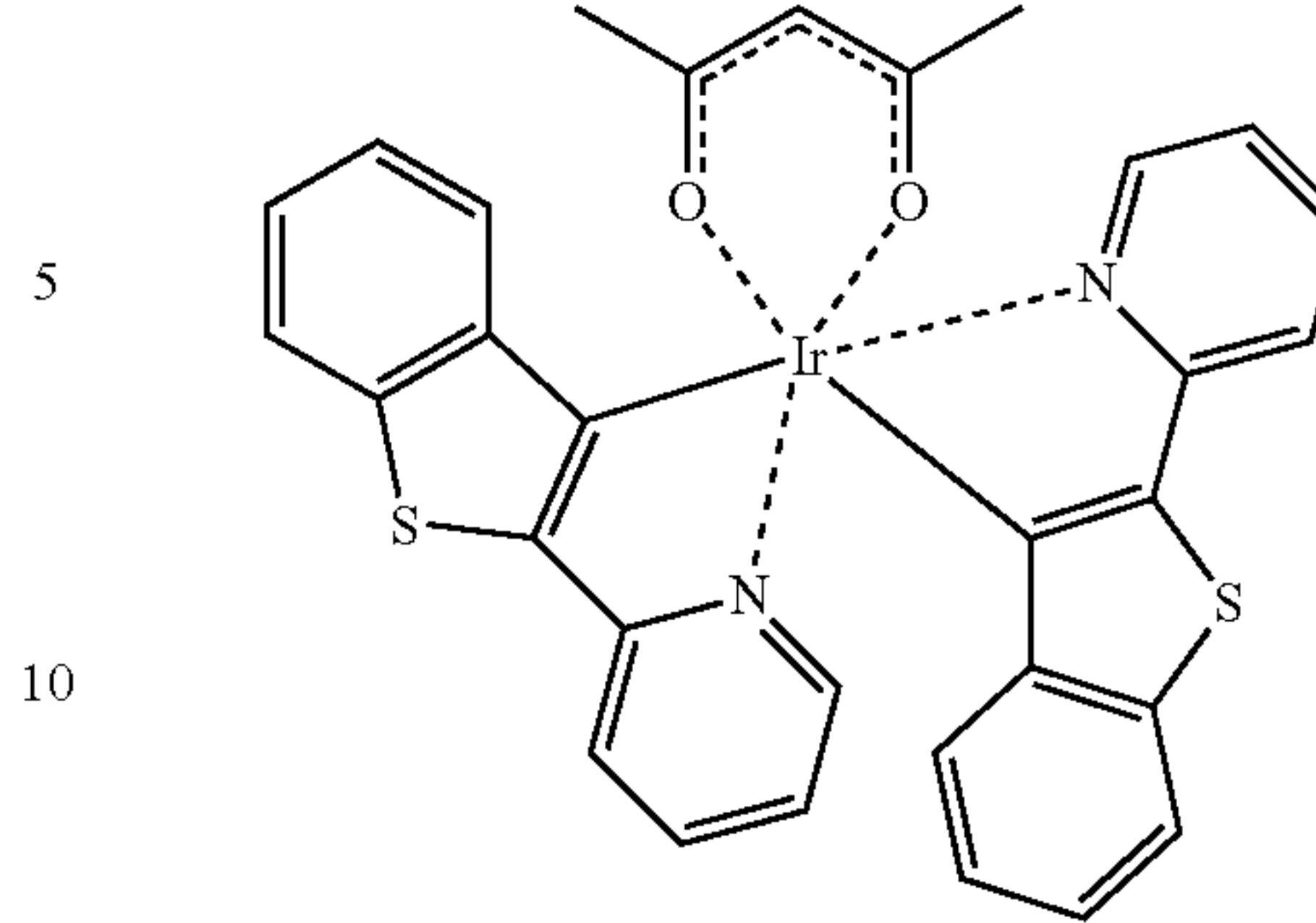
Ir(btp) 2 (acac); (Btp) 2 Ir(III)(acac); or Bis[2-(2'-benzothienyl)- pyridinato-N,C3'] iridium (III)(acetylacetonate)
