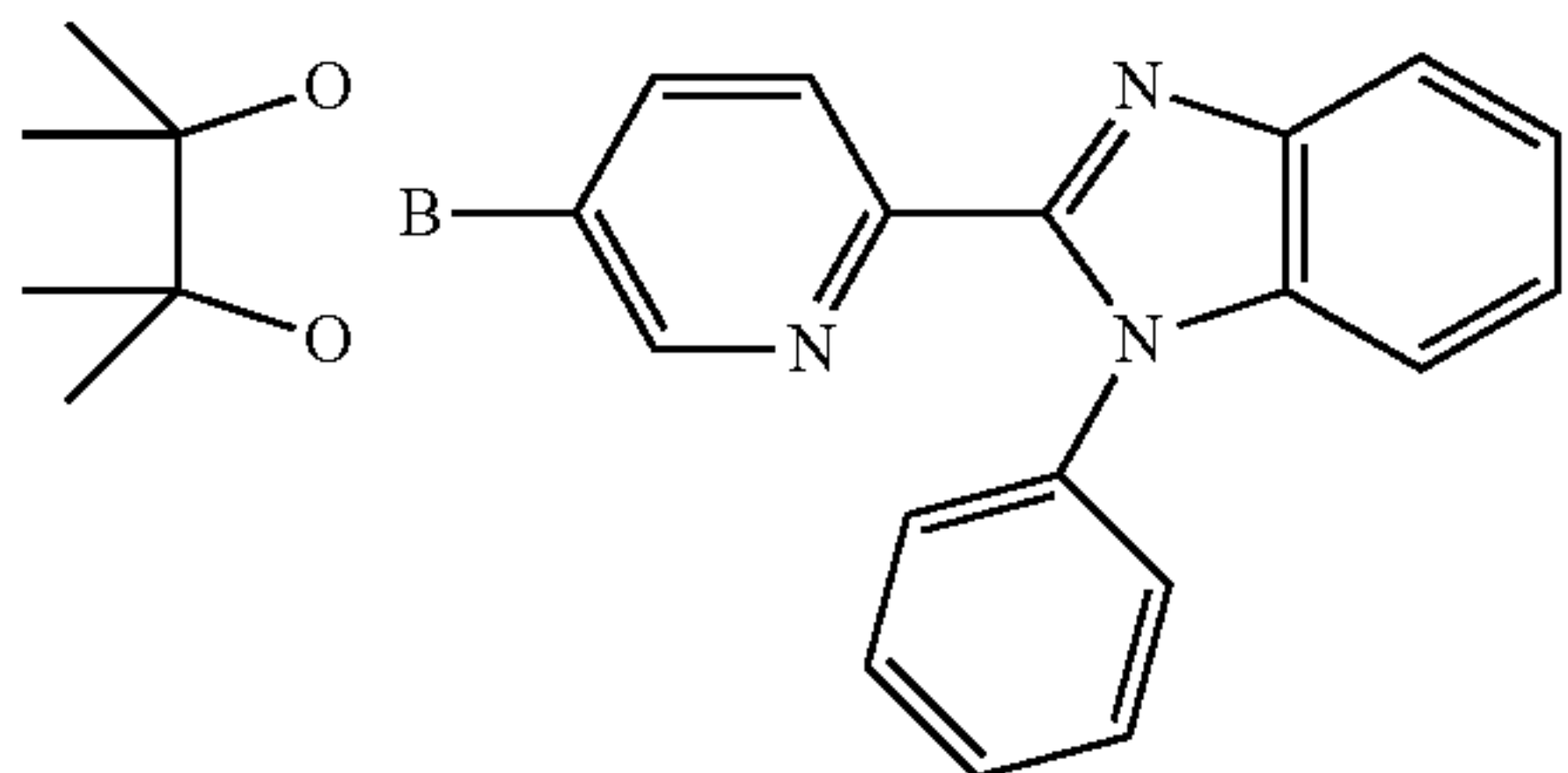
Compound 2
