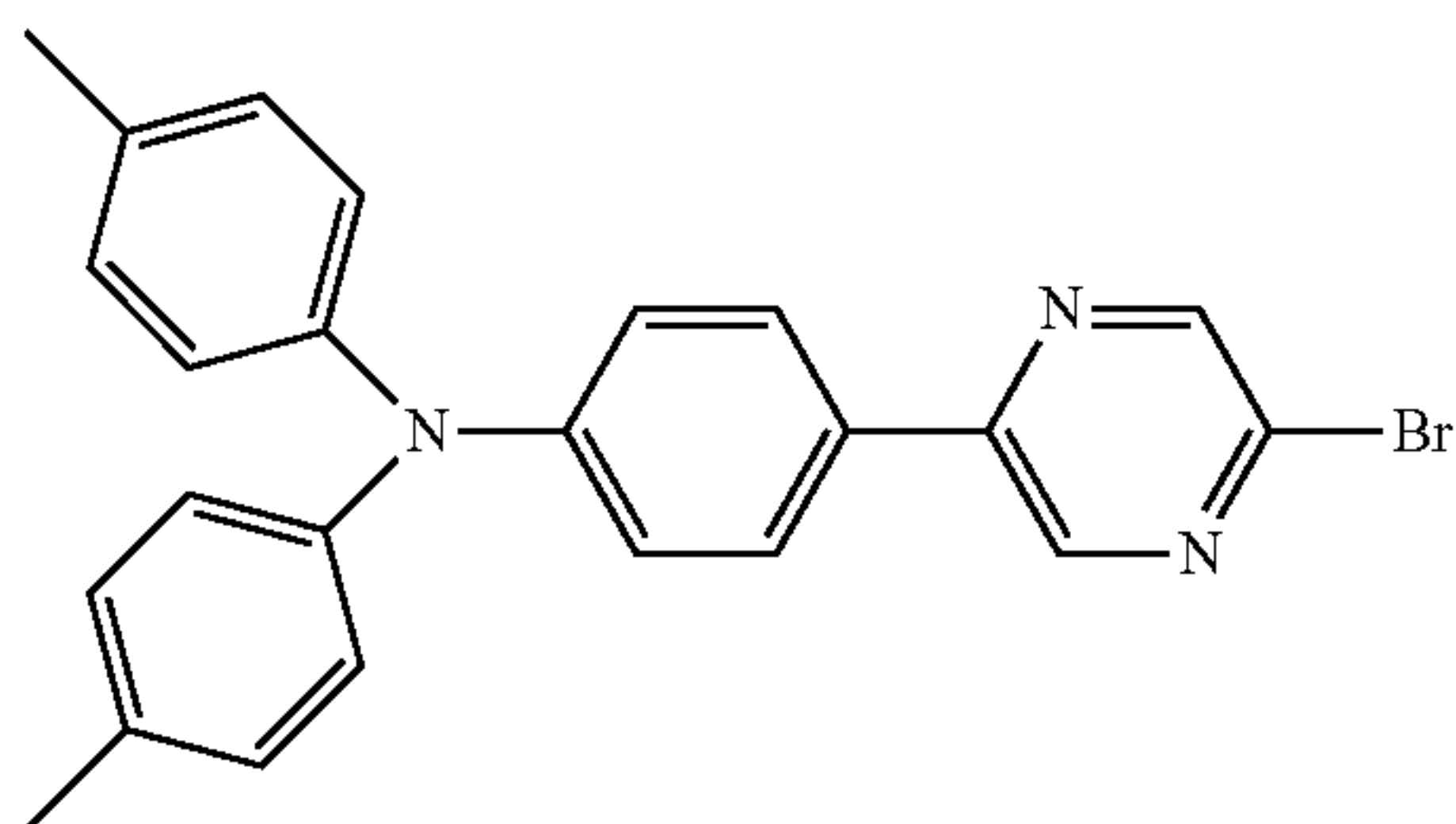
Compound 6
