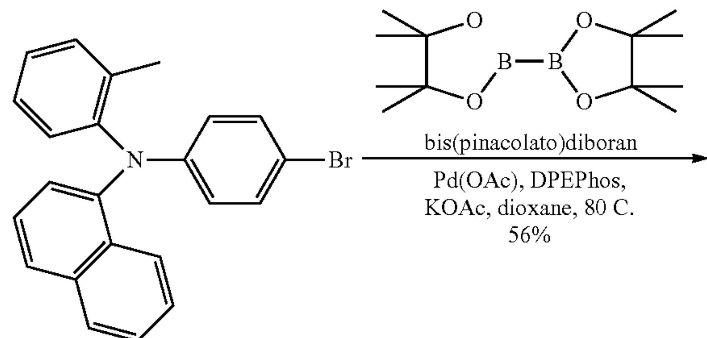
Compound 21
