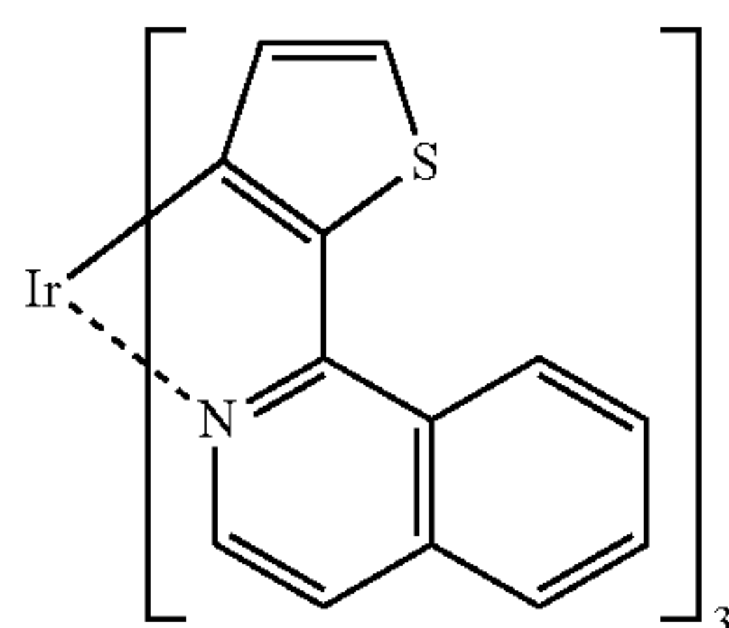
Ir(ti) 3 or Tris[1-thiophen-2- ylisoquinolino-N,C3']iridium (III)
