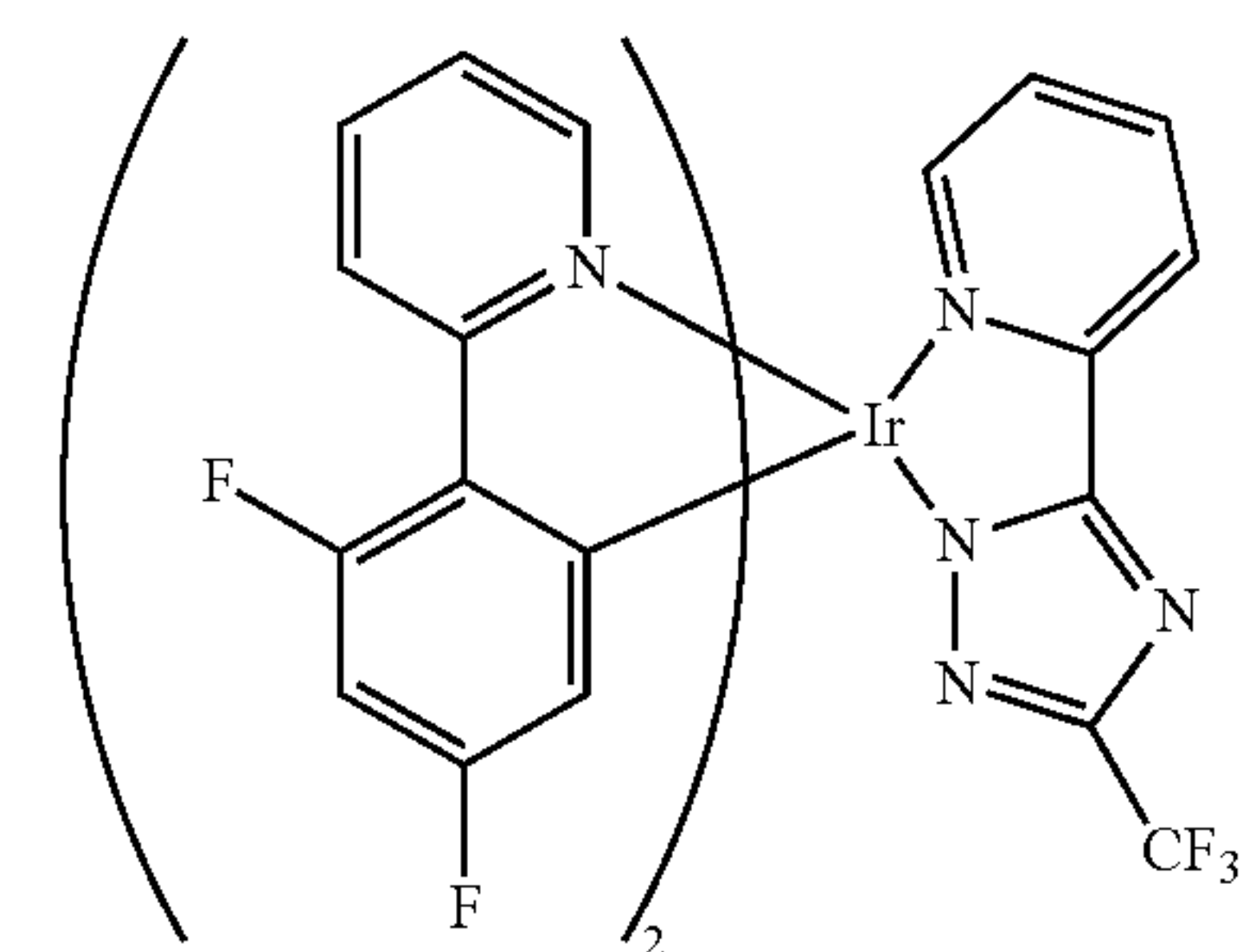
Iridium (III) bis(4,6-difluorophenylpyridinato)-3-(trifluoromethyl)-5-(pyridin-2-yl)-1,2,4-triazolate (Firtaz)
