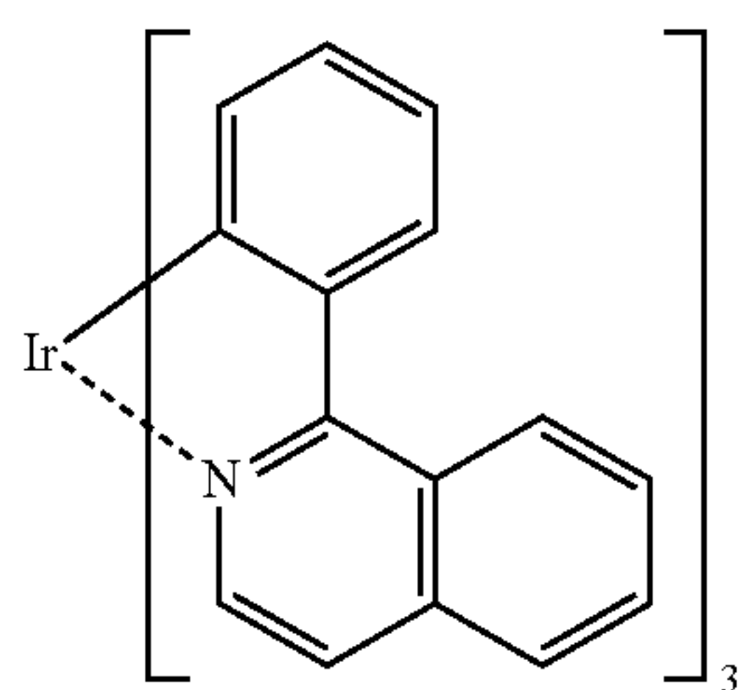
Ir(piq) 3 ; or Tris[1-phenylisoquinolino- N,C2']iridium (III)
