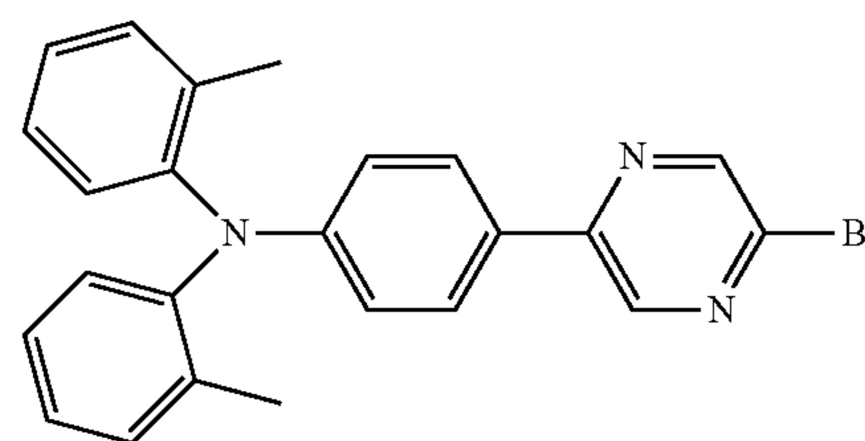
Compound 13
