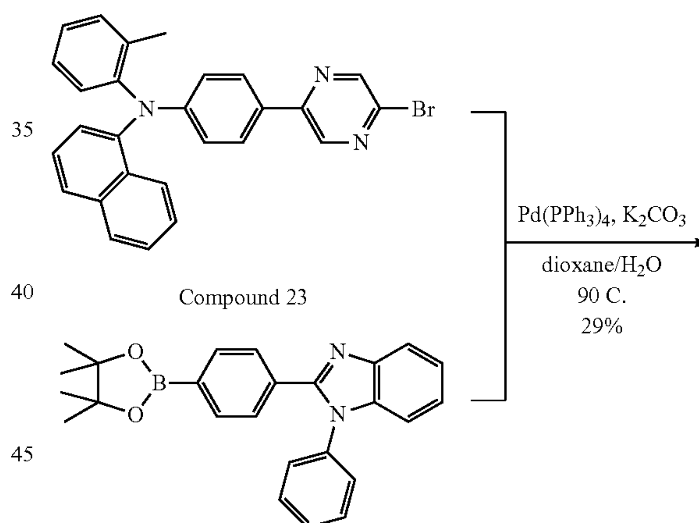
Compound 5
