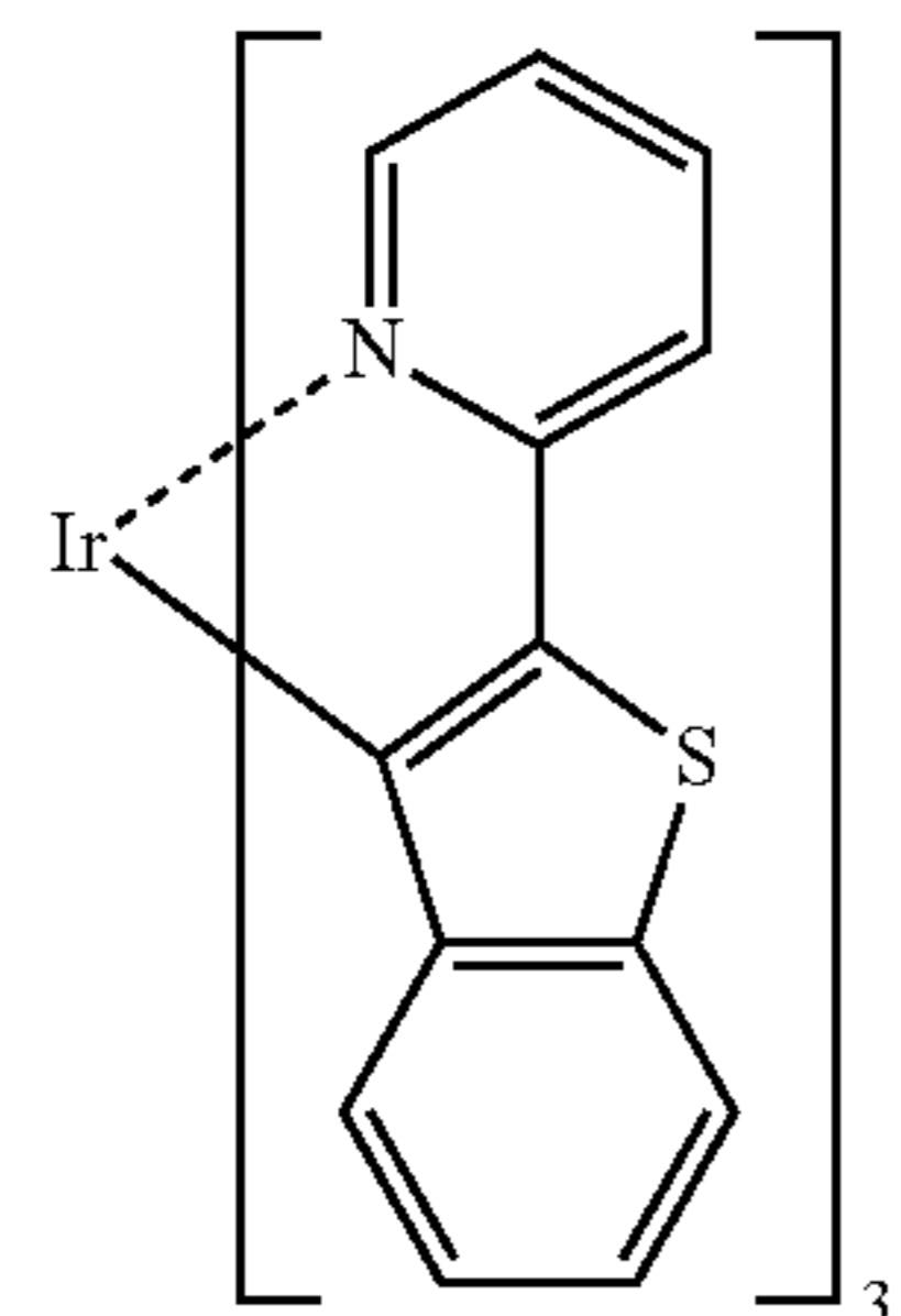
Ir(btp) 3 or Tris-[2-(2'-benzothieryl)- pyridinato-N,C3']iridium (III)
