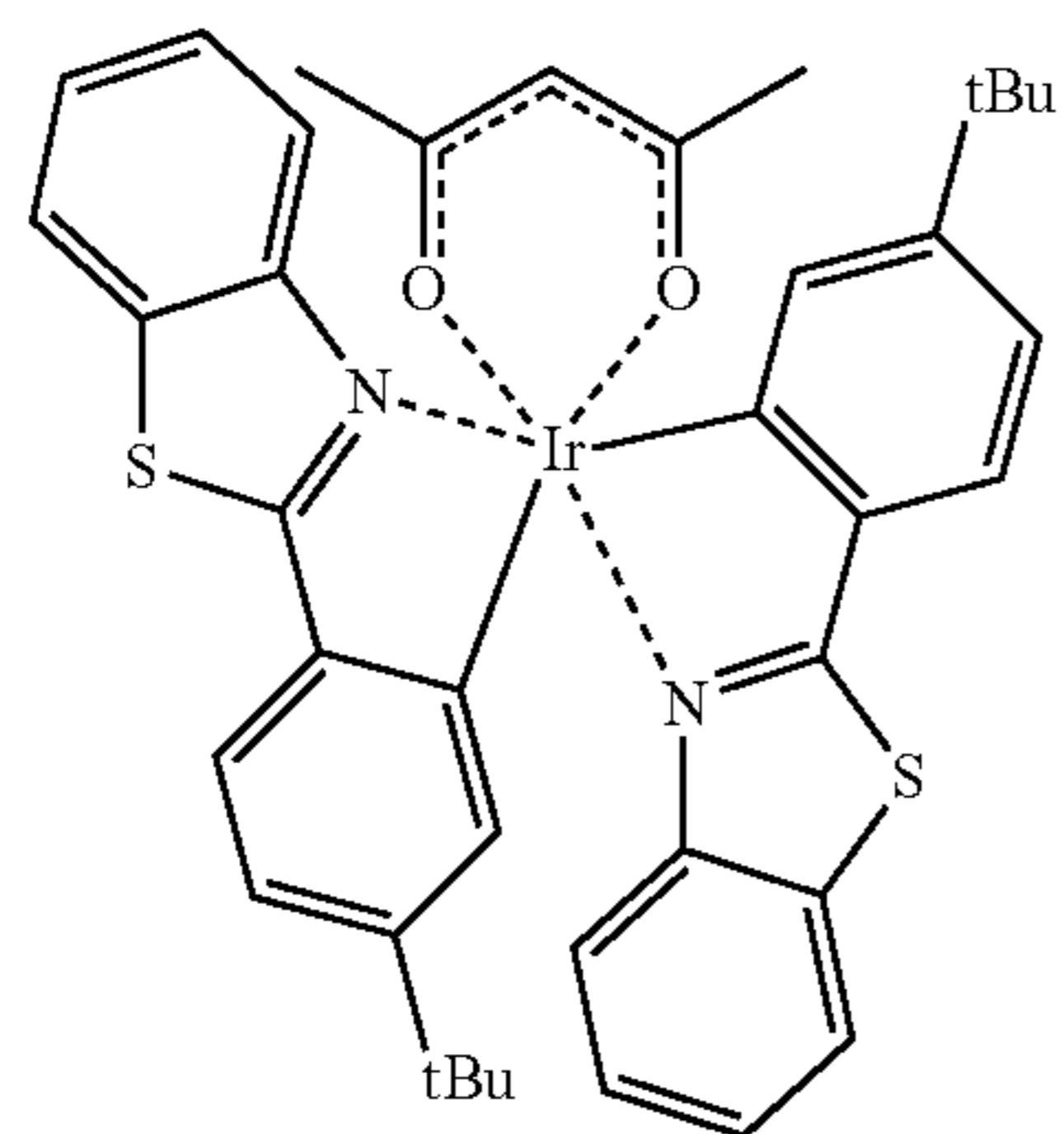
(t-bt) 2 Ir(III)(acac) Bis[2-(4-tert- butylphenyl)benzothiazolato- N,C2']iridium (III) (acetylacetonate)
