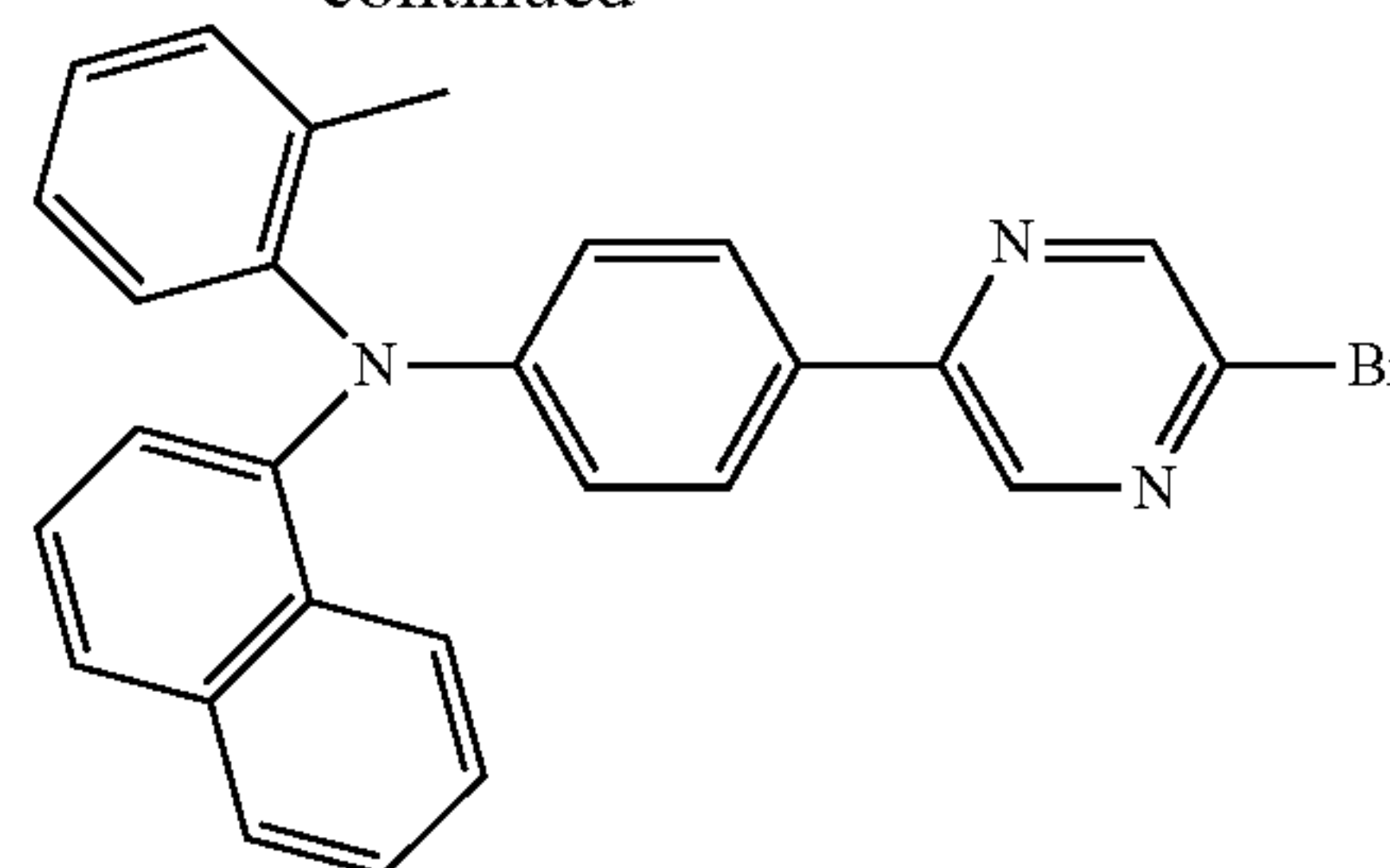
Compound 23
