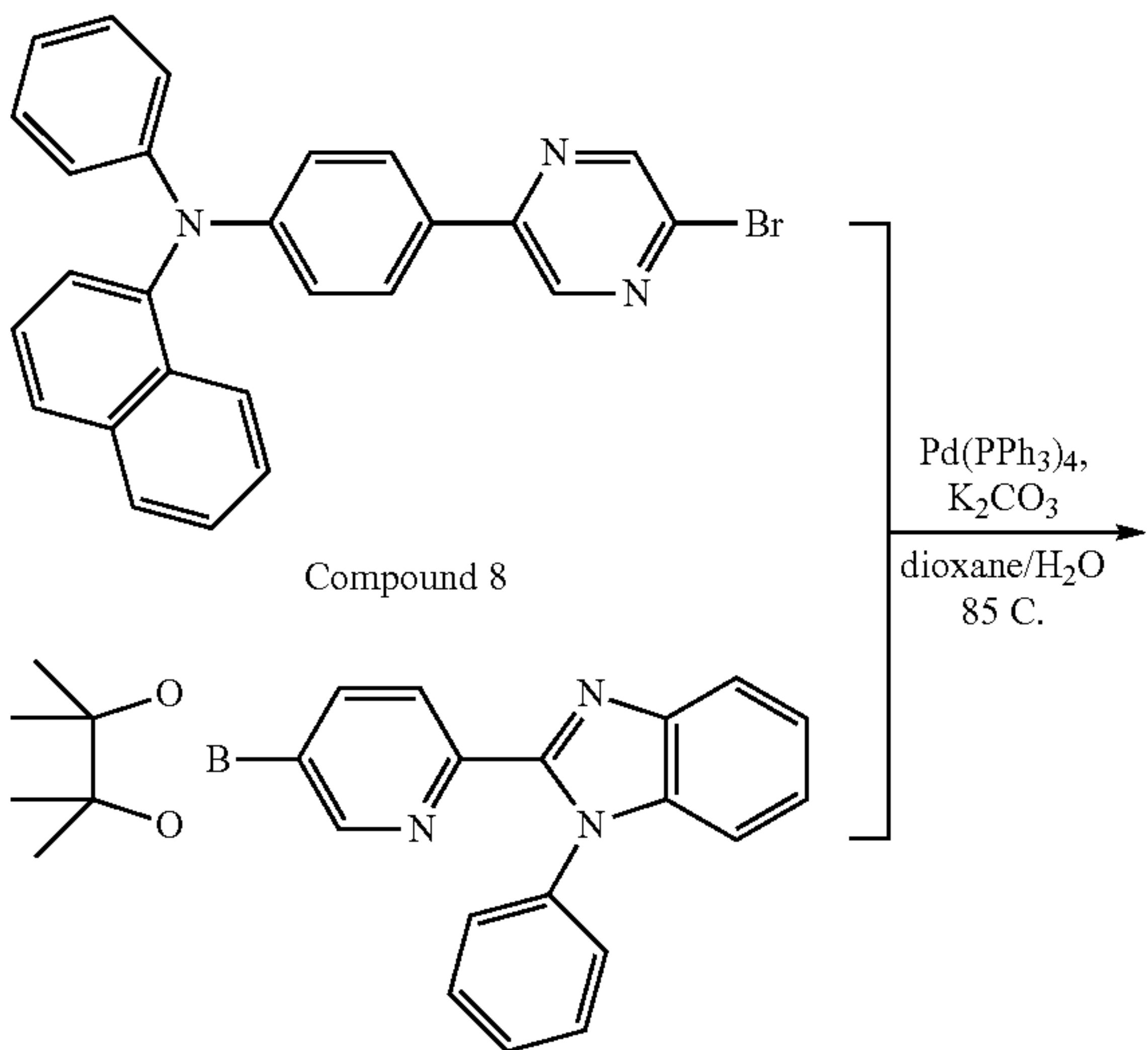
Compound 2
