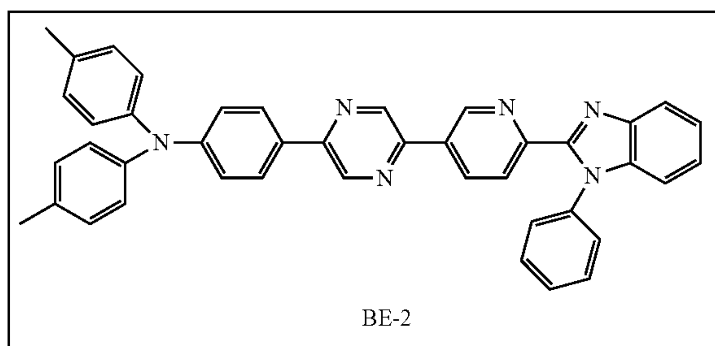
Compound 5
