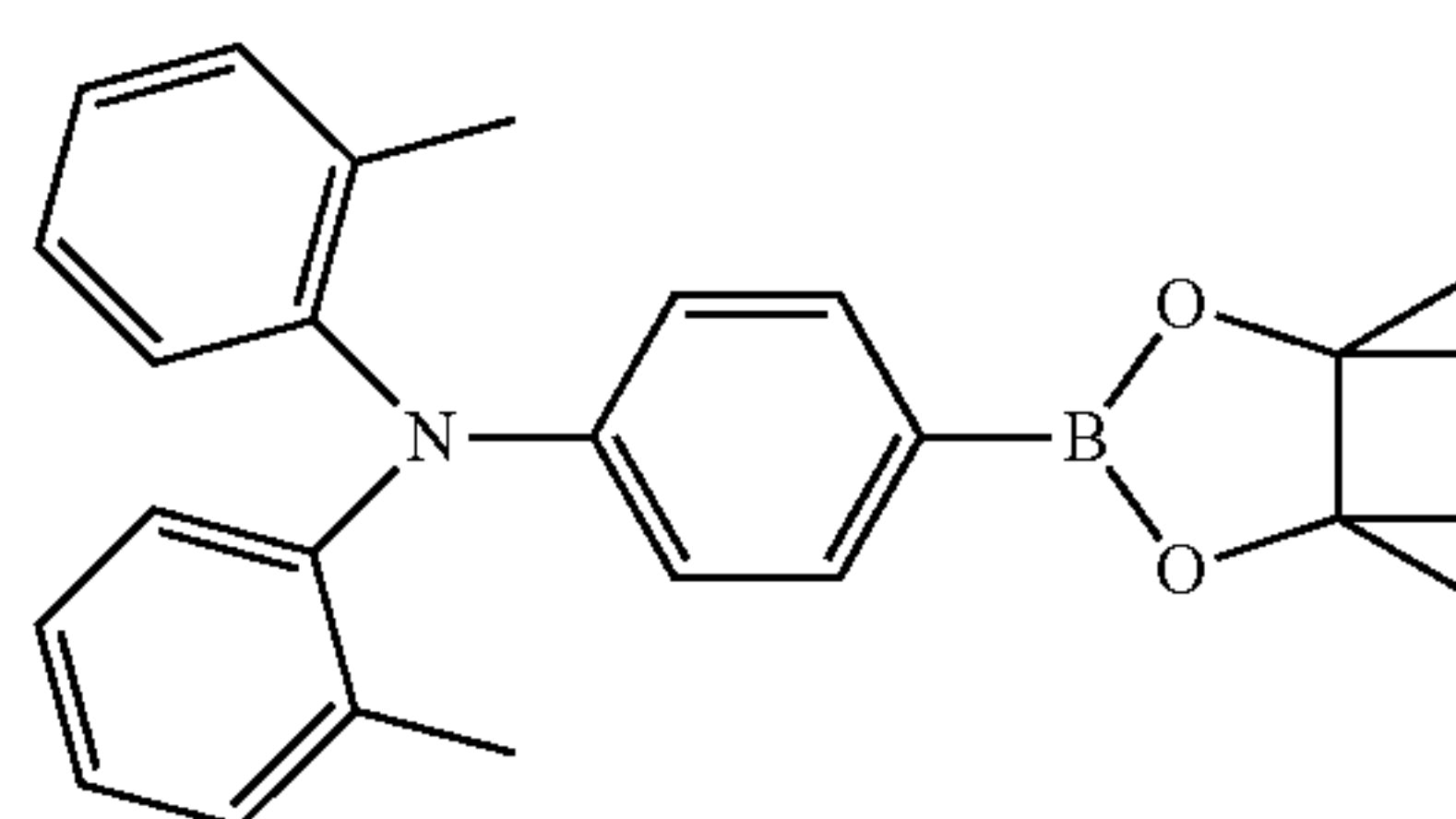
Compound 12
