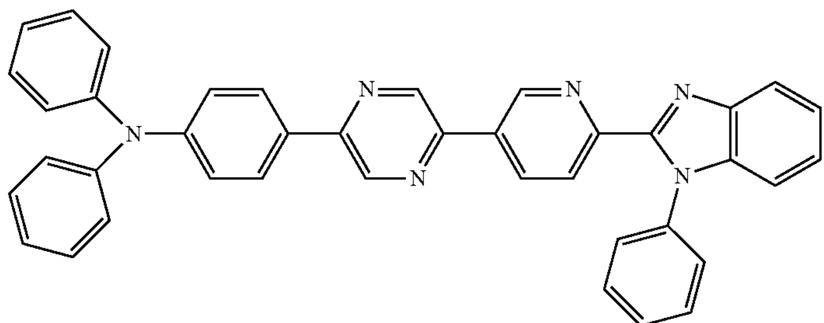
N,N-diphenyl-4-(5-(6-(1-phenyl-1H-benzo[d]imidazol-2-yl)pyridin-3-yl)pyrazin-2-yl)aniline
