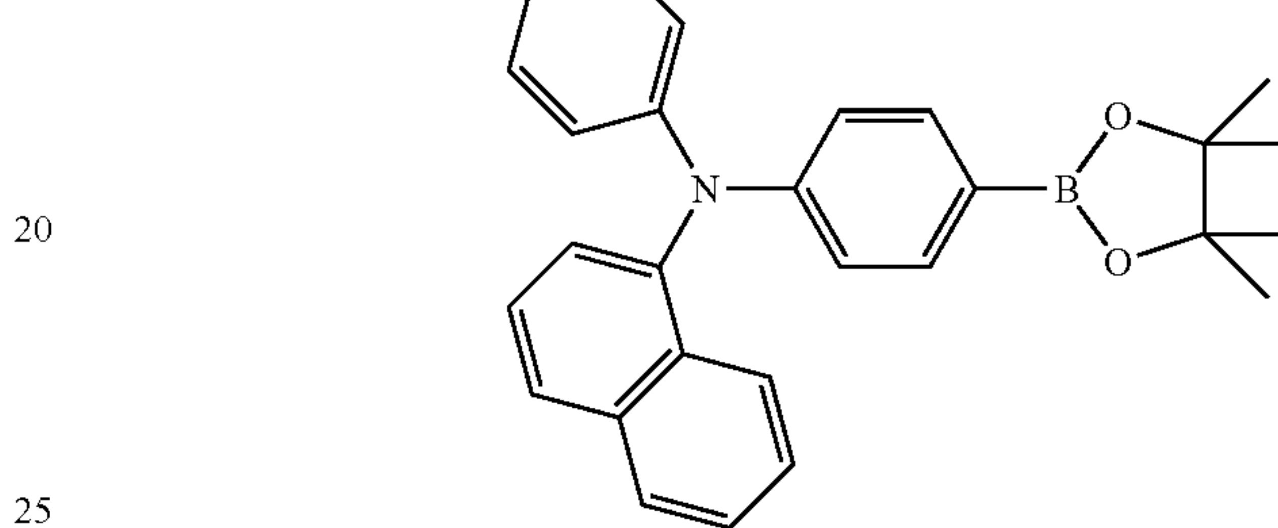
Compound 7
