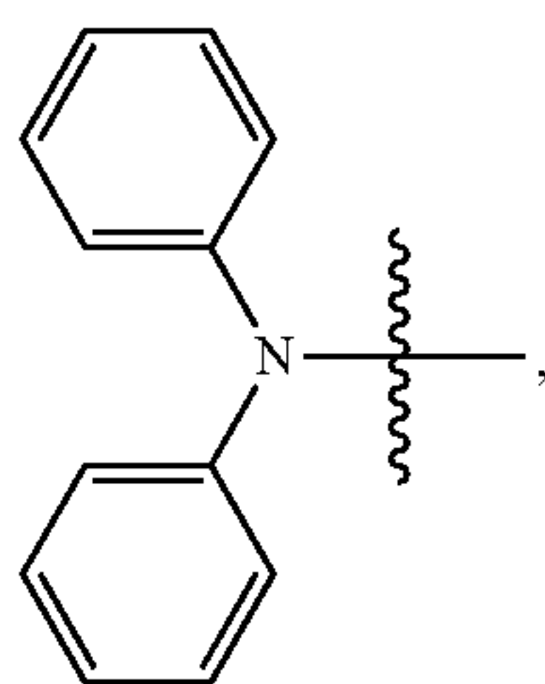
unsubstituted diphenylamine
