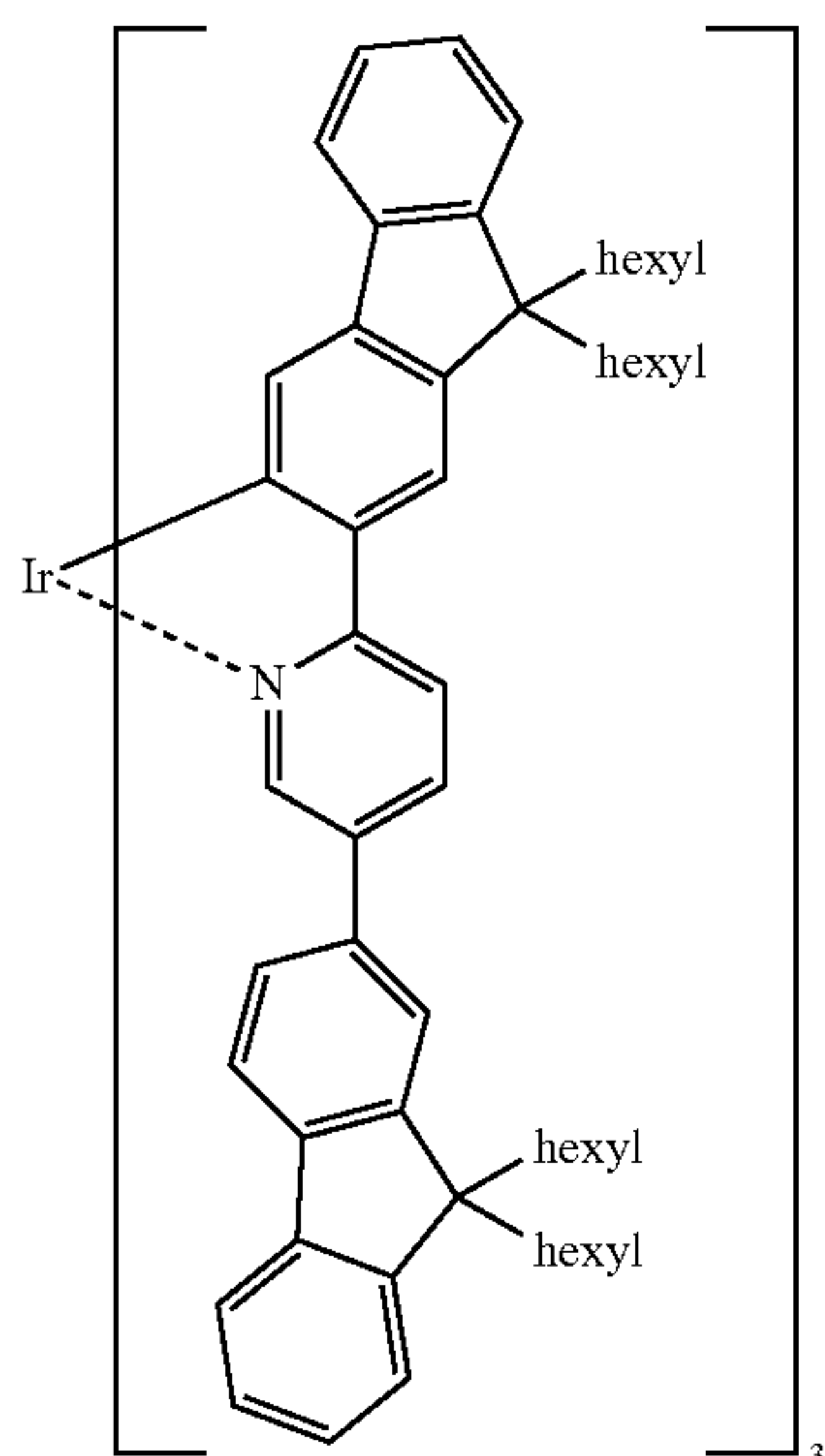
Ir(HFP) 3 or Tris(2,5-bis-2'-(9,9'- dihexylfluorene)pyridine)iridium (III)
