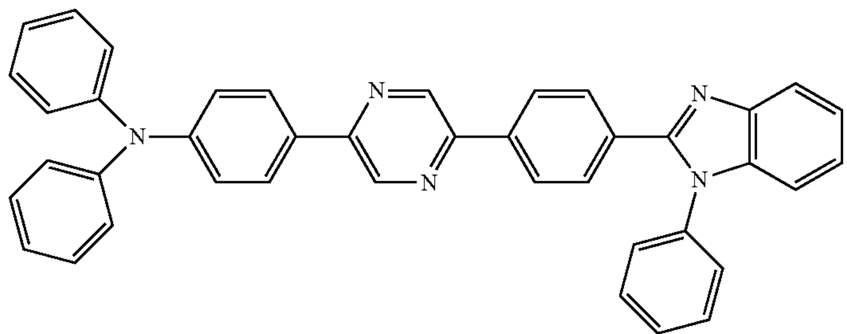
N,N-diphenyl-4-(5-(4-(1-phenyl-1H-benzo[d]imidazol-2-yl)phenyl)pyrazin-2-yl)aniline
