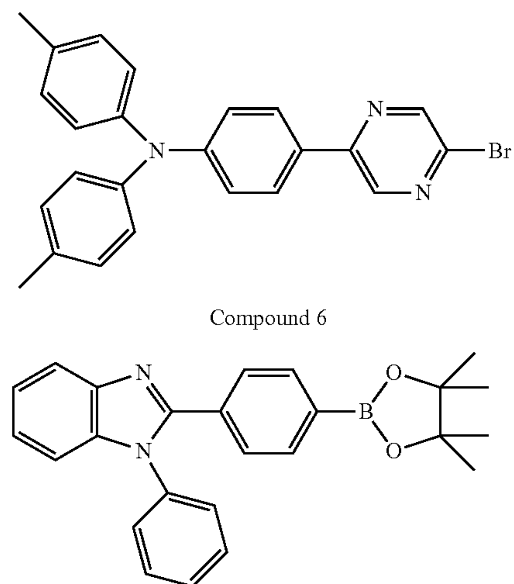
Compound 5
