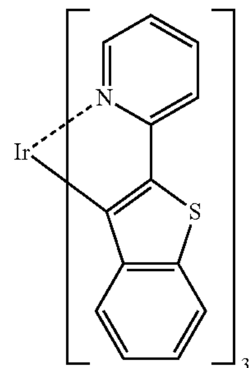
Ir(btp) 3 or Tris-[2-(2'-benzothiophenyl)- pyridinato-N,C3']iridium (III)
