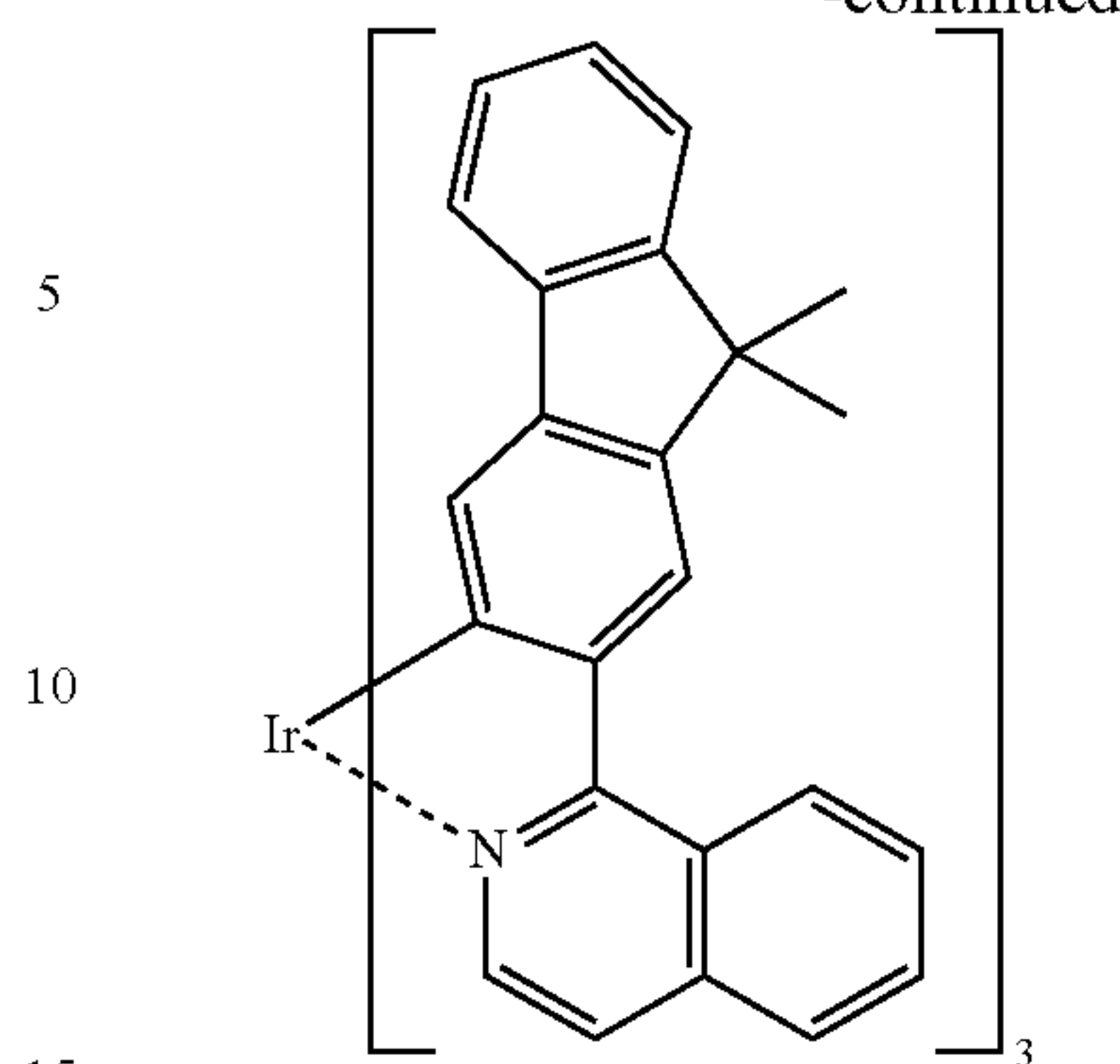
Ir(fli) 3 ; Ir(fliq) 3 ; or Tris[1-(9,9-dimethyl-9H- fluoren-2-yl)isoquinolino- (N,C3')]iridium (III)
