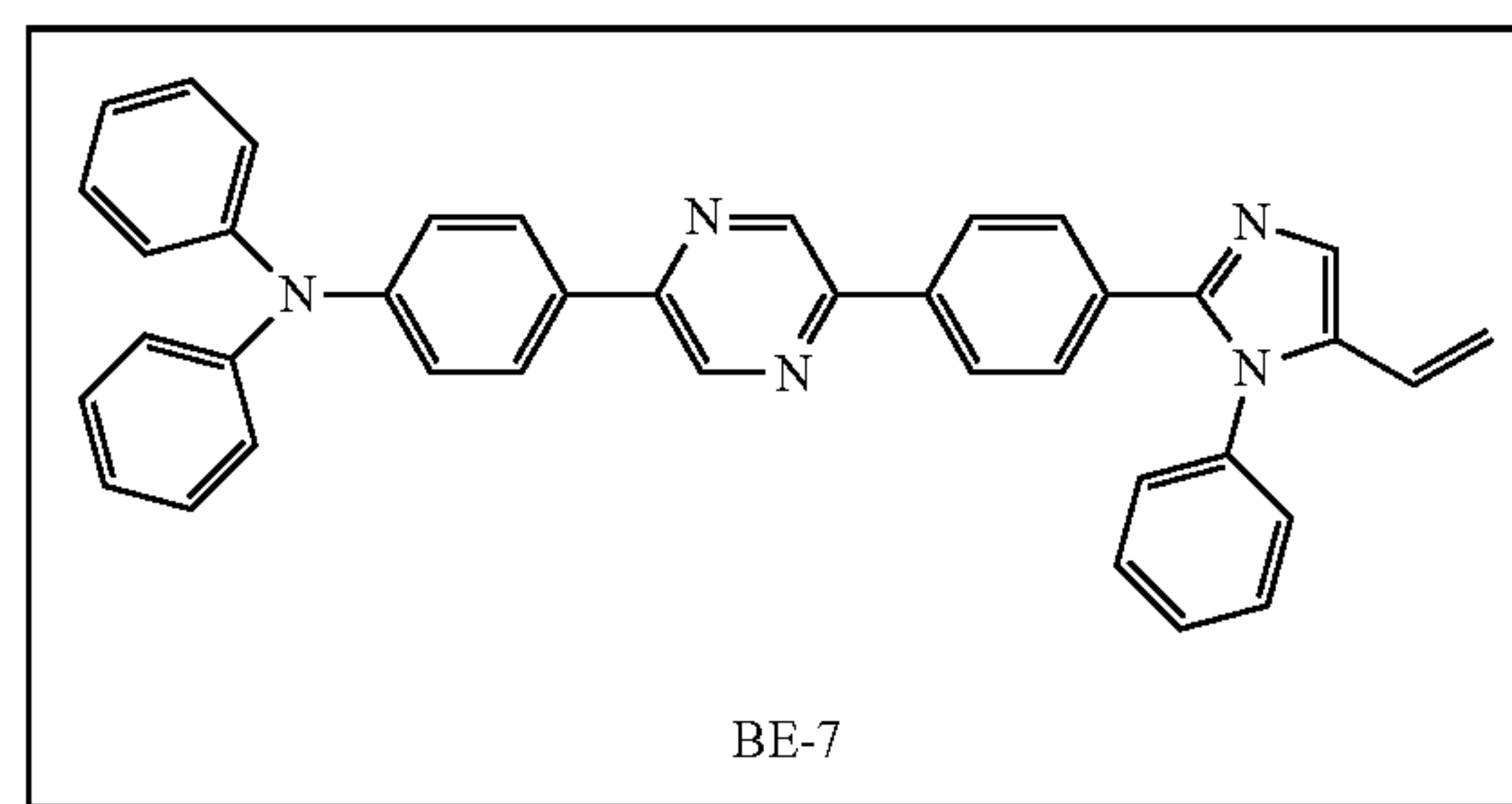
Compound 5
