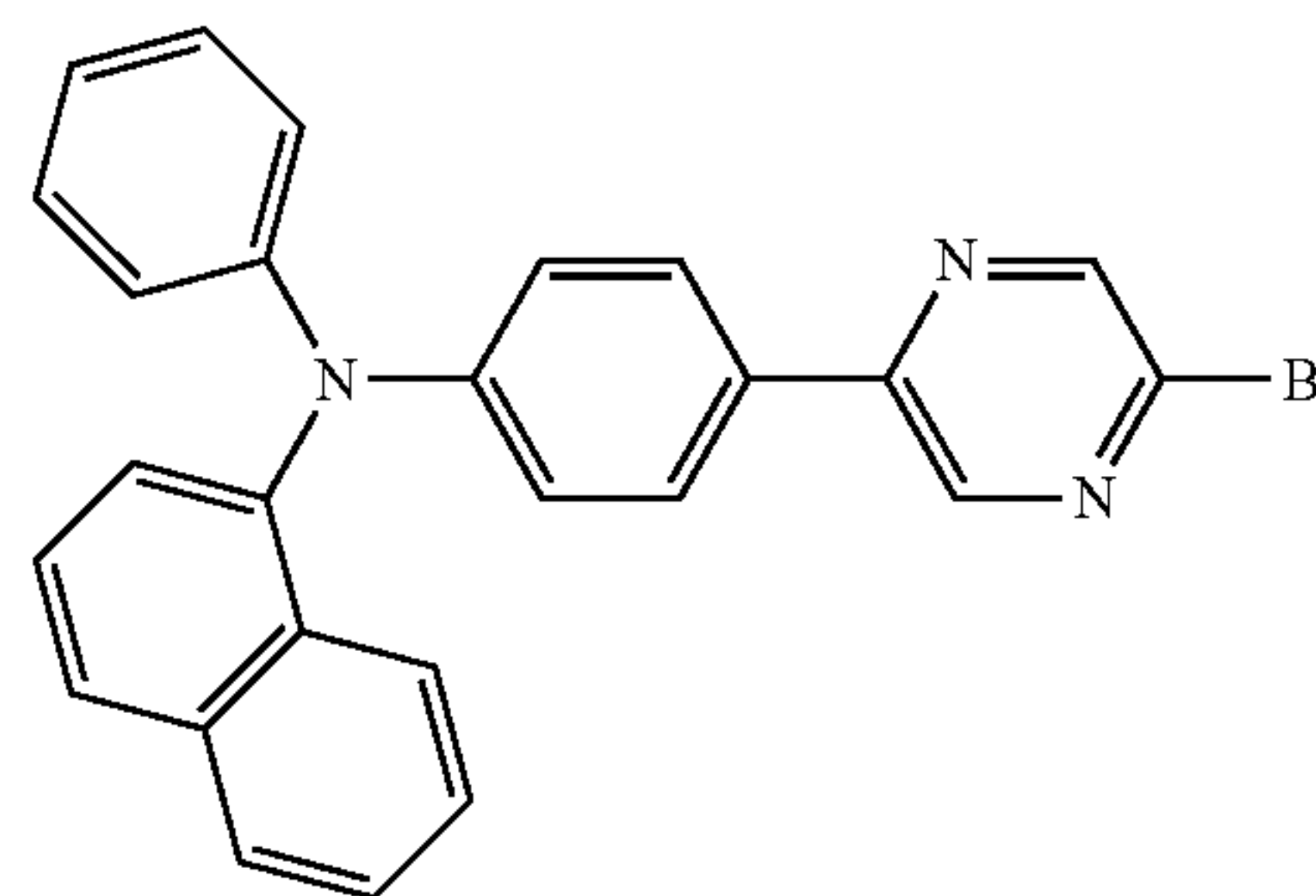
Compound 8
