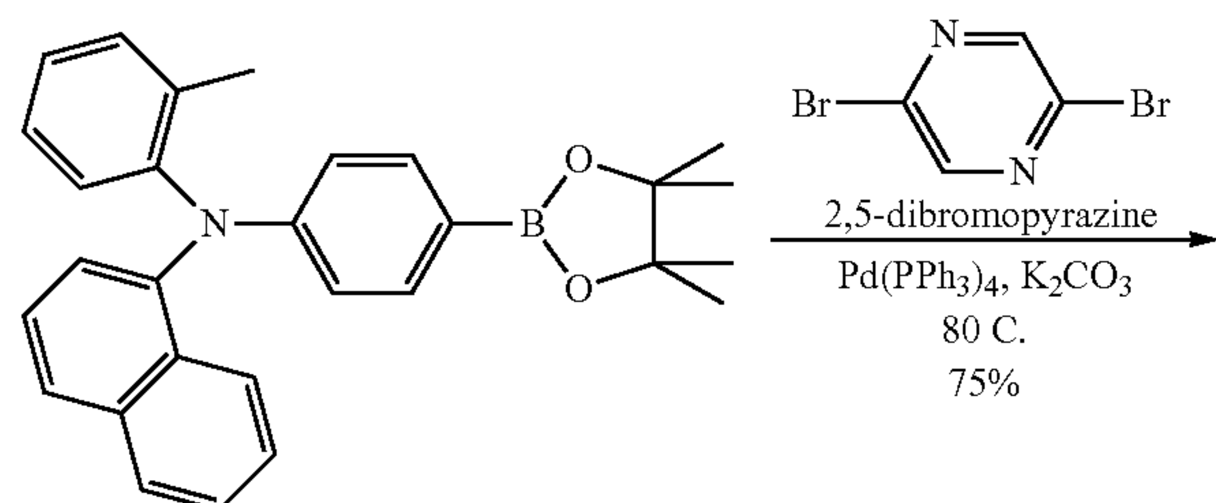
Compound 22
