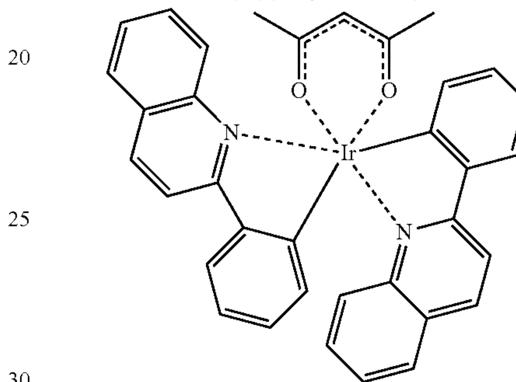
Ir(pq) 2 (acac); (Pq) 2 Ir(III)(acac); or Bis[2-phenylquinolyl- N,C2']iridium (III) (acetylacetonate)
