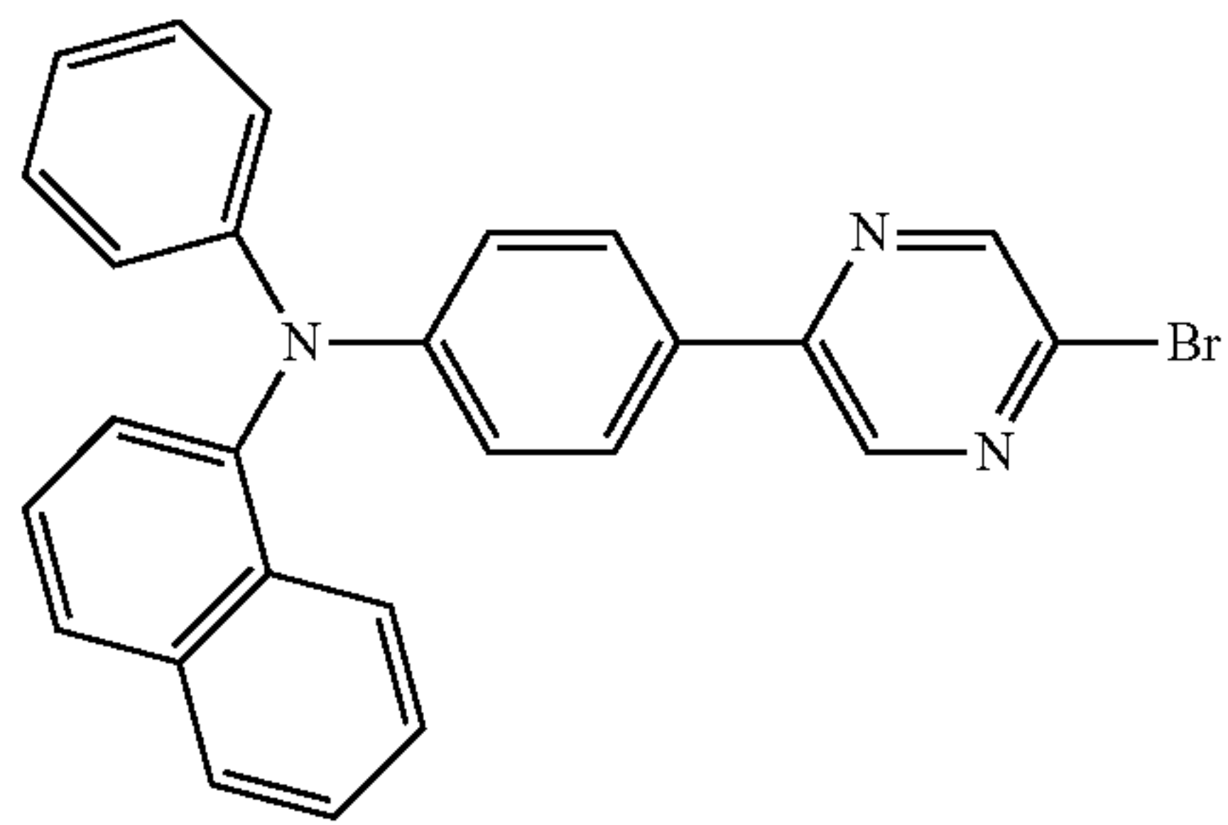
Compound 8
