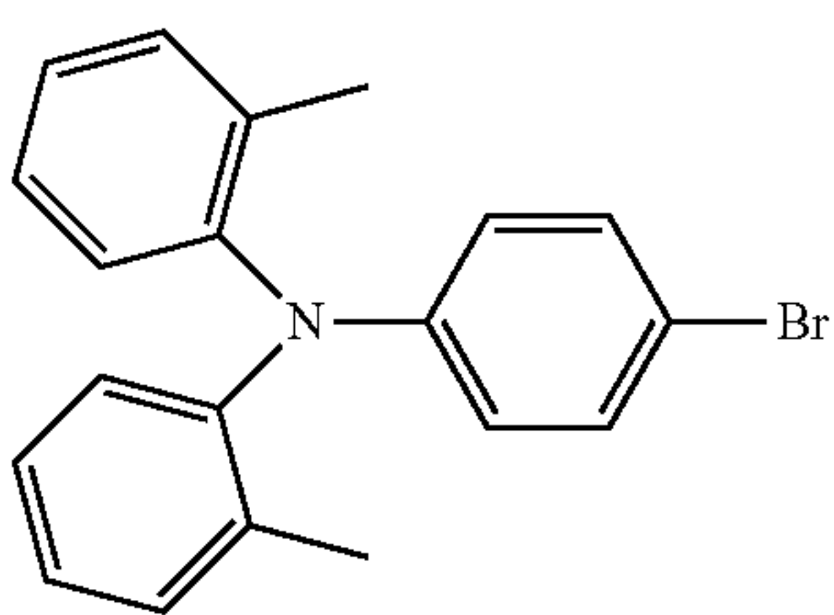
Compound 11
