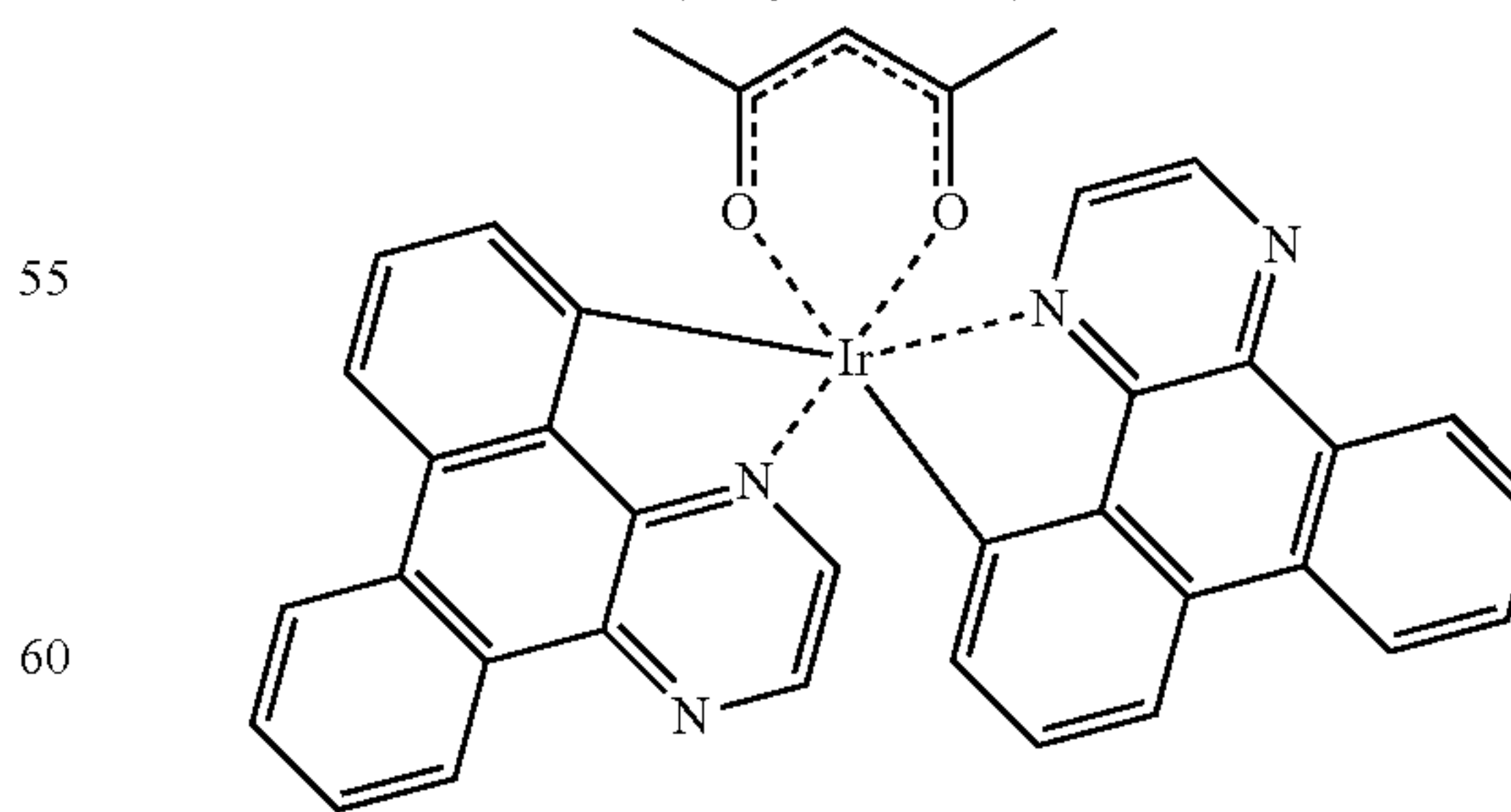
Ir(DBQ) 2 (acac); (DBQ) 2 Ir(acac); or Bis[(dibenzo[f,h]quinoxalin- N,C2')iridium (III) (acetylacetonate)
