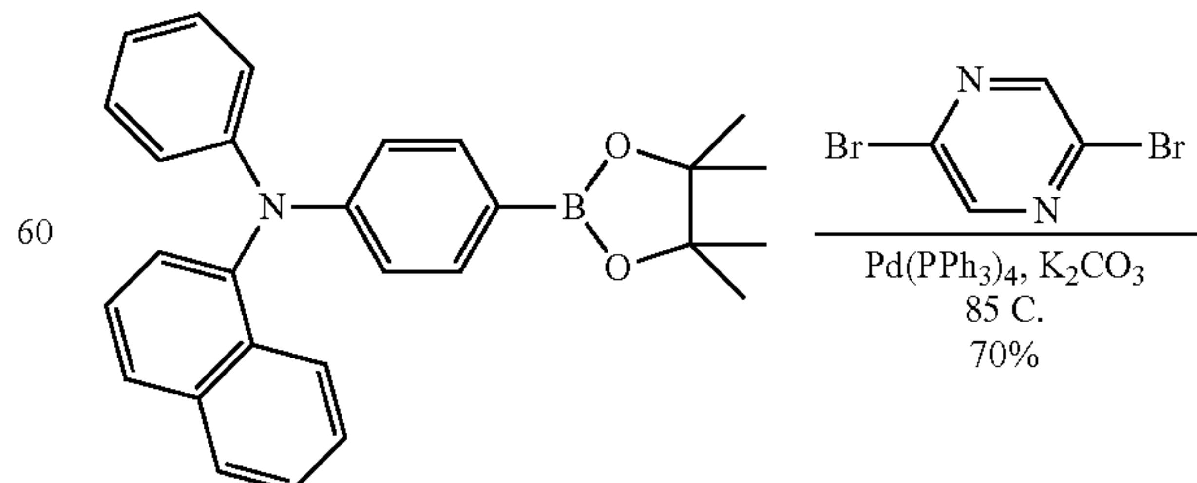
Compound 7
