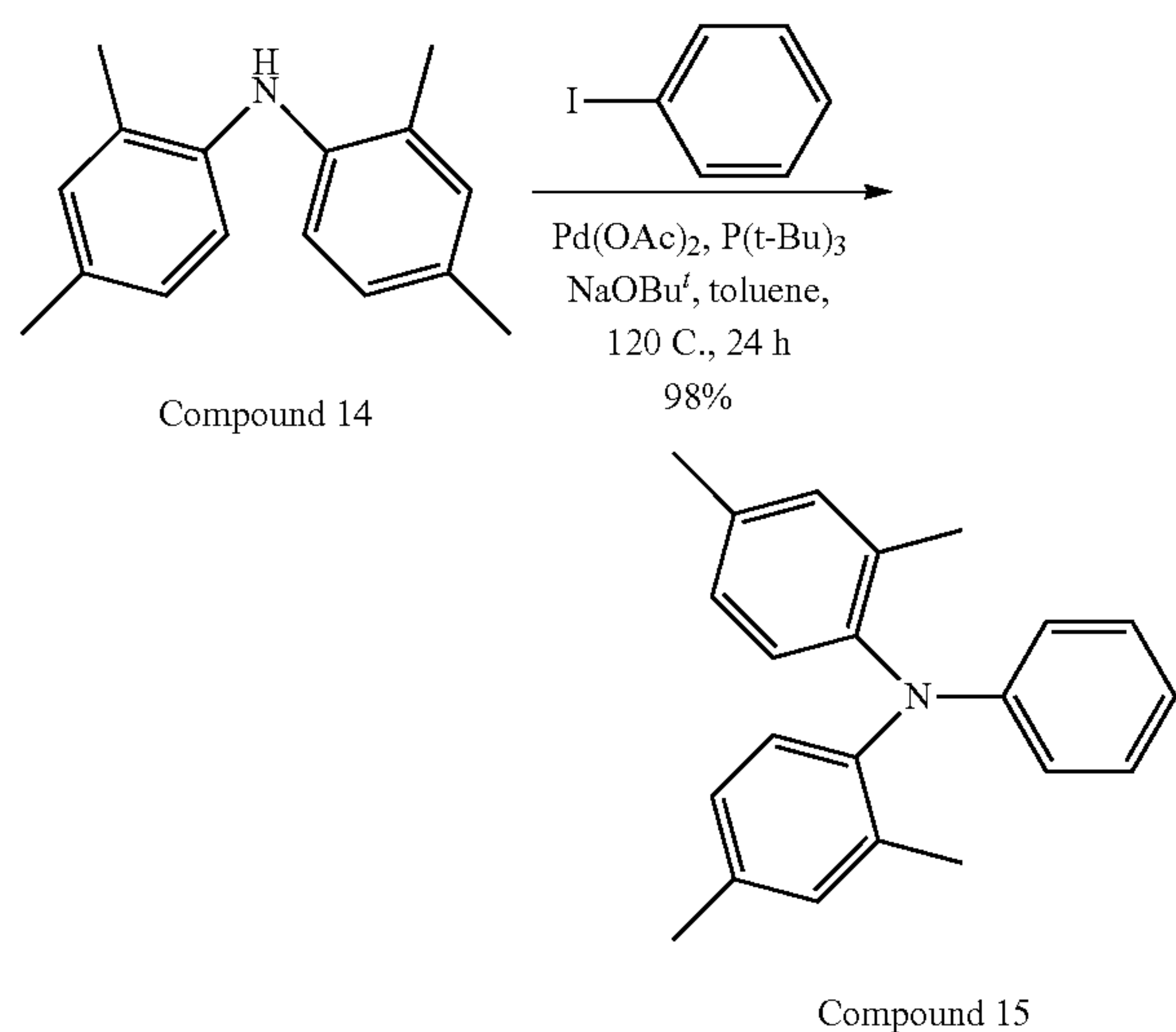
N-(2,4-dimethylphenyl)-2,4-dimethyl-N-phenylaniline (Compound 15)
