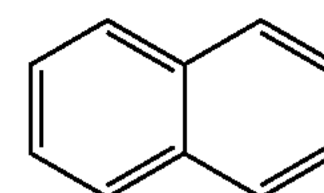
naphthyl
