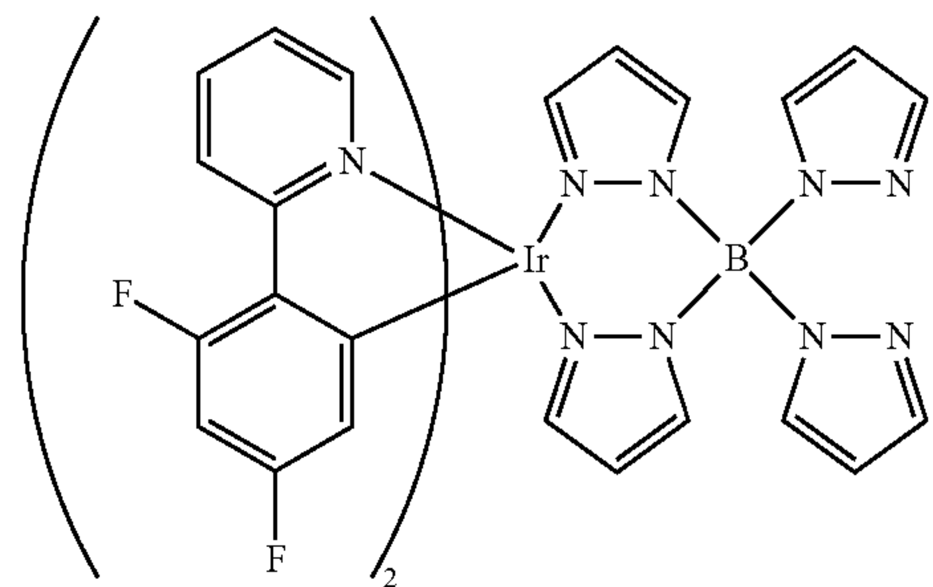
bis[2-(4,6-difluorophenyl)pyridinato-N,C2']iridium (III) tetra(1-pyrazolyl)borate(Fir6)
