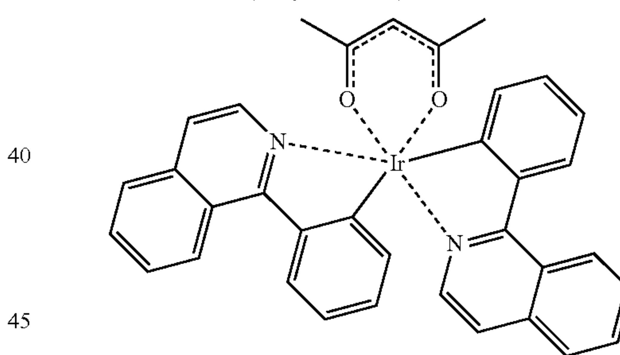
Ir(piq) 2 (acac); (Piq) 2 Ir(III)(acac); or Bis[1-phenylisoquinolinato- N,C2']iridium (III) (acetylacetonate)
