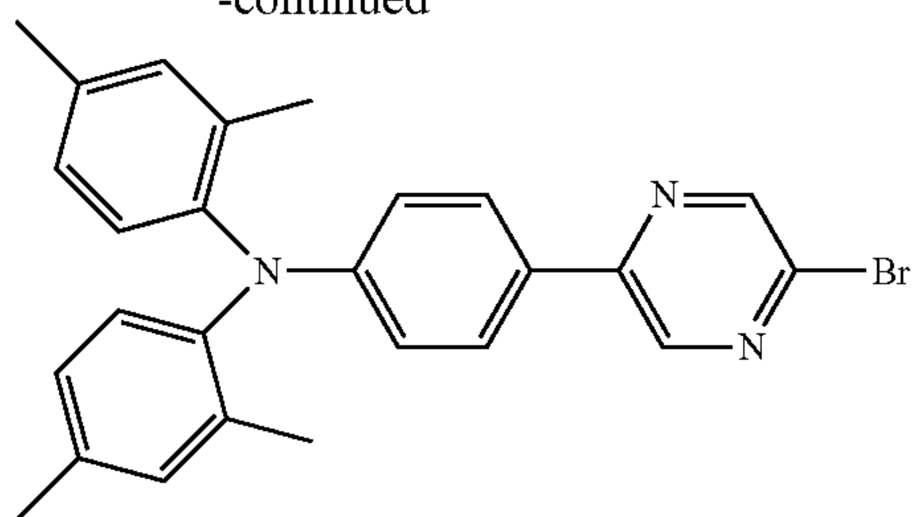
Compound 18
