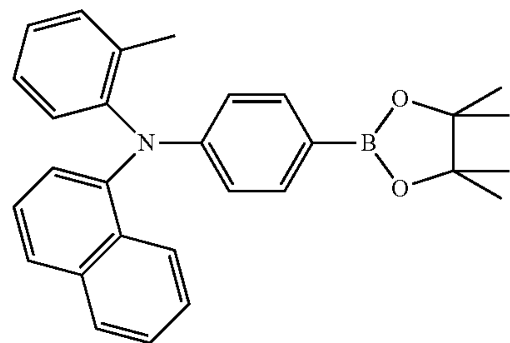
Compound 22
