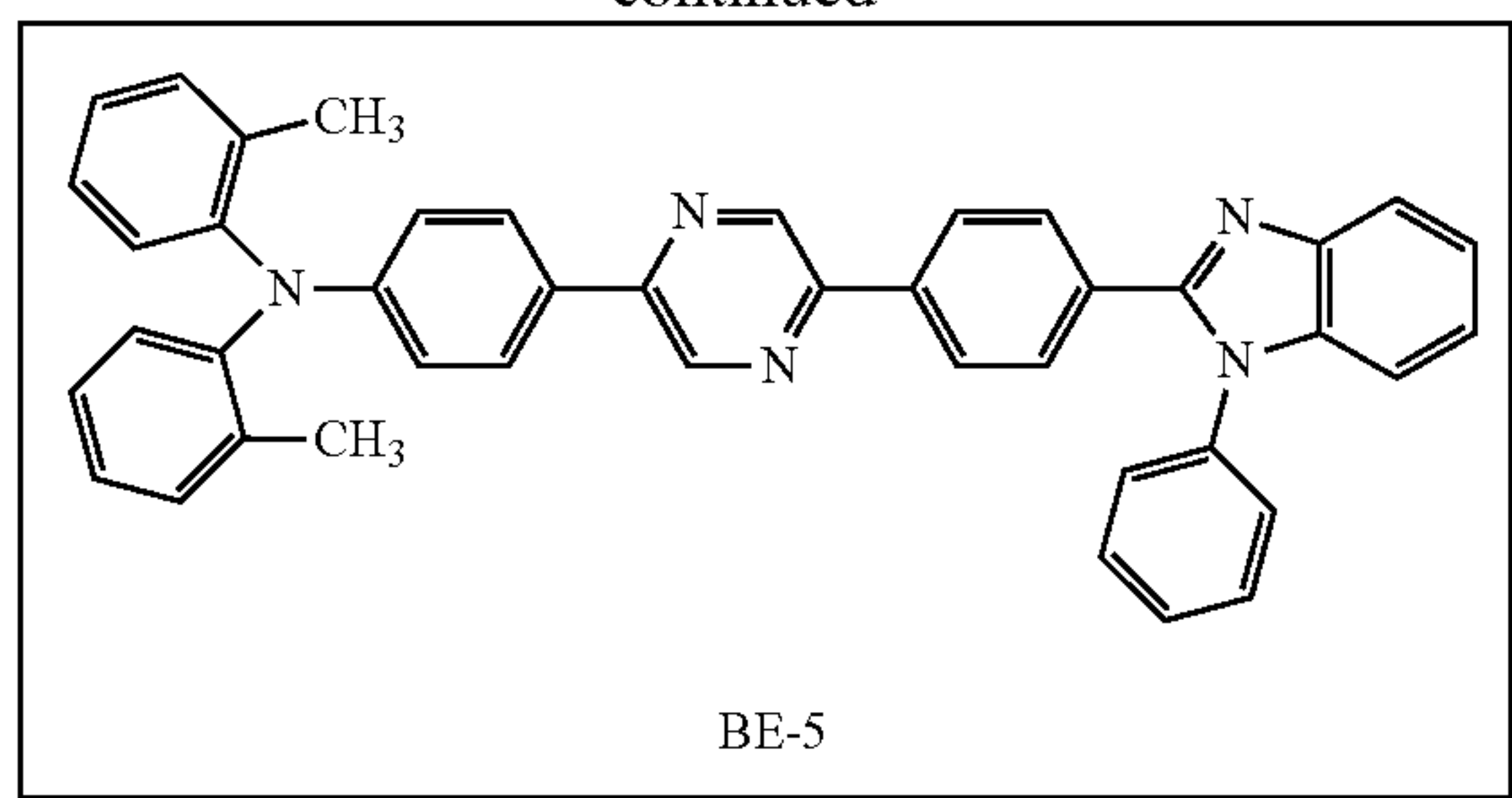
Compound BE-5
