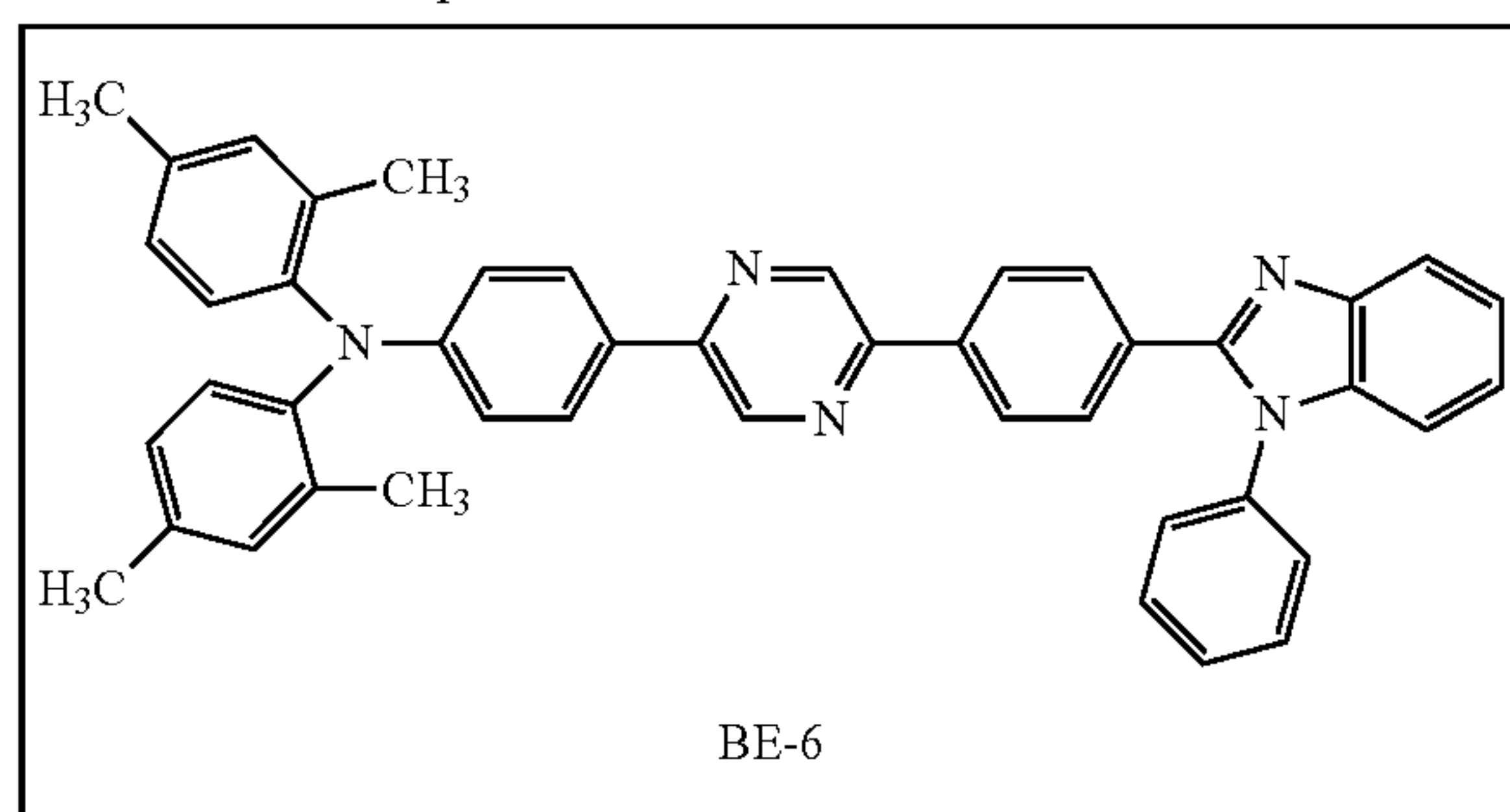
Compound BE-6
