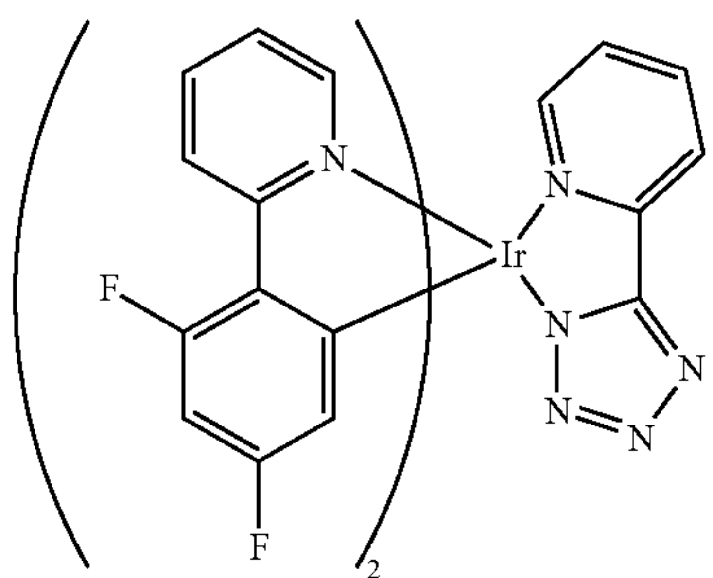
Iridium (III) bis(4,6-difluorophenylpyridinato)-5-(pyridin-2-yl)-1H-tetrazolate (FIRN4)
