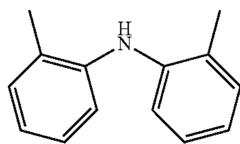
Compound 9
