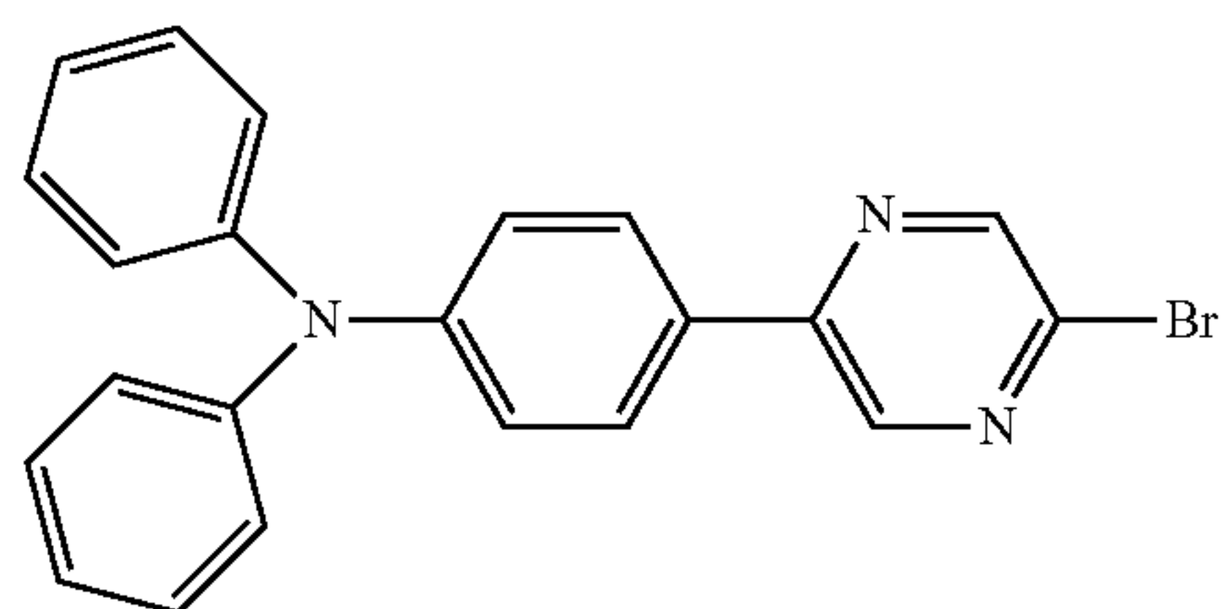
Compound 19
