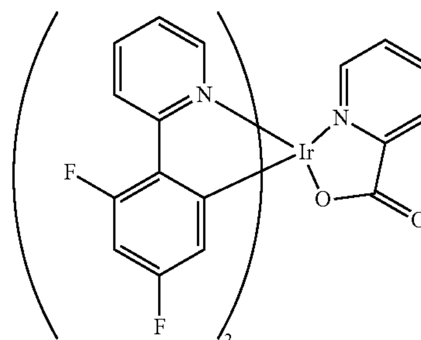
bis(2-[4,6-difluorophenyl]pyridinato-N,C2')iridium(III) picolinate [FIrPic]
