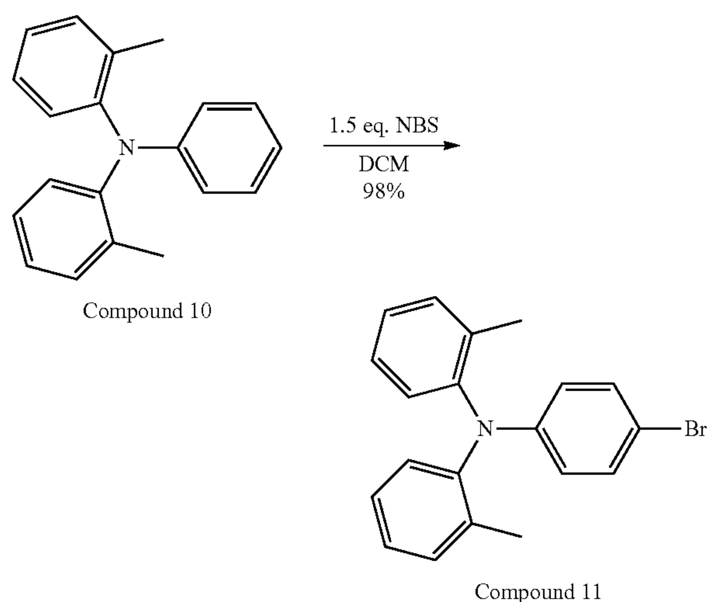
N-(4-bromophenyl)-2-methyl-N-(o-tolyl)aniline (Compound 11)
