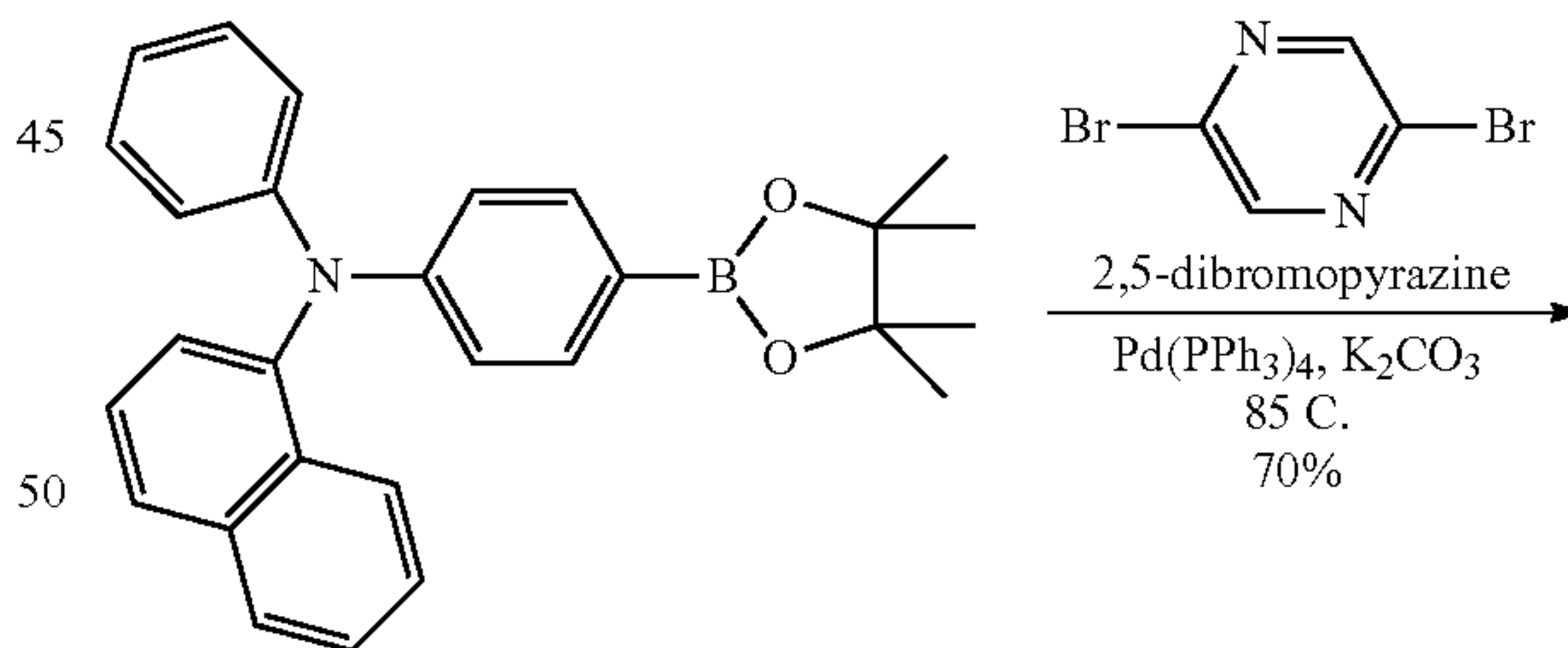
Compound 7
