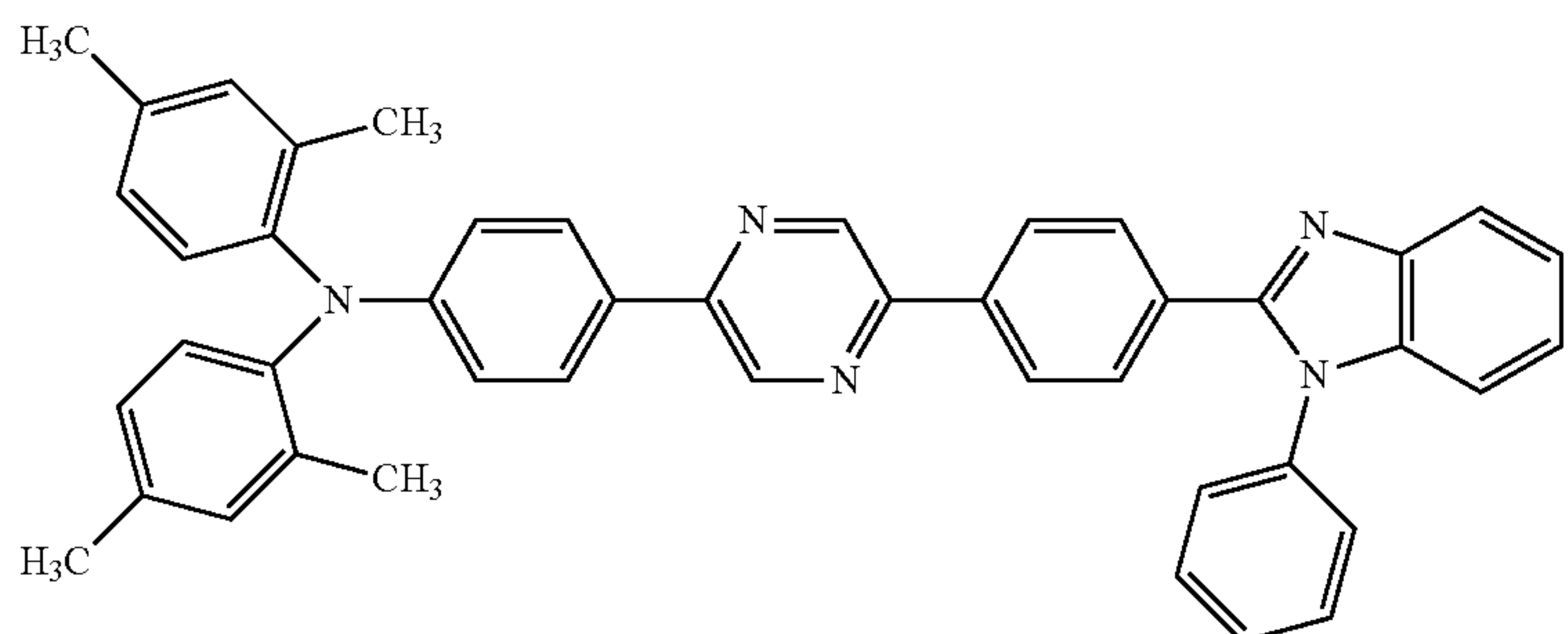
N-(2,4-dimethylphenyl)-2,4-dimethyl-N-(4-(5-(4-(1-phenyl-1H-benzo[d]imidazol-2-yl)phenyl)pyrazin-2-yl)phenyl)aniline
