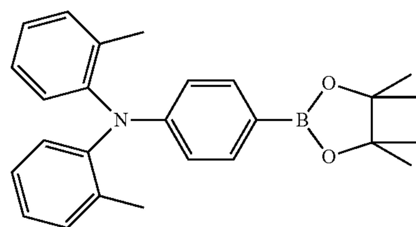
Compound 12
