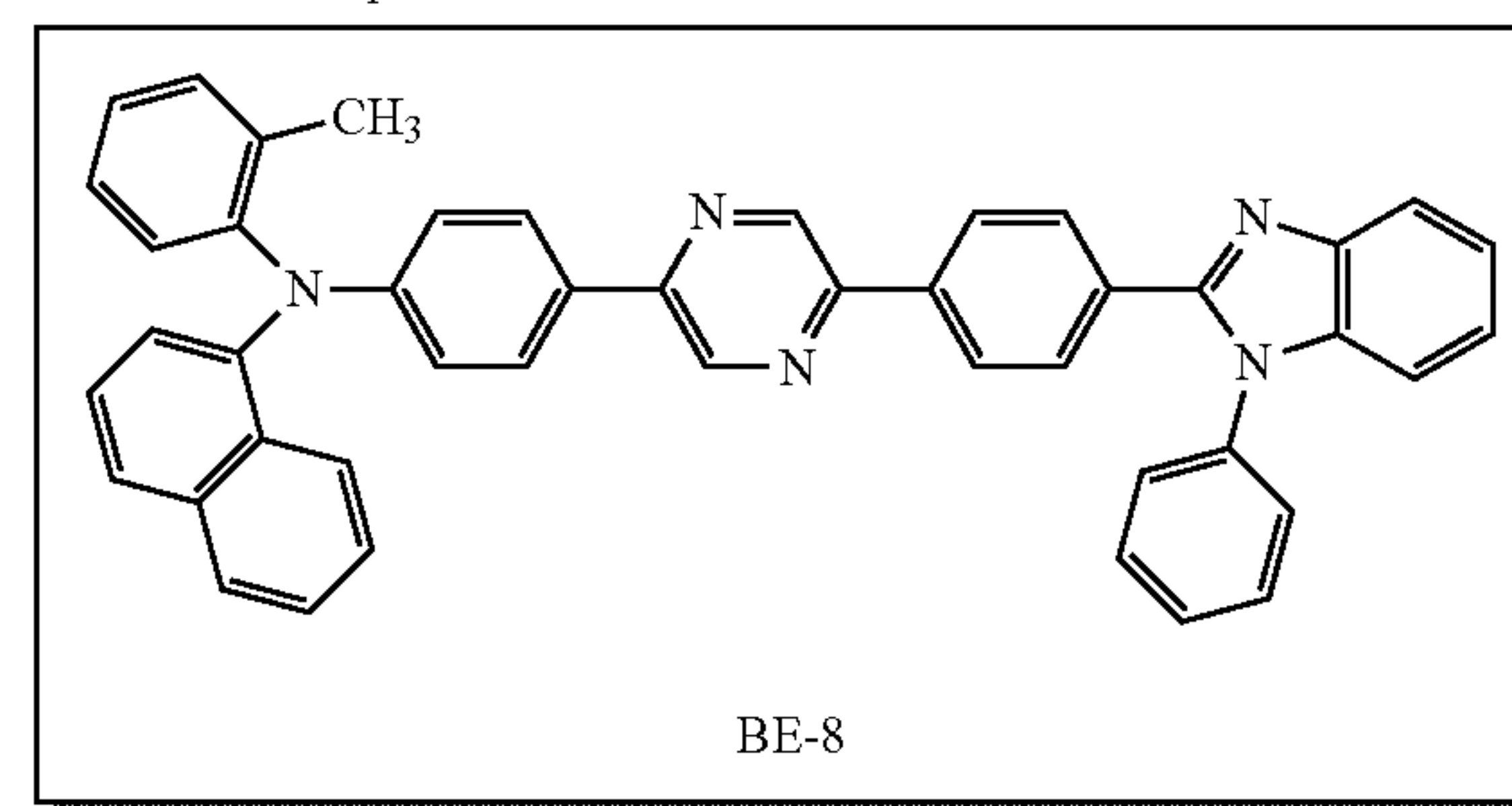
Compound 5
