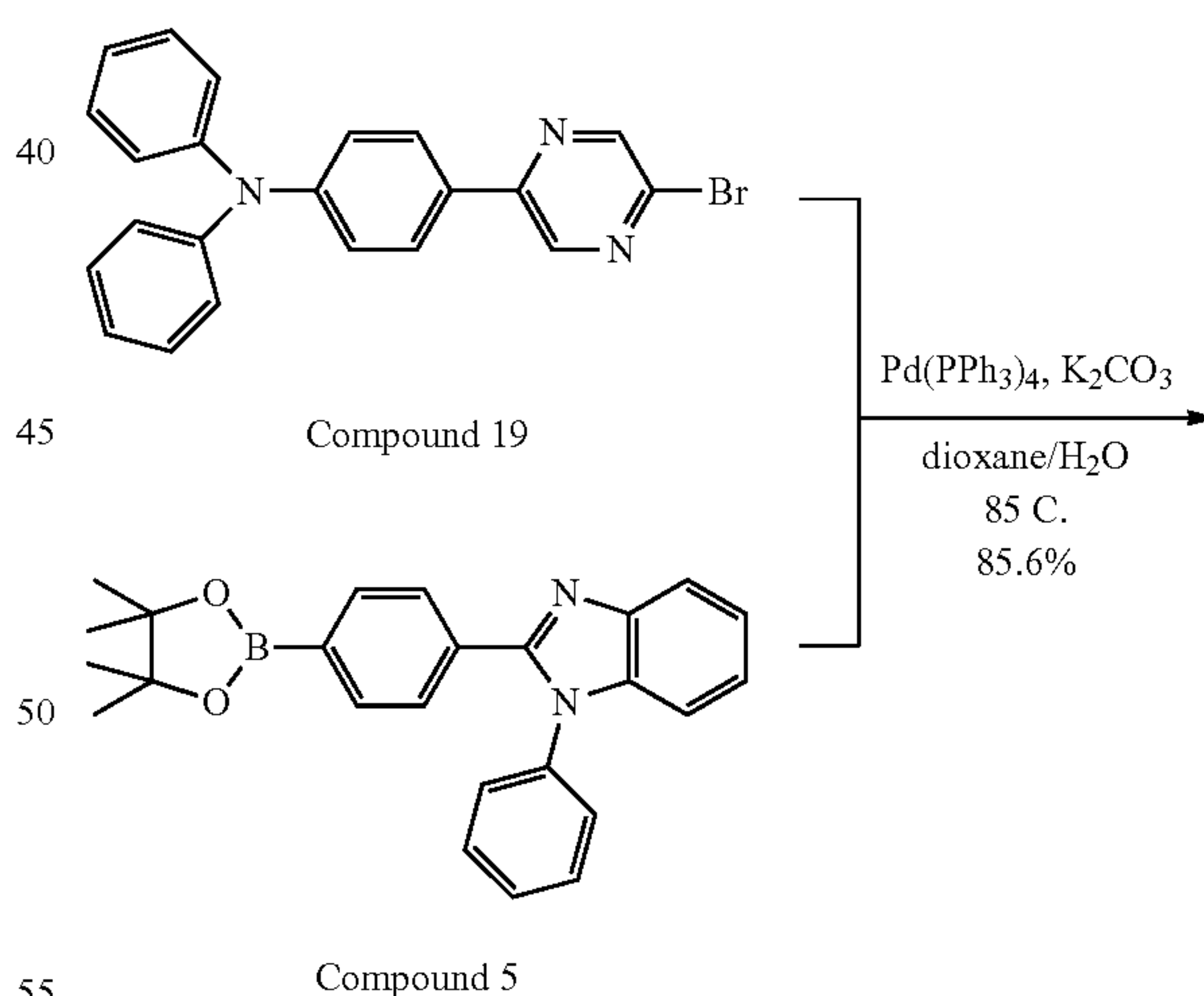
Compound 19
