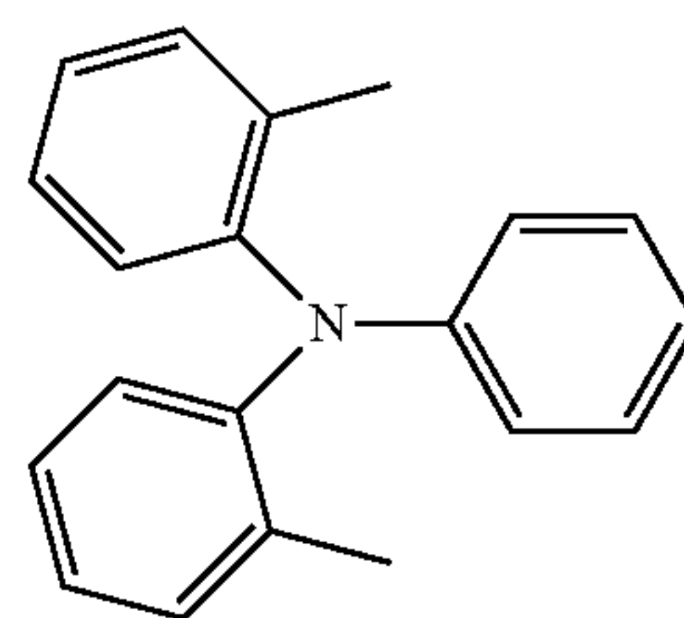
Compound 10
