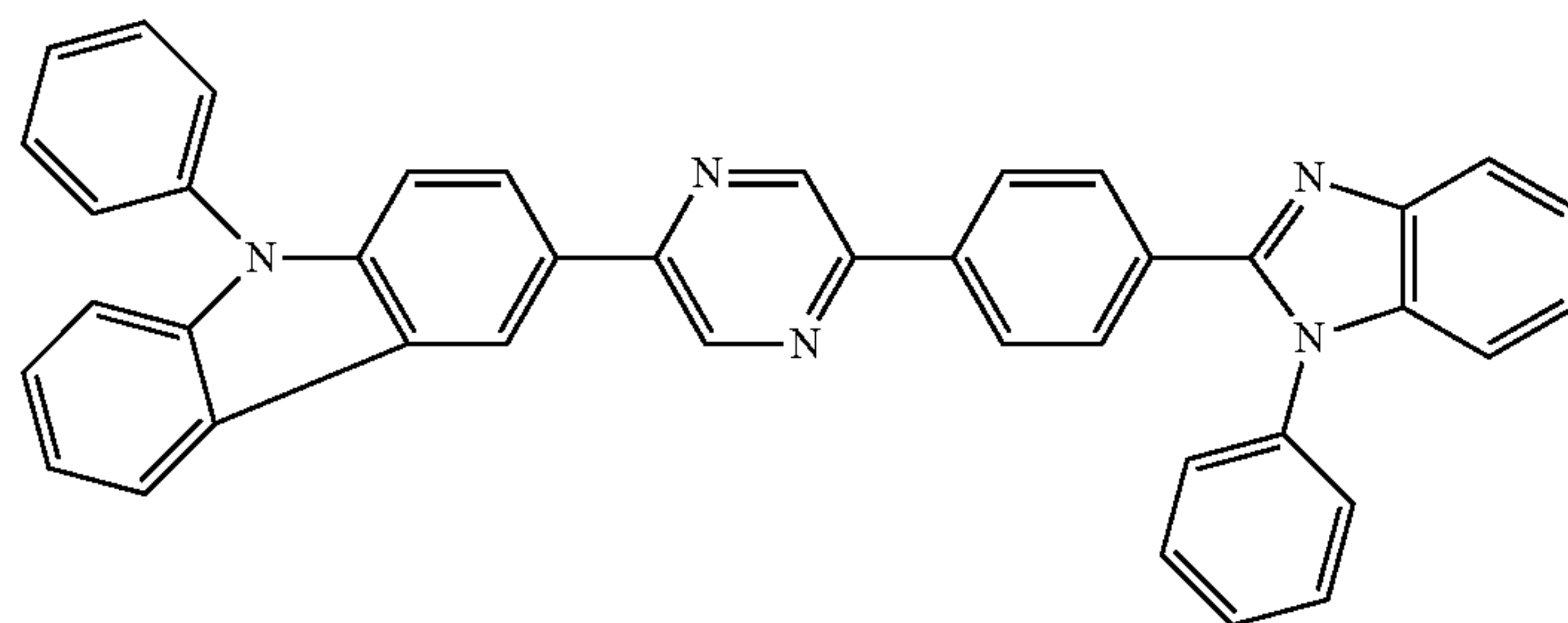
9-phenyl-3-(5-(4-(1-phenyl-1H-benzo[d]imidazol-2-yl)phenyl)pyrazin-2-yl)-9H-carbazole
