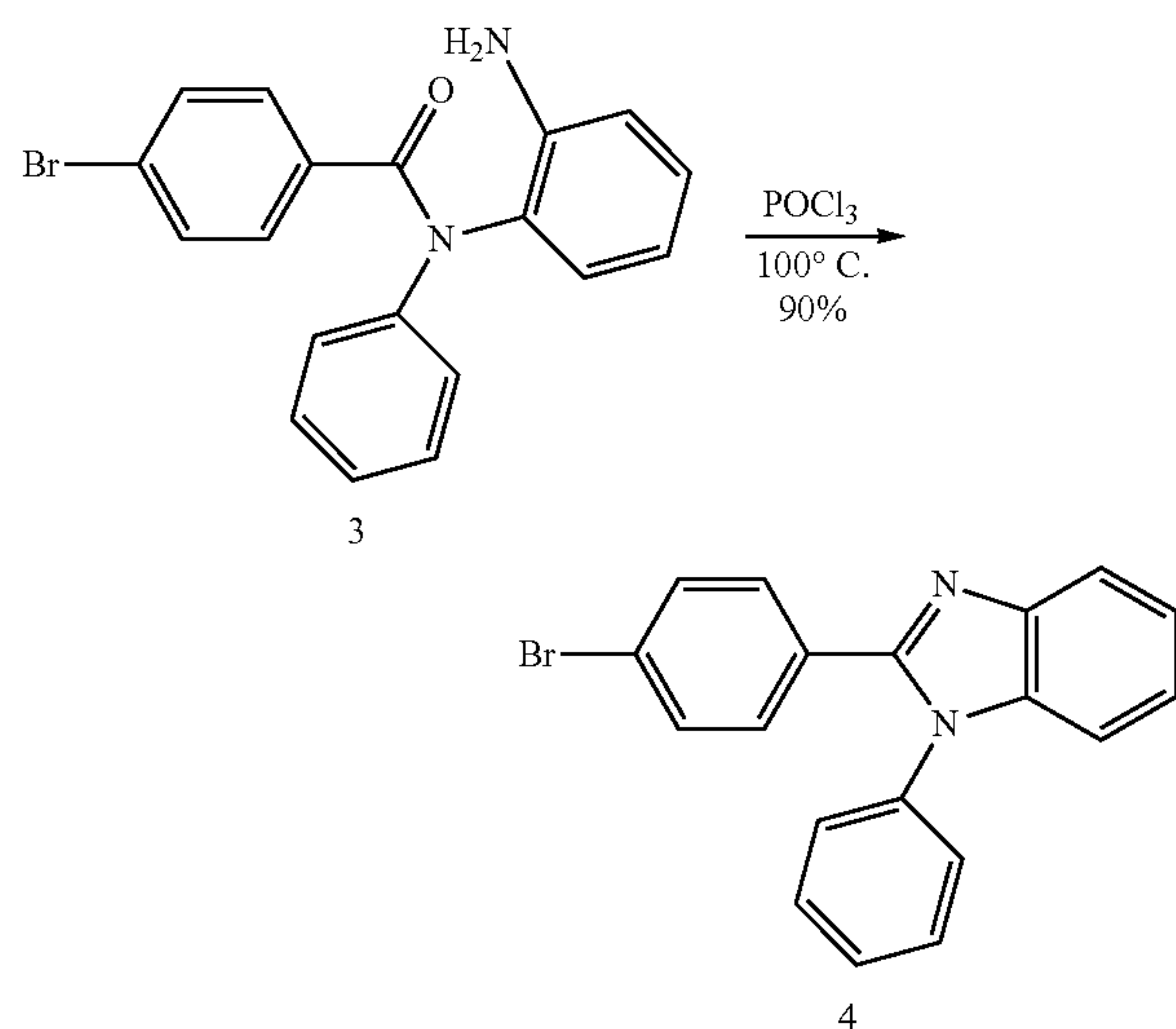
2-(4-bromophenyl)-1-phenyl-1H-benzo[d]imidazole (4)
