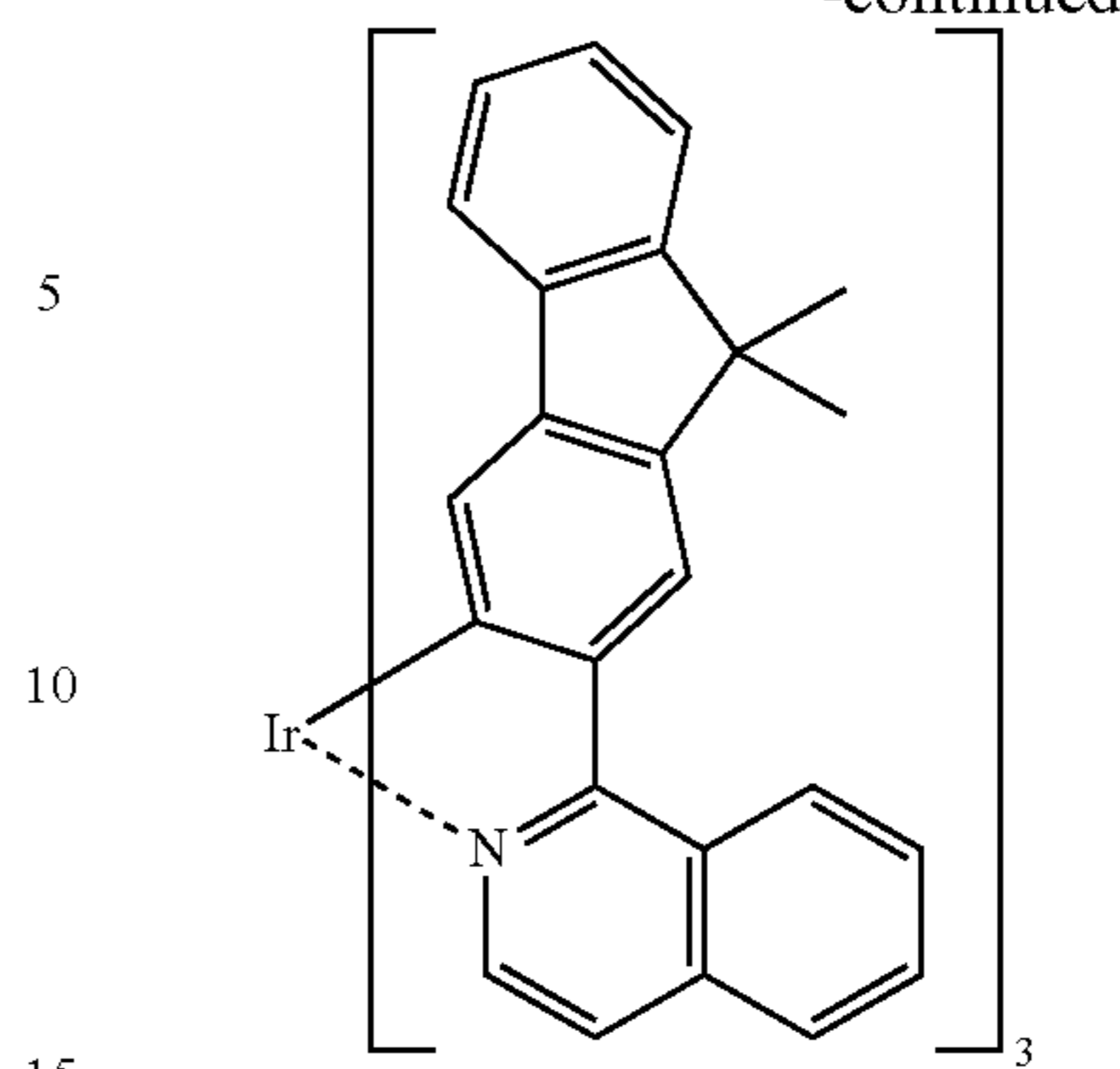
Ir(fliQ) 3 ; Ir(fliQ) 3 ; or Tris[1-(9,9-dimethyl-9H- fluoren-2-yl)isoquinolino- (N,C3')]iridium (III)
