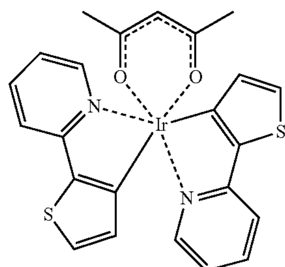
(thp) 2 Ir(III)(acac) Bis[(2-(2'-thienyl)- pyridinato-N,C3')]iridium (III) (acetylacetonate)
