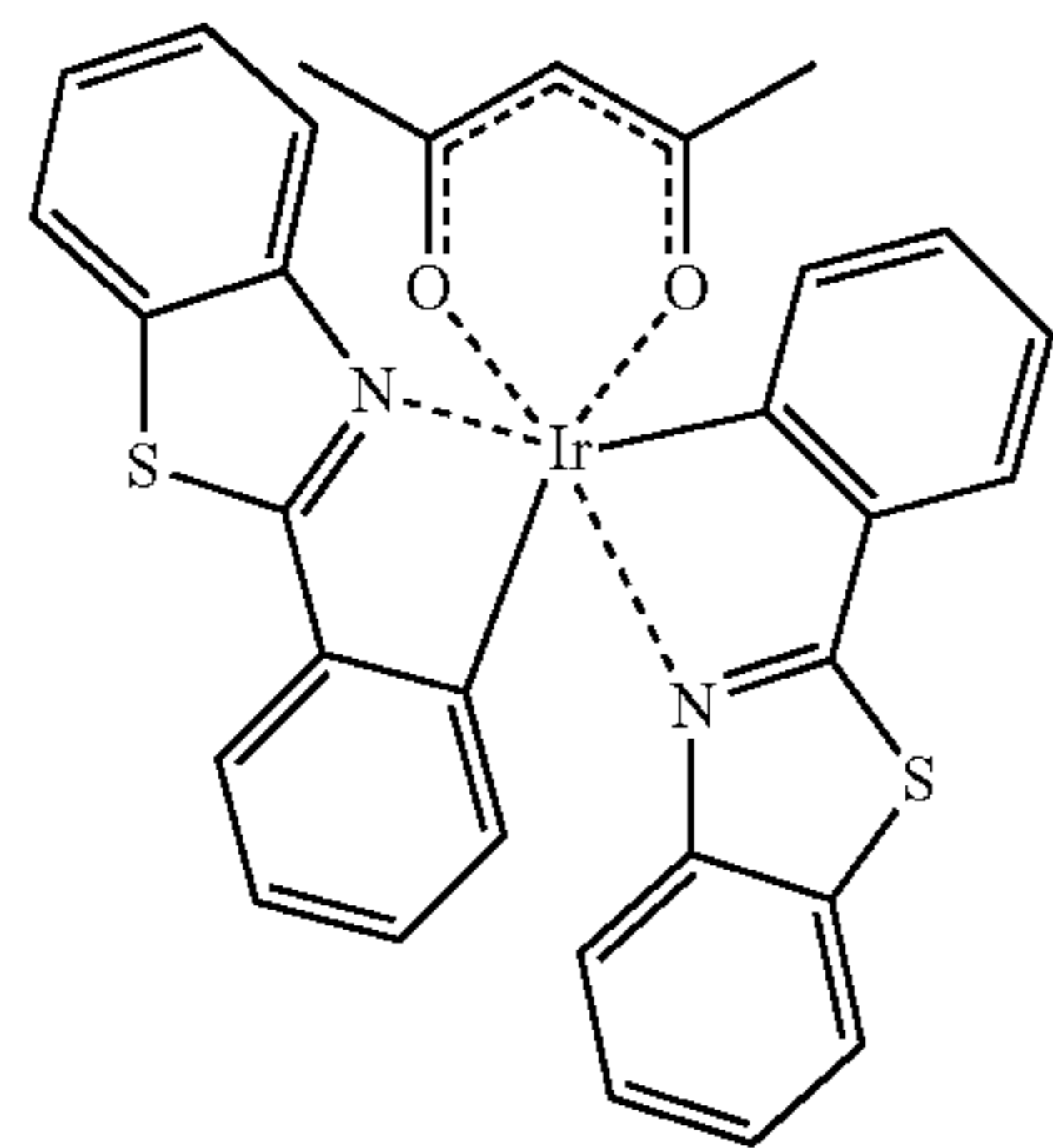
(bt) 2 Ir(III)(acac) Bis[2-phenylbenzothiazolato- N,C2'] iridium (III) (acetylacetonate)
