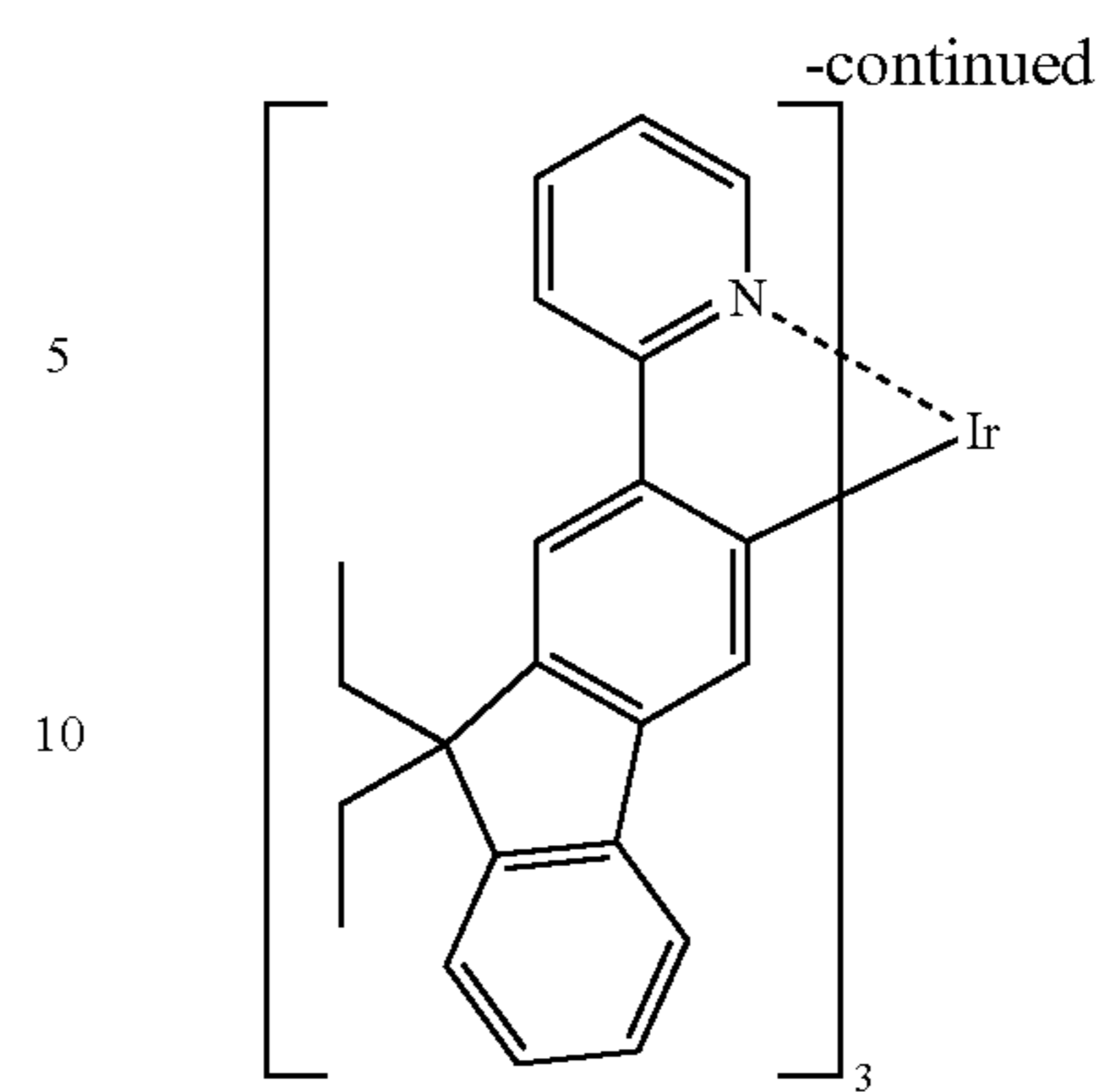
[Ir(Flpy) 3 ] Tris[2-(9,9- dimethylfluorene-2- yl)pyridinato- (N,C3')]iridium (III)
