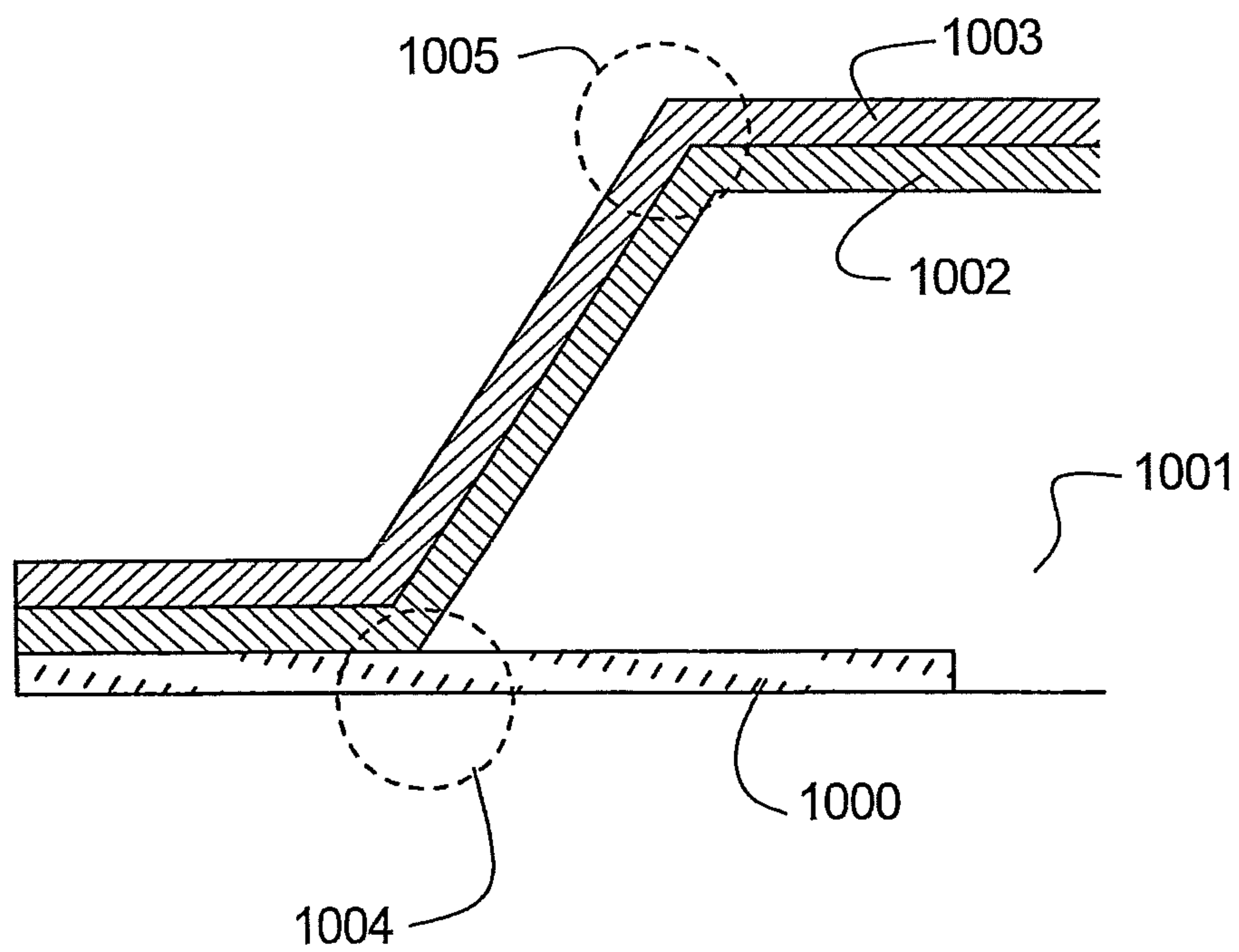
FIG. 18 PRIOR ART
