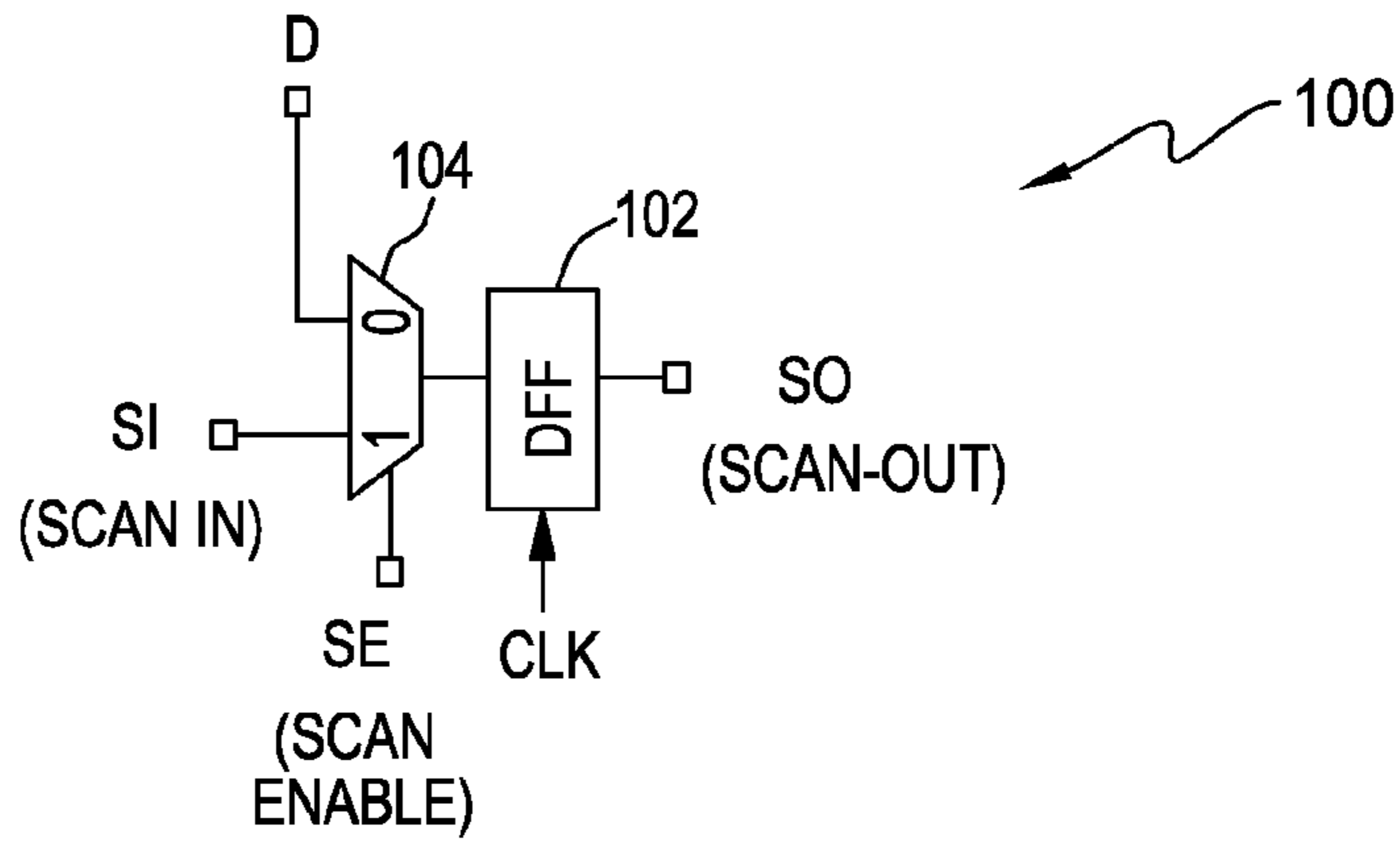
FIG. 1 PRIOR ART
