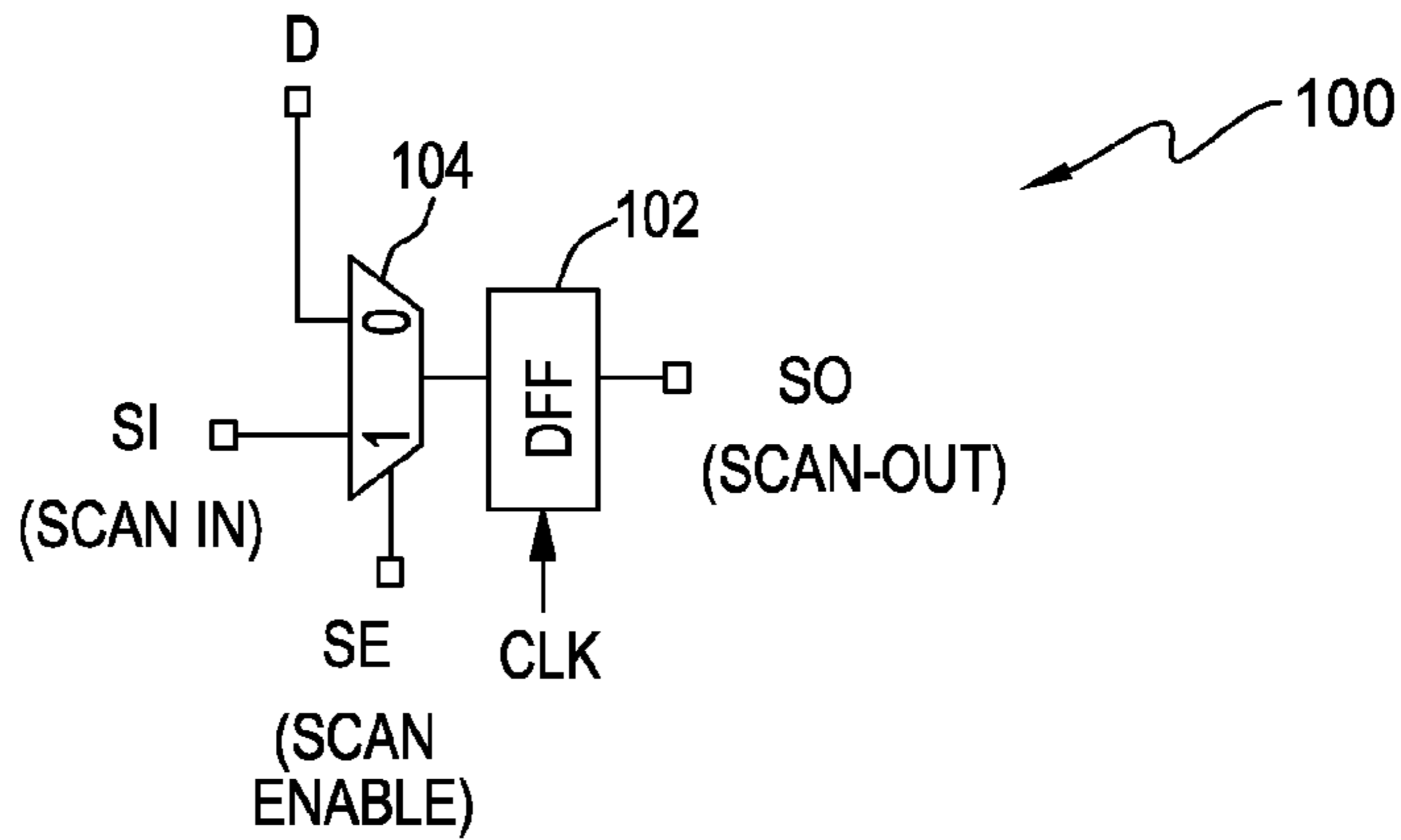
FIG. 1 PRIOR ART
