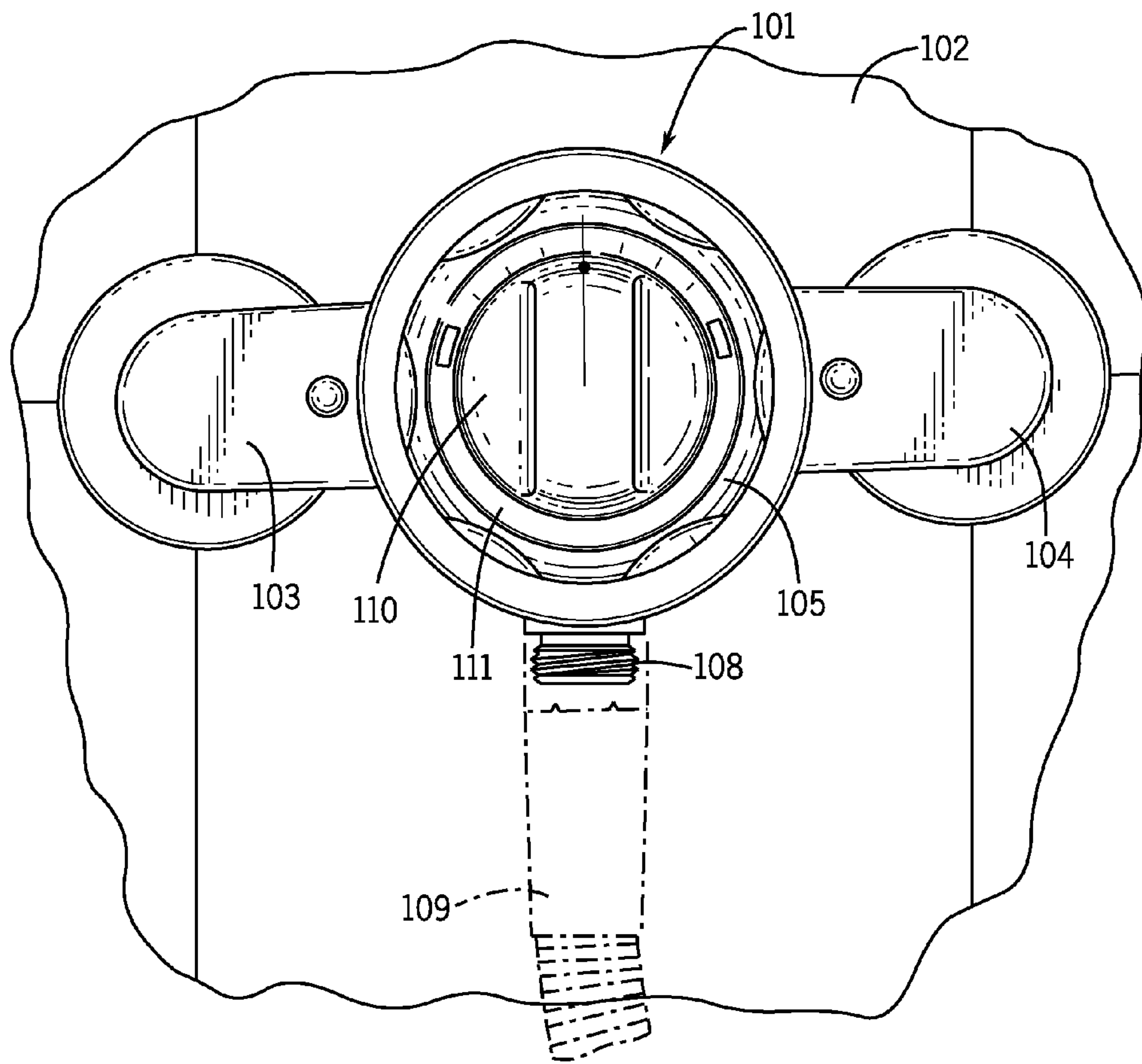
FIG. 12 PRIOR ART
