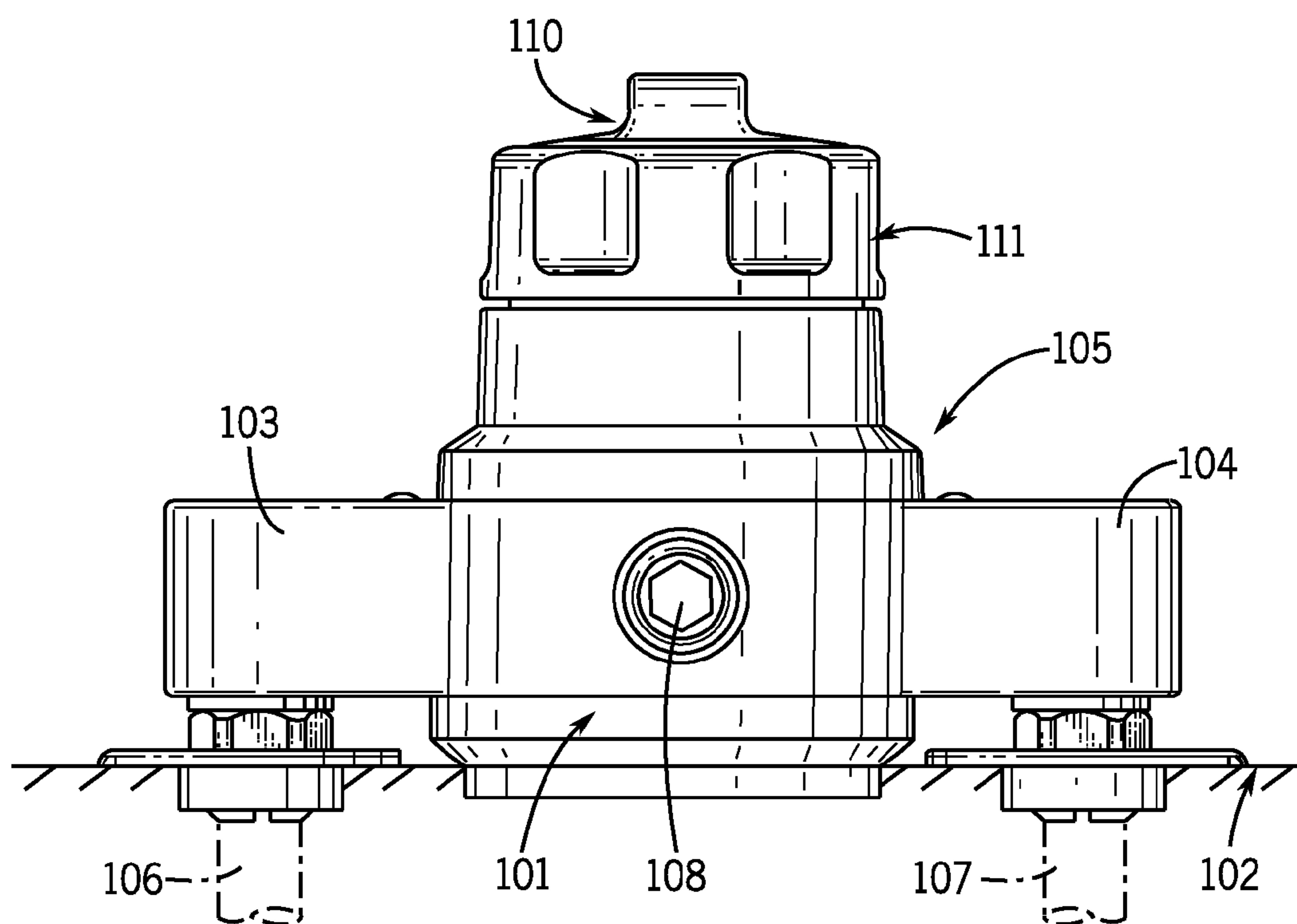
FIG. 13 PRIOR ART
