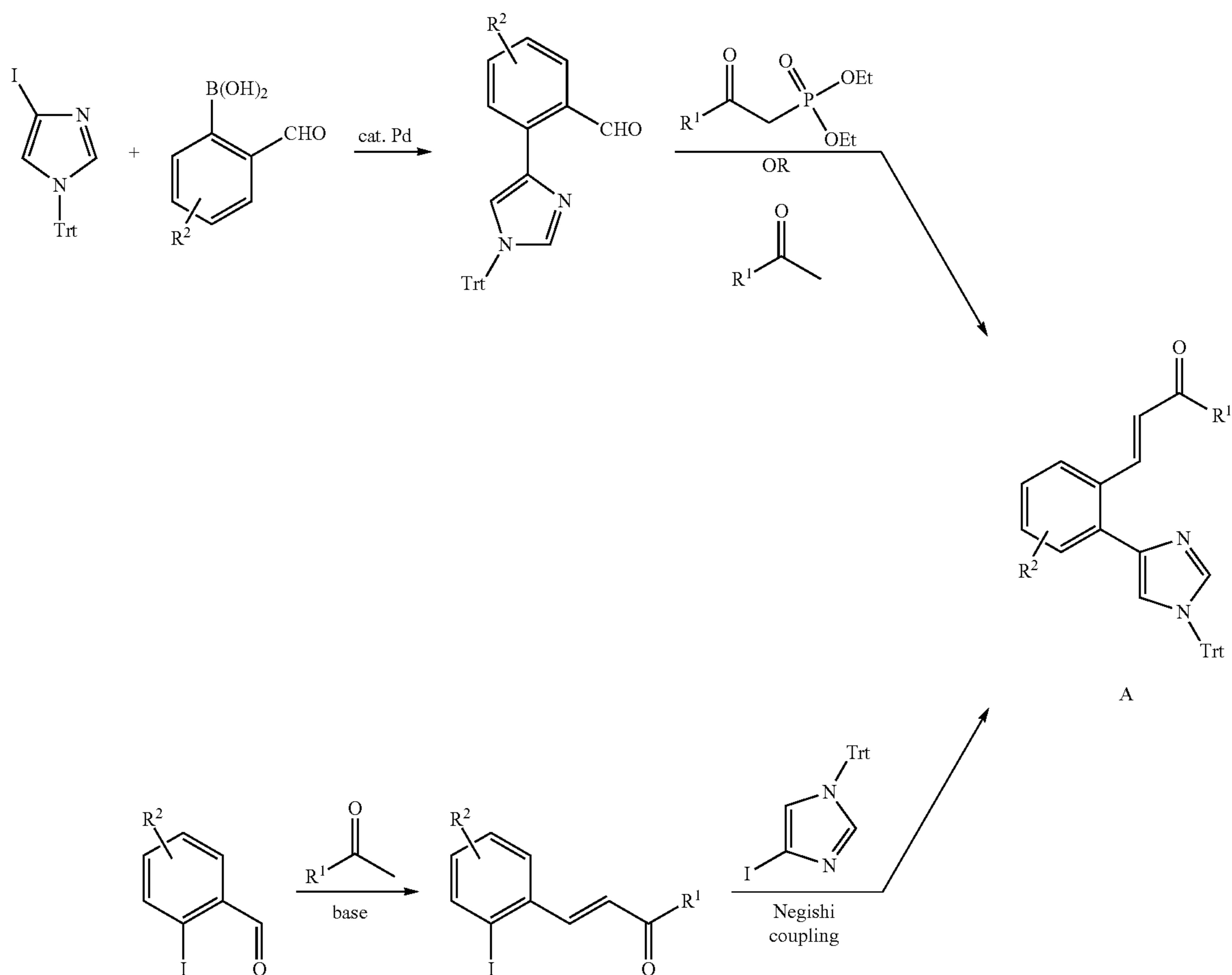
Scheme 2. Synthesis of 2-(5H-imidazo[5,1-a]isoindol-5-yl)ethanones and Their Corresponding 2-(5H-imidazo[5,1-a]isoindol-5-yl)ethanols
