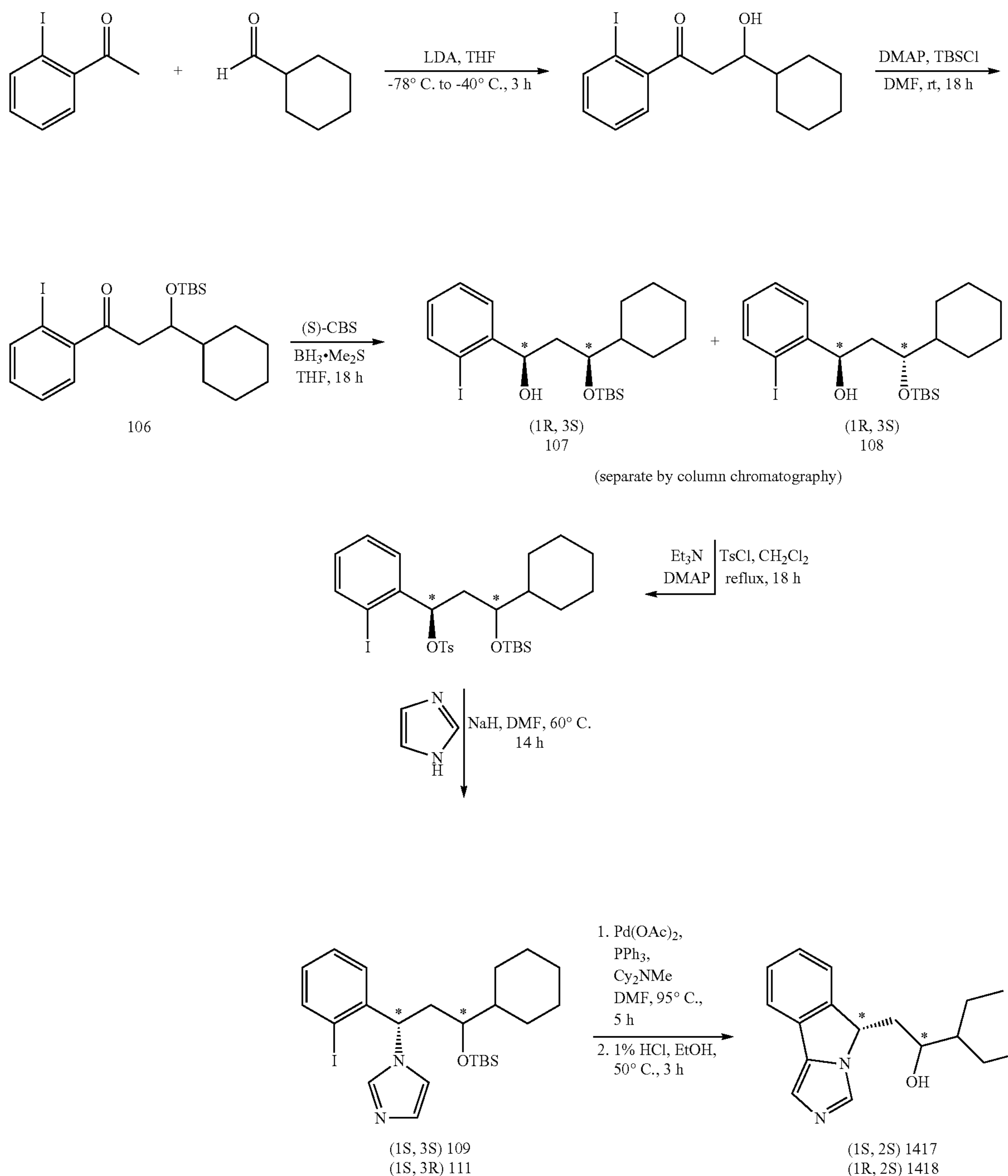
Scheme 3. Enantioselective Synthesis of (S)-1-cyclohexyl-2-((S)-5H-imidazo[5,1-a]isoindol-5-yl)ethanol (1417) and (R)-1-cyclohexyl-2-((S)-5H-imidazo[5,1-a]isoindol-5-yl)ethanol (1418) SCHEME 3
