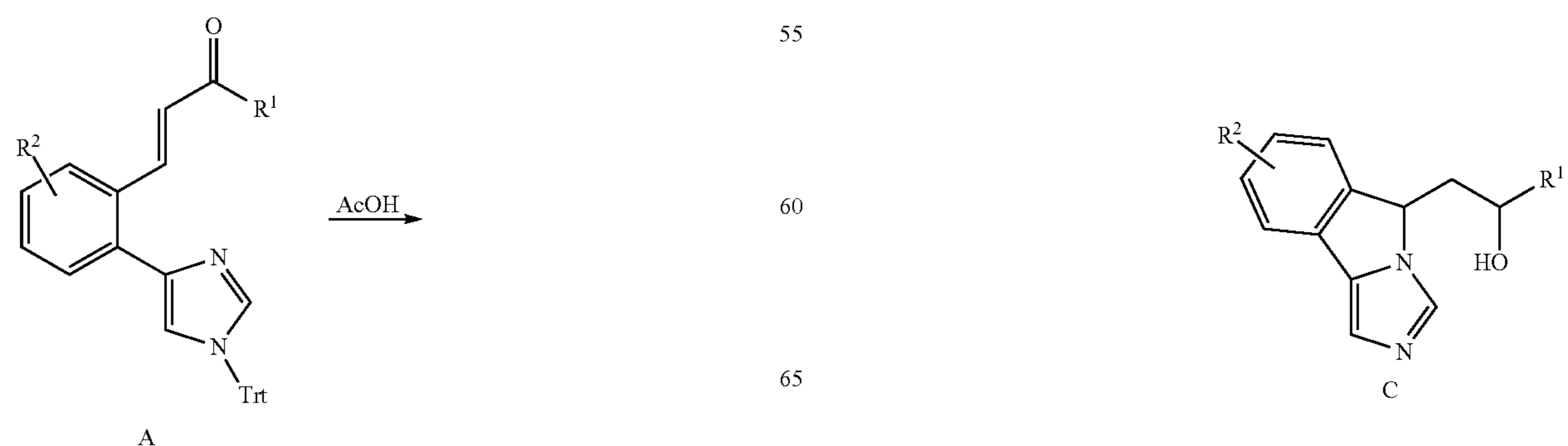
Scheme 2. Synthesis of 2-(5H-imidazo[5,1-a]isoindol-5-yl)ethanones and Their Corresponding 2-(5H-imidazo[5,1-a]isoindol-5-yl)ethanols
