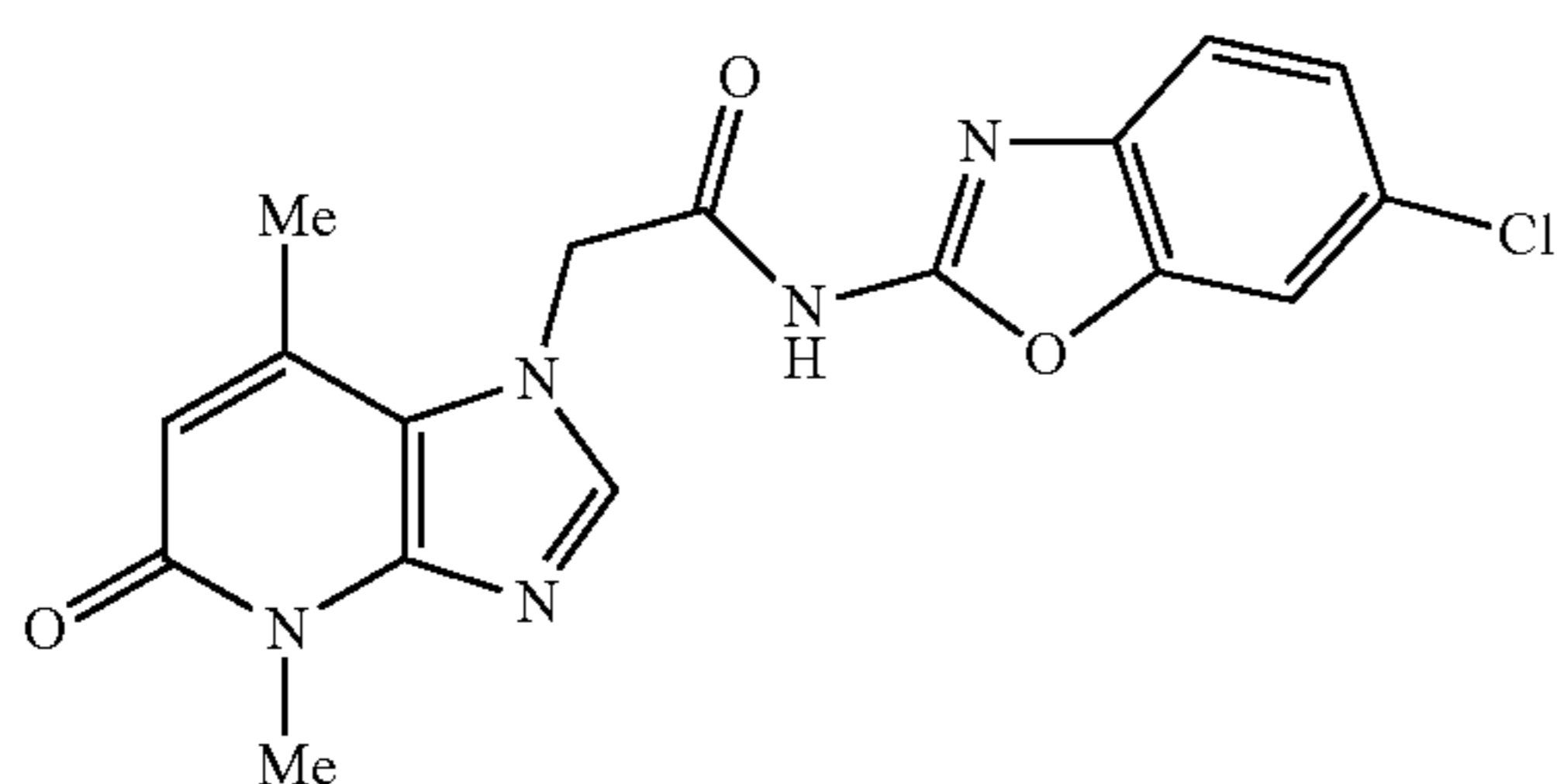
N-(6-chlorobenzo[d]oxazol-2-yl)-2-(4,7-dimethyl-5-oxo-4,5-dihydro-1H-imidazo[4,5-b]pyridin-1-yl)acetamide
