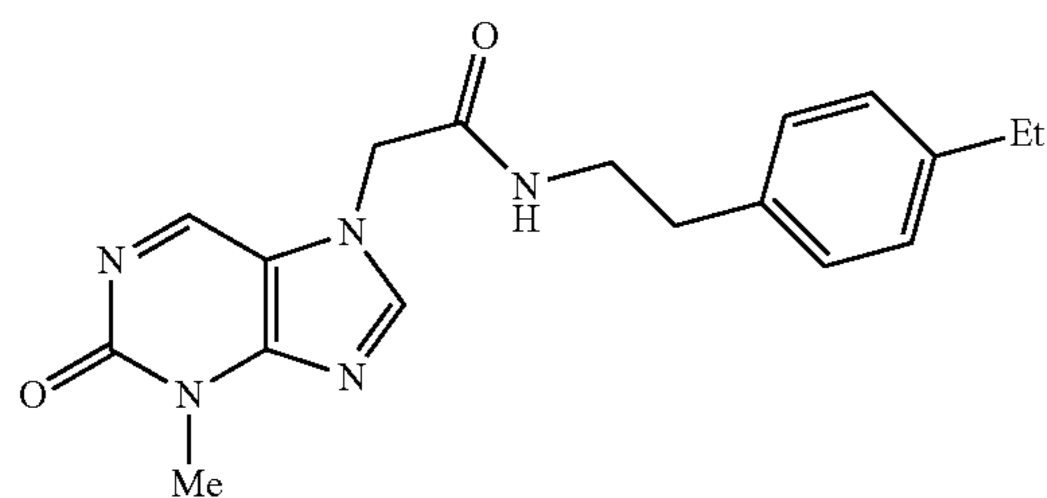
N-(4-ethylphenethyl)-2-(3-methyl-2-oxo-2,3-dihydropurin-7-yl)acetamide
