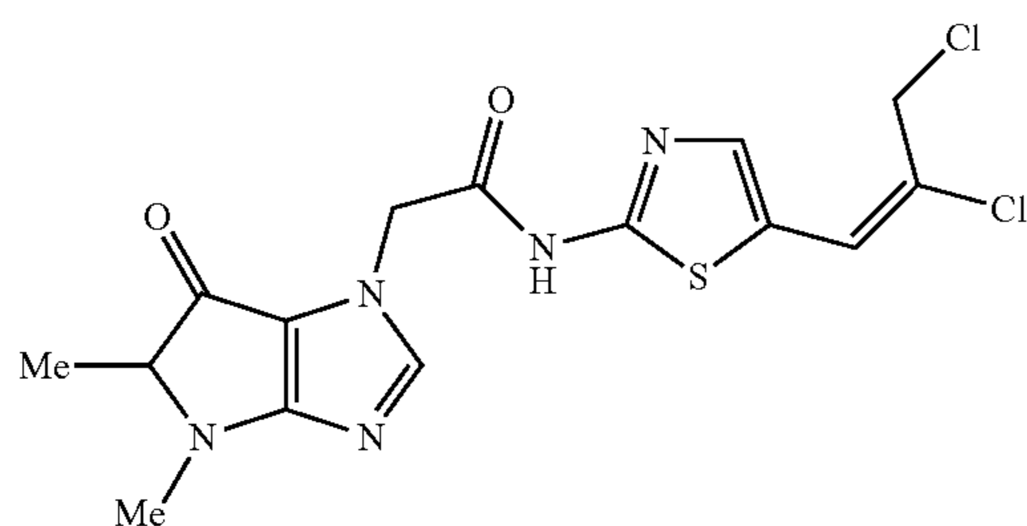
(E)-N-(5-(2,3-dichloroprop-1-enyl)thiazol-2-yl)-2-(4,5-dimethyl-6-oxo-5,6-dihydropyrrolo[3,2-d]imidazol-1(4H)-yl)acetamide
