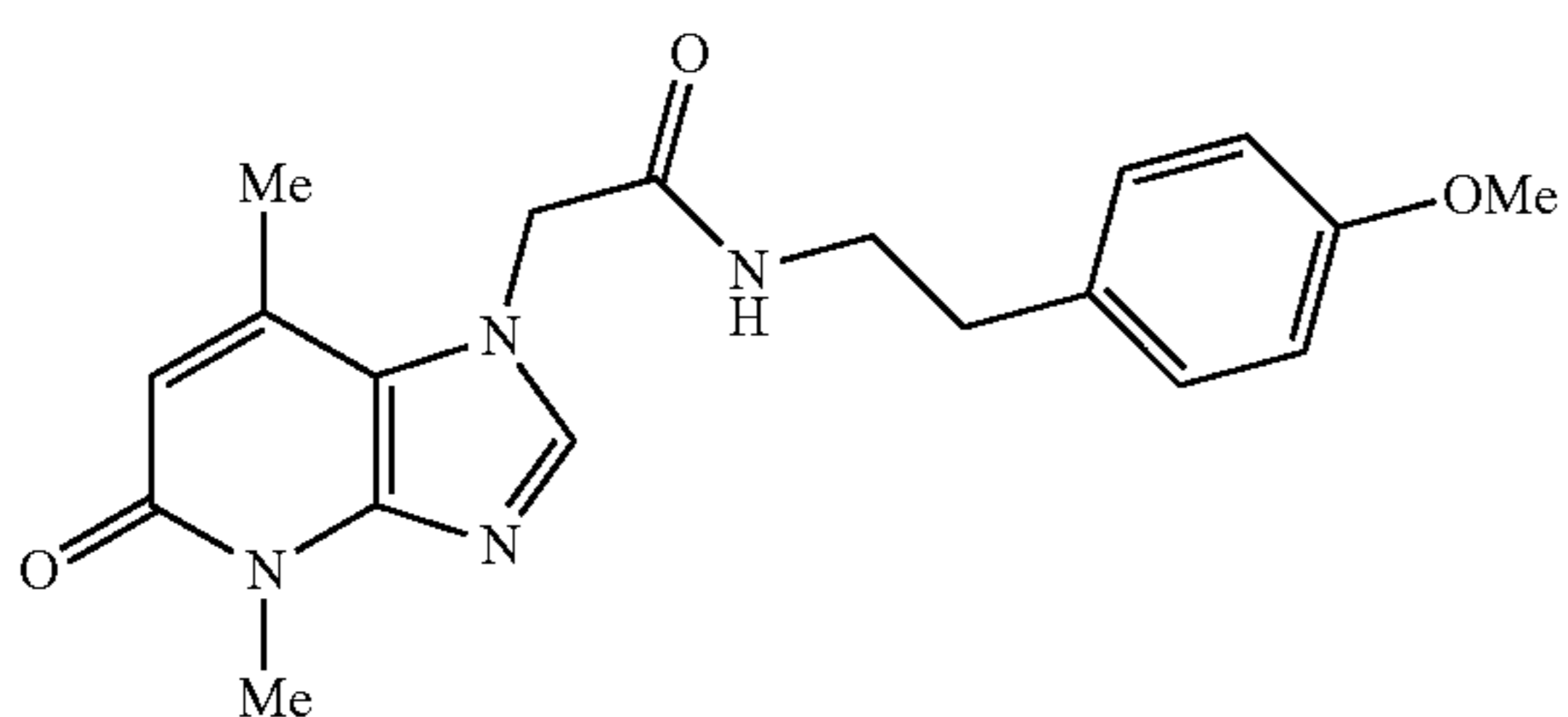
2-(4,7-dimethyl-5-oxo-4,5-dihydro-1H-imidazo[4,5-b]pyridin-1-yl)-N-(4-methoxyphenethyl)acetamide
