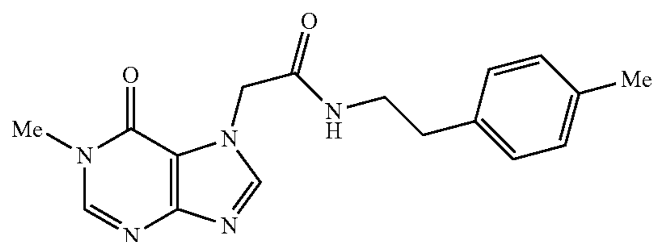
2-(1-methyl-6-oxo-1H-purin-7(6H)-yl)-N-(4-methylphenethyl)acetamide
