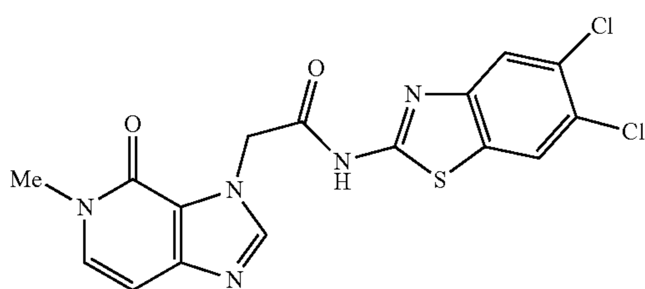
N-(5,6-dichlorobenzo[d]thiazol-2-yl)-2-(5-methyl-4-oxo-4,5-dihydro-3H-imidazo[4,5-c]pyridin-3-yl)acetamide
