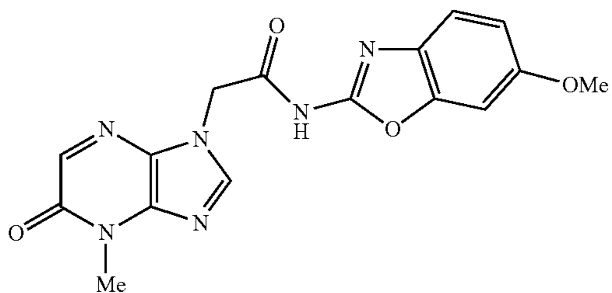
N-(6-methoxybenzo[d]oxazol-2-yl)-2-(4-methyl-5-oxo-4,5-dihydro-1H-imidazo[4,5-b]pyridin-1-yl)acetamide
