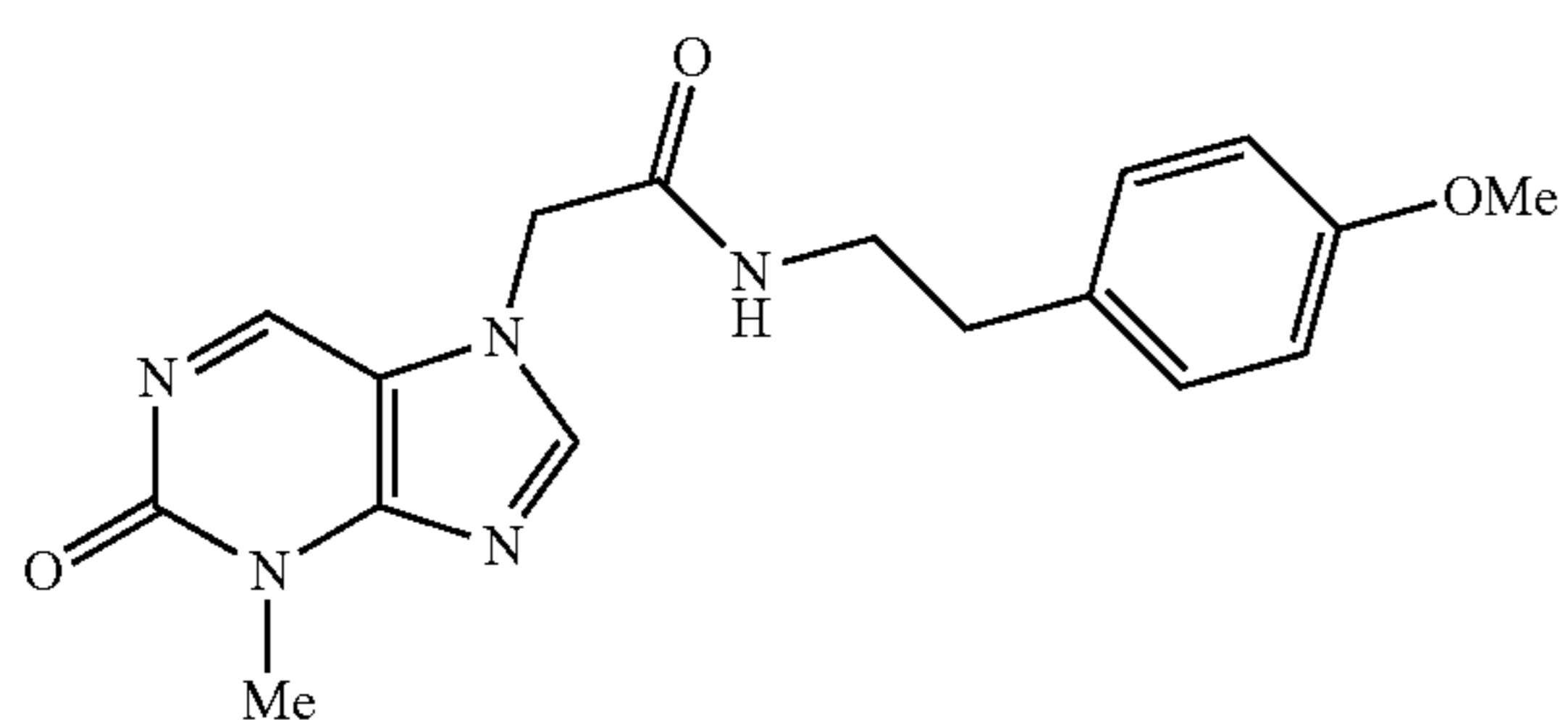
N-(4-methoxyphenethyl)-2-(3-methyl-2-oxo-2,3-dihydropurin-7-yl)acetamide
