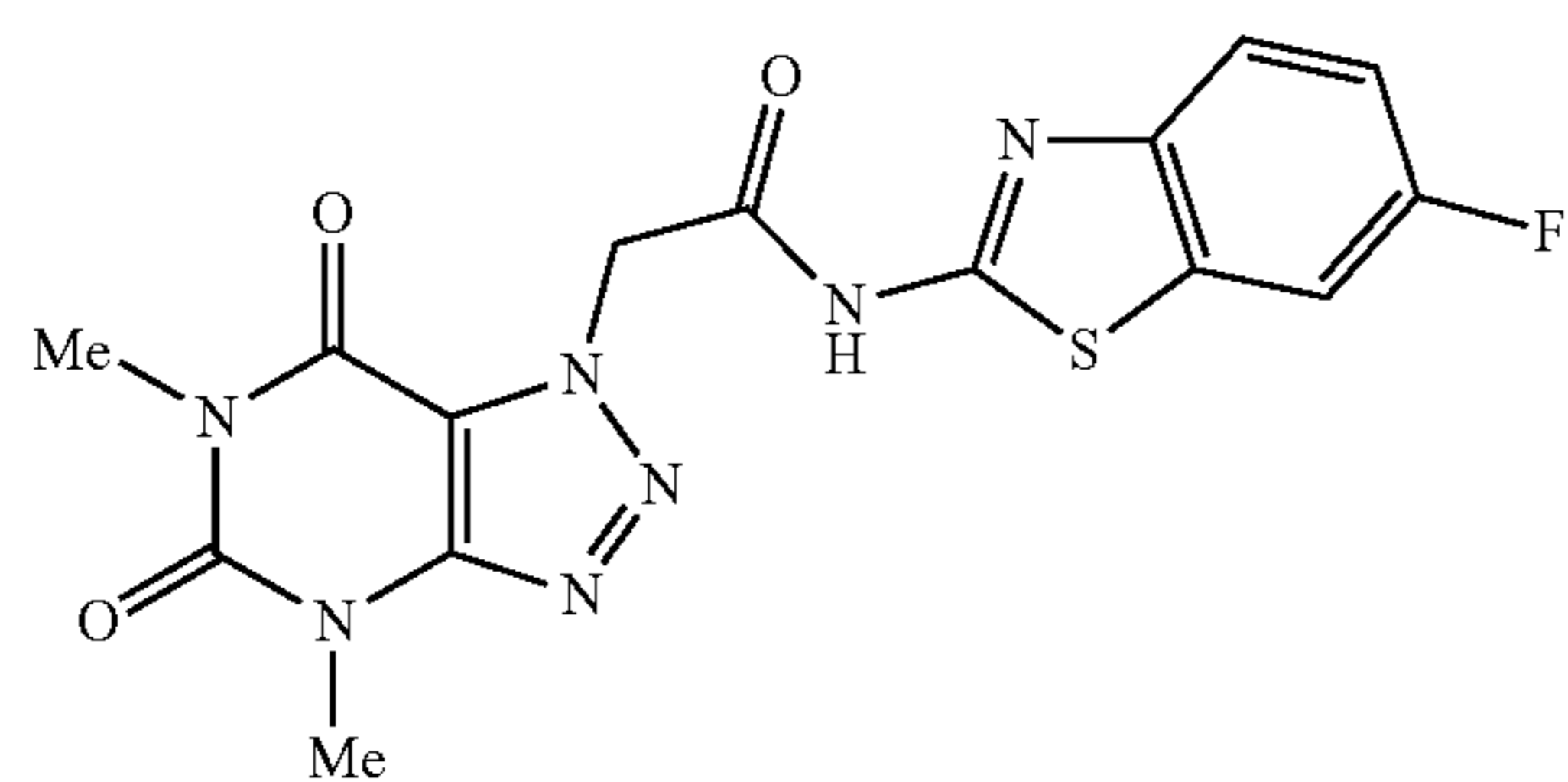
2-(4,6-dimethyl-5,7-dioxo-4,5,6,7-tetrahydro-1H-[1,2,3]triazolo[4,5-d]pyrimidin-1-yl)-N-(6-fluorobenzo[d]thiazol-2-yl)acetamide
