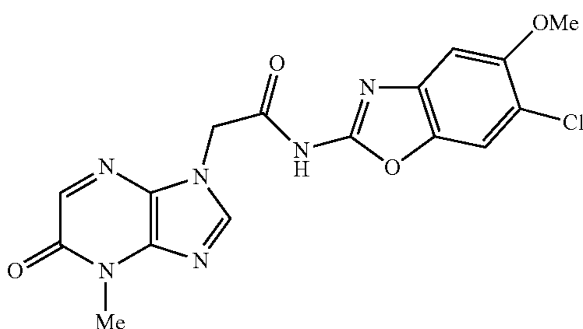
N-(6-chloro-5-methoxybenzo[d]oxazol-2-yl)-2-(4-methyl-5-oxo-4,5-dihydro-1H-imidazo[4,5-b]pyridin-1-yl)acetamide
