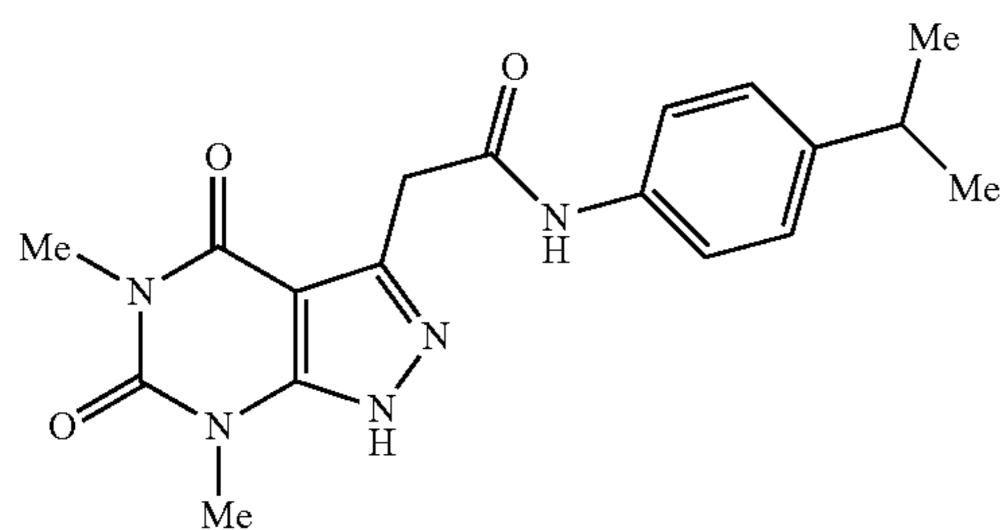
2-(5,7-dimethyl-4,6-dioxo-4,5,6,7-tetrahydro-1H-pyrazolo[3,4-d]pyrimidin-3-yl)-N-(4-isopropylphenyl)acetamide
