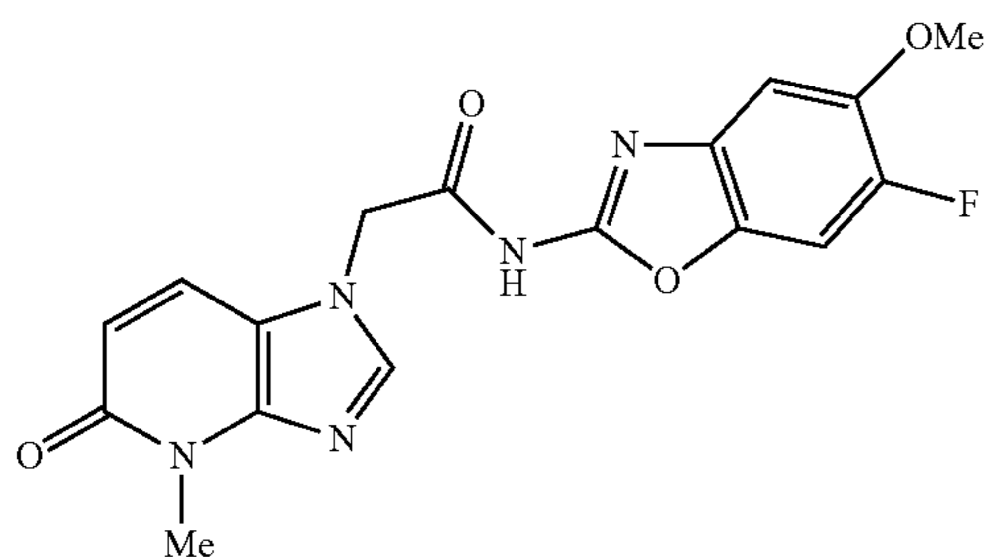
N-(6-fluoro-5-methoxybenzo[d]oxazol-2-yl)-2-(4-methyl-5-oxo-4,5-dihydro-1H-imidazo[4,5-b]pyridin-1-yl)acetamide
