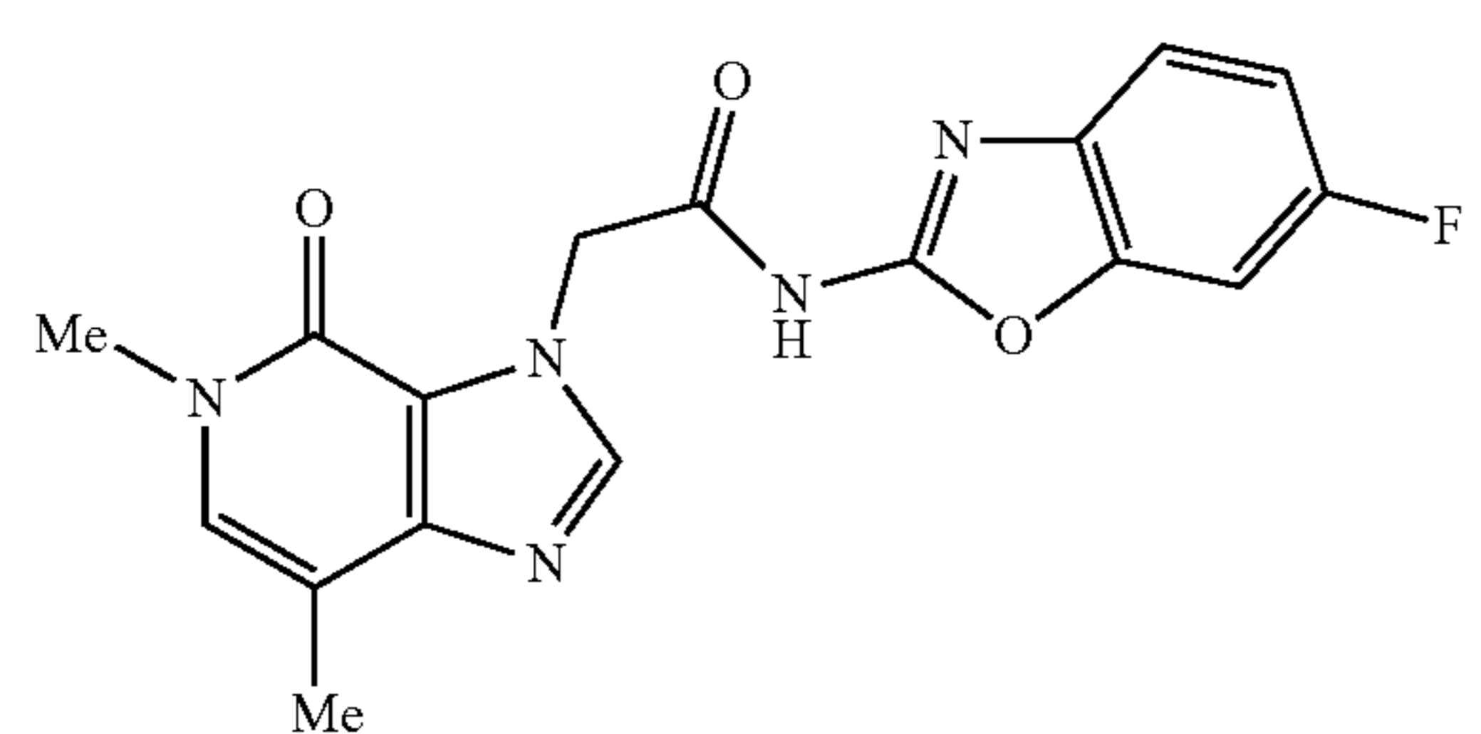
2-(5,7-dimethyl-4-oxo-4,5-dihydro-3H-imidazo[4,5-c]pyridin-3-yl)-N-(6-fluorobenzo[d]oxazol-2-yl)acetamide
