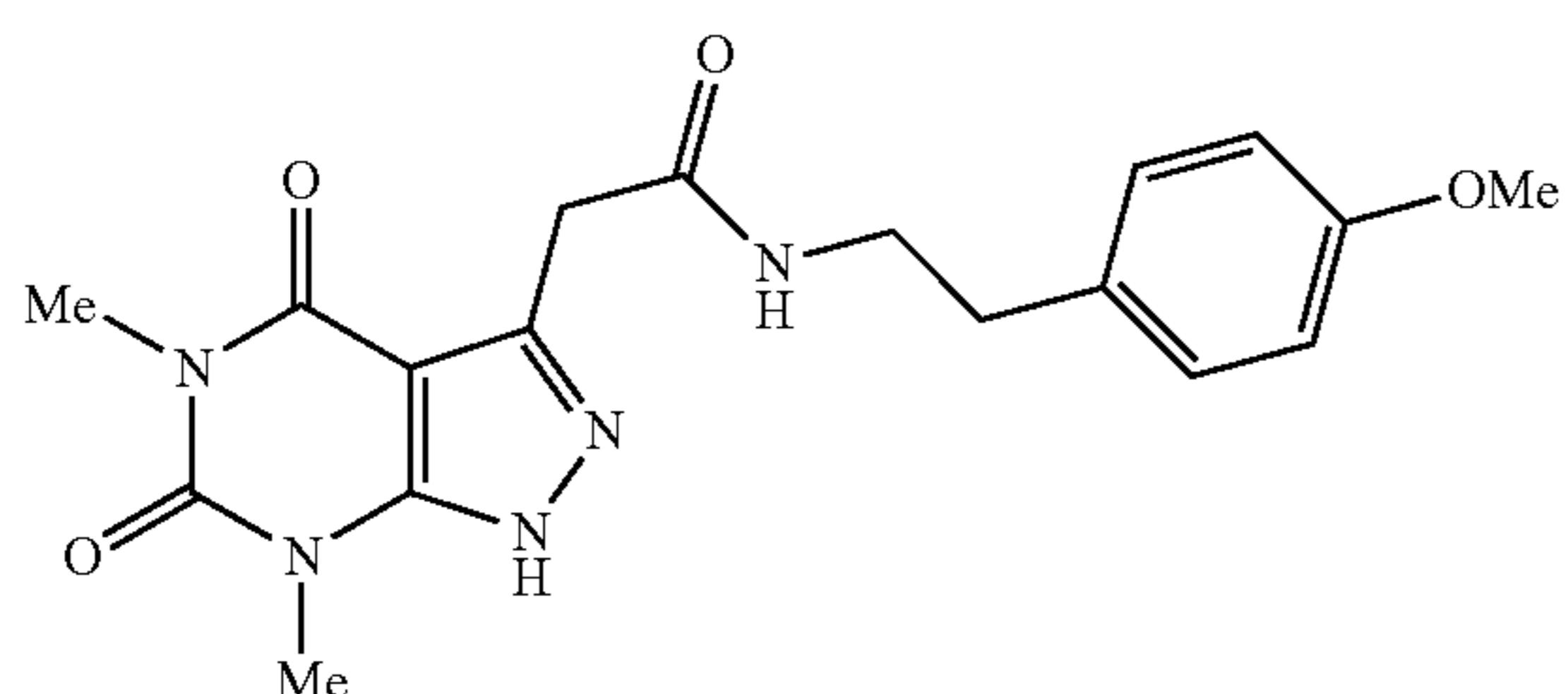
2-(5,7-dimethyl-4,6-dioxo-4,5,6,7-tetrahydro-1H-pyrazolo[3,4-d]pyrimidin-3-yl)-N-(4-methoxyphenethyl)acetamide
