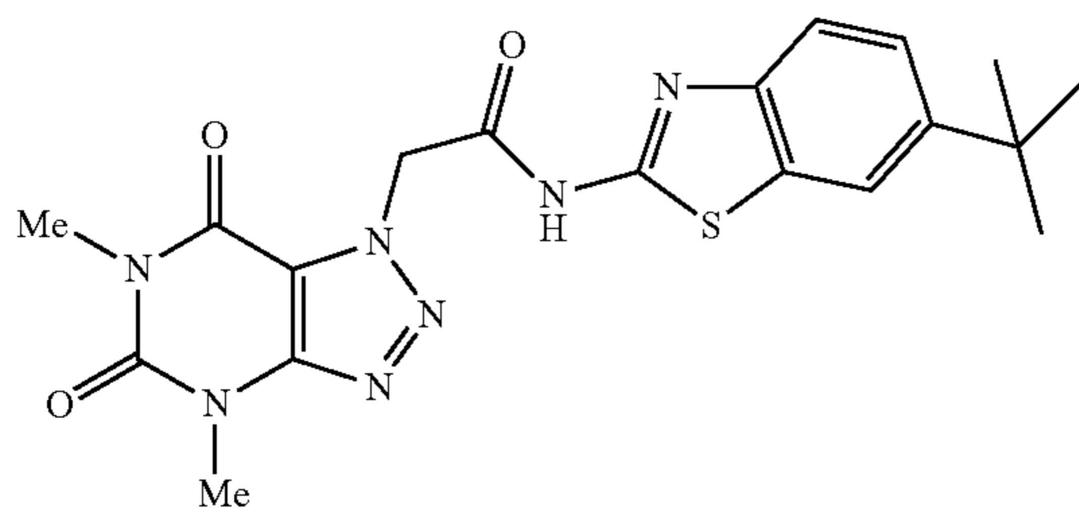
N-(6-tert-butylbenzo[d]thiazol-2-yl)-2-(4,6-dimethyl-5,7-dioxo-4,5,6,7-tetrahydro-1H-[1,2,3]triazolo[4,5-d]pyrimidin-1-yl)acetamide
