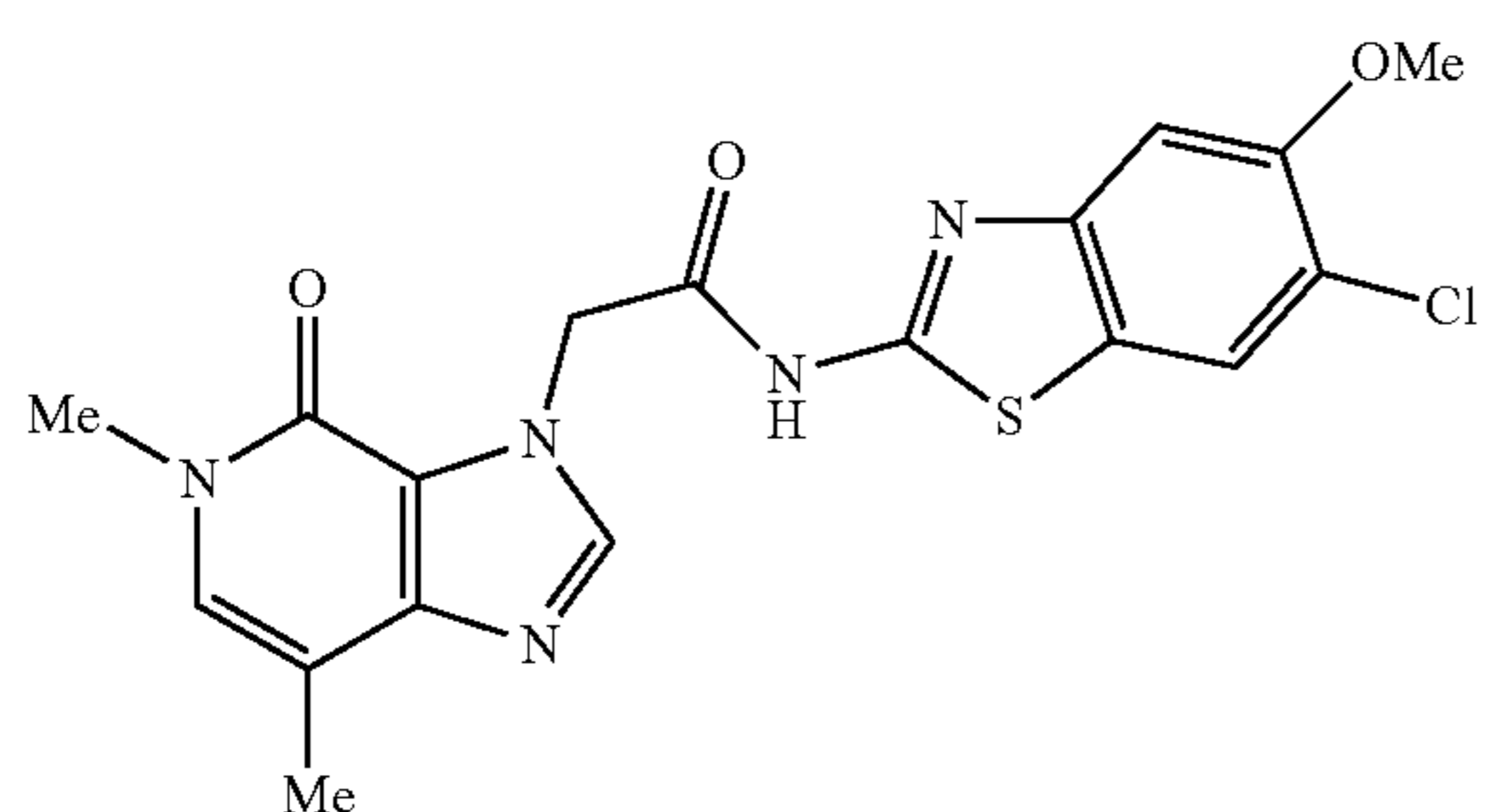
N-(6-chloro-5-methoxybenzo[d]thiazol-2-yl)-2-(5,7-dimethyl-4-oxo-4,5-dihydro-3H-imidazo[4,5-c]pyridin-3-yl)acetamide
