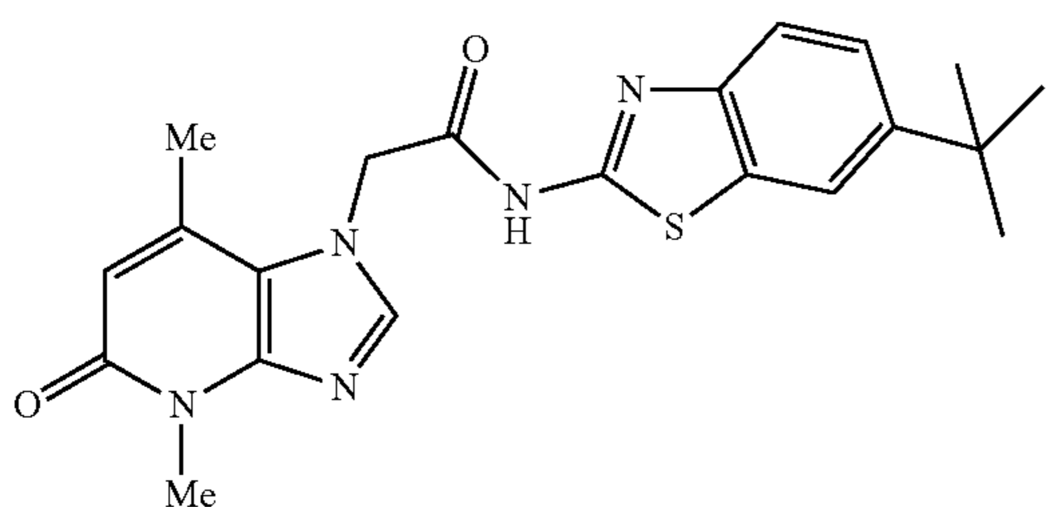
N-(6-tert-butylbenzo[d]thiazol-2-yl)-2-(4,7-dimethyl-5-oxo-4,5-dihydro-1H-imidazo[4,5-b]pyridin-1-yl)acetamide
