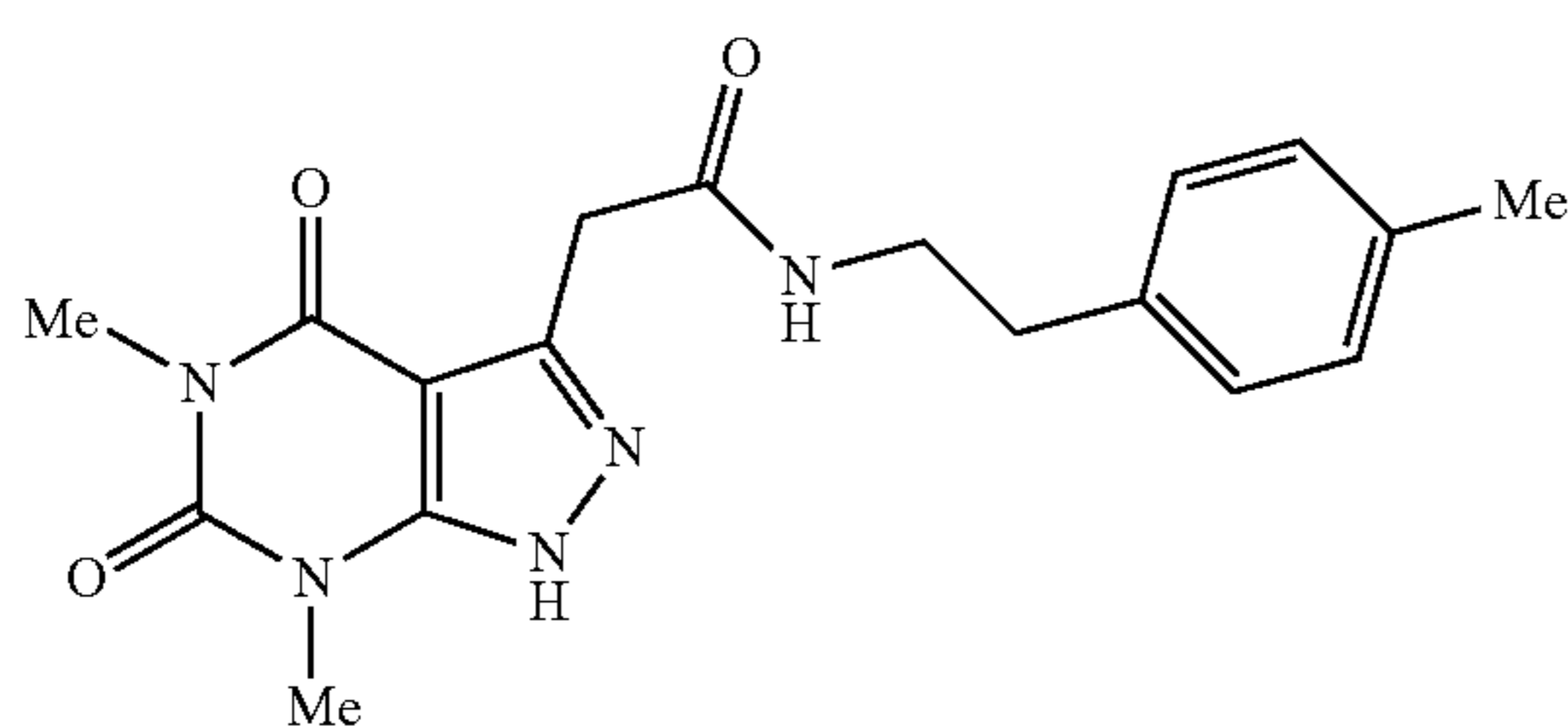
2-(5,7-dimethyl-4,6-dioxo-4,5,6,7-tetrahydro-1H-pyrazolo[3,4-d]pyrimidin-3-yl)-N-(4-methylphenethyl)acetamide
