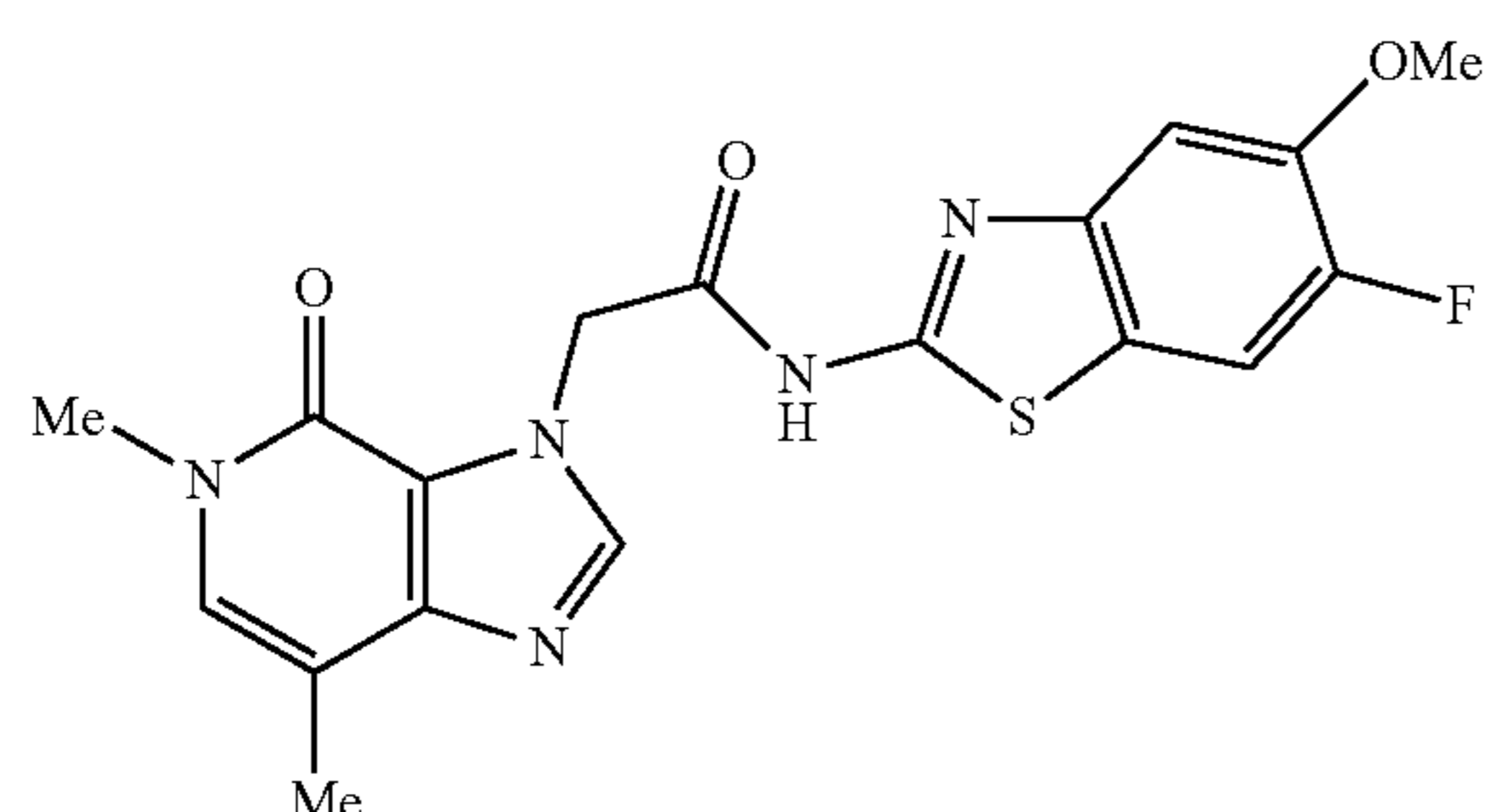
2-(5,7-dimethyl-4-oxo-4,5-dihydro-3H-imidazo[4,5-c]pyridin-3-yl)-N-(6-fluoro-5-methoxybenzo[d]thiazol-2-yl)acetamide
