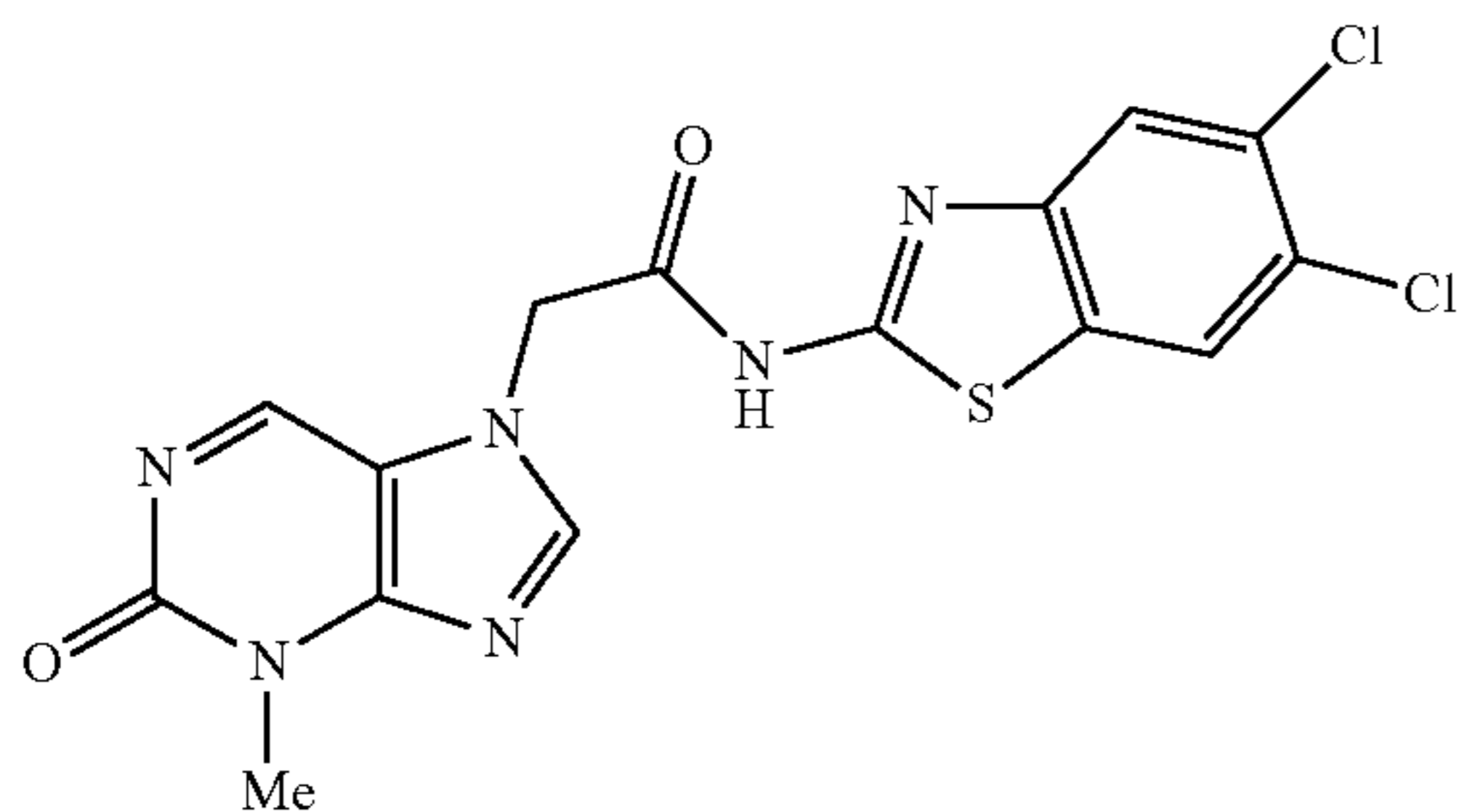
N-(5,6-dichlorobenzo[d]thiazol-2-yl)-2-(3-methyl-2-oxo-2,3-dihydropurin-7-yl)acetamide
