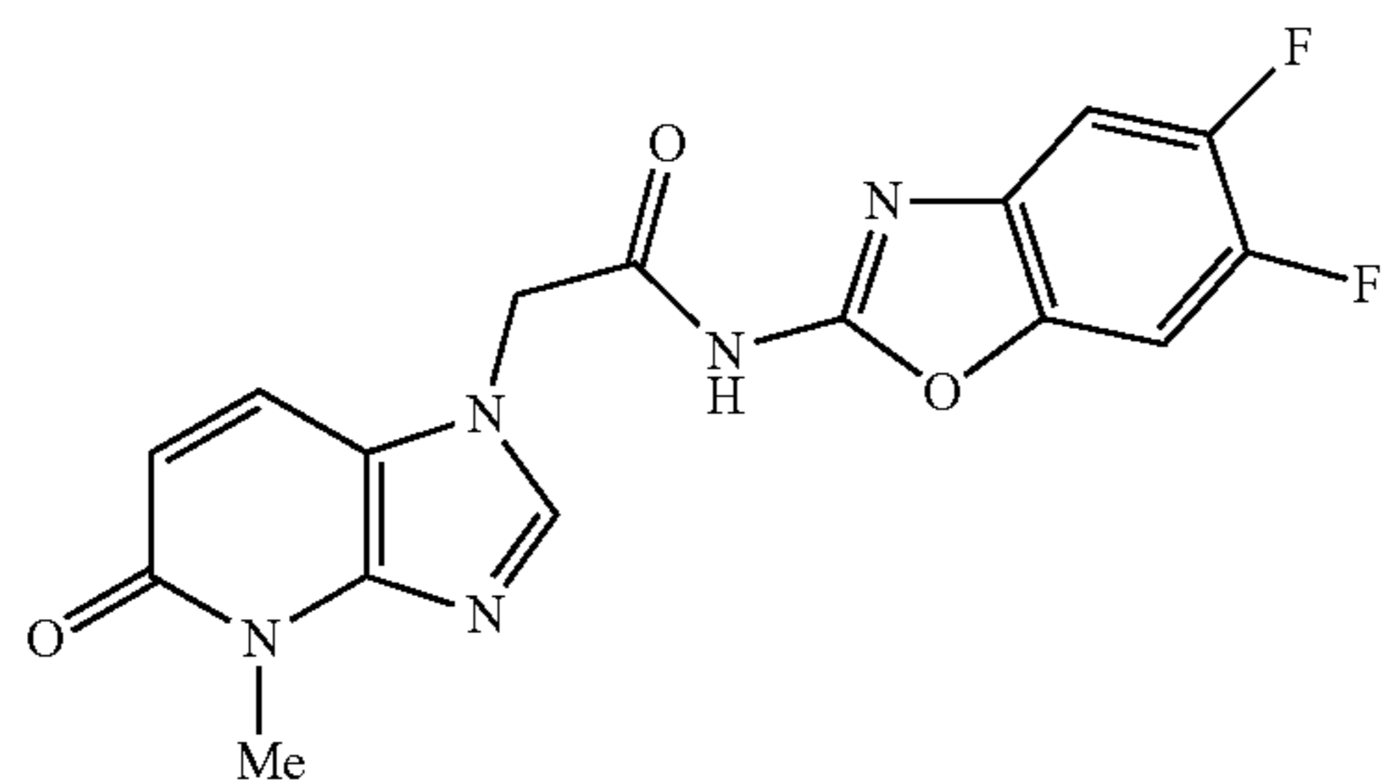
N-(5,6-difluorobenzo[d]oxazol-2-yl)-2-(4-methyl-5-oxo-4,5-dihydro-1H-imidazo[4,5-b]pyridin-1-yl)acetamide
