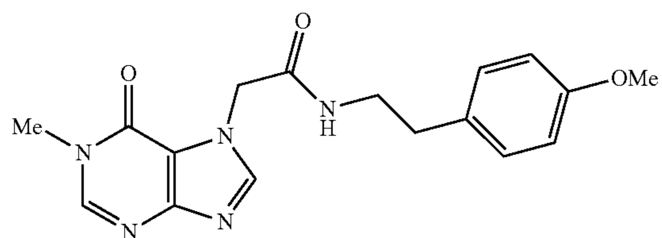
N-(4-methoxyphenethyl)-2-(1-methyl-6-oxo-1H-purin-7(6H)-yl)acetamide
