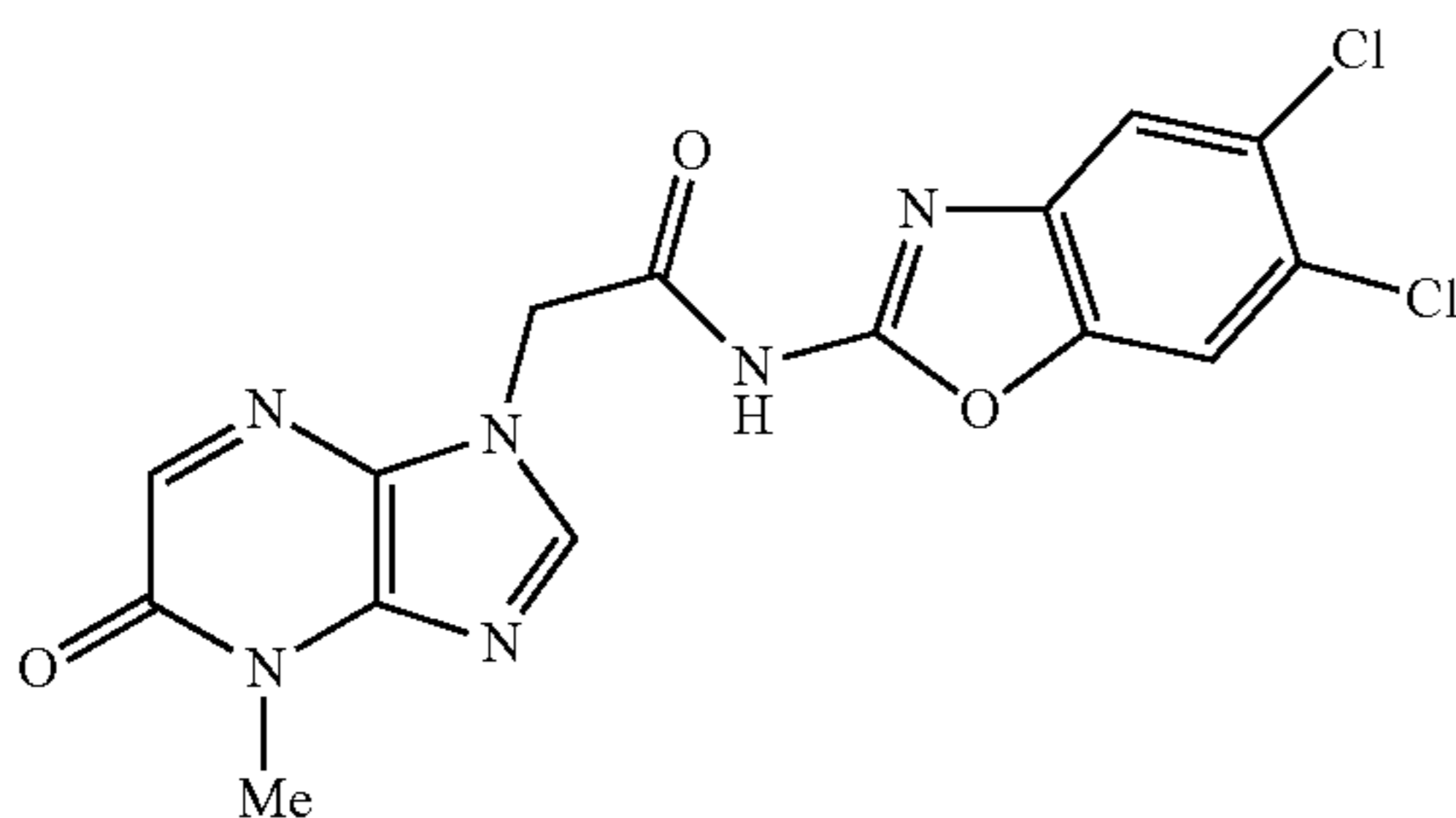
N-(5,6-dichlorobenzo[d]oxazol-2-yl)-2-(4-methyl-5-oxo-4,5-dihydro-1H-imidazo[4,5-b]pyridin-1-yl)acetamide
