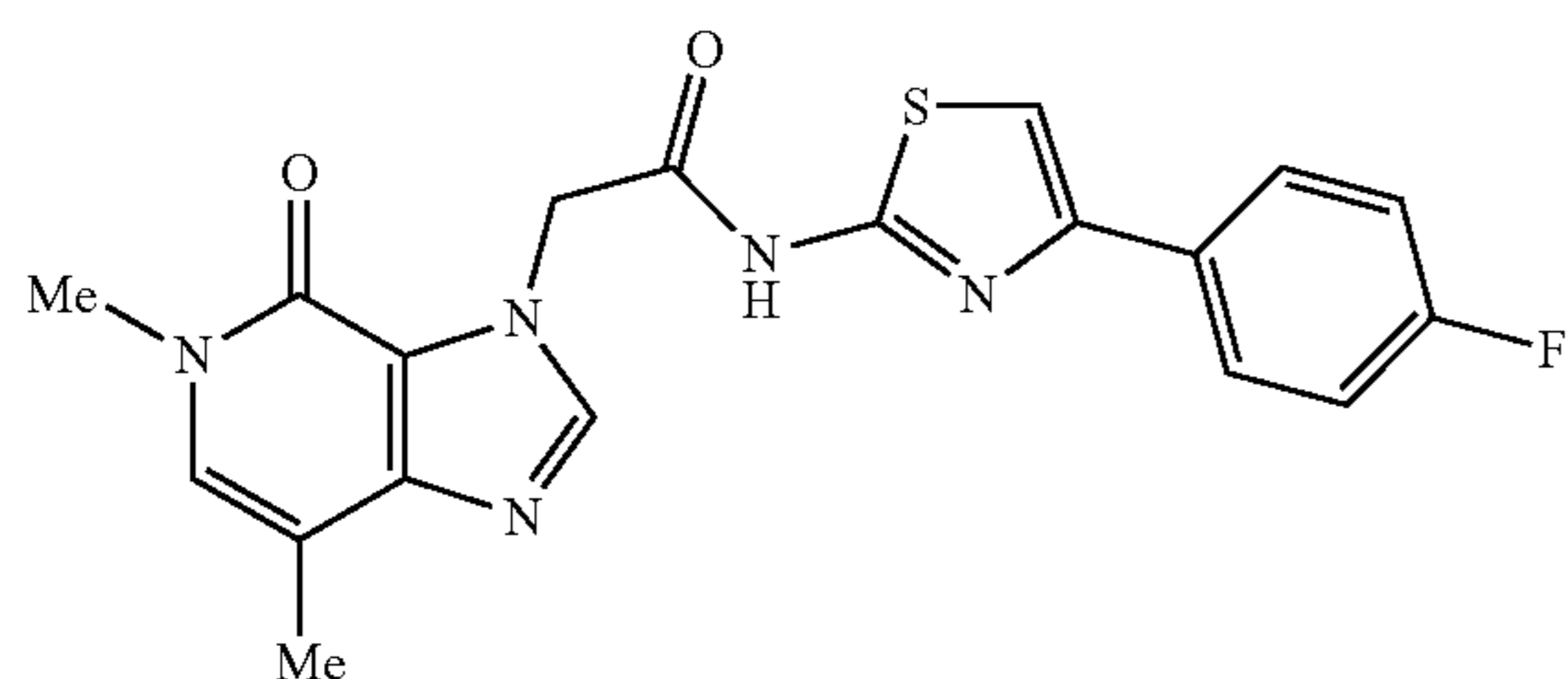
2-(5,7-dimethyl-4-oxo-4,5-dihydro-3H-imidazo[4,5-c]pyridin-3-yl)-N-(4-(4-fluorophenyl)thiazol-2-yl)acetamide
