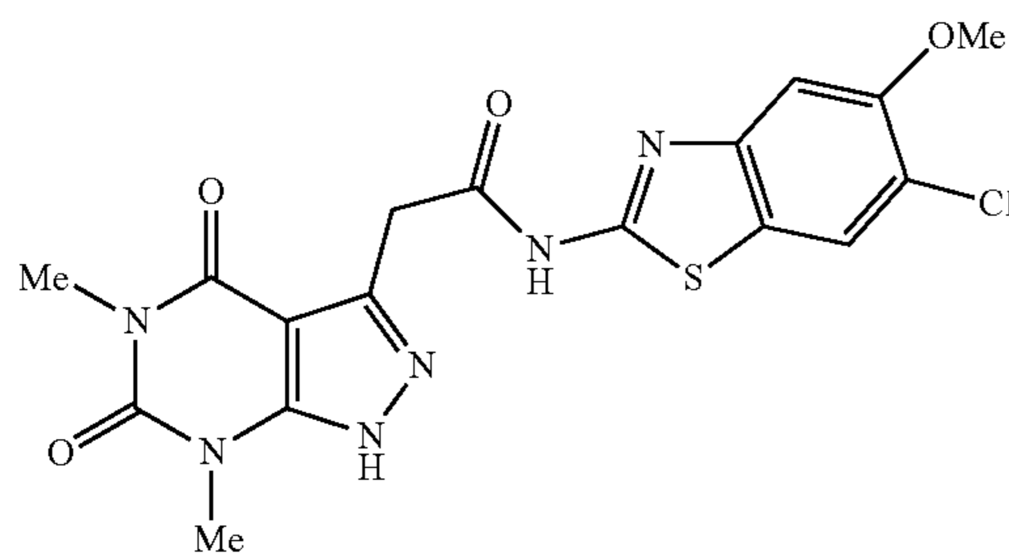
N-(6-chloro-5-methoxybenzo[d]thiazol-2-yl)-2-(5,7-dimethyl-4,6-dioxo-4,5,6,7-tetrahydro-1H-pyrazolo[3,4-d]pyrimidin-3-yl)acetamide
