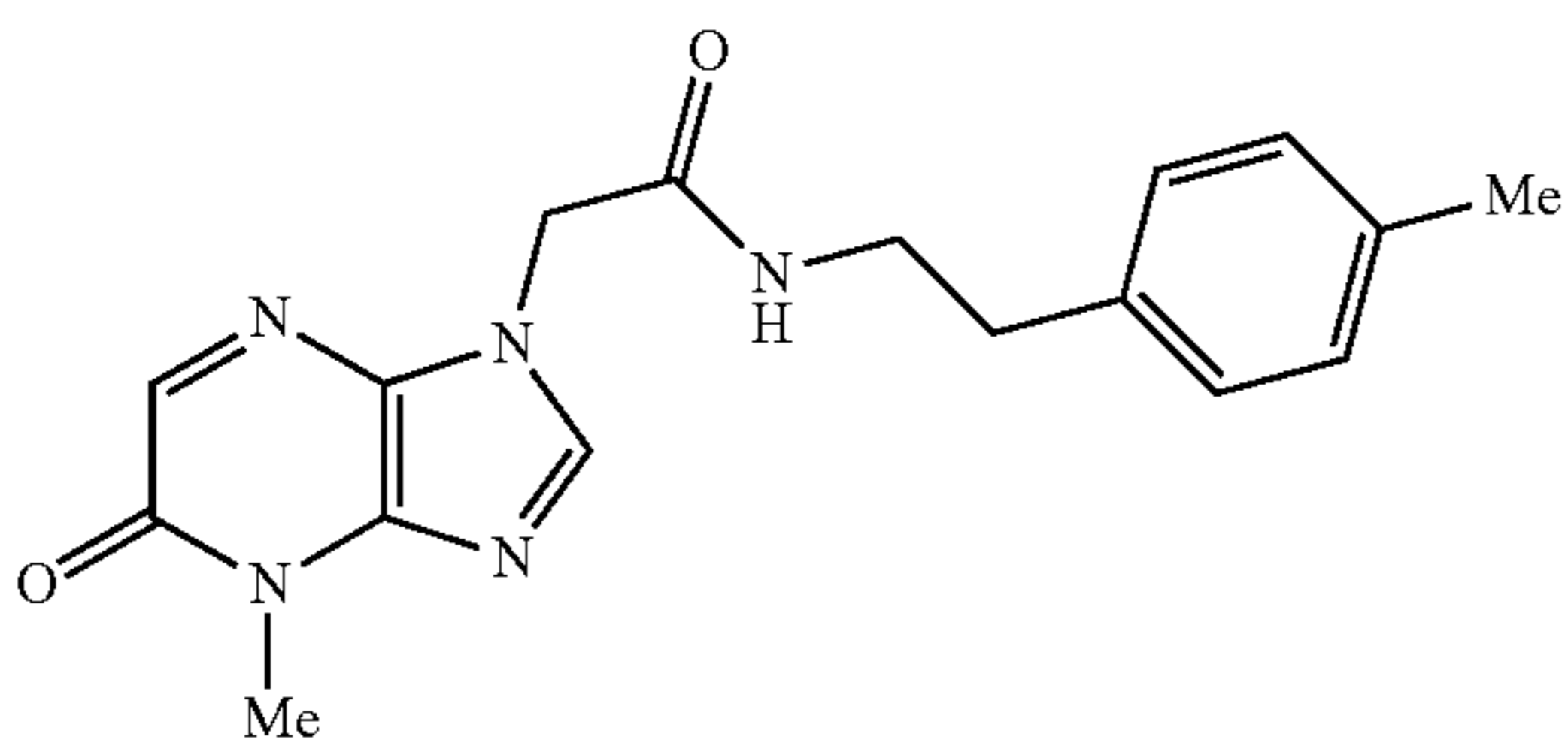
2-(4-methyl-5-oxo-4,5-dihydro-1H-imidazo[4,5-b]pyrazin-1-yl)-N-(4-methylphenethyl)acetamide
