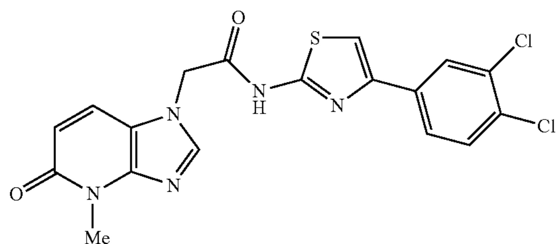
N-(4-(3,4-dichlorophenyl)thiazol-2-yl)-2-(4-methyl-5-oxo-4,5-dihydro-1H-imidazo[4,5-b]pyridin-1-yl)acetamide
