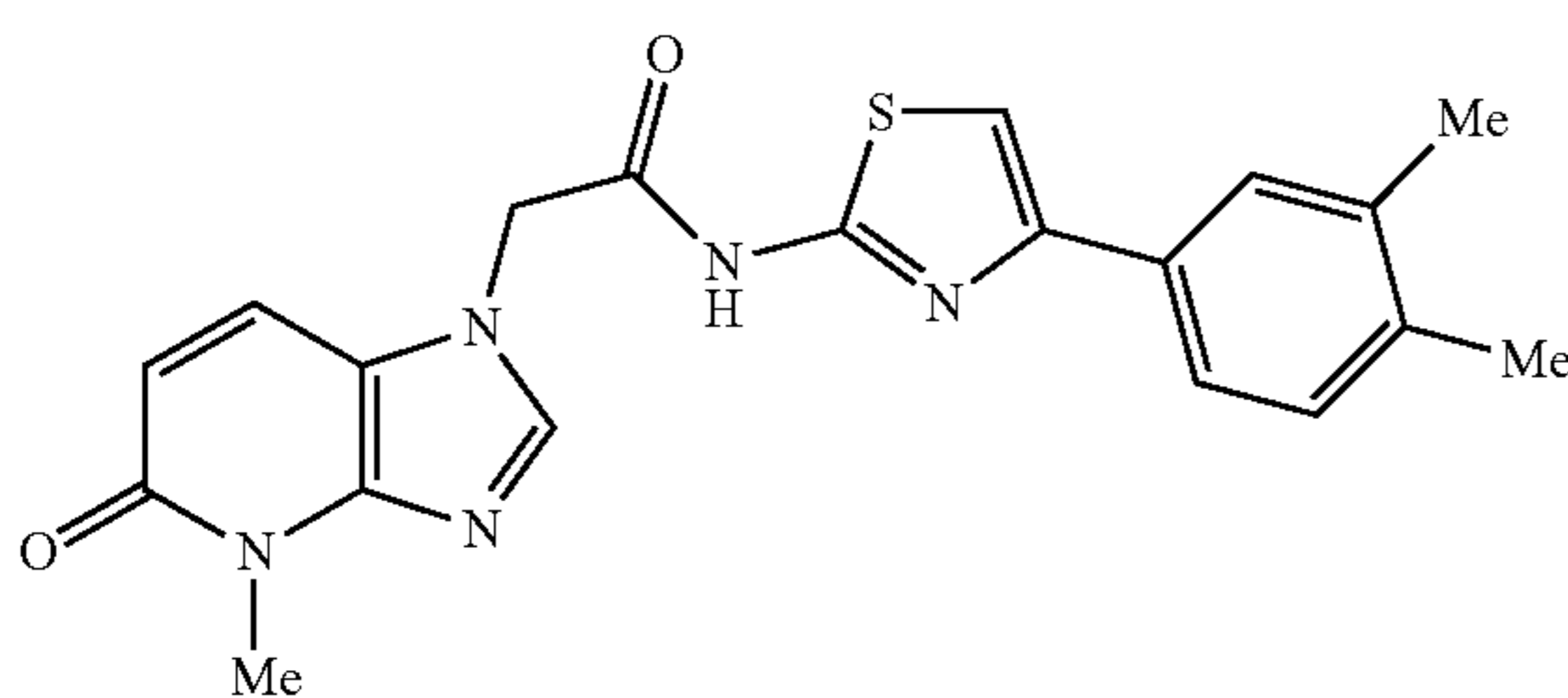
N-(4-(3,4-dimethylphenyl)thiazol-2-yl)-2-(4-methyl-5-oxo-4,5-dihydro-1H-imidazo[4,5-b]pyridin-1-yl)acetamide
