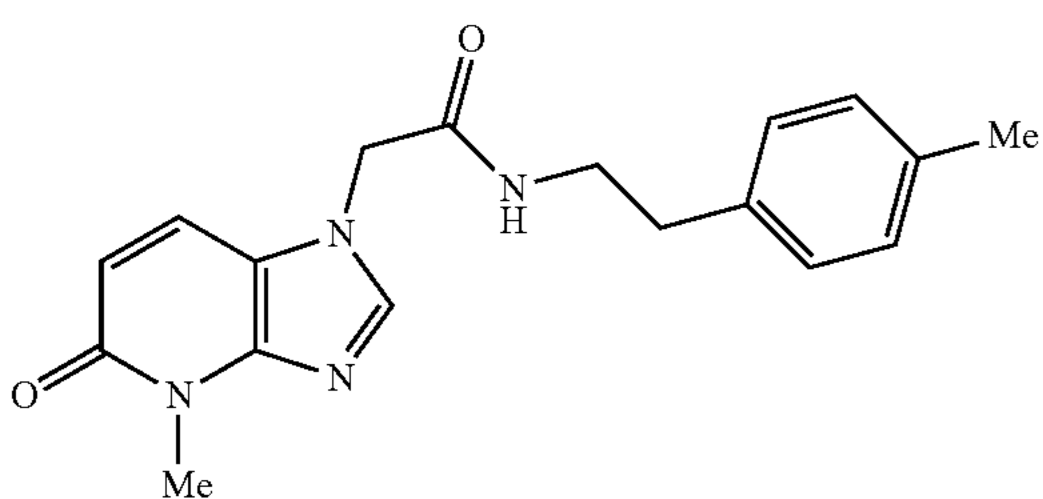
2-(4-methyl-5-oxo-4,5-dihydro-1H-imidazo[4,5-b]pyridin-1-yl)-N-(4-methylphenethyl)acetamide
