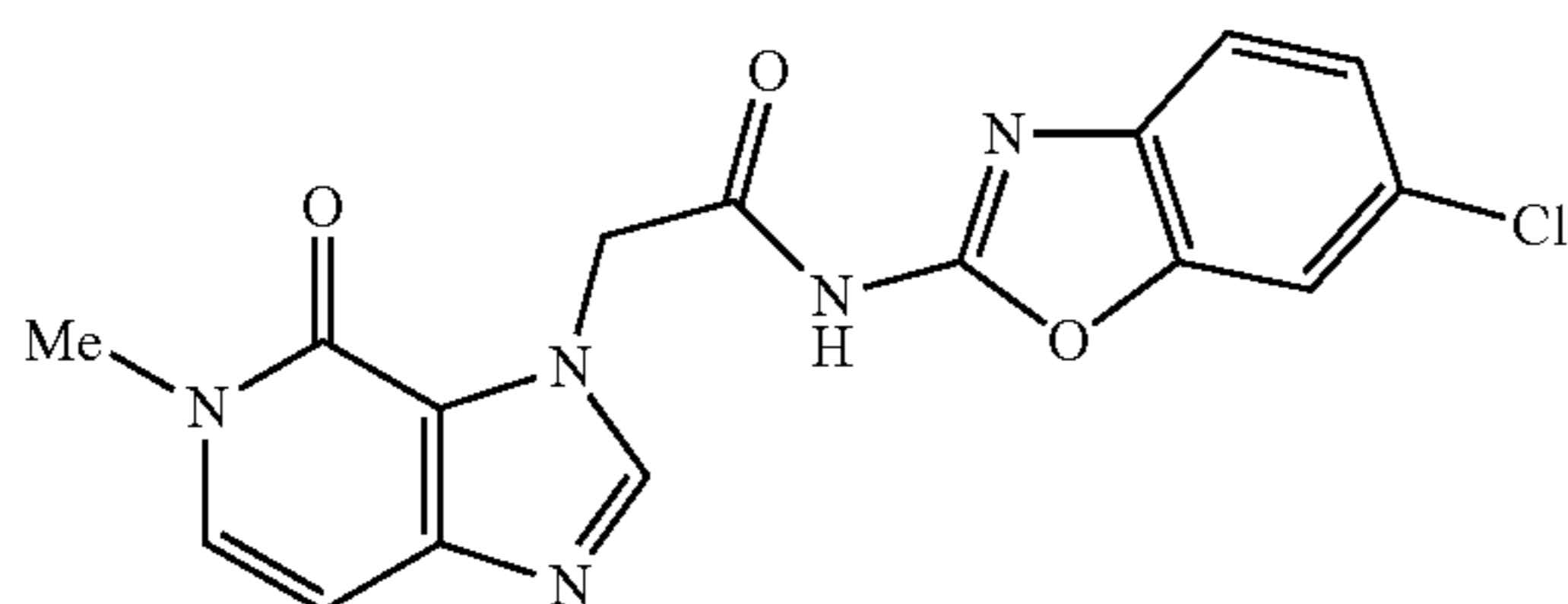
N-(6-chlorobenzo[d]oxazol-2-yl)-2-(5-methyl-4-oxo-4,5-dihydro-3H-imidazo[4,5-c]pyridin-3-yl)acetamide
