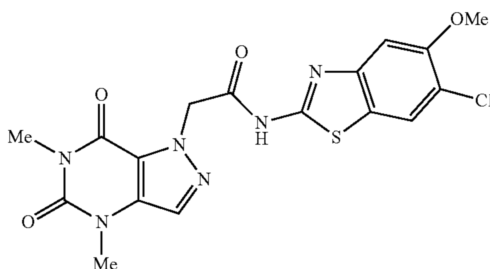
N-(6-chloro-5-methoxybenzo[d]thiazol-2-yl)-2-(4,6-dimethyl-5,7-dioxo-4,5,6,7-tetrahydro-1H-pyrazolo[4,3-d]pyrimidin-1-yl)acetamide
