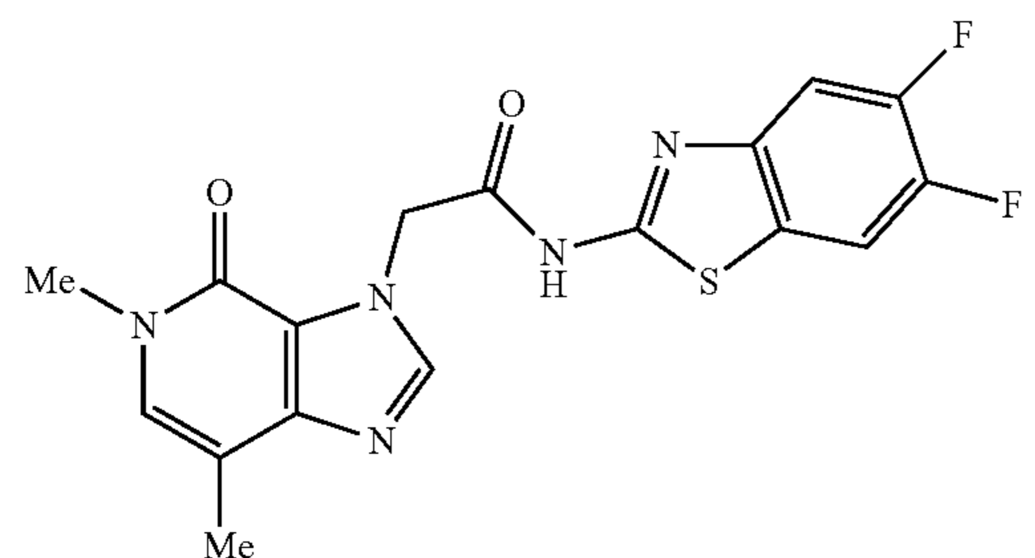
N-(5,6-difluorobenzo[d]thiazol-2-yl)-2-(5,7-dimethyl-4-oxo-4,5-dihydro-3H-imidazo[4,5-c]pyridin-3-yl)acetamide
