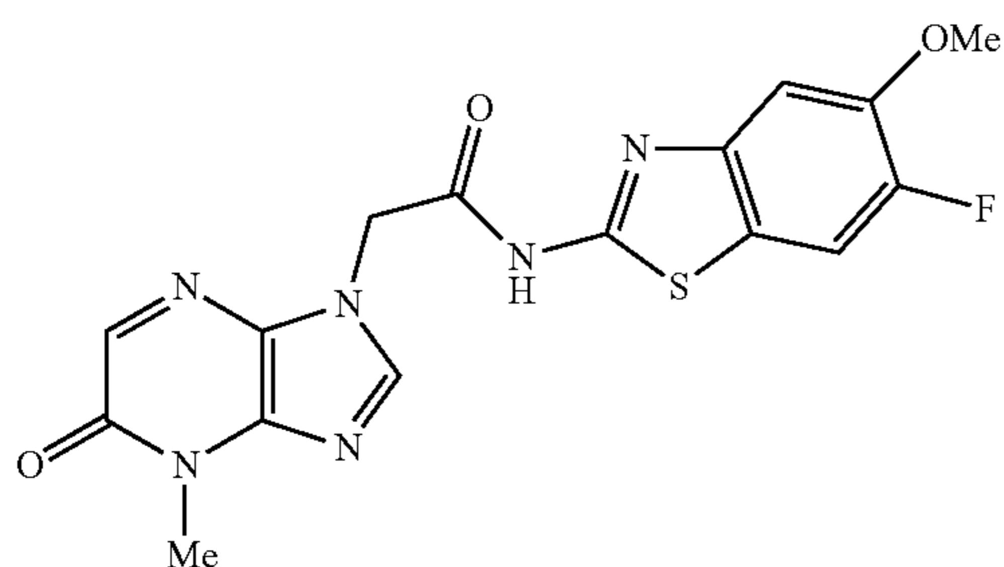
N-(6-fluoro-5-methoxybenzo[d]thiazol-2-yl)-2-(4-methyl-5-oxo-4,5-dihydro-1H-imidazo[4,5-b]pyridin-1-yl)acetamide
