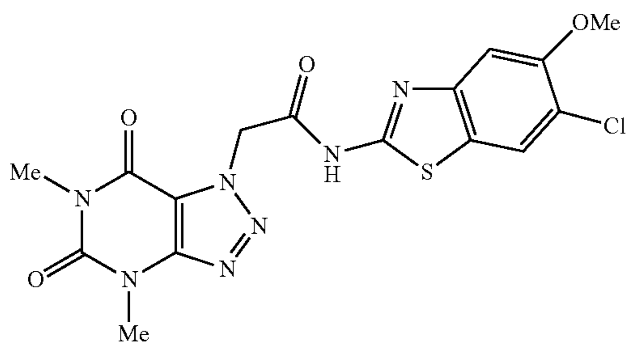
N-(6-chloro-5-methoxybenzo[d]thiazol-2-yl)-2-(4,6-dimethyl-5,7-dioxo-4,5,6,7-tetrahydro-1H-[1,2,3]triazolo[4,5-d]pyrimidin-1-yl)acetamide
