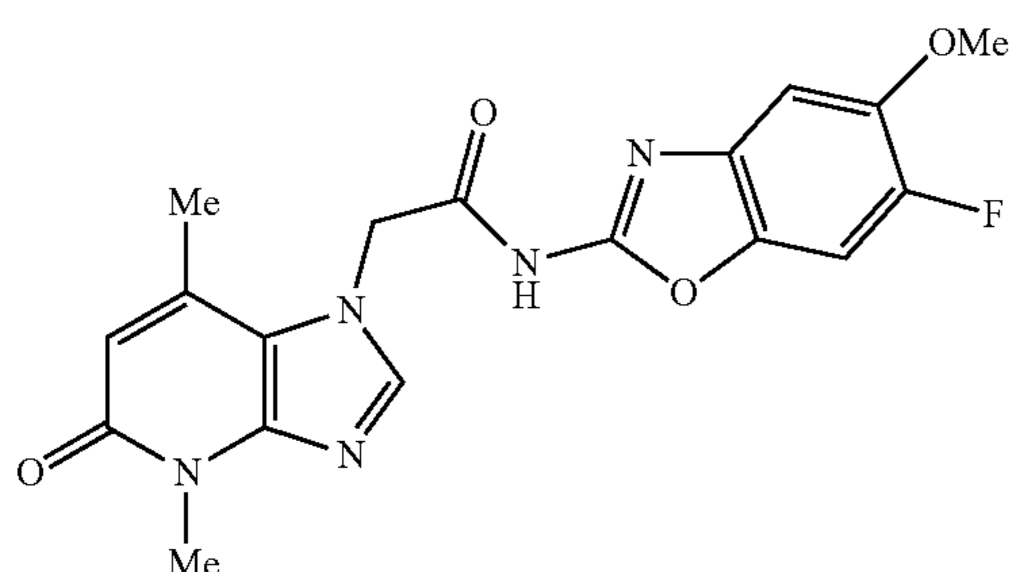
2-(4,7-dimethyl-5-oxo-4,5-dihydro-1H-imidazo[4,5-b]pyridin-1-yl)-N-(6-fluoro-5-methoxybenzo[d]oxazol-2-yl)acetamide
