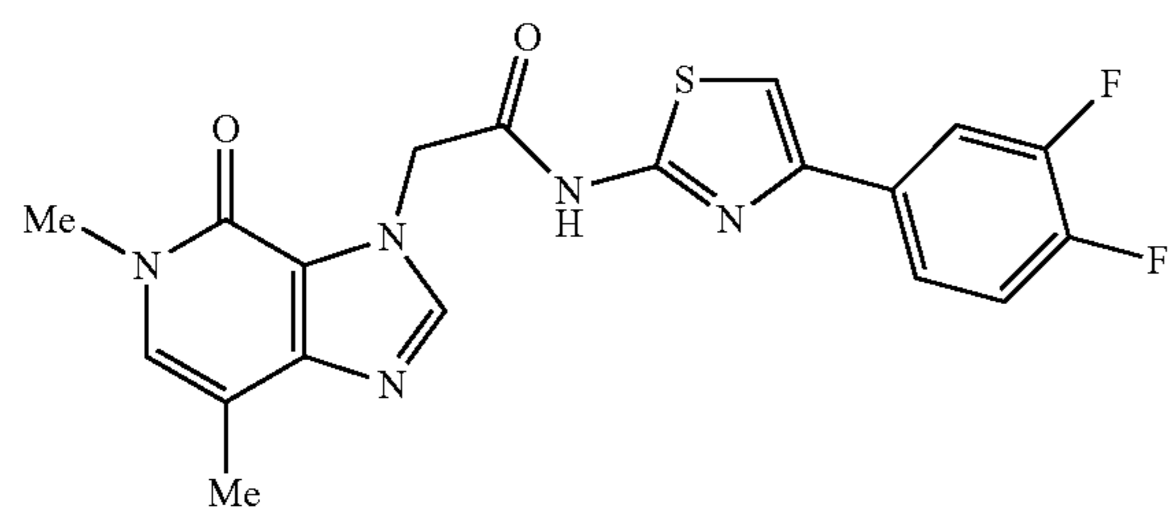
N-(4-(3,4-difluorophenyl)thiazol-2-yl)-2-(5,7-dimethyl-4-oxo-4,5-dihydro-3H-imidazo[4,5-c]pyridin-3-yl)acetamide
