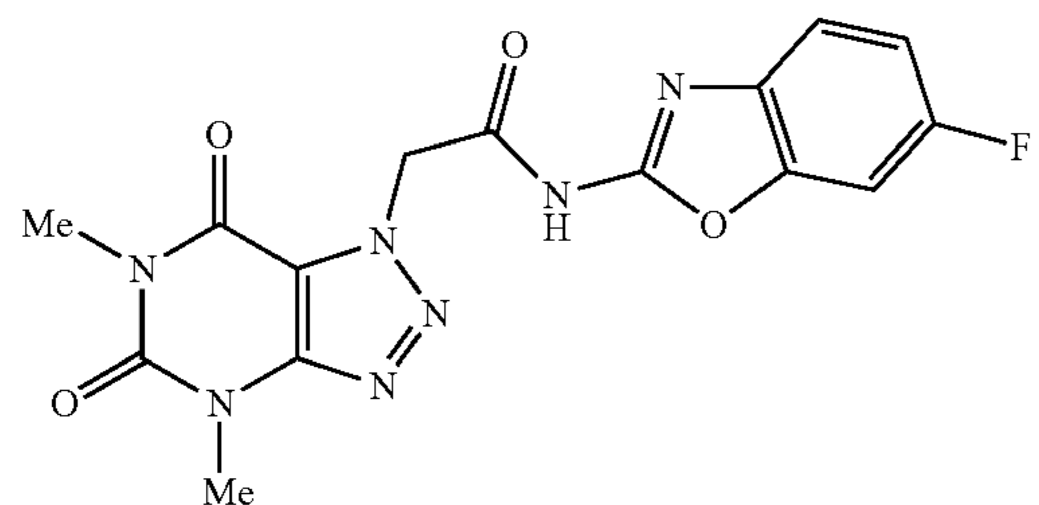
2-(4,6-dimethyl-5,7-dioxo-4,5,6,7-tetrahydro-1H-[1,2,3]triazolo[4,5-d]pyrimidin-1-yl)-N-(6-fluorobenzo[d]oxazol-2-yl)acetamide
