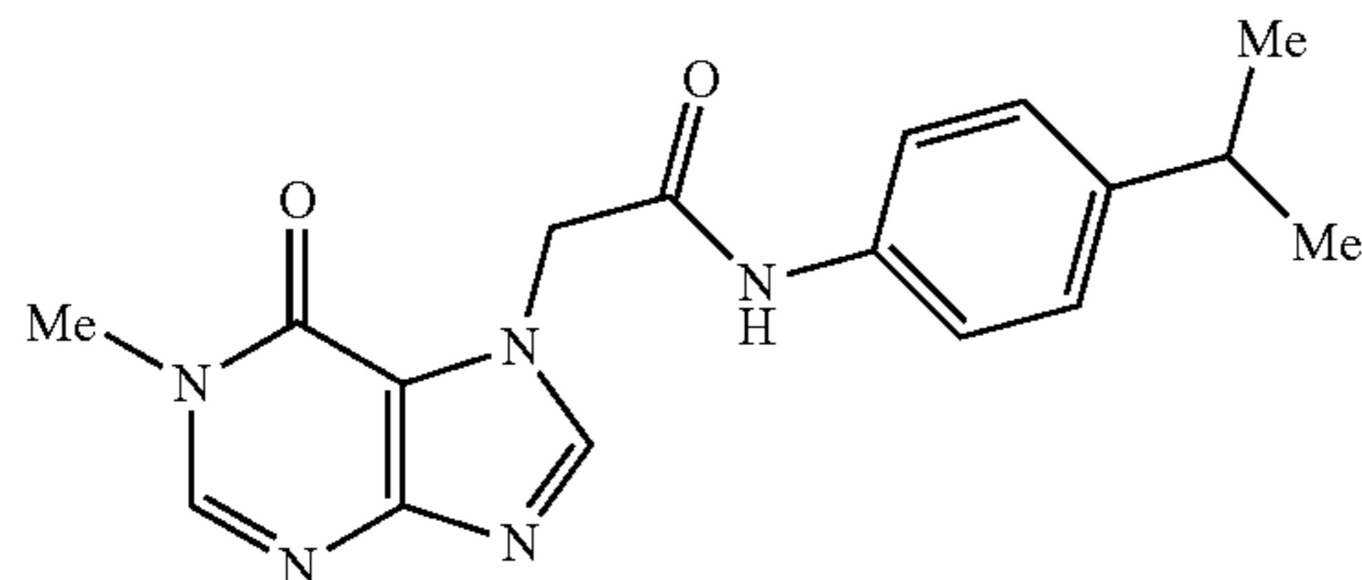
N-(4-isopropylphenyl)-2-(1-methyl-6-oxo-1H-purin-7(6H)-yl)acetamide
