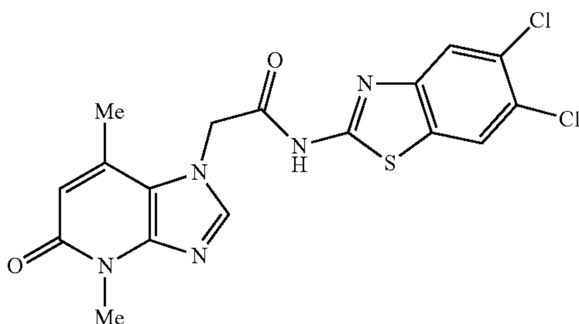
N-(5,6-dichlorobenzo[d]thiazol-2-yl)-2-(4,7-dimethyl-5-oxo-4,5-dihydro-1H-imidazo[4,5-b]pyridin-1-yl)acetamide
