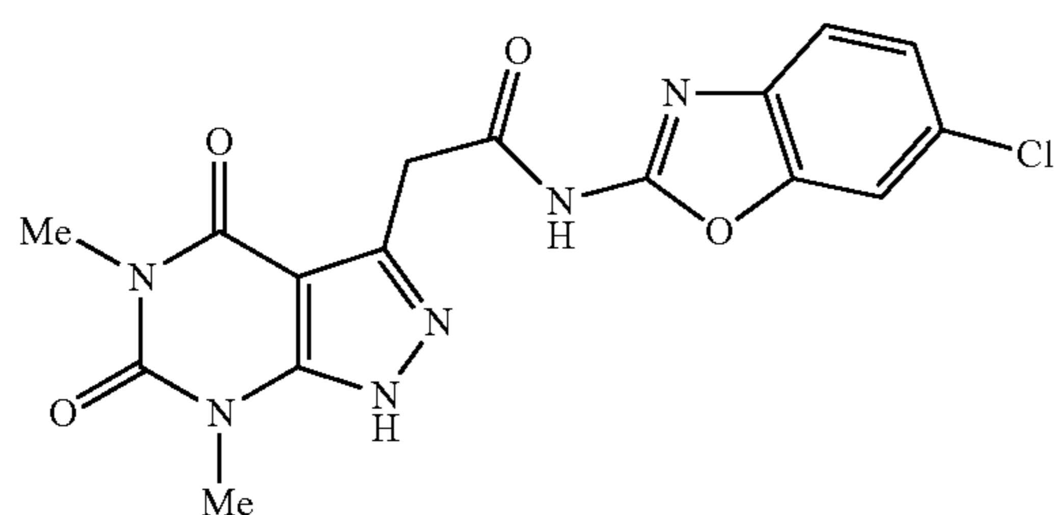
N-(6-chlorobenzo[d]oxazol-2-yl)-2-(5,7-dimethyl-4,6-dioxo-4,5,6,7-tetrahydro-1H-pyrazolo[3,4-d]pyrimidin-3-yl)acetamide
