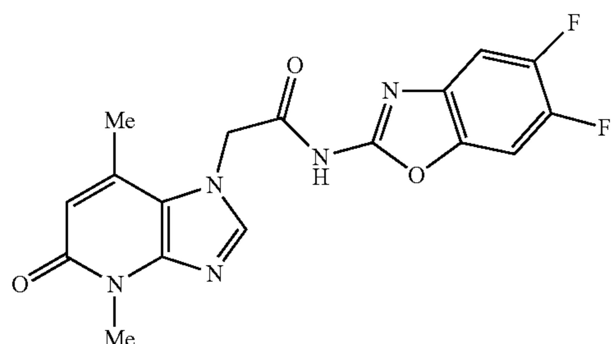
N-(5,6-difluorobenzo[d]oxazol-2-yl)-2-(4,7-dimethyl-5-oxo-4,5-dihydro-1H-imidazo[4,5-b]pyridin-1-yl)acetamide
