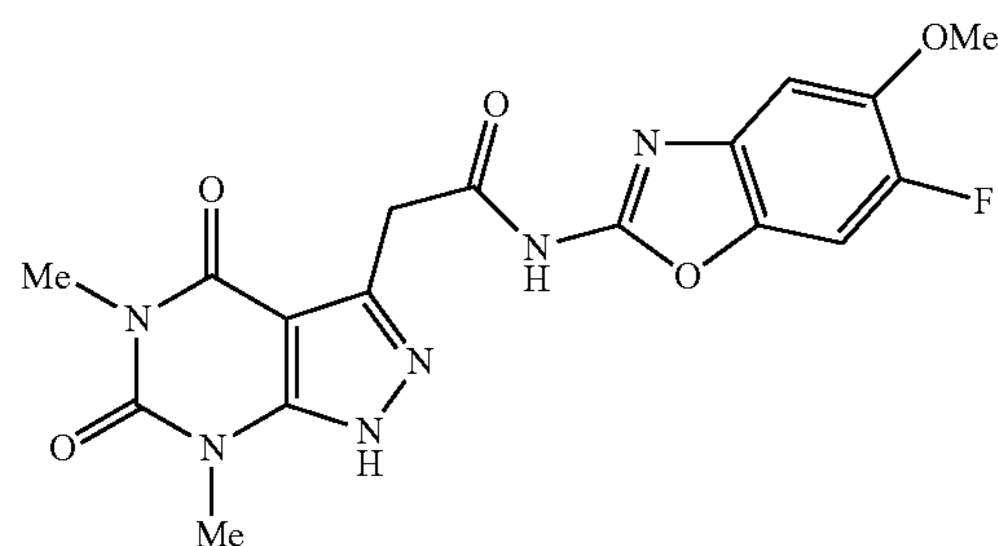
2-(5,7-dimethyl-4,6-dioxo-4,5,6,7-tetrahydro-1H-pyrazolo[3,4-d]pyrimidin-3-yl)-N-(6-fluoro-5-methoxybenzo[d]oxazol-2-yl)acetamide
