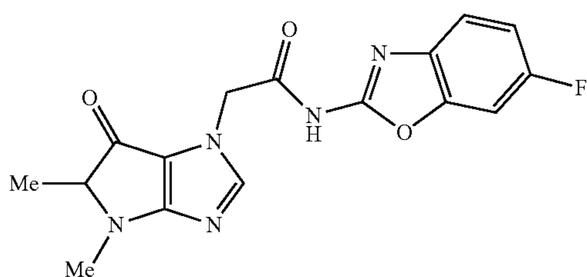
2-(4,5-dimethyl-6-oxo-5,6-dihydropyrrolo[3,2-d]imidazol-1(4H)-yl)-N-(6-fluorobenzo[d]oxazol-2-yl)acetamide
