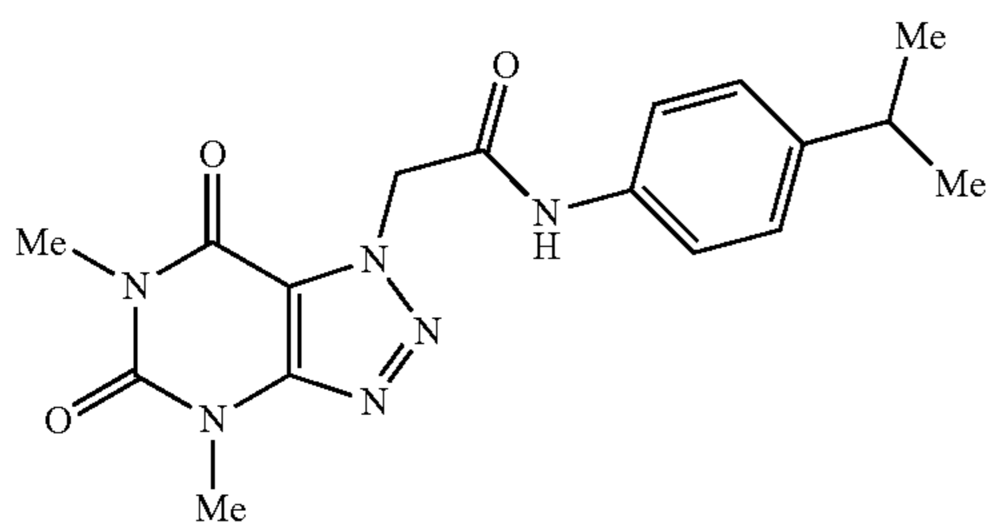
2-(4,6-dimethyl-5,7-dioxo-4,5,6,7-tetrahydro-1H-[1,2,3]triazolo[4,5-d]pyrimidin-1-yl)-N-(4-isopropylphenyl)acetamide
