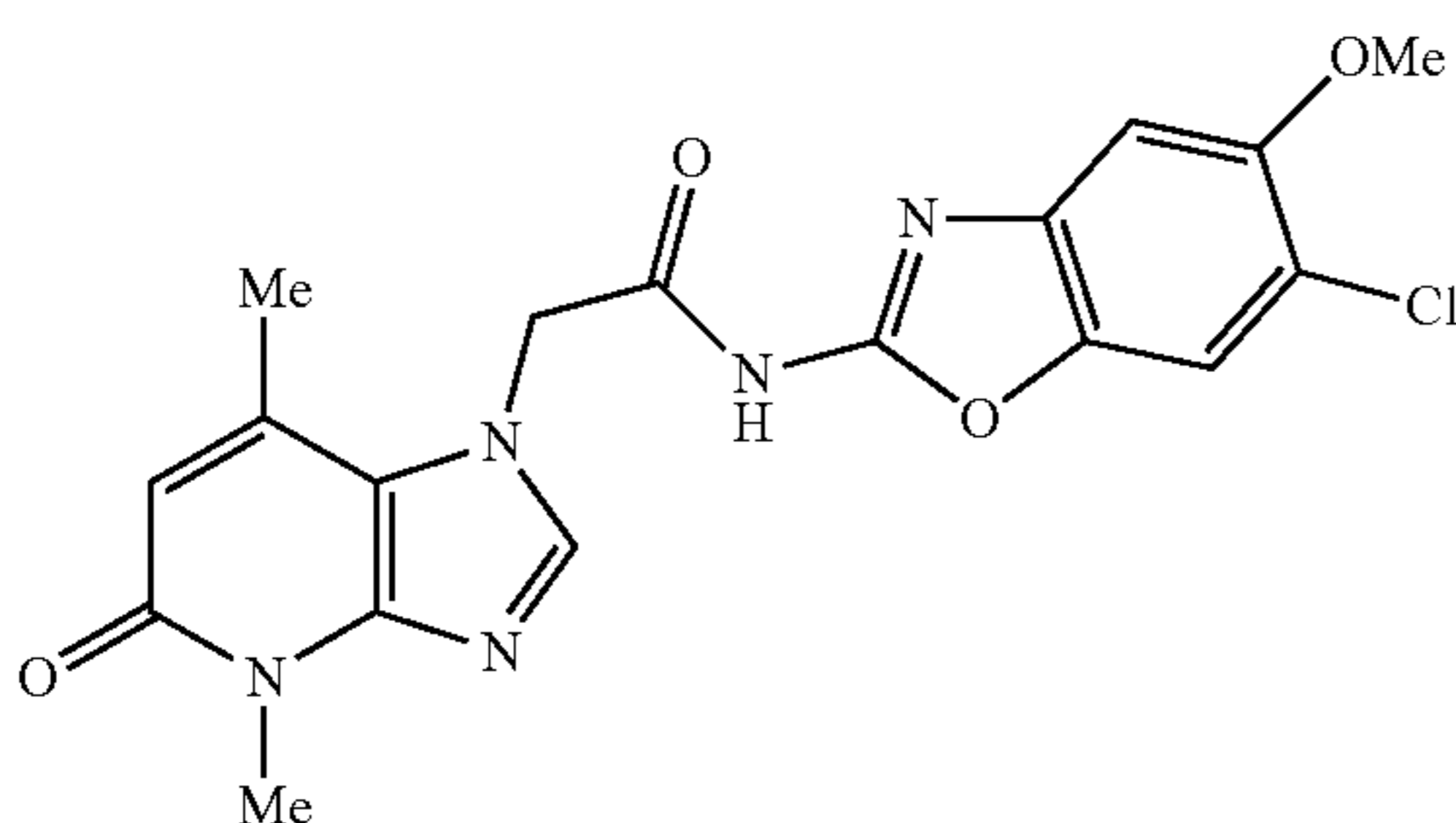
N-(6-chloro-5-methoxybenzo[d]oxazol-2-yl)-2-(4,7-dimethyl-5-oxo-4,5-dihydro-1H-imidazo[4,5-b]pyridin-1-yl)acetamide
