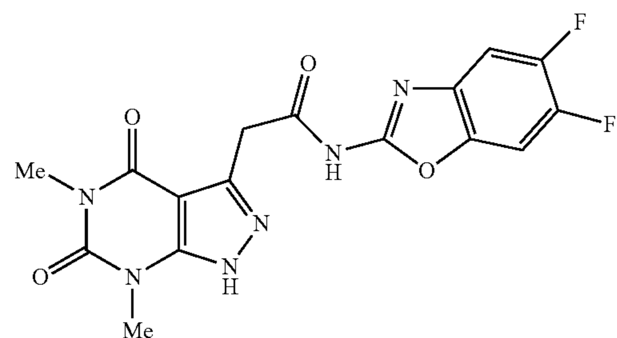
N-(5,6-difluorobenzo[d]oxazol-2-yl)-2-(5,7-dimethyl-4,6-dioxo-4,5,6,7-tetrahydro-1H-pyrazolo[3,4-d]pyrimidin-3-yl)acetamide
