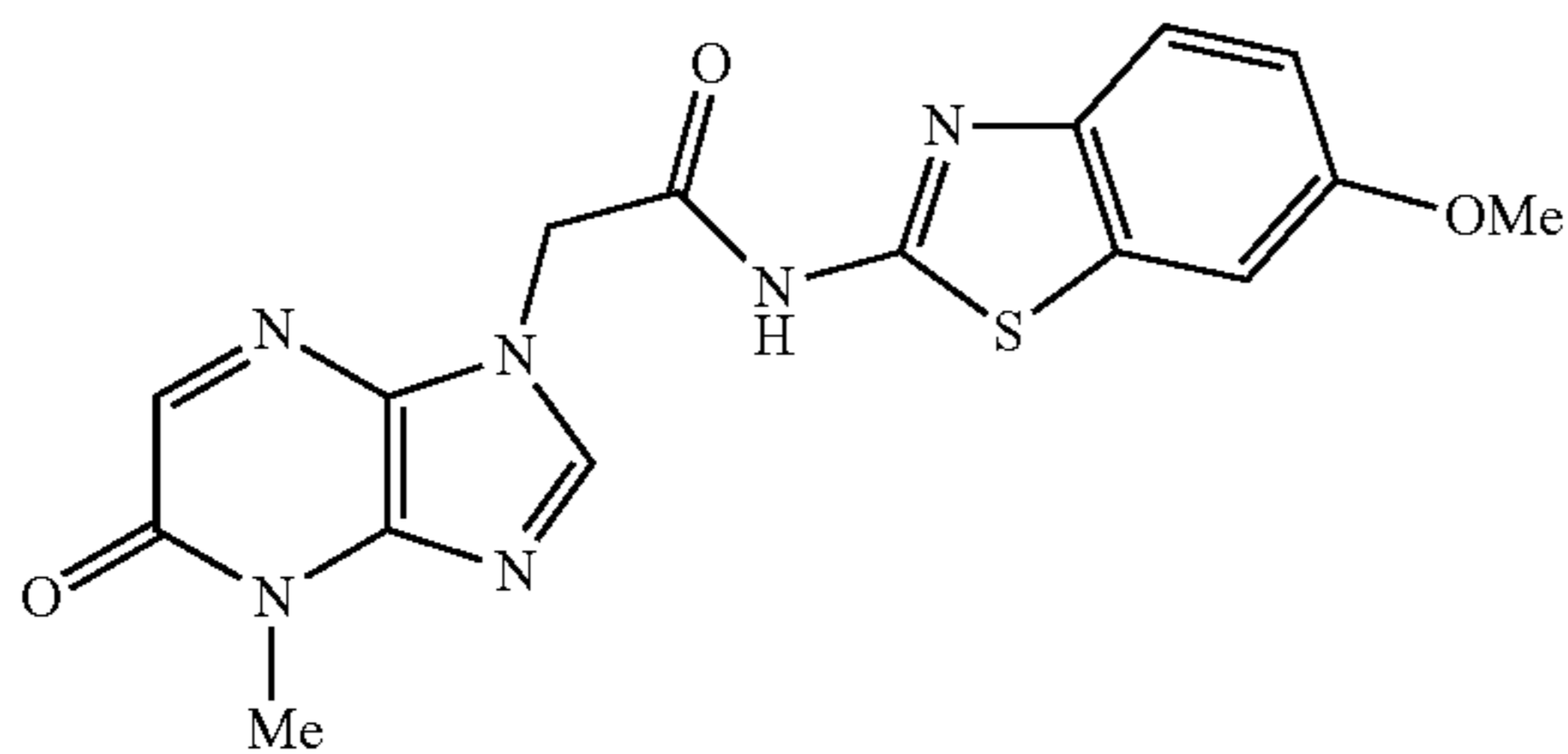
N-(6-methoxybenzo[d]thiazol-2-yl)-2-(4-methyl-5-oxo-4,5-dihydro-1H-imidazo[4,5-b]pyridin-1-yl)acetamide
