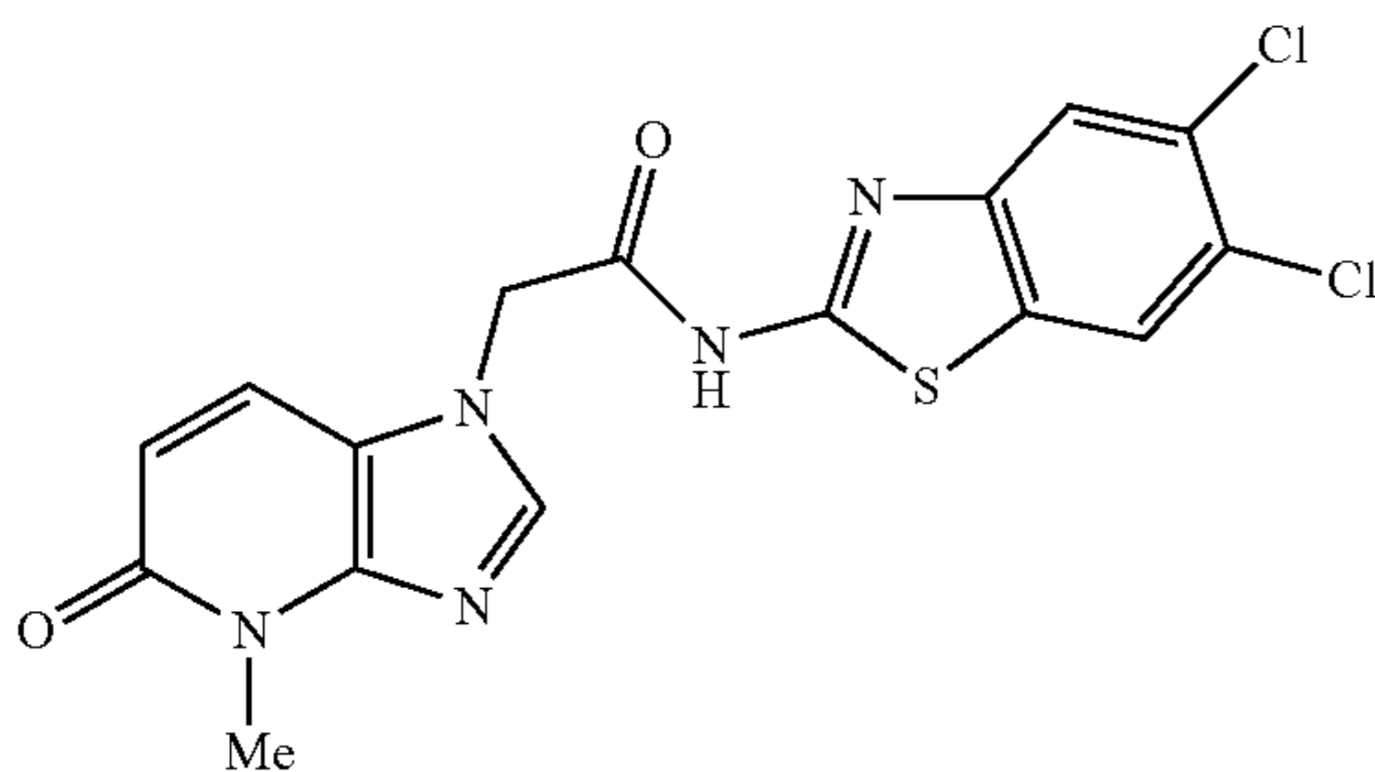
N-(5,6-dichlorobenzo[d]thiazol-2-yl)-2-(4-methyl-5-oxo-4,5-dihydro-1H-imidazo[4,5-b]pyridin-1-yl)acetamide
