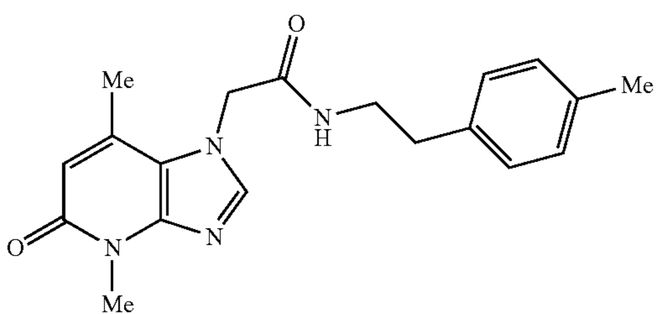
2-(4,7-dimethyl-5-oxo-4,5-dihydro-1H-imidazo[4,5-b]pyridin-1-yl)-N-(4-methylphenethyl)acetamide
