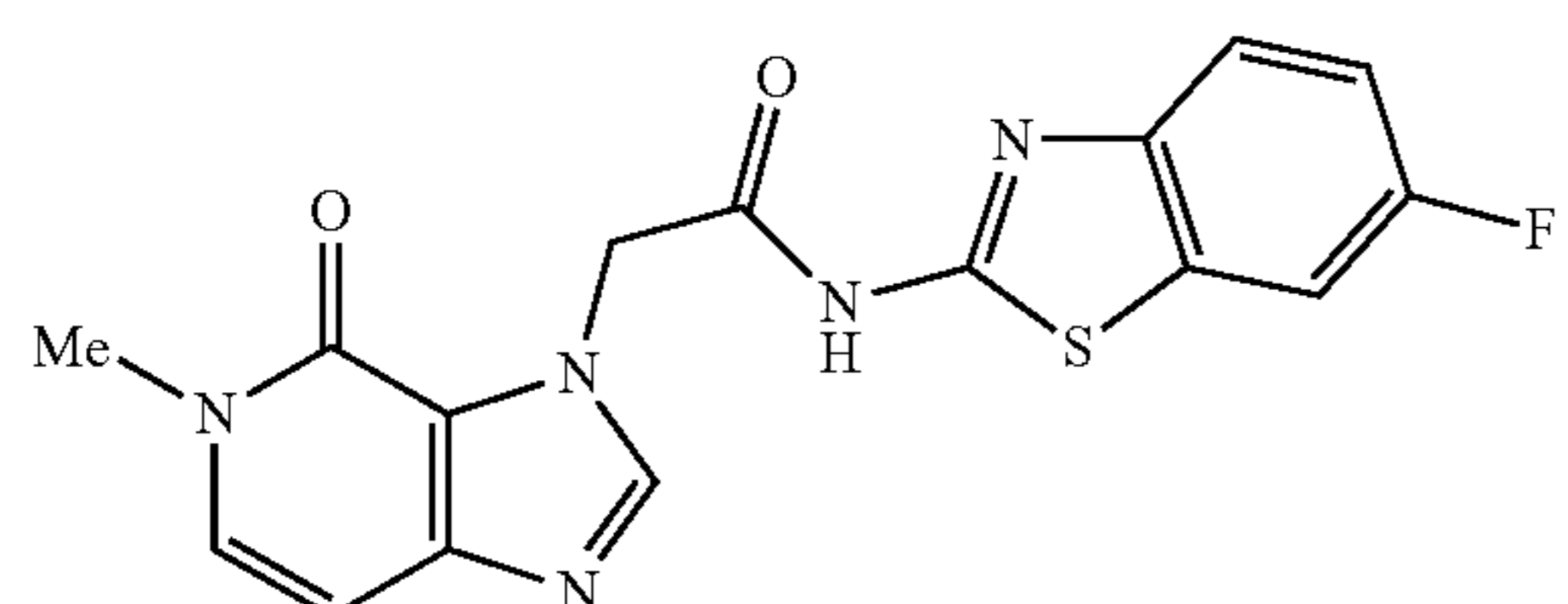
N-(6-fluorobenzo[d]thiazol-2-yl)-2-(5-methyl-4-oxo-4,5-dihydro-3H-imidazo[4,5-c]pyridin-3-yl)acetamide
