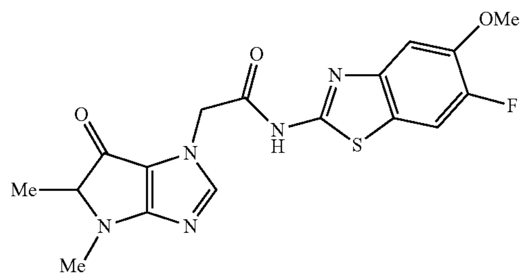
2-(4,5-dimethyl-6-oxo-5,6-dihydropyrrolo[3,2-d]imidazol-1(4H)-yl)-N-(6-fluoro-5-methoxybenzo[d]thiazol-2-yl)acetamide
