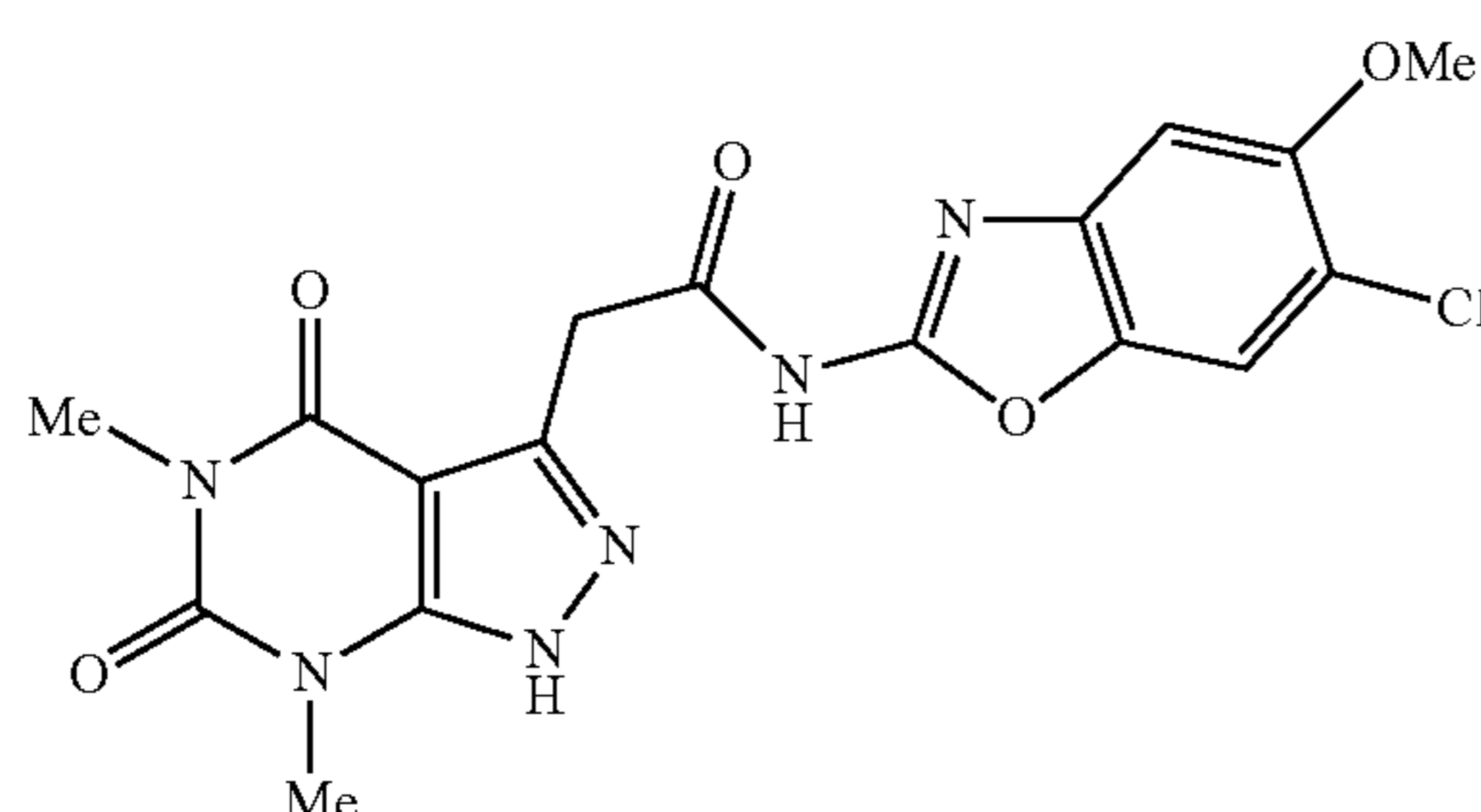
N-(6-chloro-5-methoxybenzo[d]oxazol-2-yl)-2-(5,7-dimethyl-4,6-dioxo-4,5,6,7-tetrahydro-1H-pyrazolo[3,4-d]pyrimidin-3-yl)acetamide
