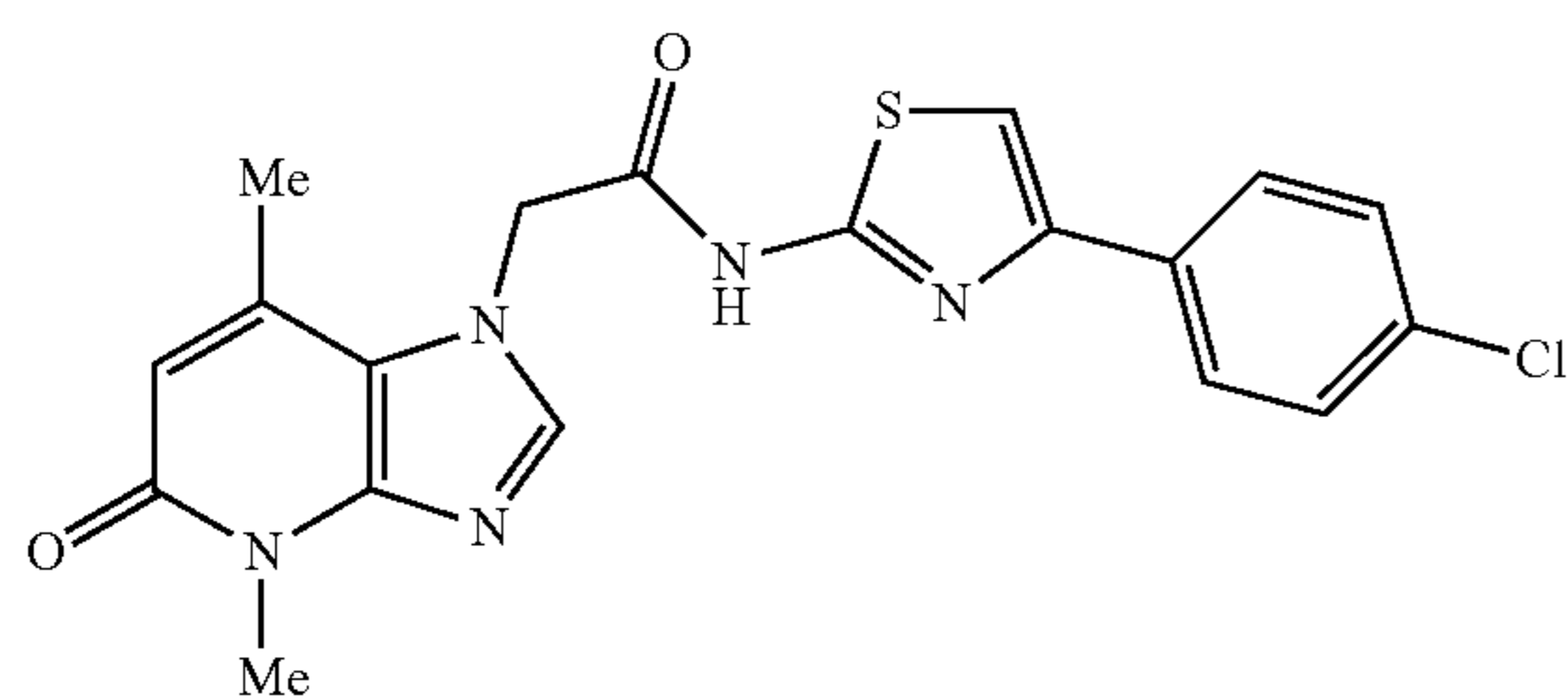
N-(4-(4-chlorophenyl)thiazol-2-yl)-2-(4,7-dimethyl-5-oxo-4,5-dihydro-1H-imidazo[4,5-b]pyridin-1-yl)acetamide
