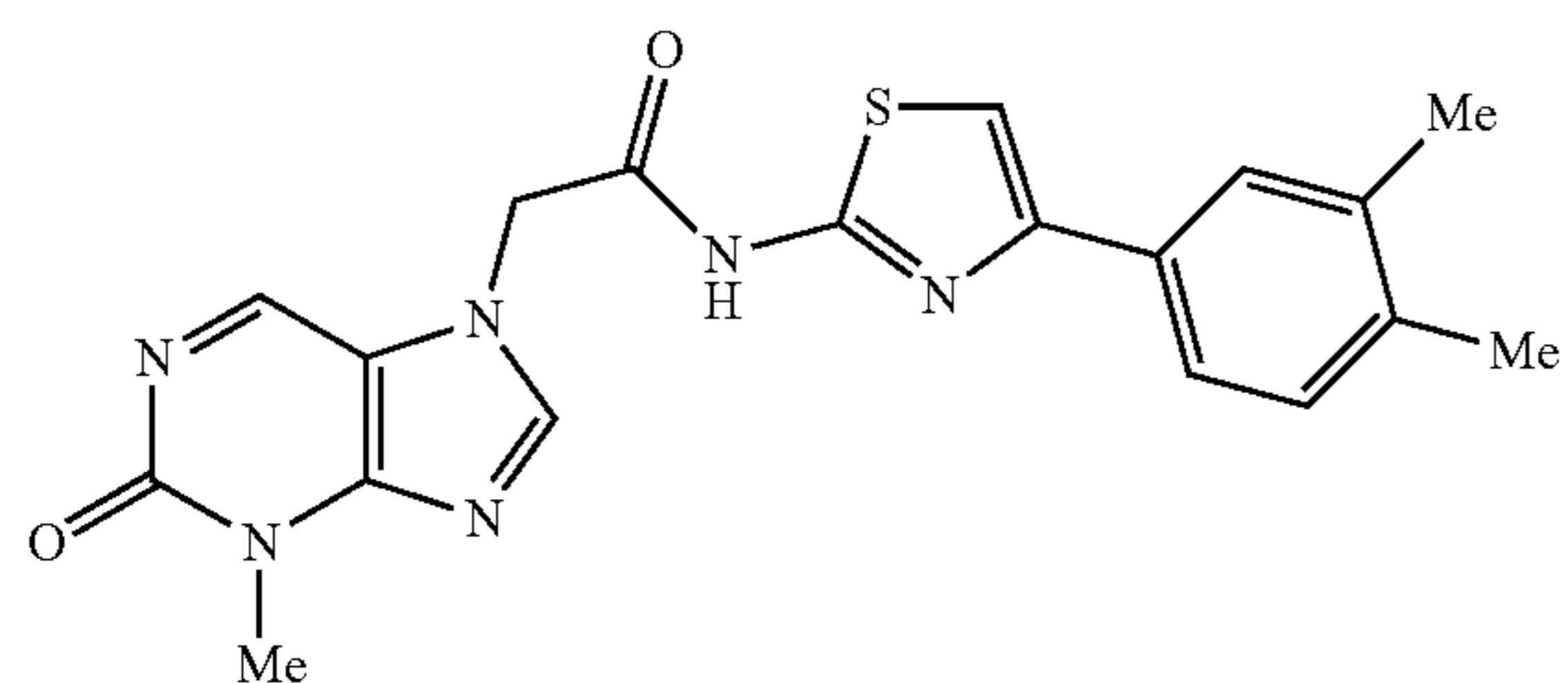
N-(4-(3,4-dimethylphenyl)thiazol-2-yl)-2-(3-methyl-2-oxo-2,3-dihydropurin-7-yl)acetamide
