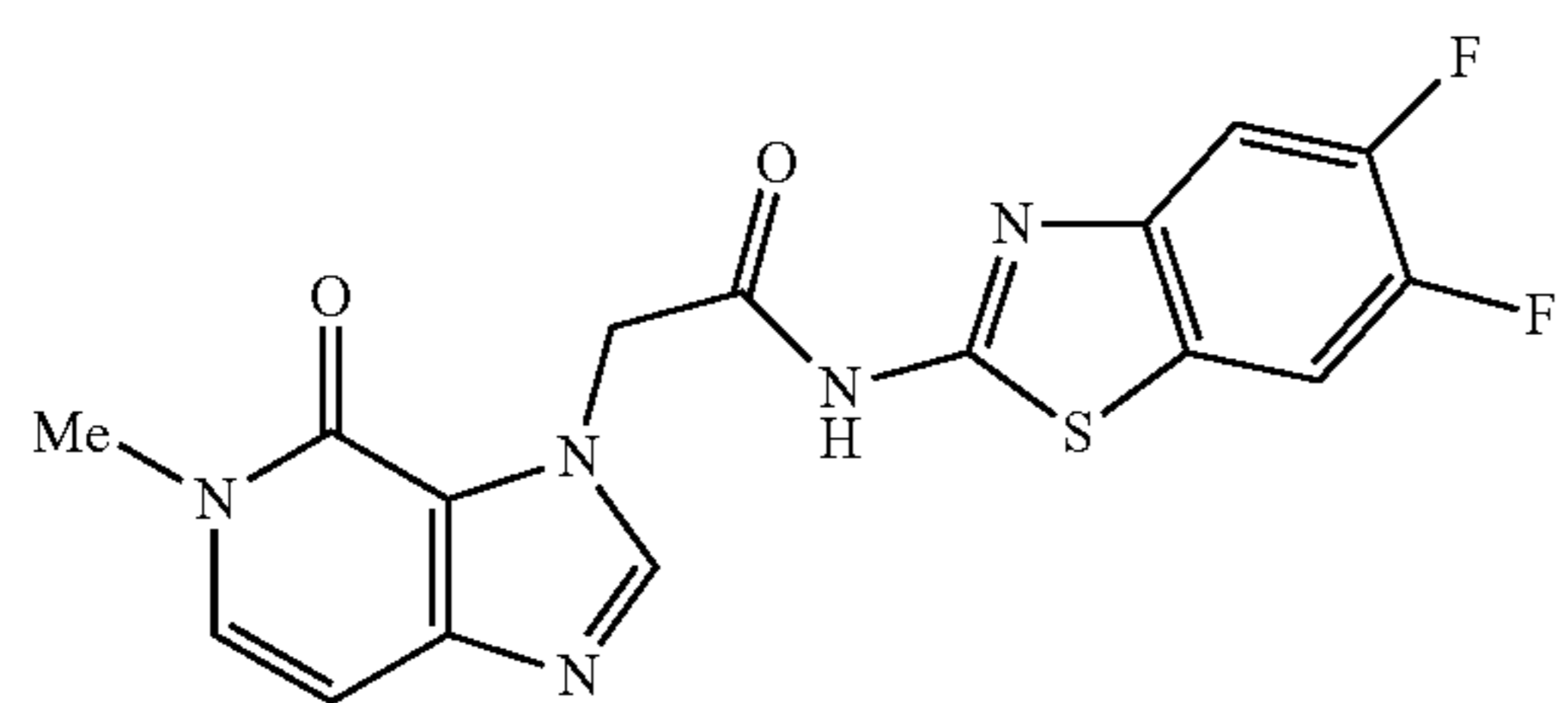
N-(5,6-difluorobenzo[d]thiazol-2-yl)-2-(5-methyl-4-oxo-4,5-dihydro-3H-imidazo[4,5-c]pyridin-3-yl)acetamide
