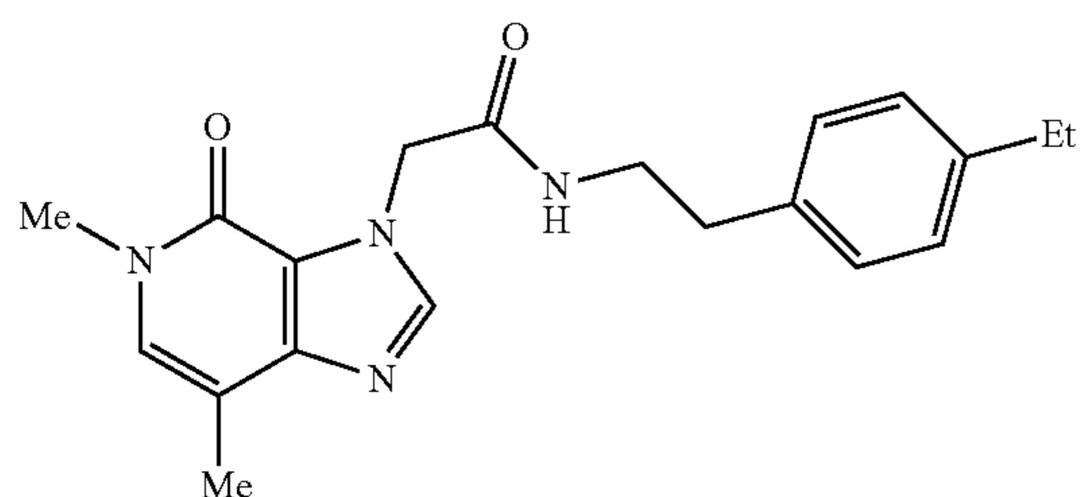
2-(5,7-dimethyl-4-oxo-4,5-dihydro-3H-imidazo[4,5-c]pyridin-3-yl)-N-(4-ethylphenethyl)acetamide
