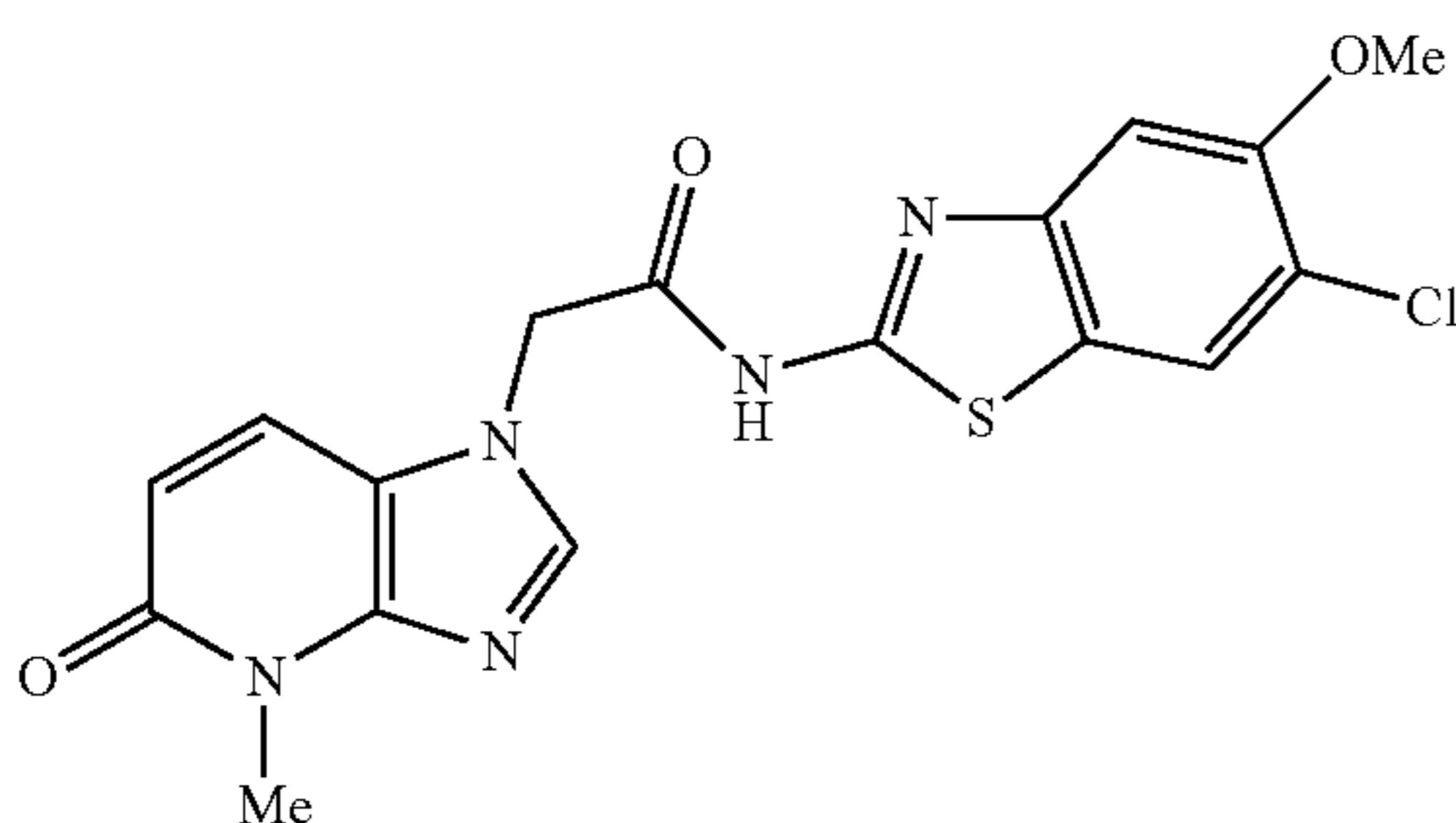
N-(6-chloro-5-methoxybenzo[d]thiazol-2-yl)-2-(4-methyl-5-oxo-4,5-dihydro-1H-imidazo[4,5-b]pyridin-1-yl)acetamide
