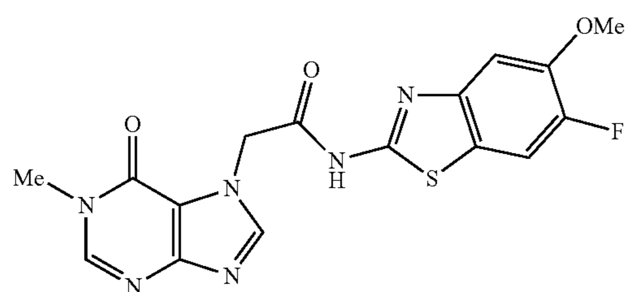
N-(6-fluoro-5-methoxybenzo[d]thiazol-2-yl)-2-(1-methyl-6-oxo-1H-purin-7(6H)-yl)acetamide
