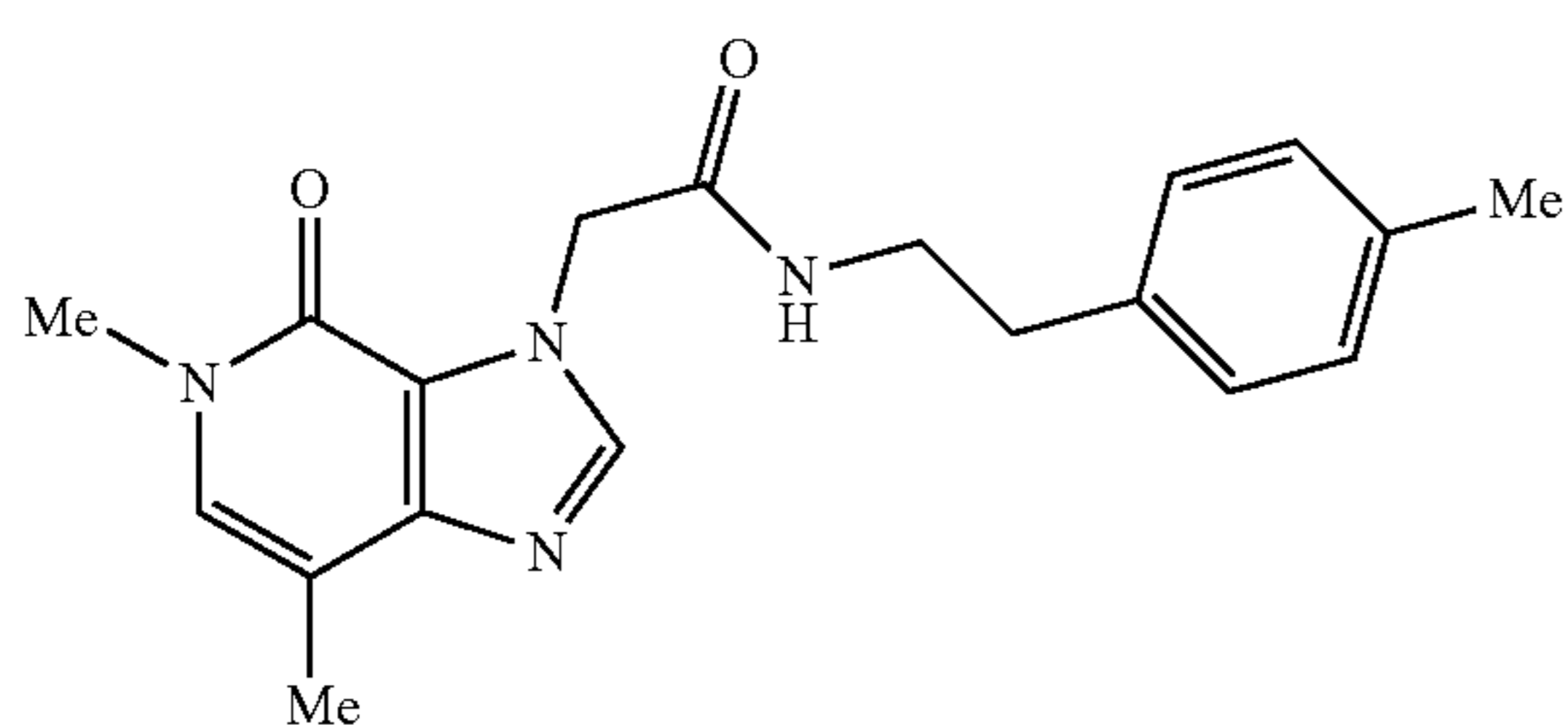
2-(5,7-dimethyl-4-oxo-4,5-dihydro-3H-imidazo[4,5-c]pyridin-3-yl)-N-(4-methylphenethyl)acetamide
