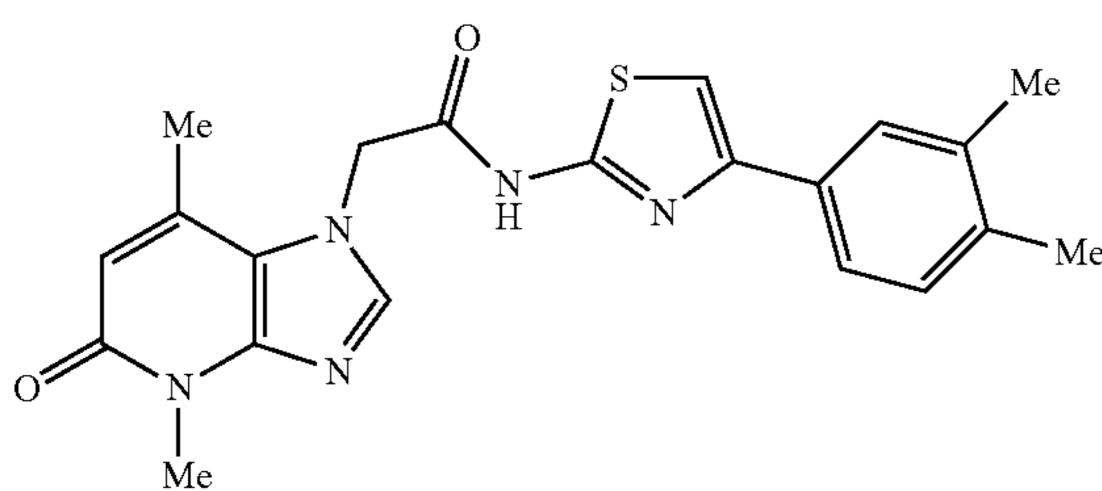
2-(4,7-dimethyl-5-oxo-4,5-dihydro-1H-imidazo[4,5-b]pyridin-1-yl)-N-(4-(3,4-dimethylphenyl)thiazol-2-yl)acetamide
