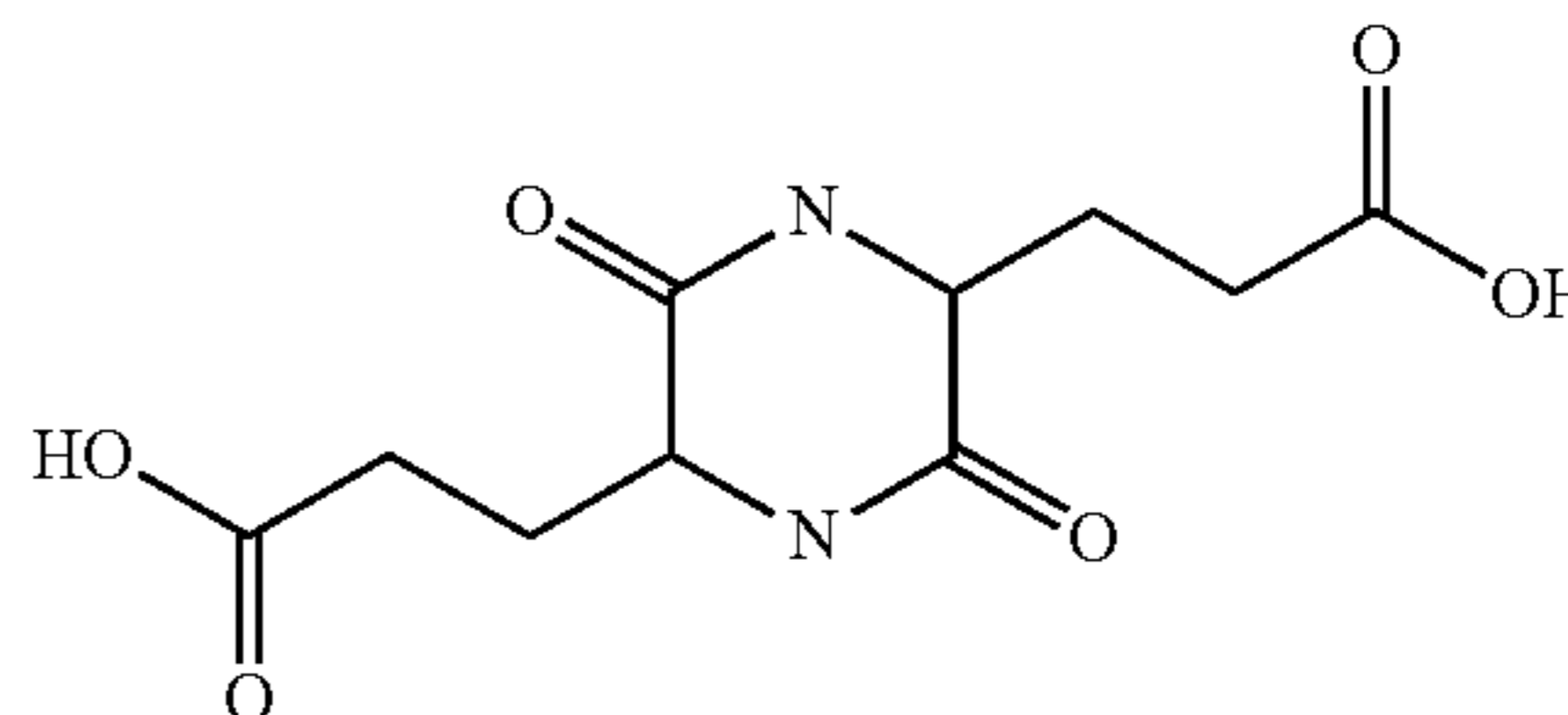
3-[5-(2-carboxy-ethyl)-3,6-dioxo-piperazin-2-yl]-propionic acid
