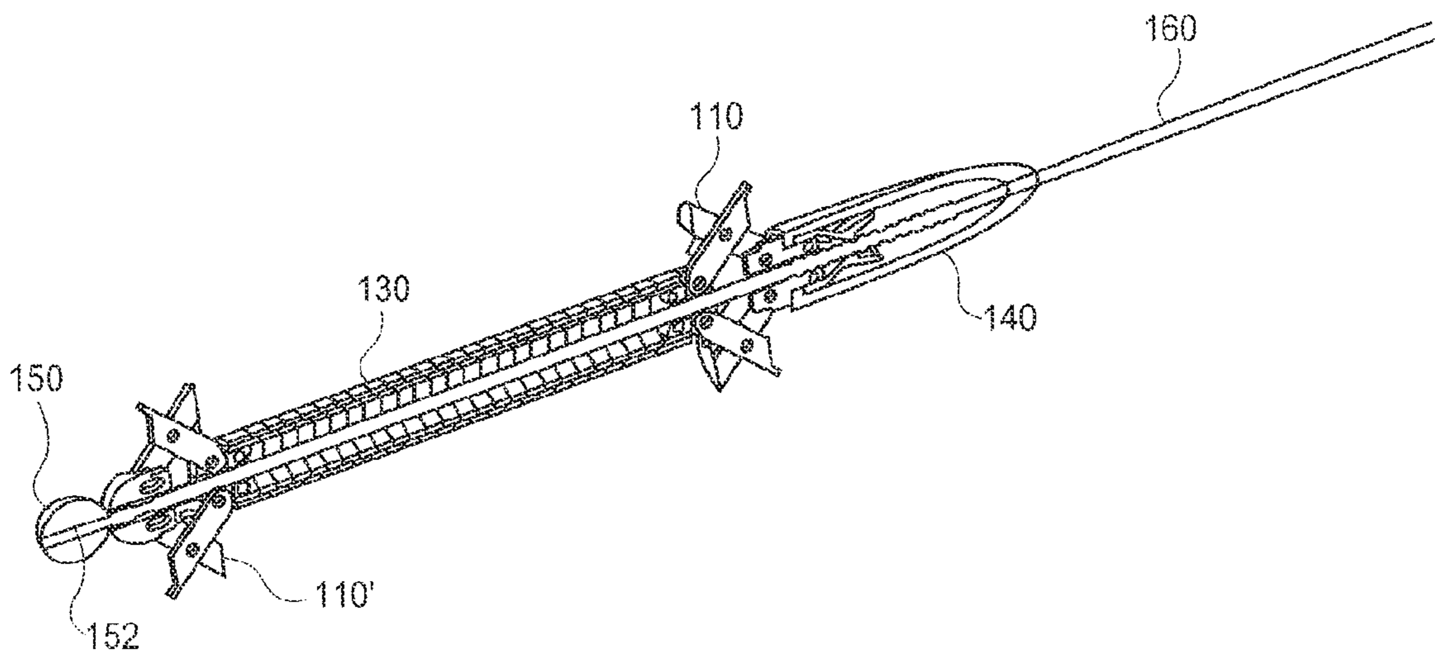
CROSS-SECTION DEPLOYED
