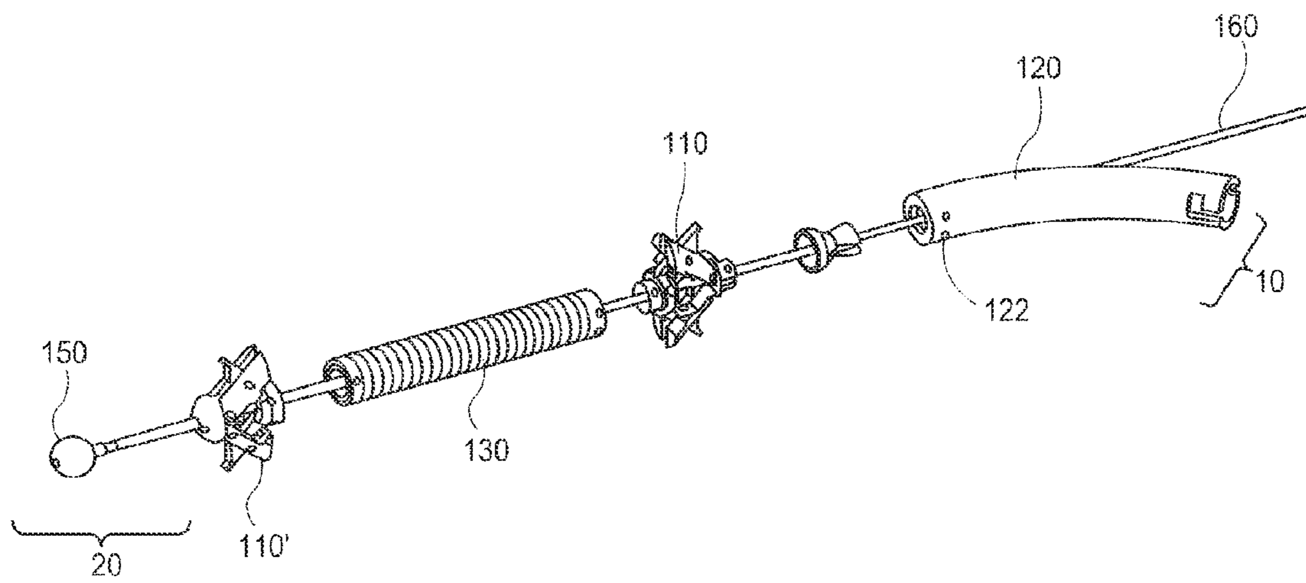
EXPLODED ASSEMBLY
