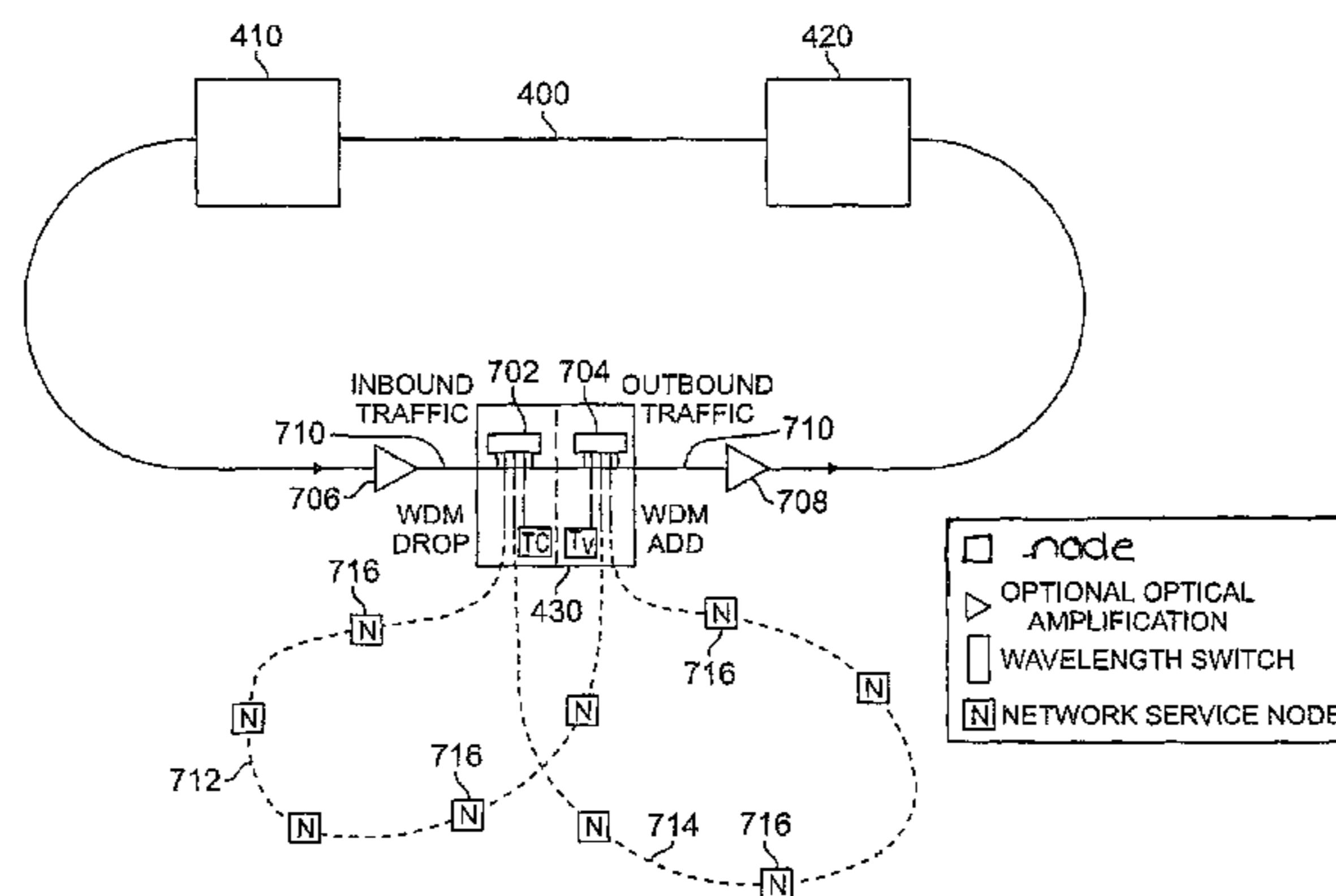
COMMUNICATION SYSTEM TO ADD/DROP SIGNALS ONTO SUBTENDING RINGS (1 FIBER OF UNIDIRECTIONAL RING OR A SINGLE FIBER BIDIRECTIONAL RING)
