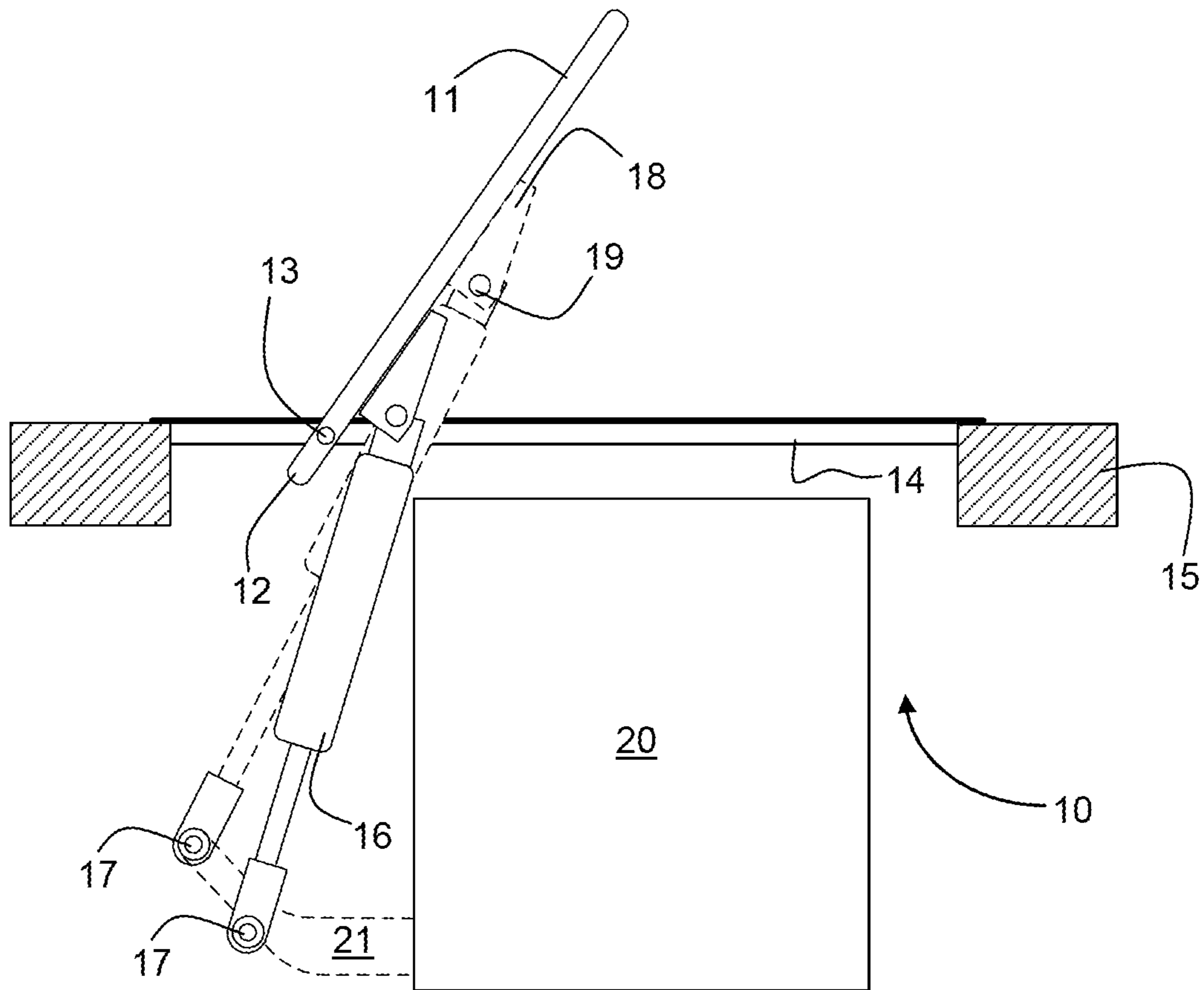
FIG. 3 (PRIOR ART)
