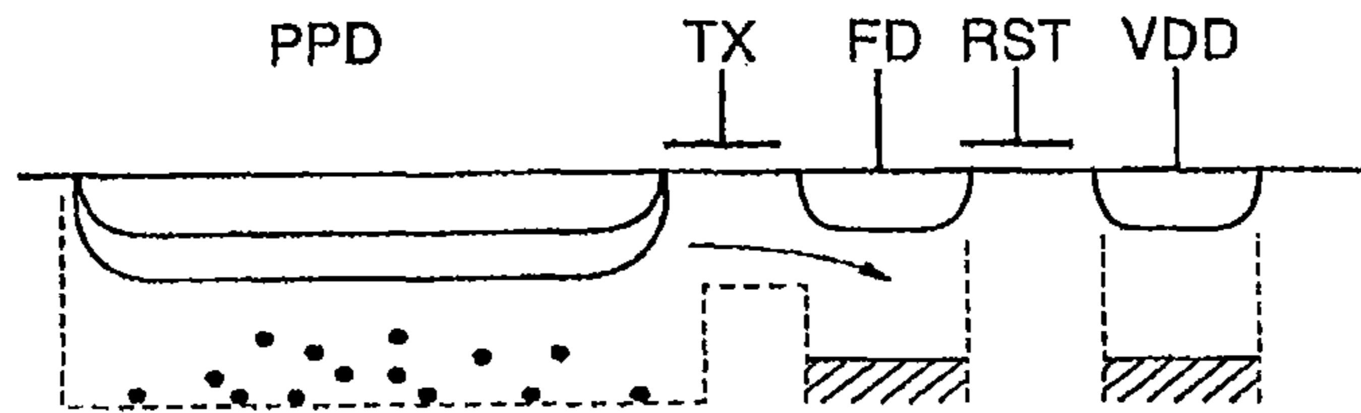
FIG. 1 (PRIOR ART)
