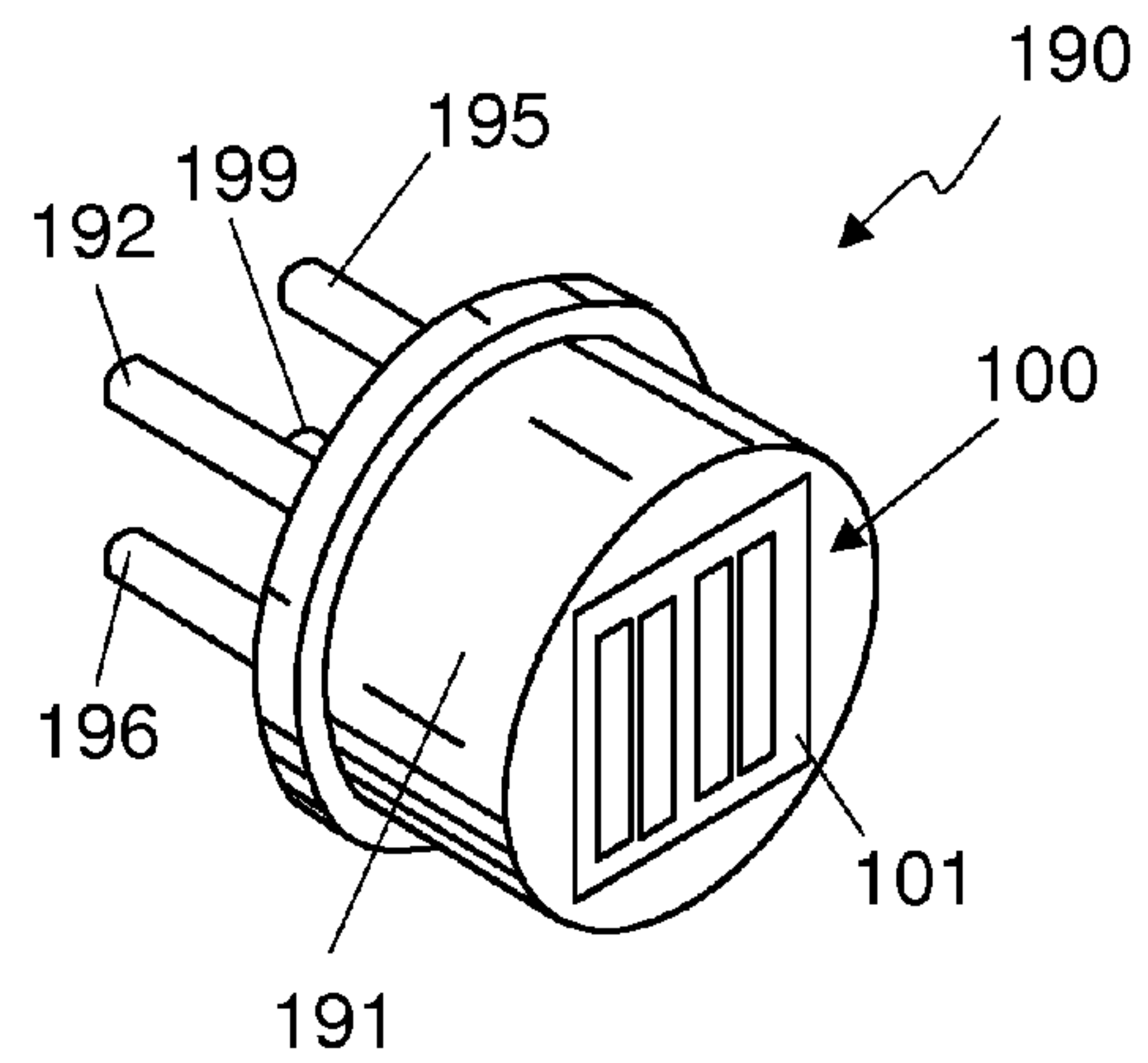
FIG. 1D
