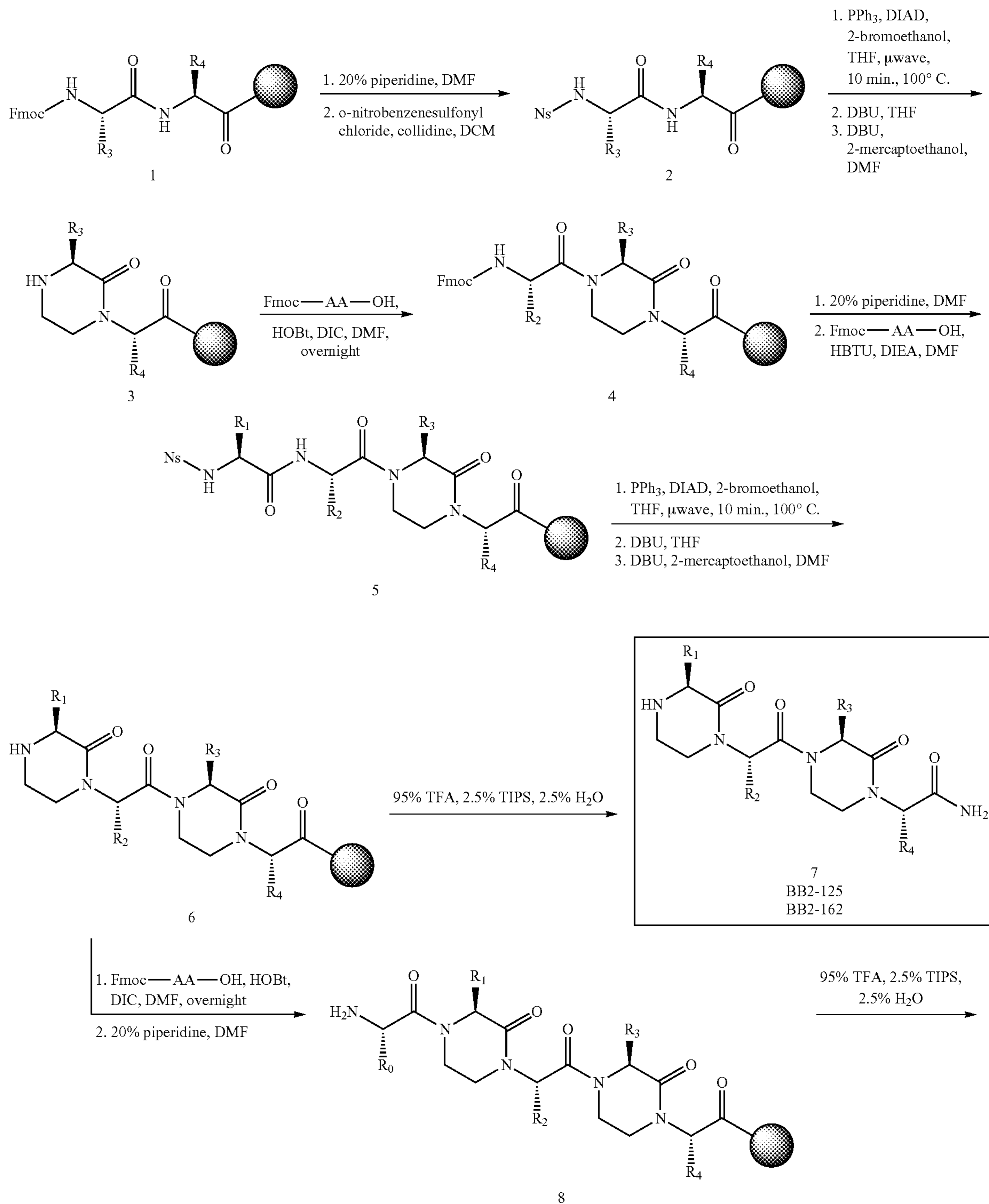
Scheme 1
