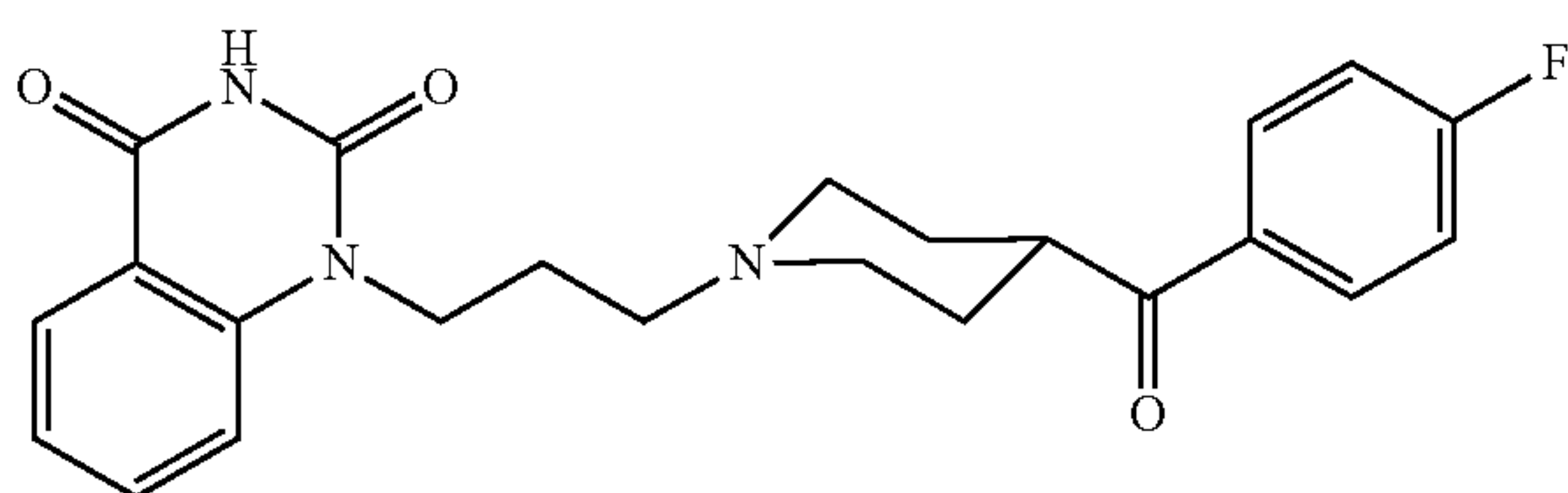
compound 11
