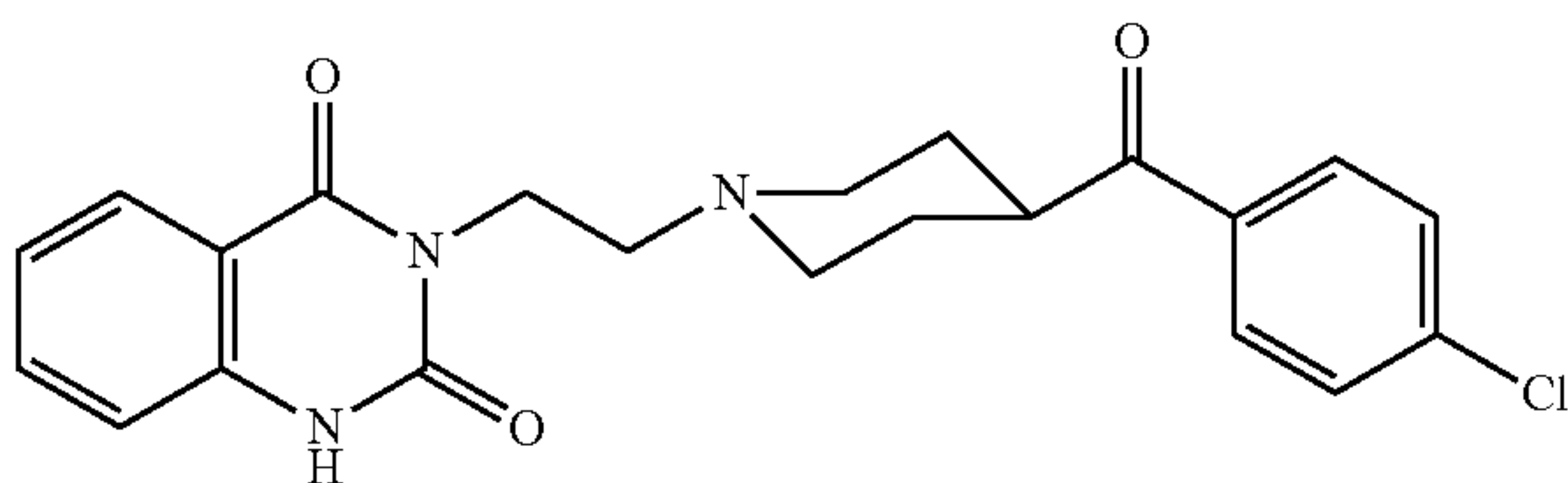
compound 12
