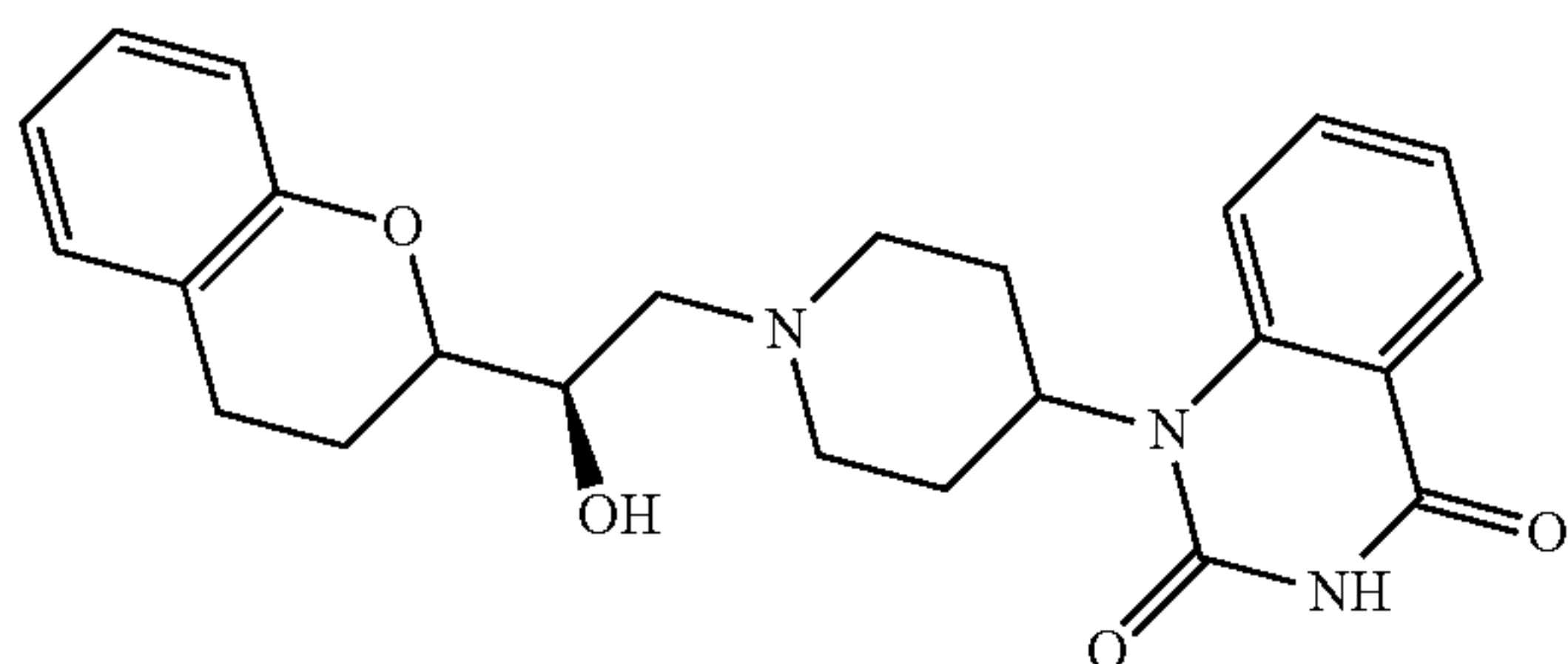
compound 9
