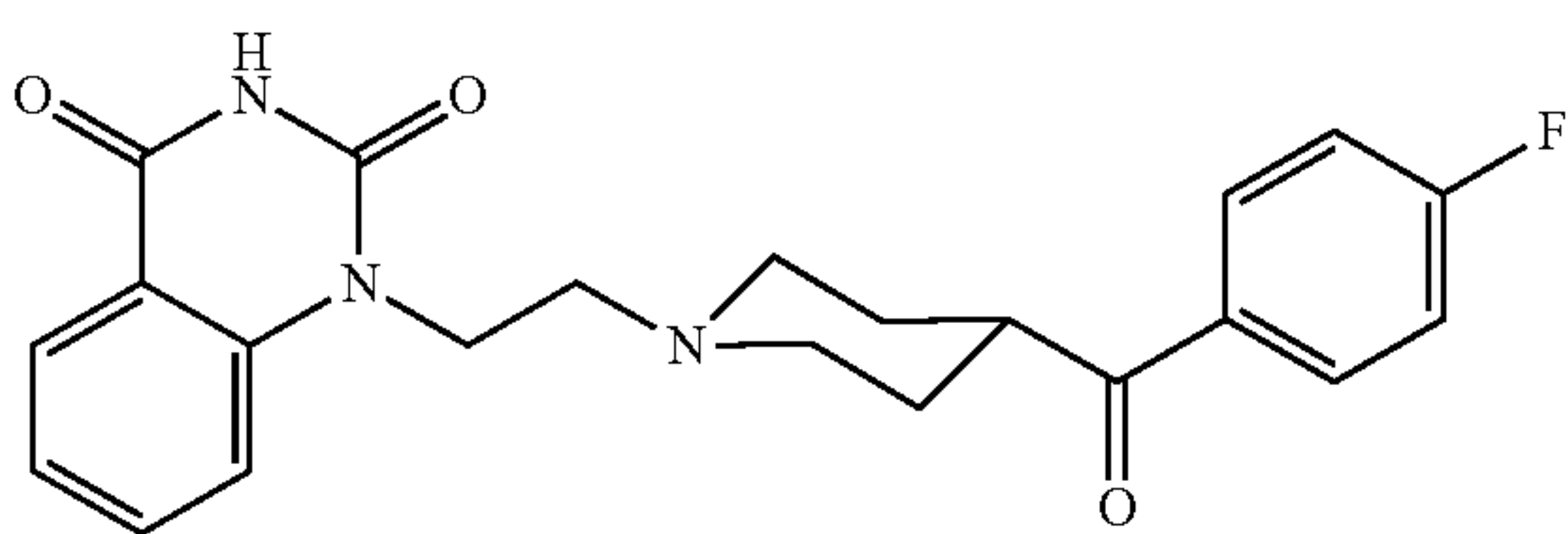
compound 10
