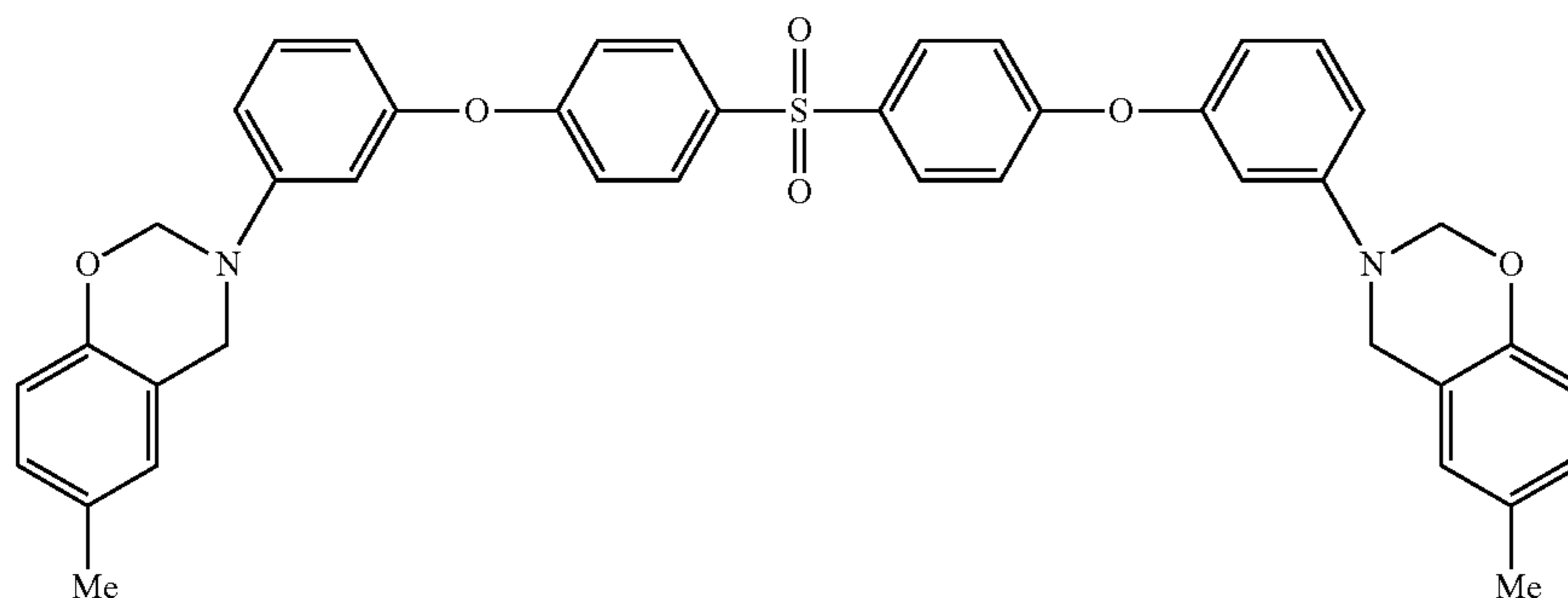
M-ESEDA based benzoxazine
