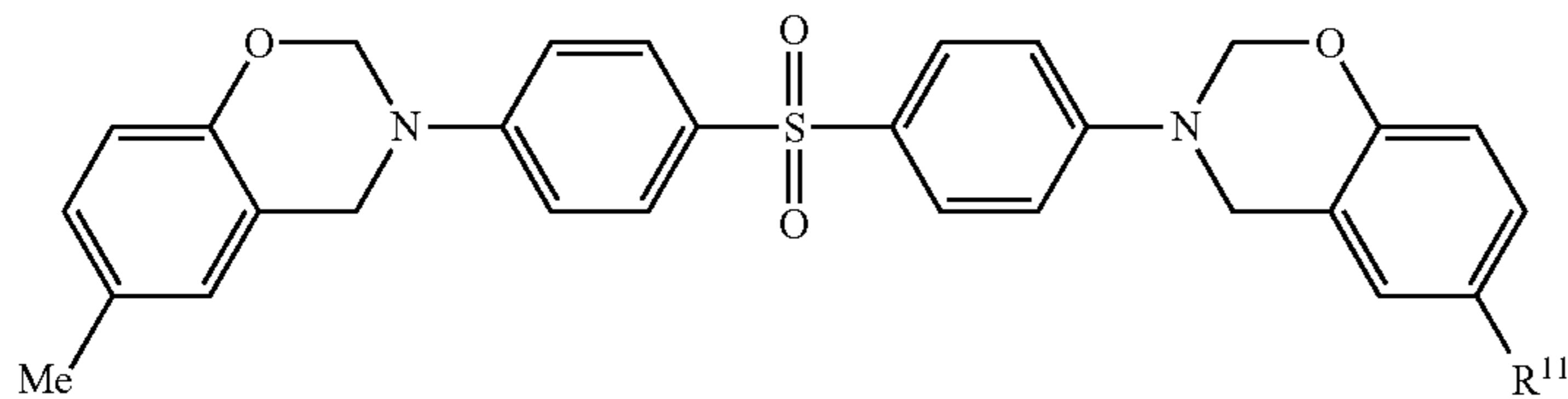
4,4'-DDS based benzoxazine
