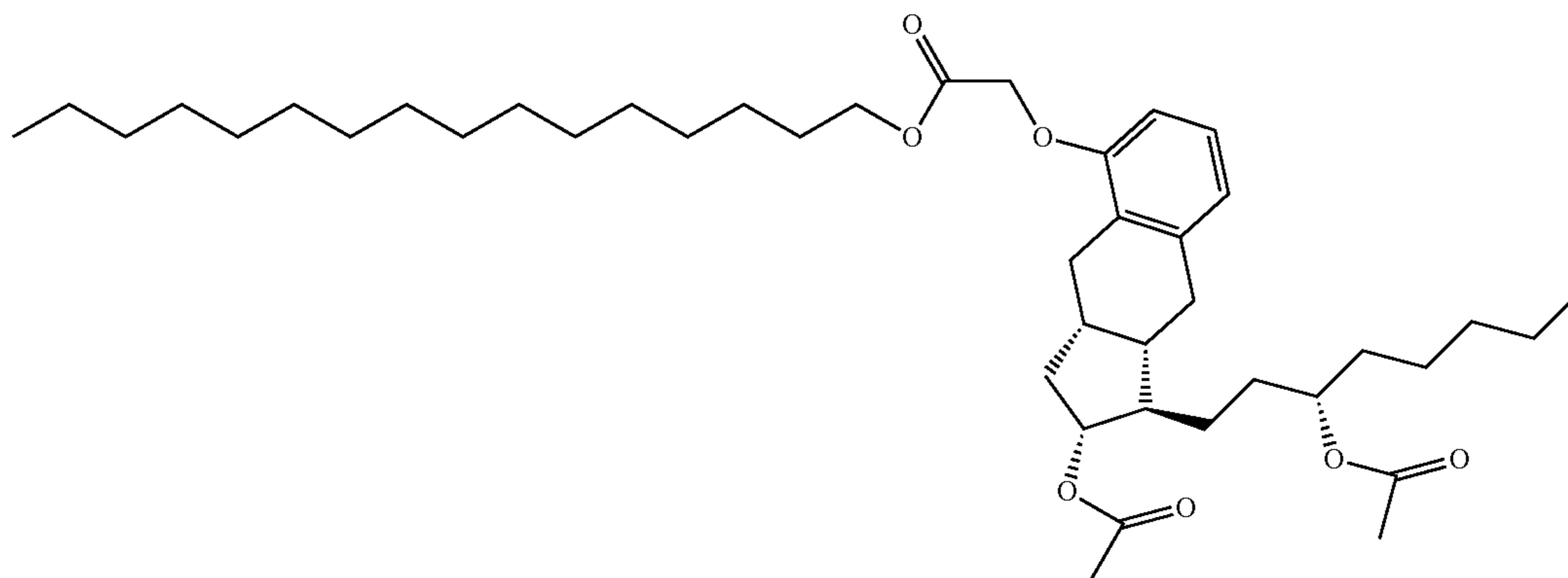
Synthesis of C 16 TR-OAc
