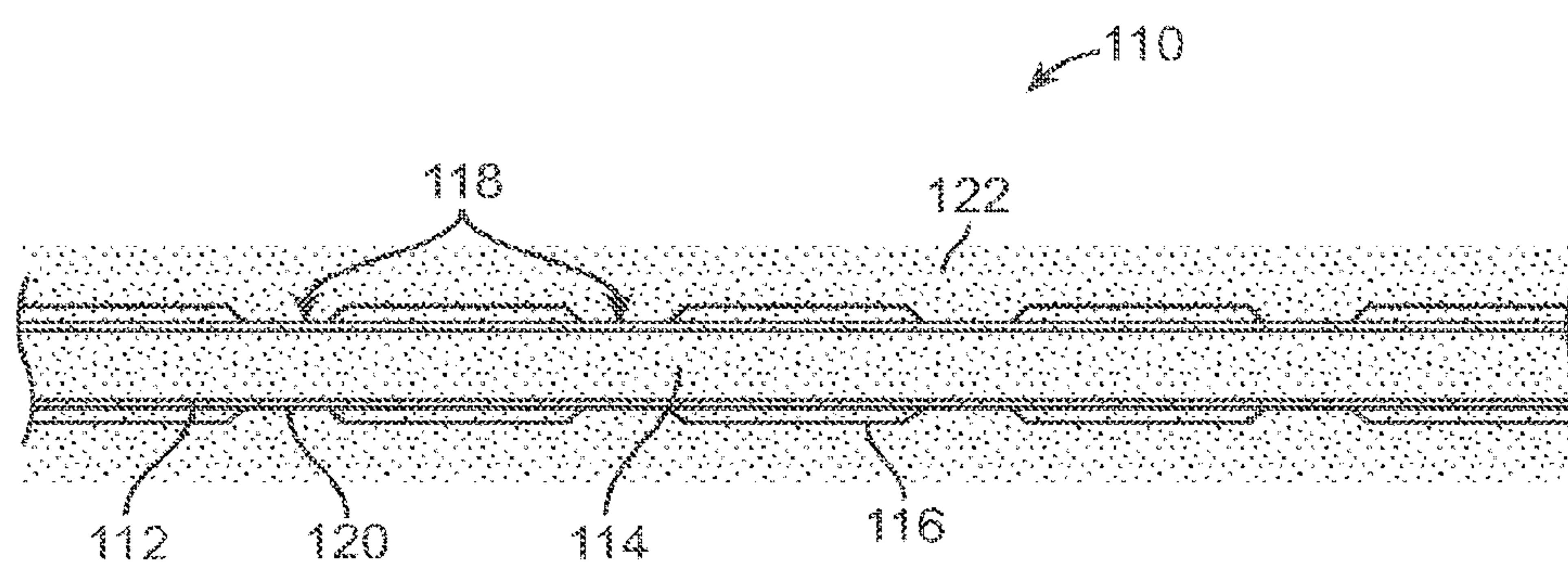
FIG. 6 (PRIOR ART)
