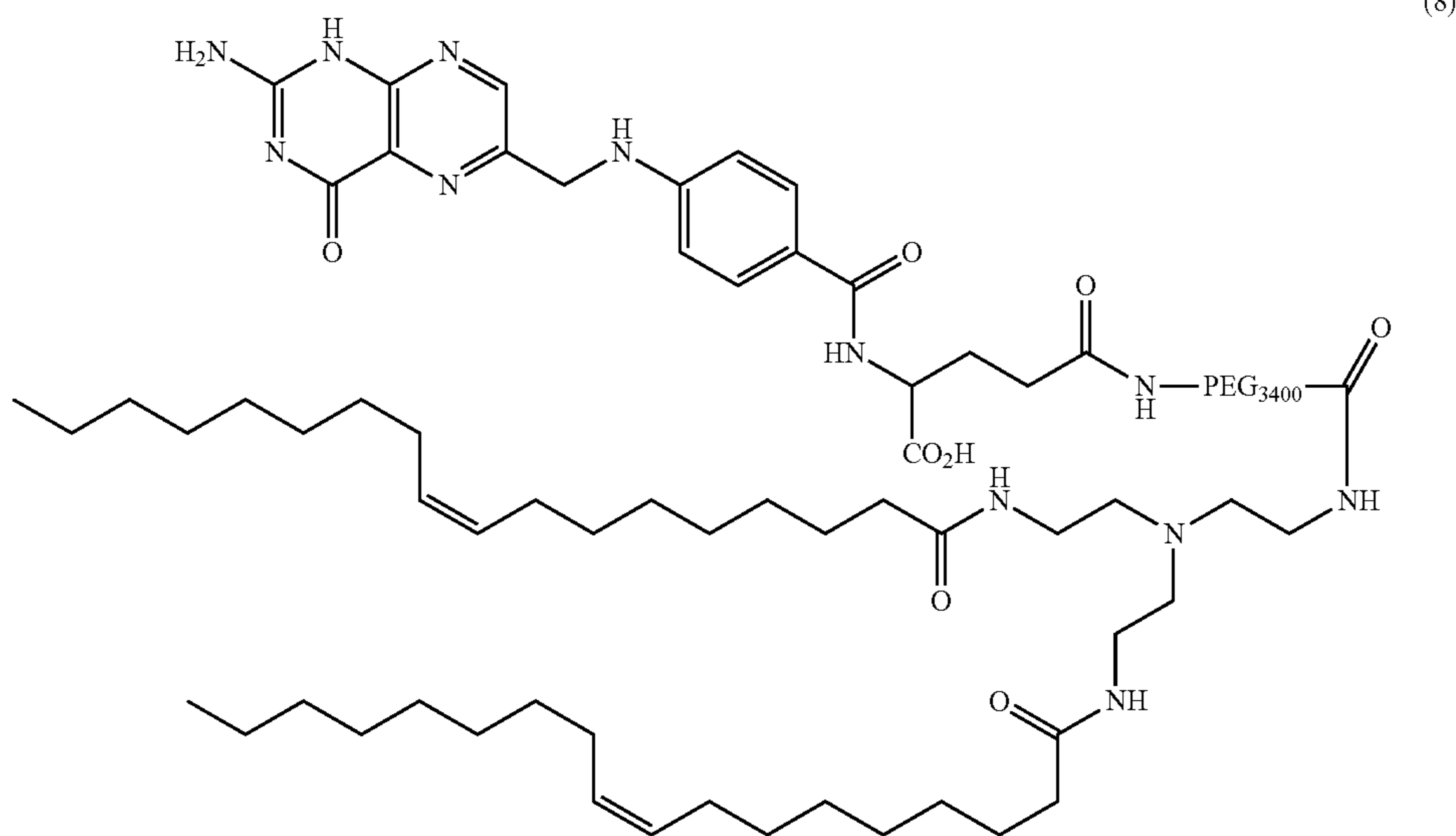
folate-PEG-dioleoyl monoamine
