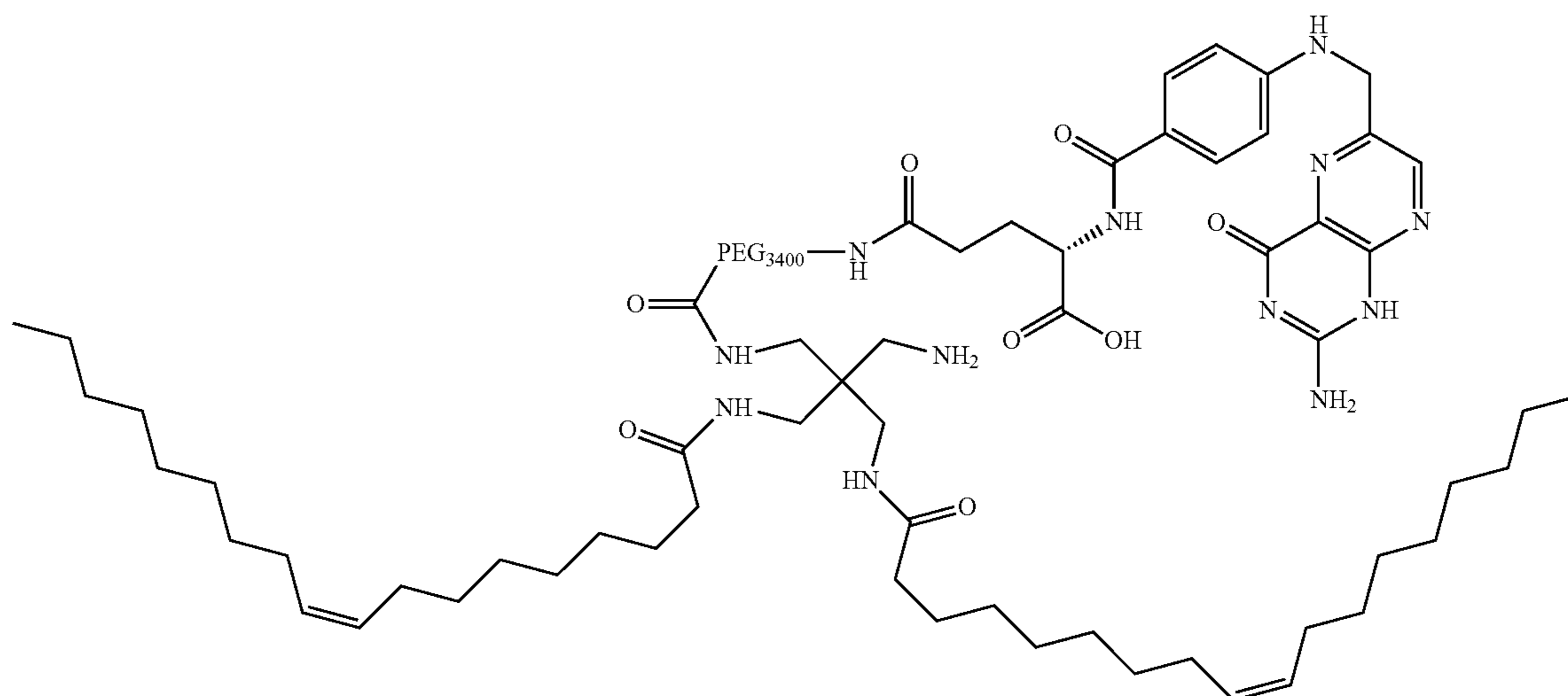
folate-PEG-dioleoyl crossamine
