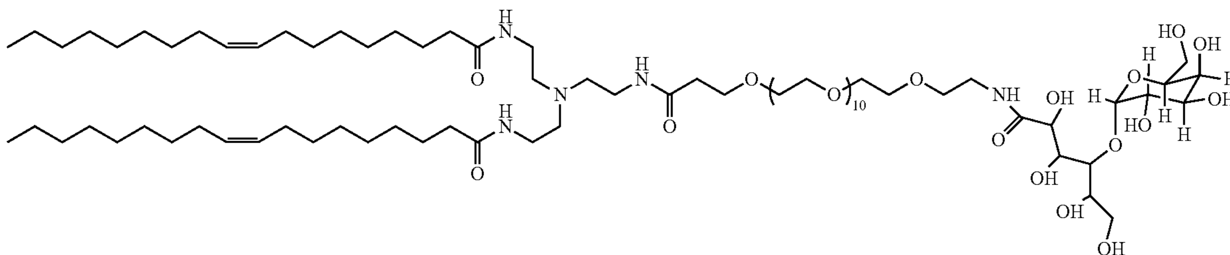
lactobionyl-dioleoyl monoamine
