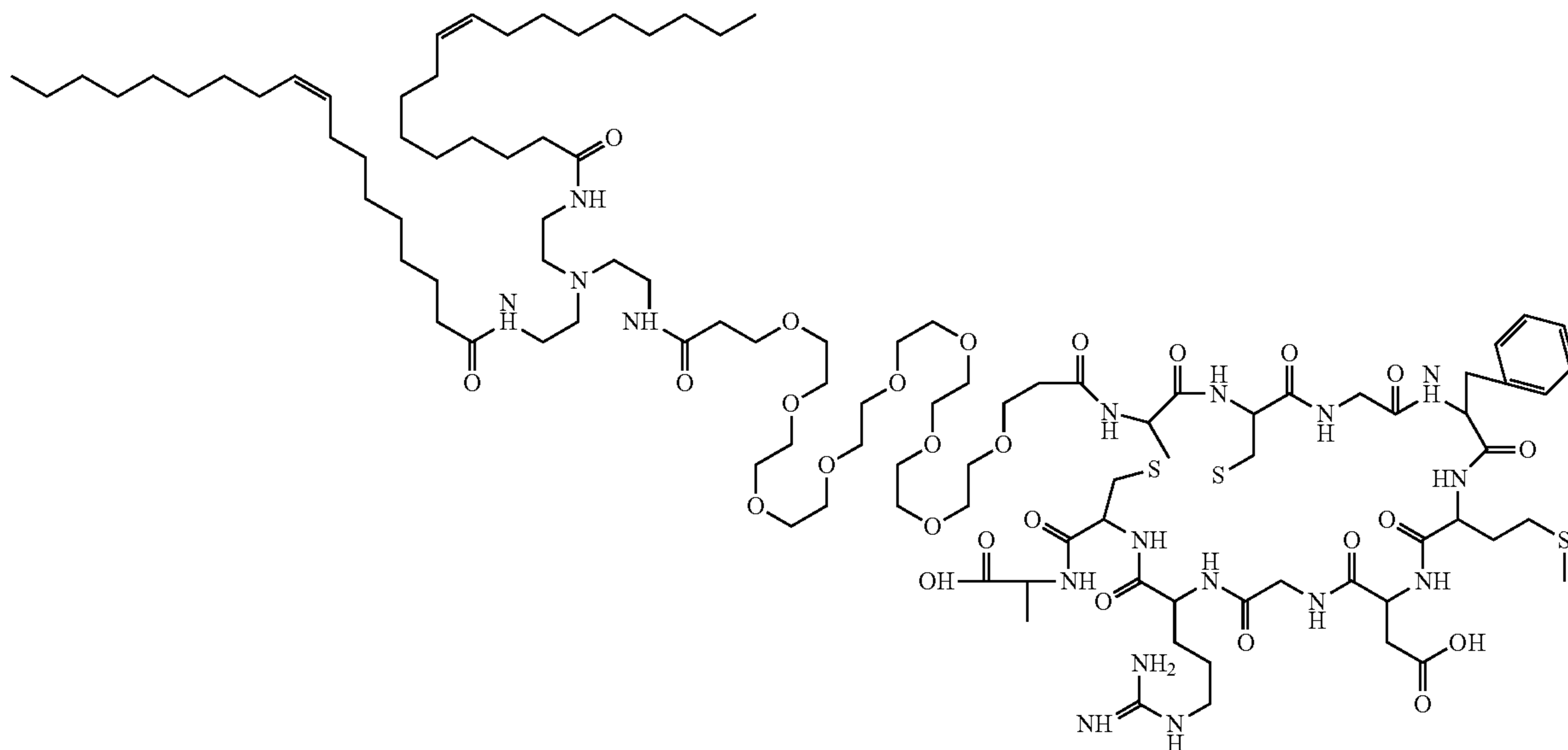
RGD-dioleoyl monoamine
