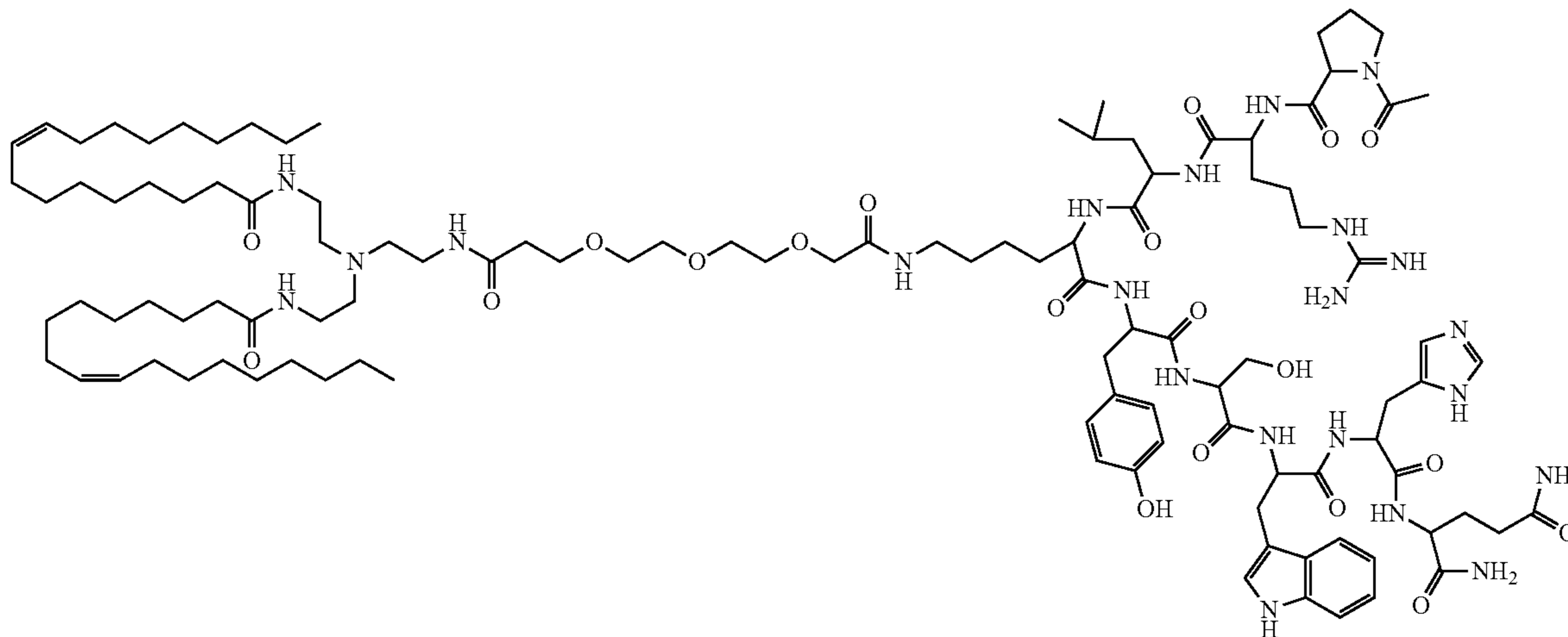
LHRH-dioleoyl monoamine
