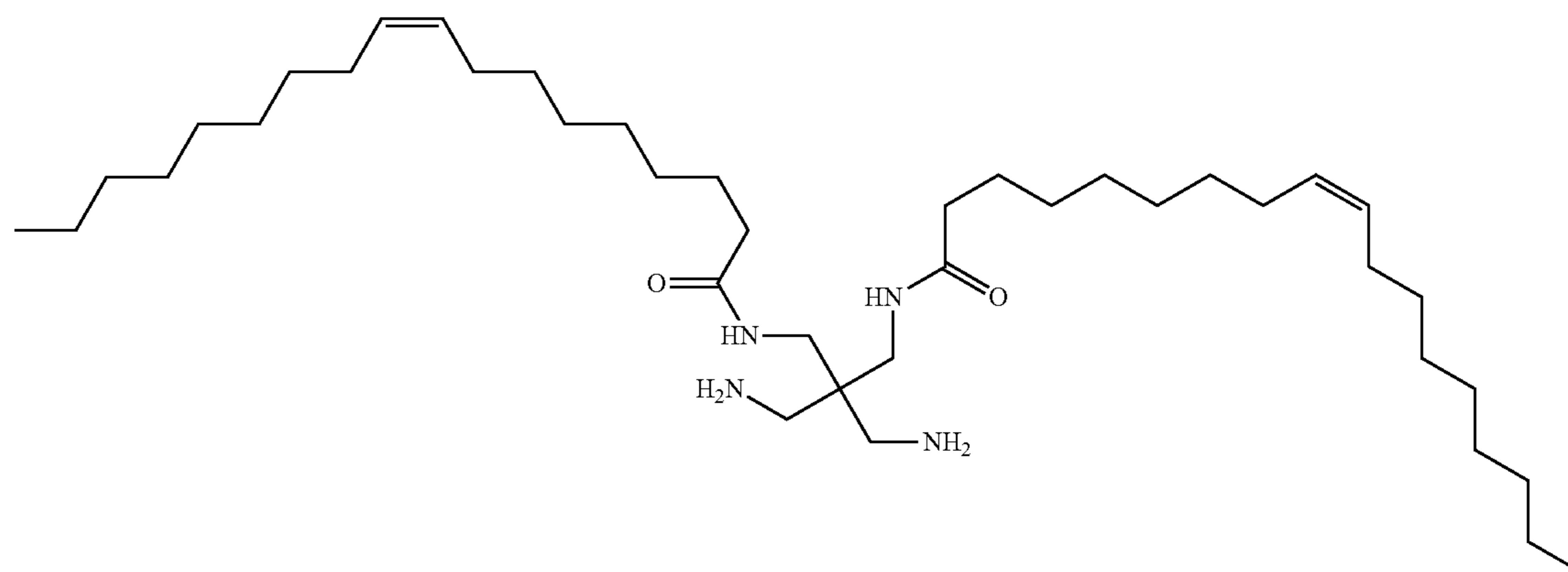
dioleoyl crossamine
