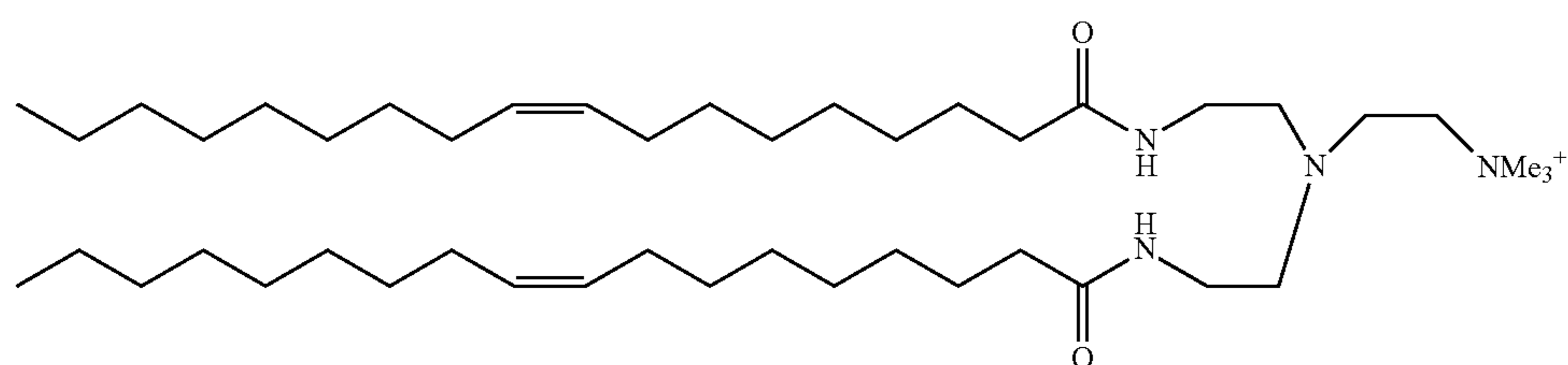
Methyl-dioleoyl monoamine
