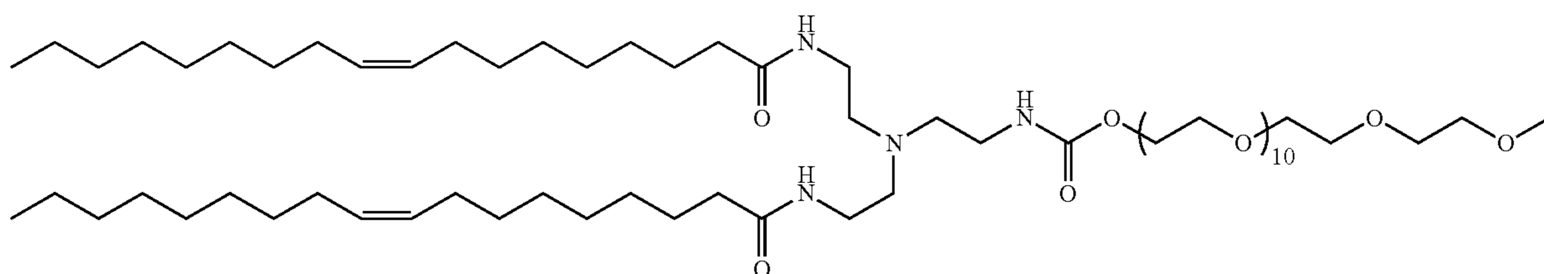
mPEG-dioleoyl monoamine
