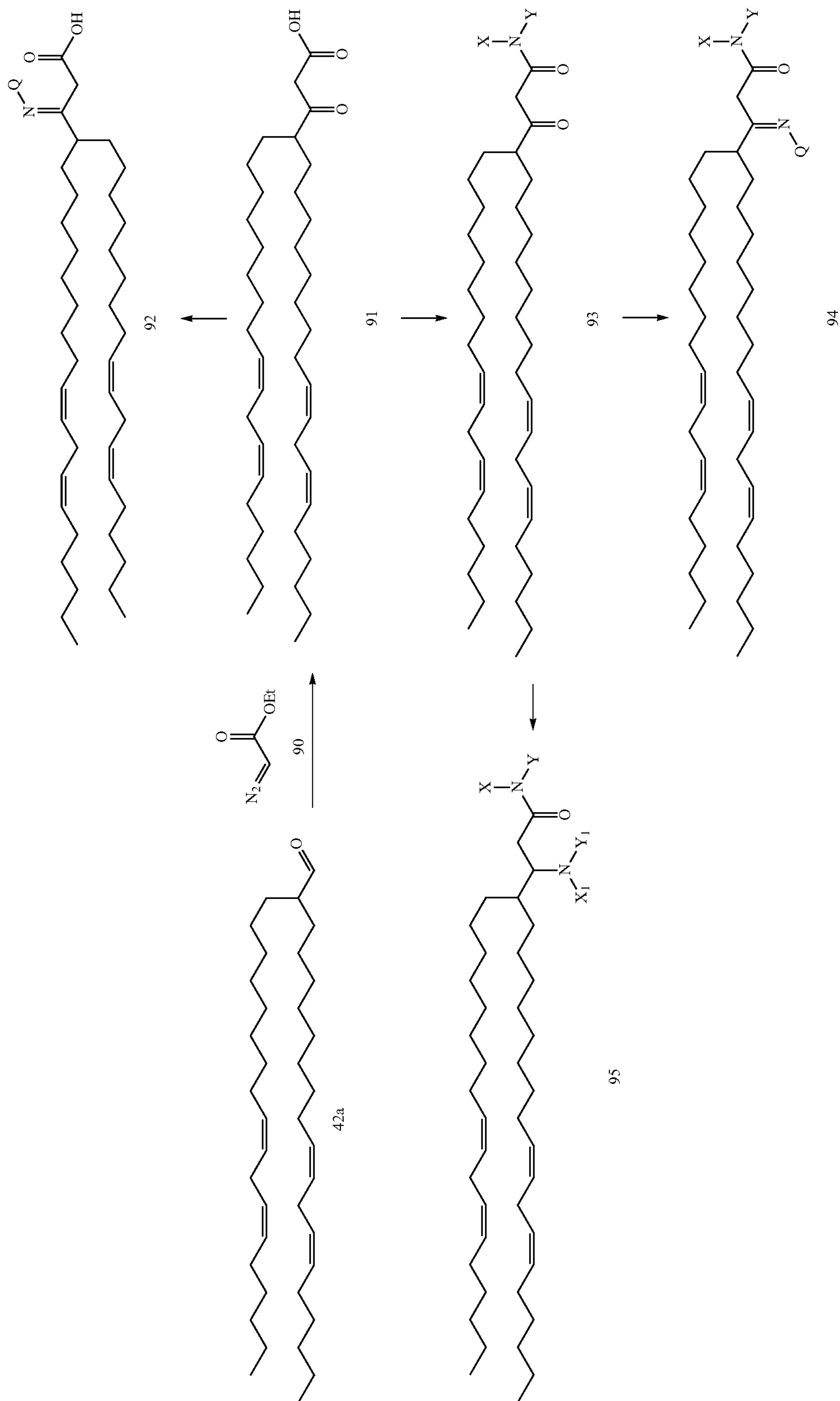
Scheme 7a ( \beta -Keto Acid Analogs) (See, e.g., J. Org. Chem. , 54(14), 1989, 3259 (Table 1))
