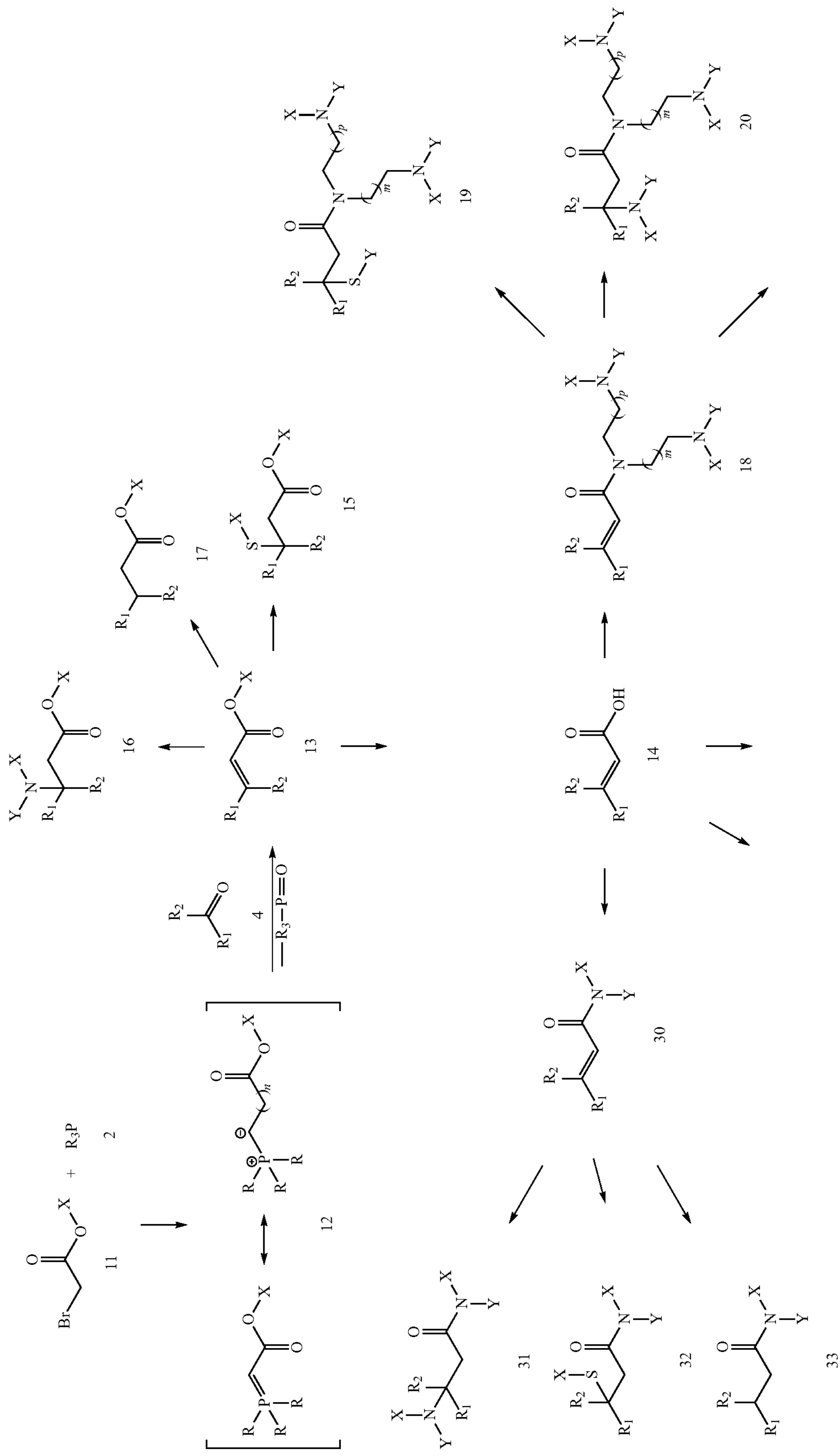
Scheme 2a (Wittig Reaction Followed By 1,4-Michael Addition)
