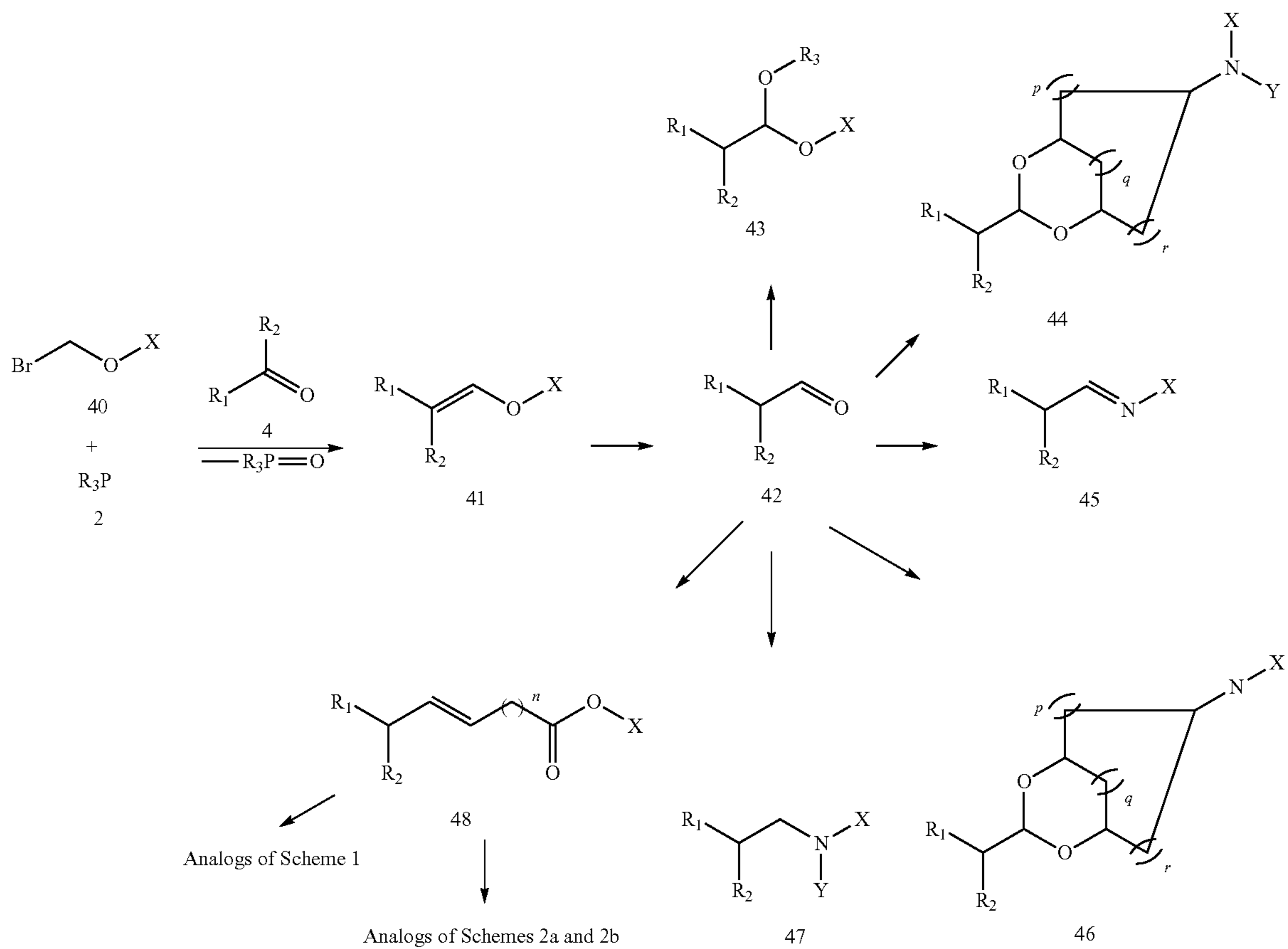
Scheme 3 (Wittig Reaction Followed By Michael Addition)
