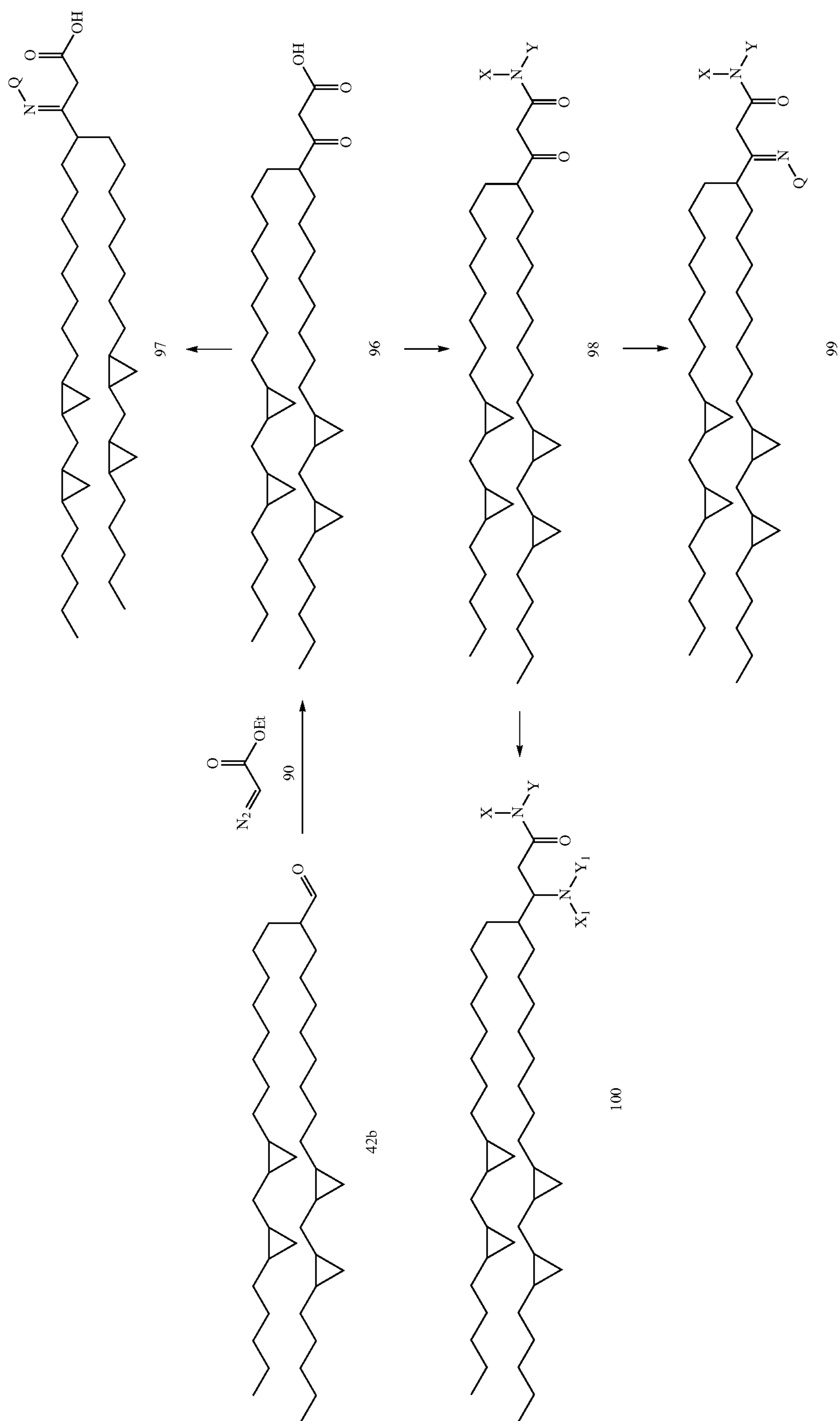
Scheme 7b ( \beta -Keto Acid Analogs)
