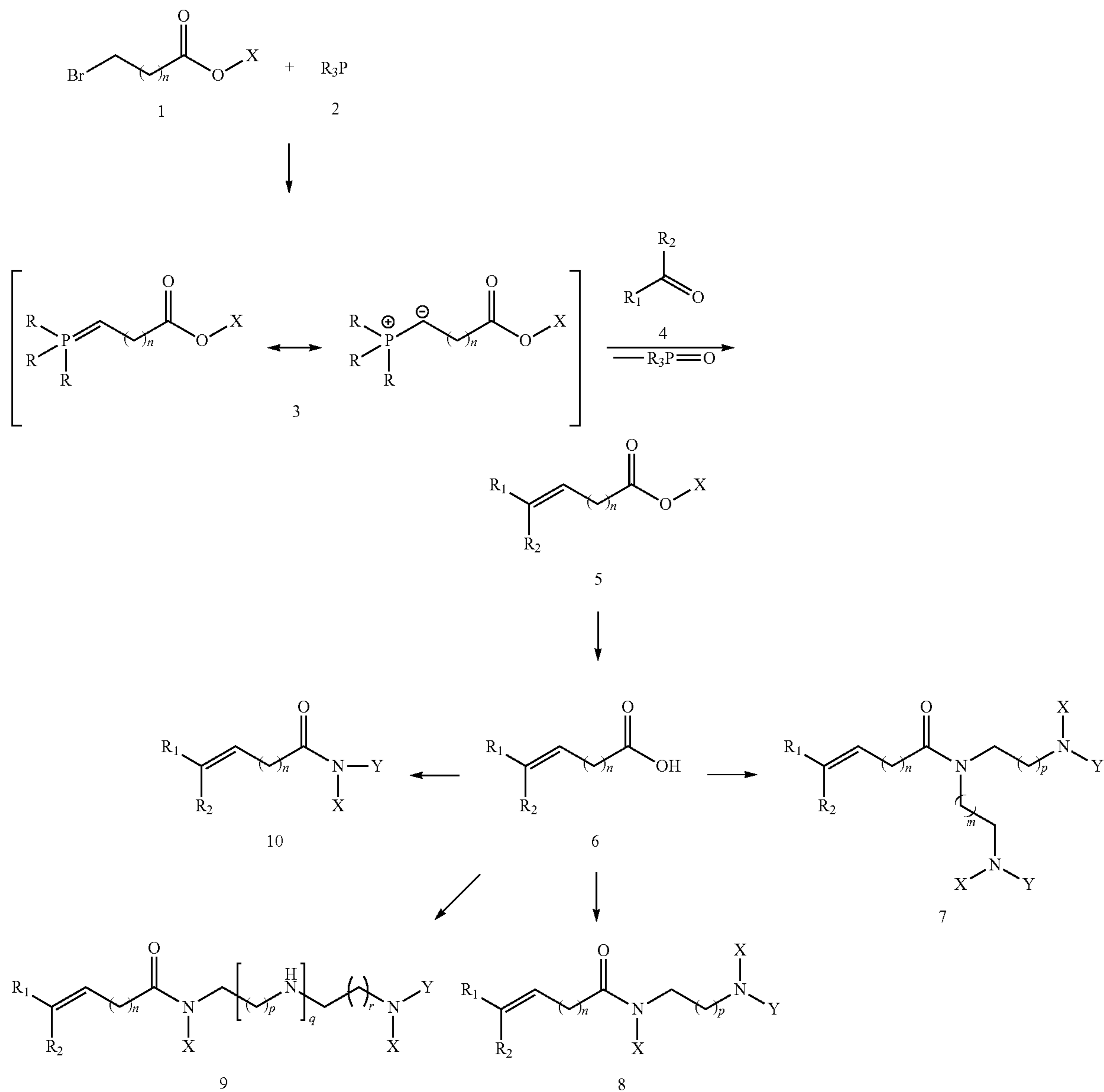
Scheme 1 (Wittig Reaction)
