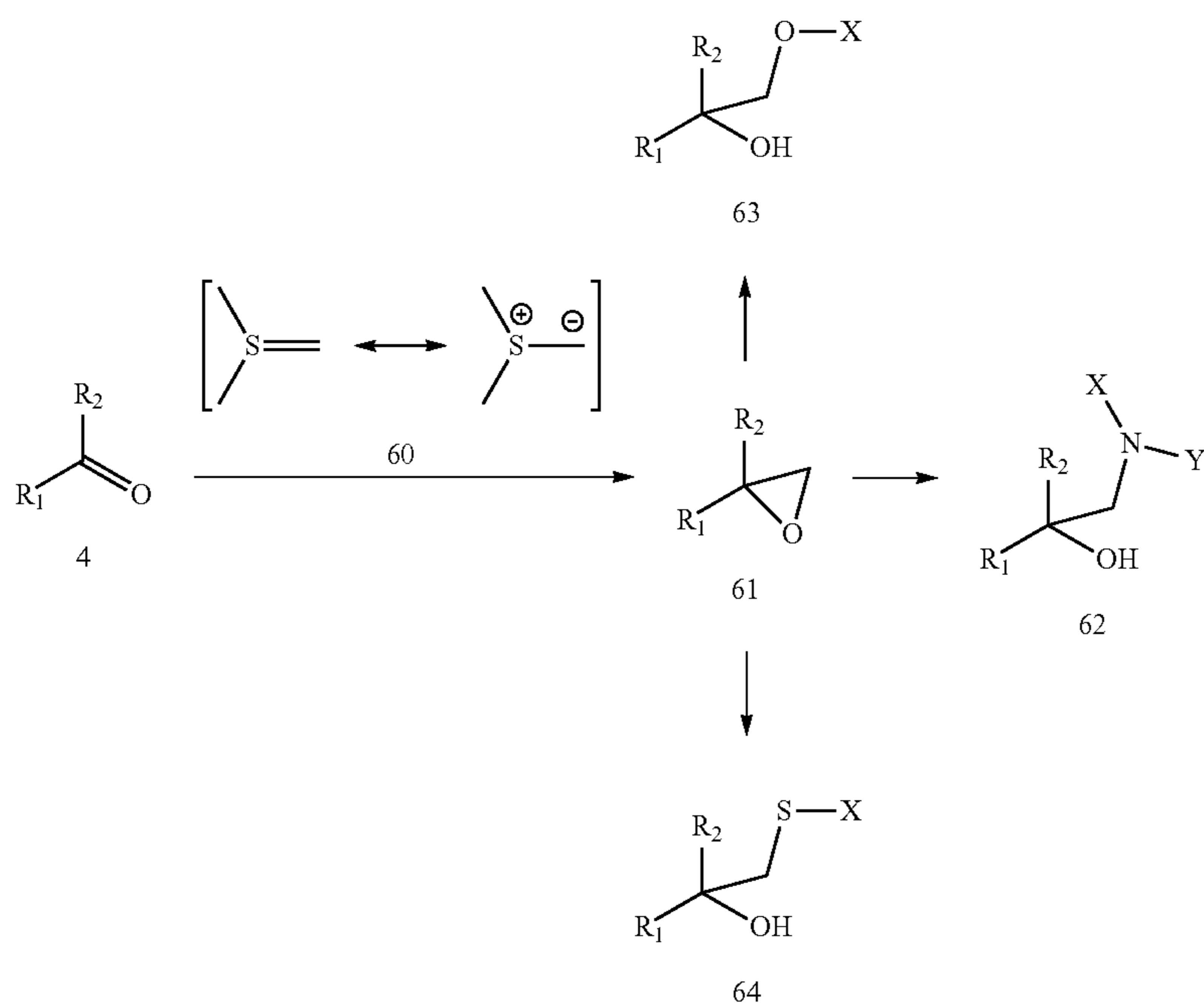
Scheme 4 (Sulfur Ylides)
