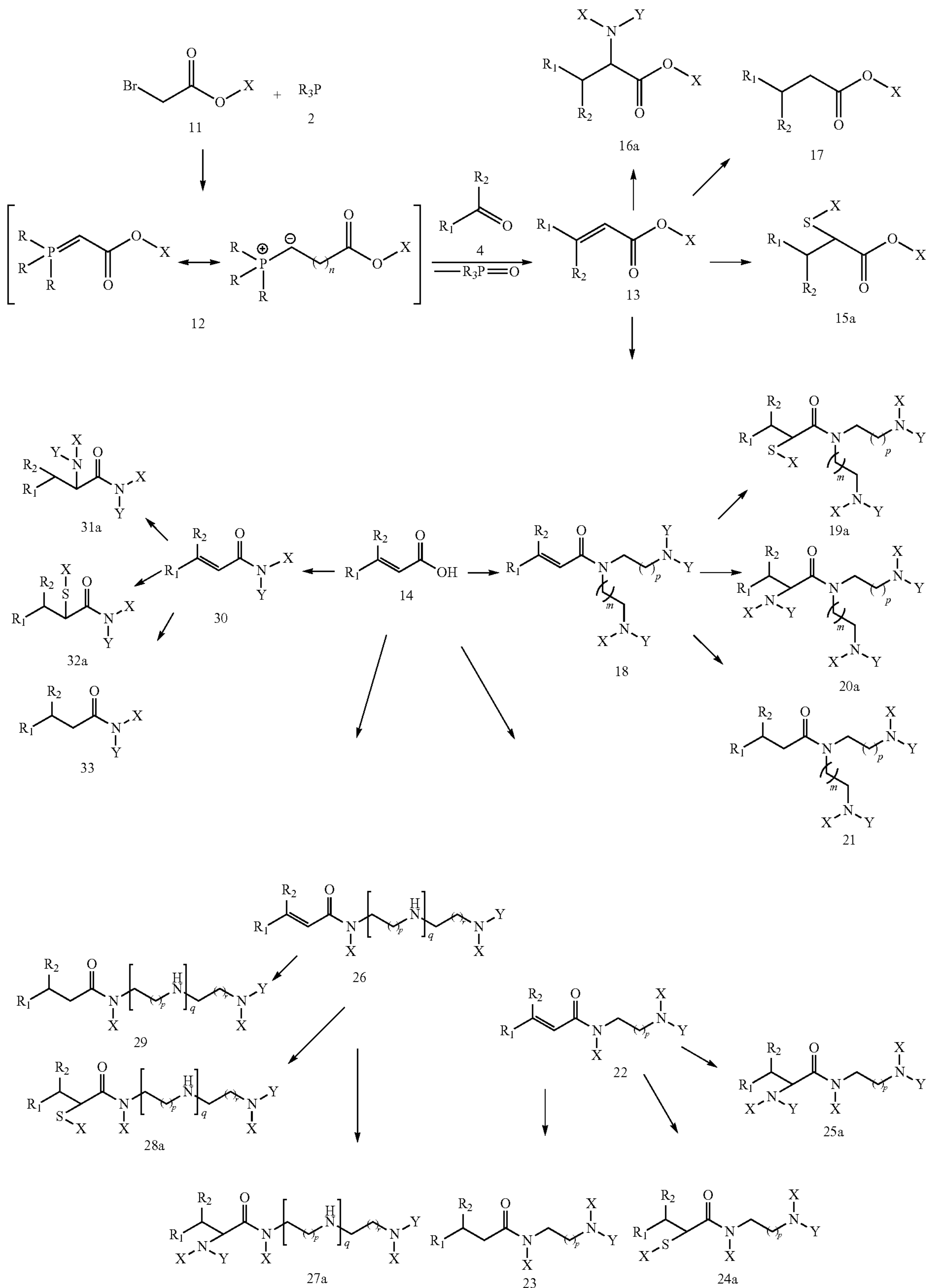
Scheme 2b (Wittig Reaction Followed By 1,2-Michael Addition)
