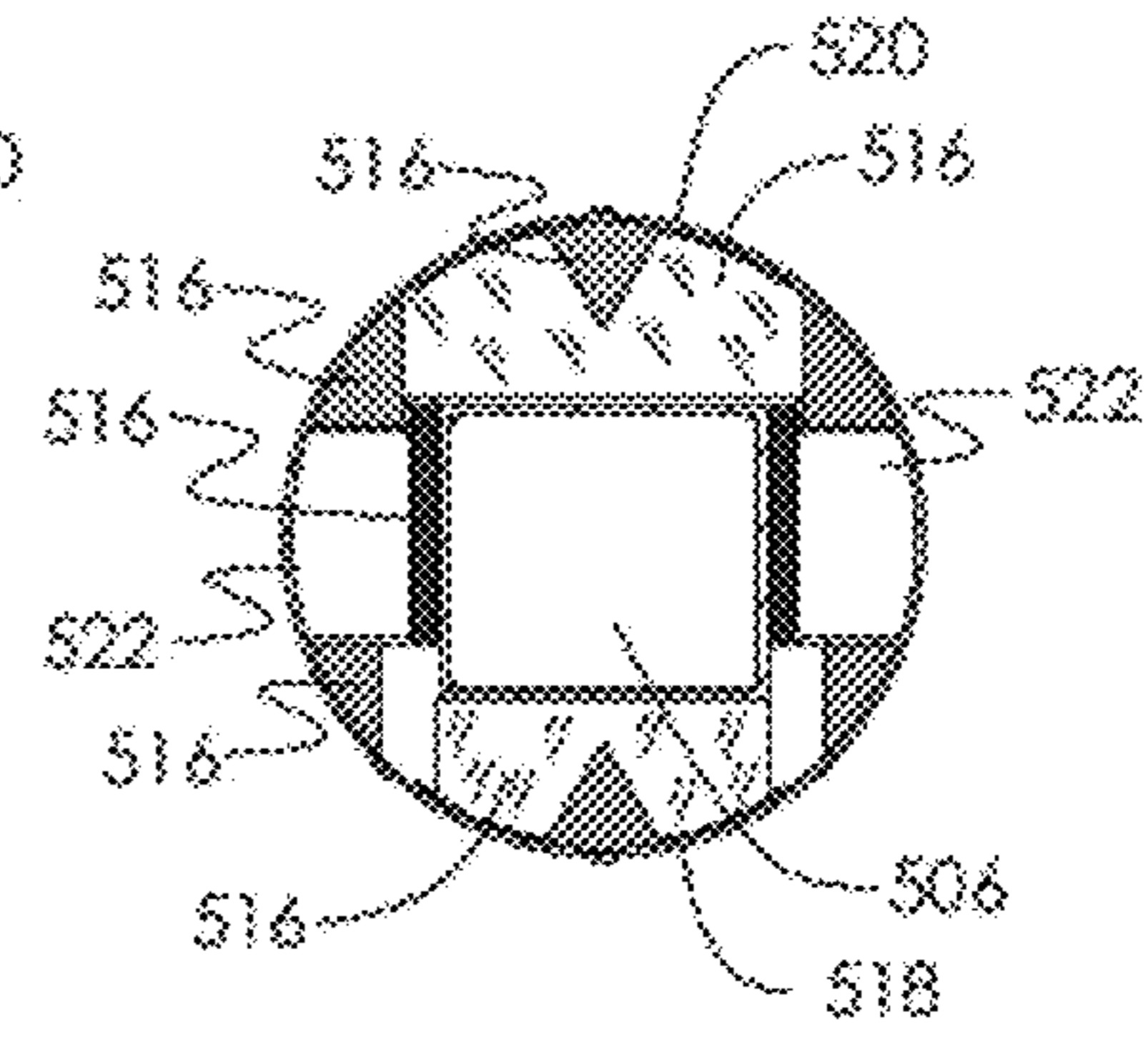
SECTION B-B FIG. 5C
