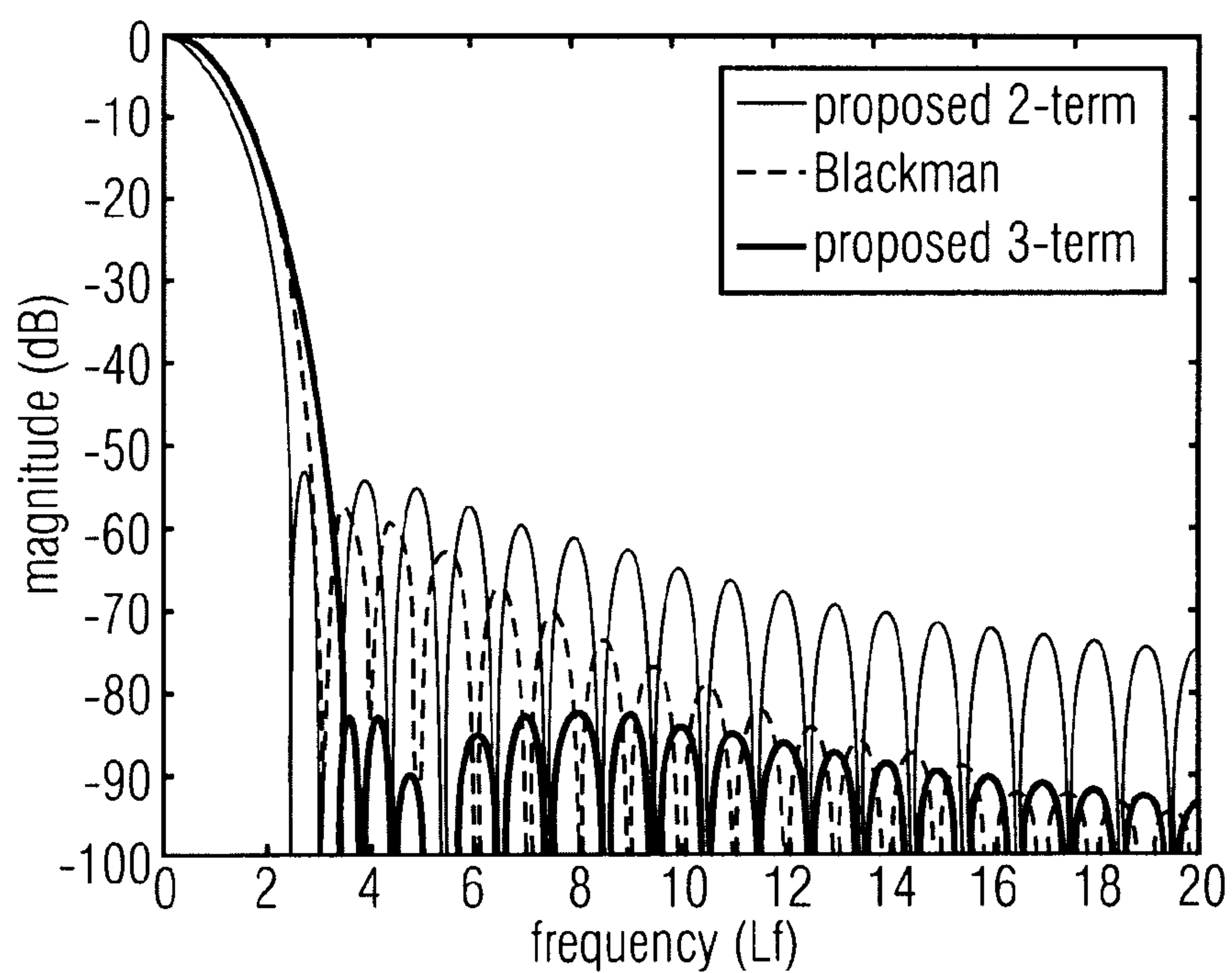
FIG. 13 (THE PROPOSED OPTIMIZED SUM-OF-SINES WINDOWS (19))
