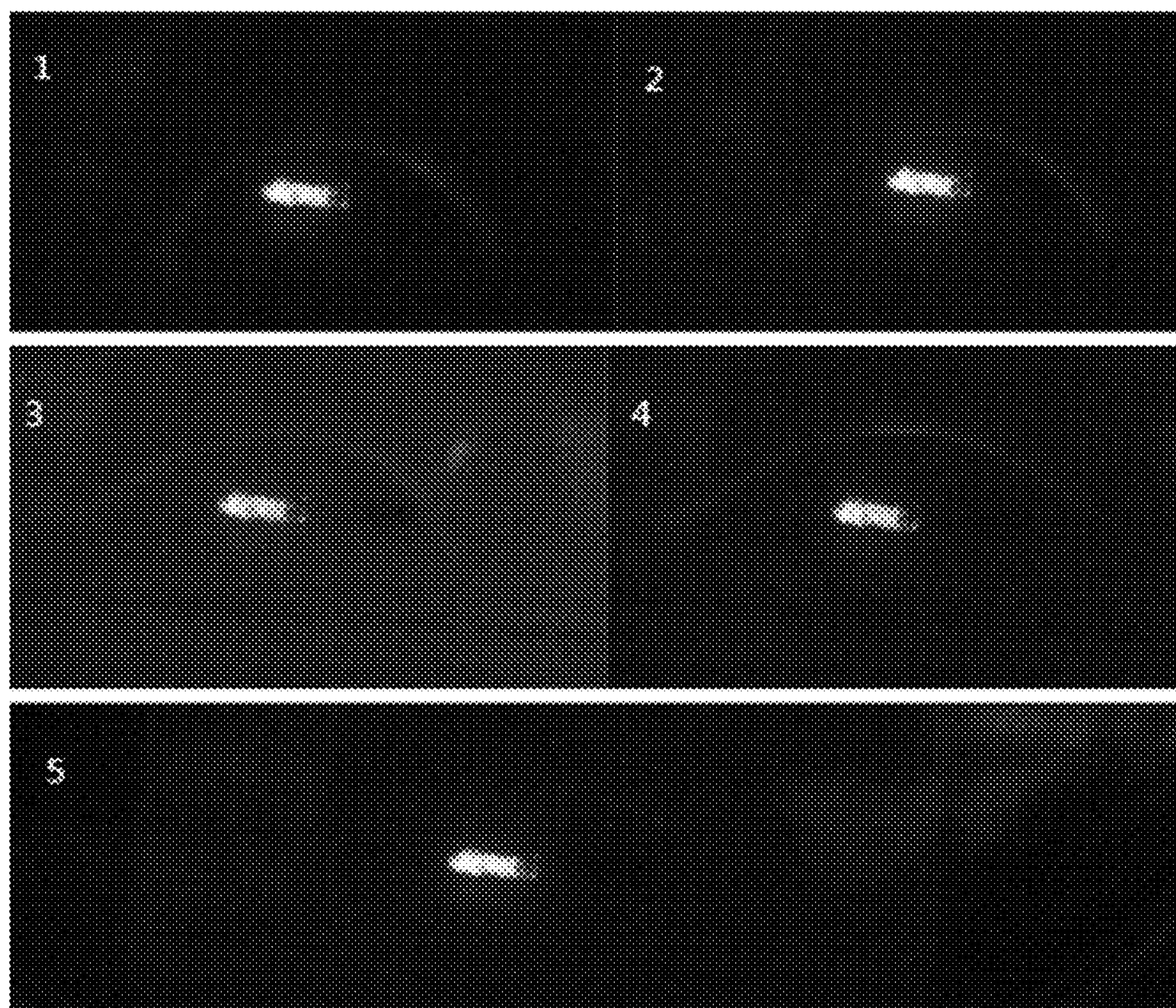
Anode spots under different vacuum pressures
