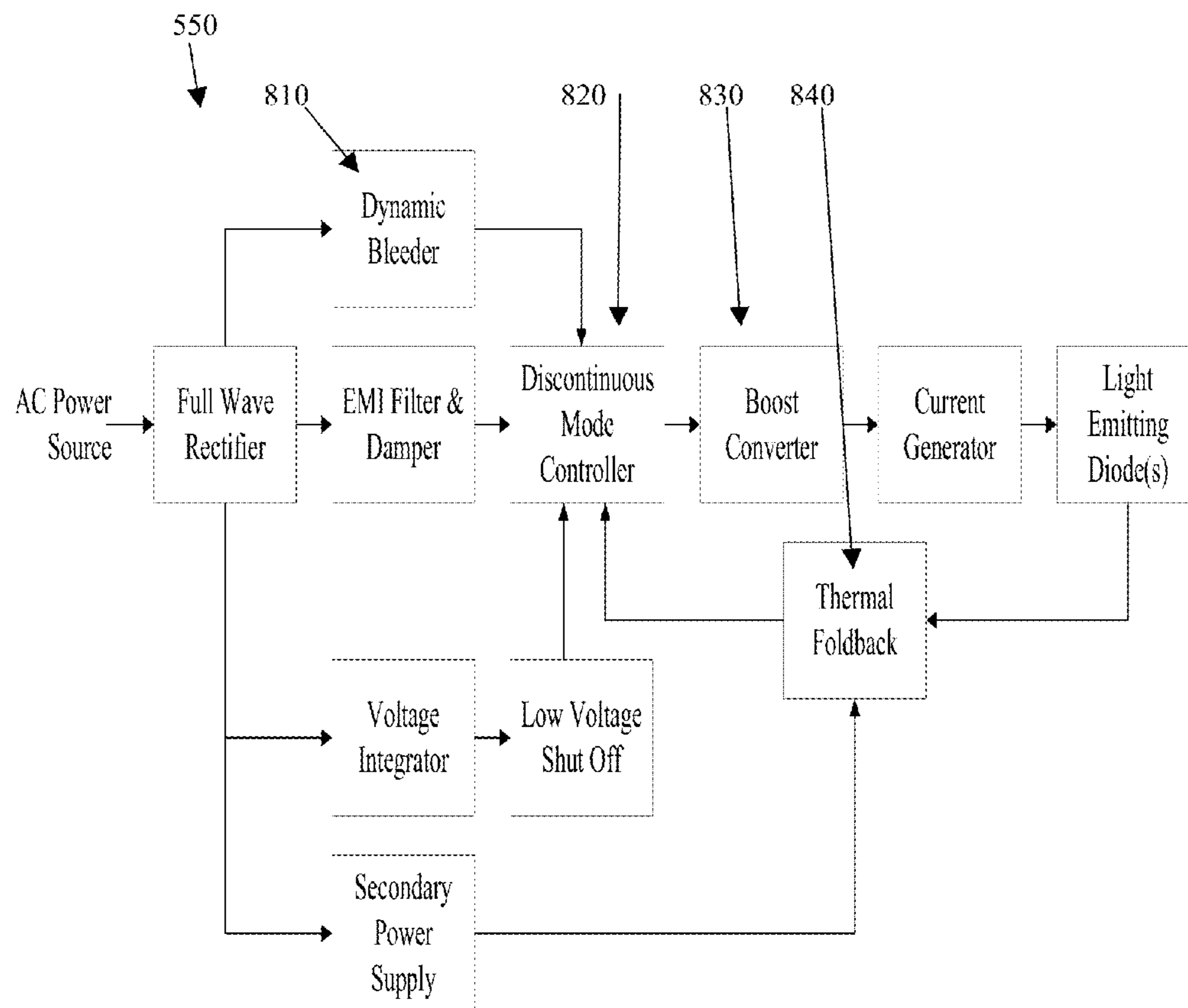
FIG. 4 Electrical Block Diagram
