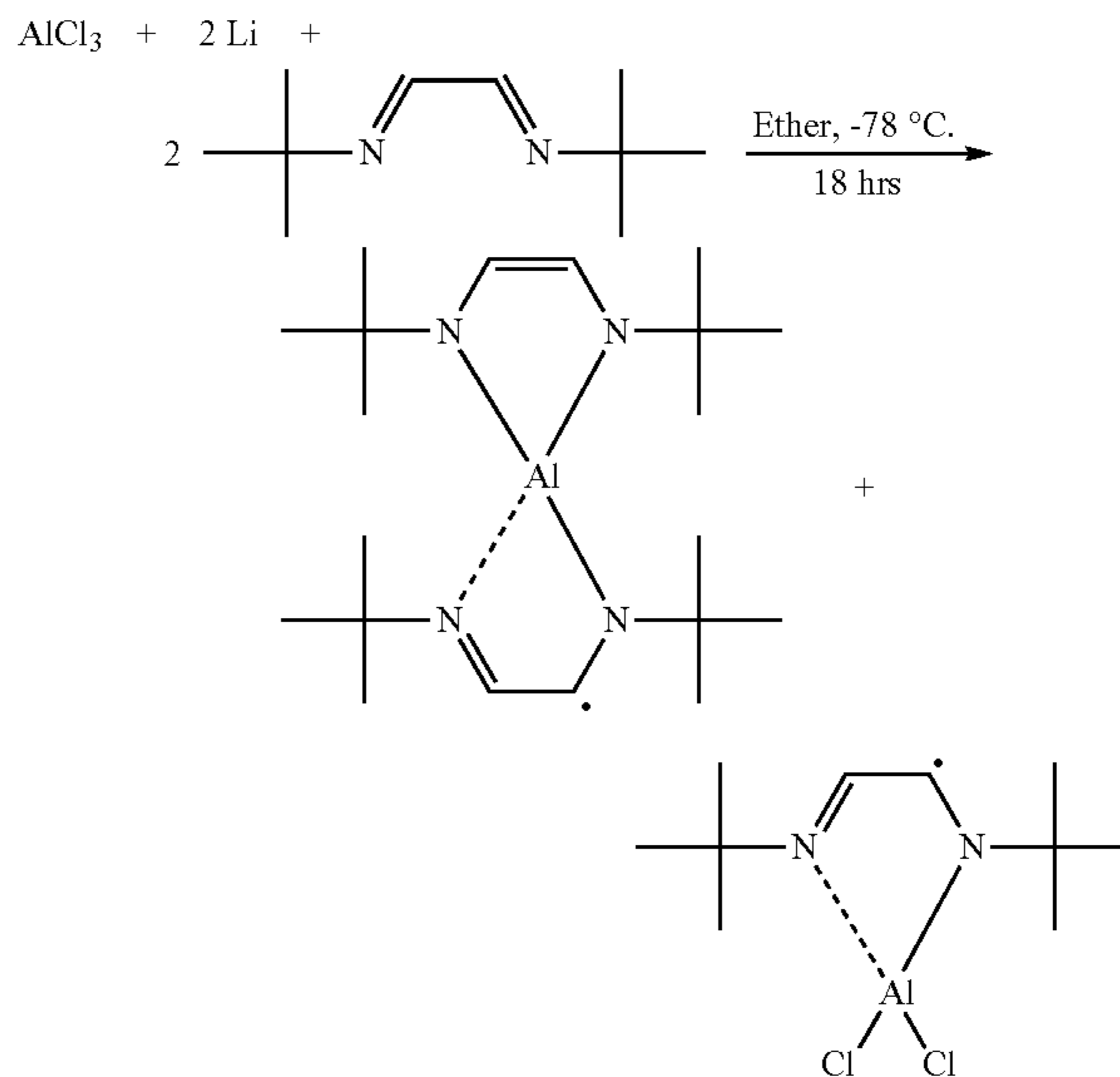
Scheme 4: Synthetic procedure for \text{Al}(\text{dad}^{t\text{Bu}2})\text{Cl}_2
