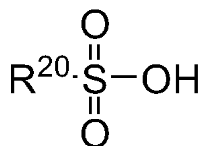
sulfonic acids
