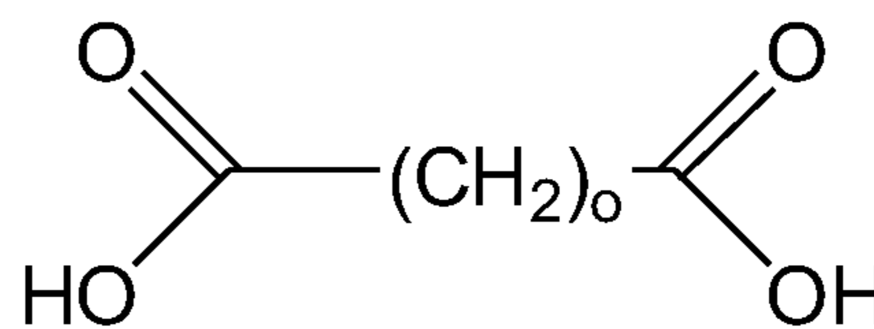
dicarboxylic acids
