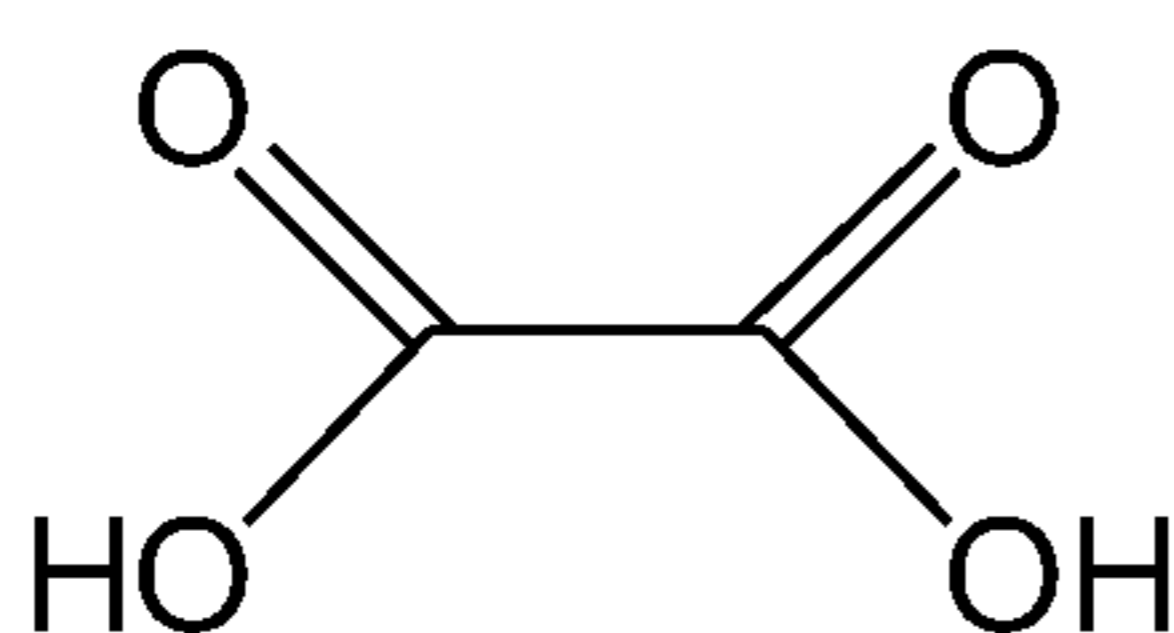
oxalic acid
