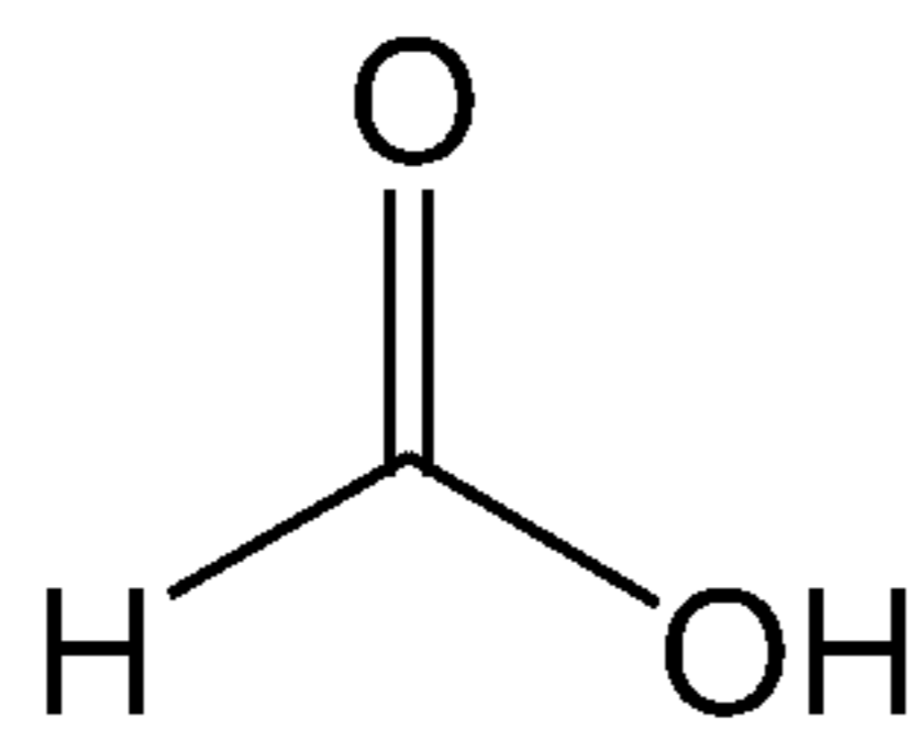
formic acid
