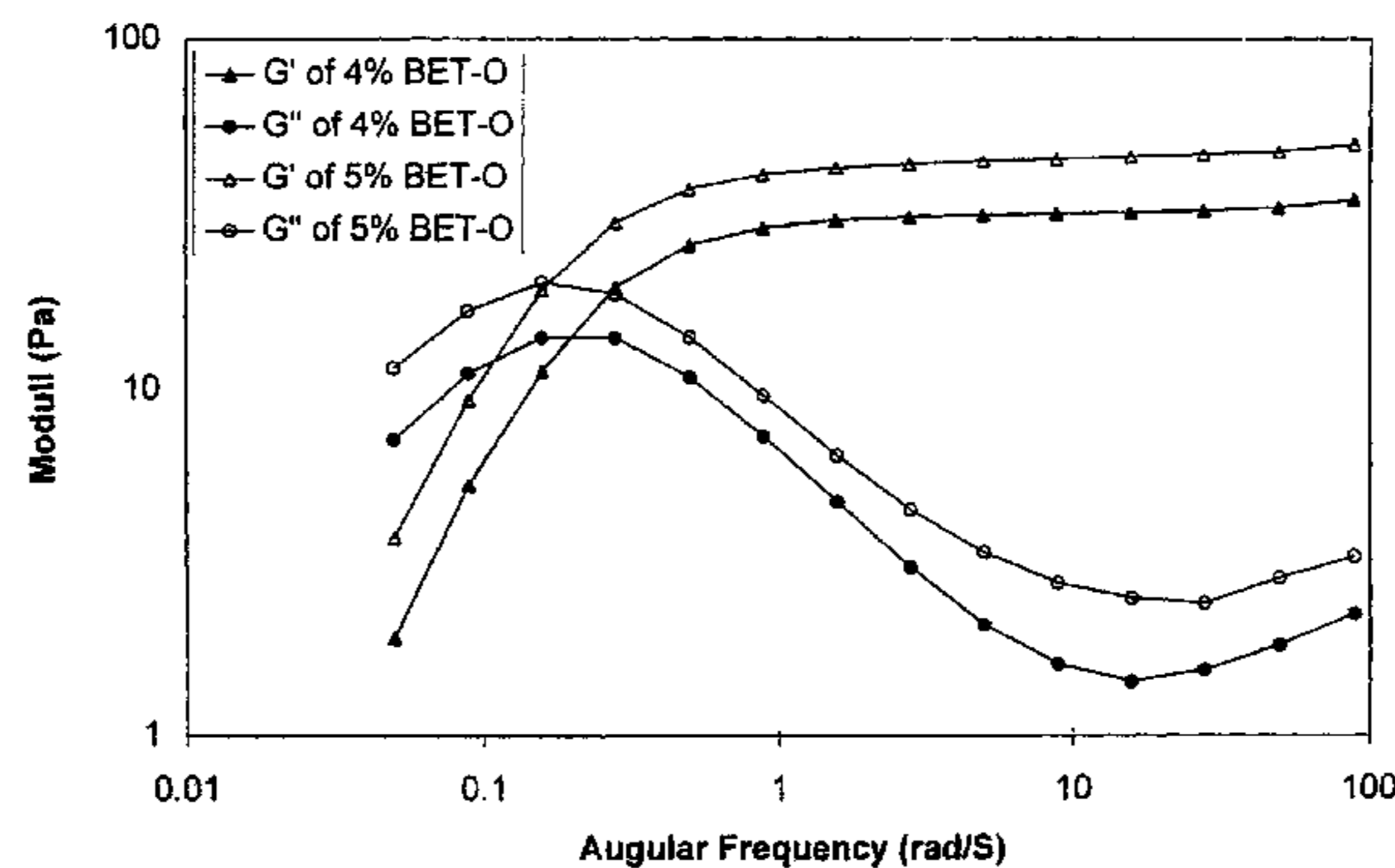
Dynamic shear moduli of different amount of oleamidopropyl betaine (BET-O) in presence of 3% KCl and 0.5% phthalic acid at 25 C.
