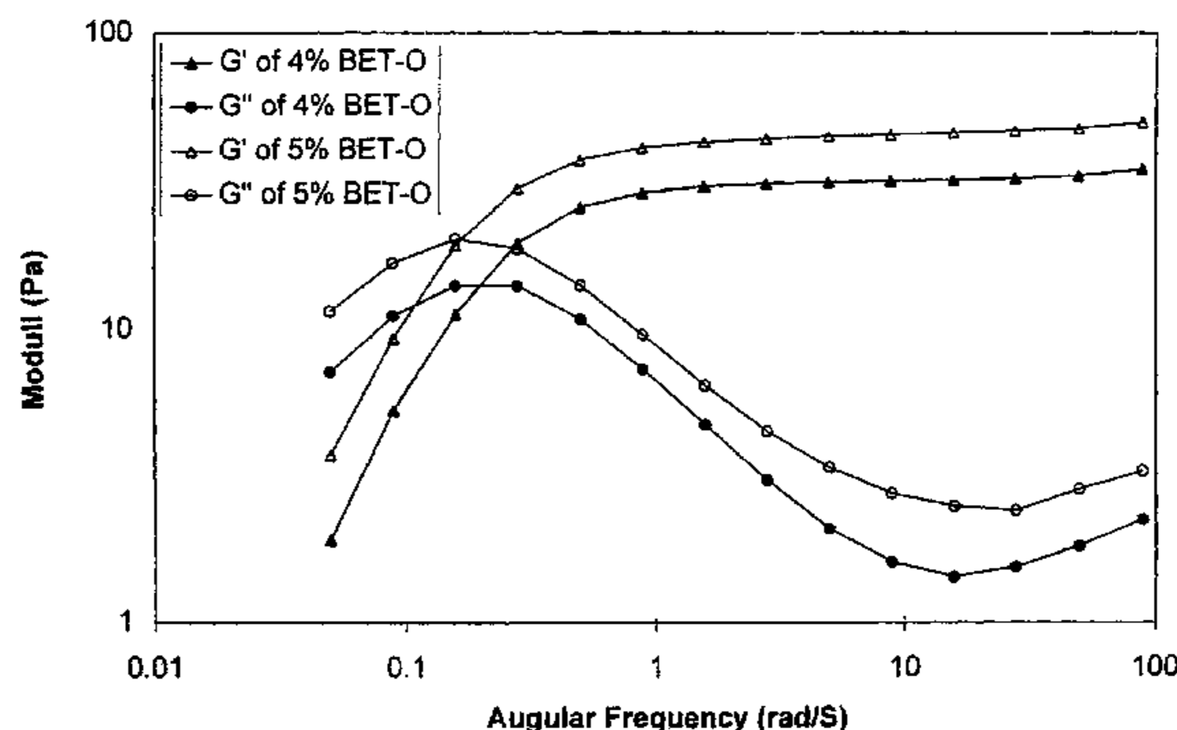
Dynamic shear moduli of different amount of oleamidopropyl betaine (BET-O) in presence of 3% KCl and 0.5% phthalic acid at 25 C.
