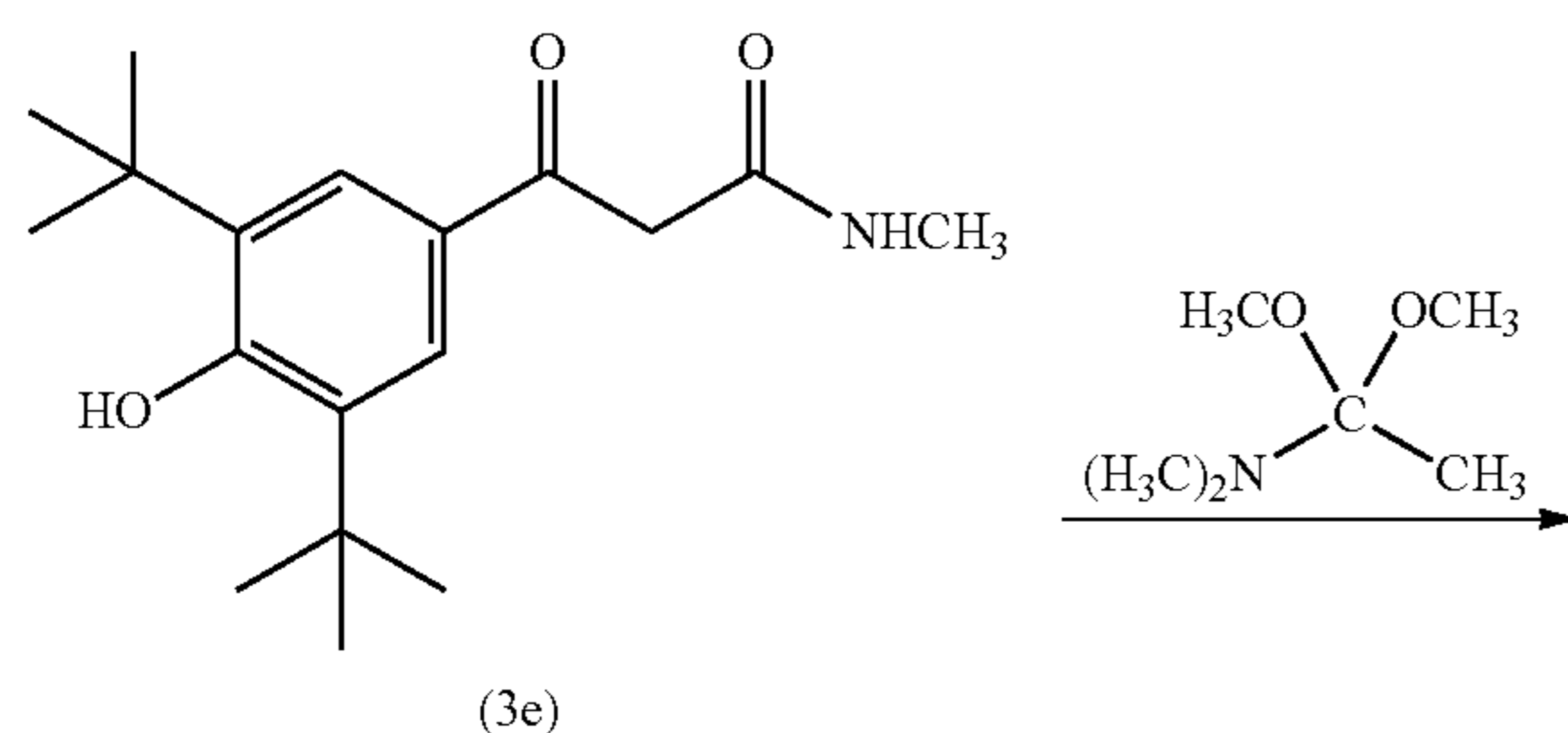
Reaction Scheme II
