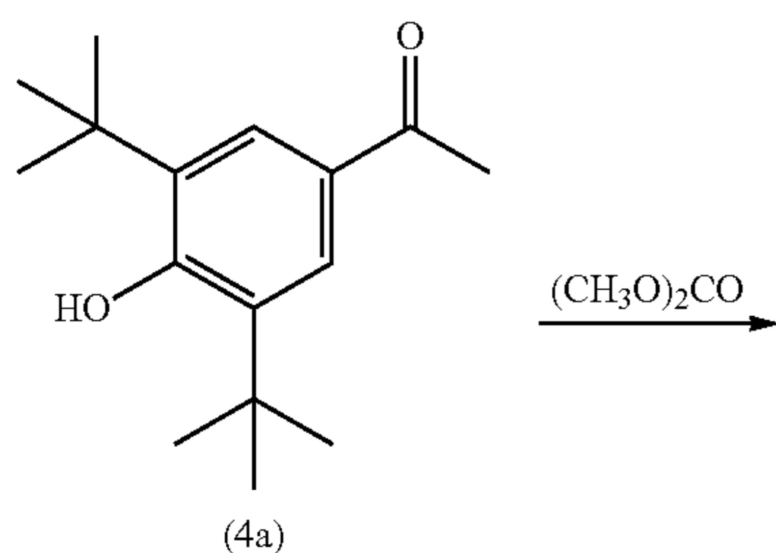
Reaction Scheme I
