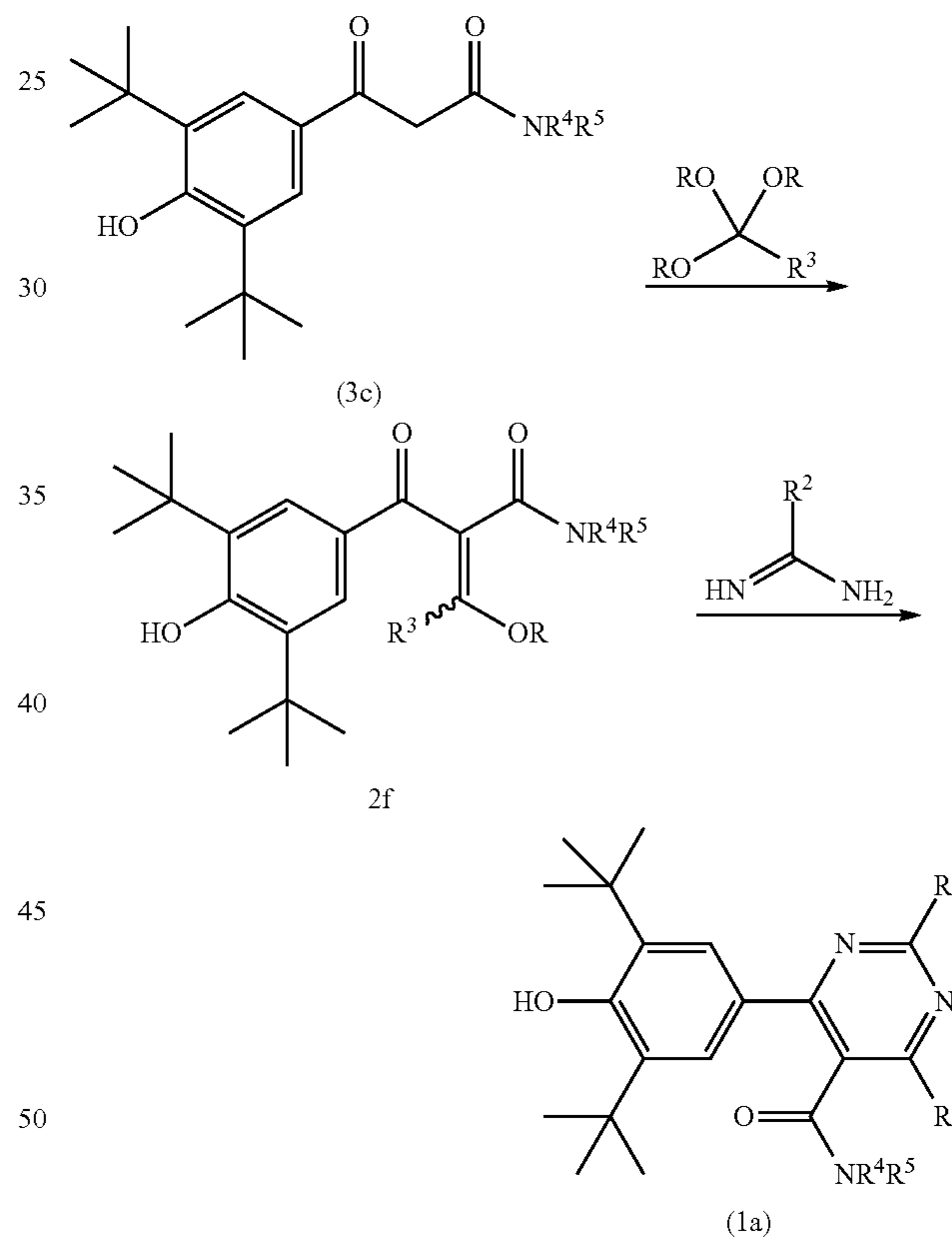
Reaction Scheme VI
