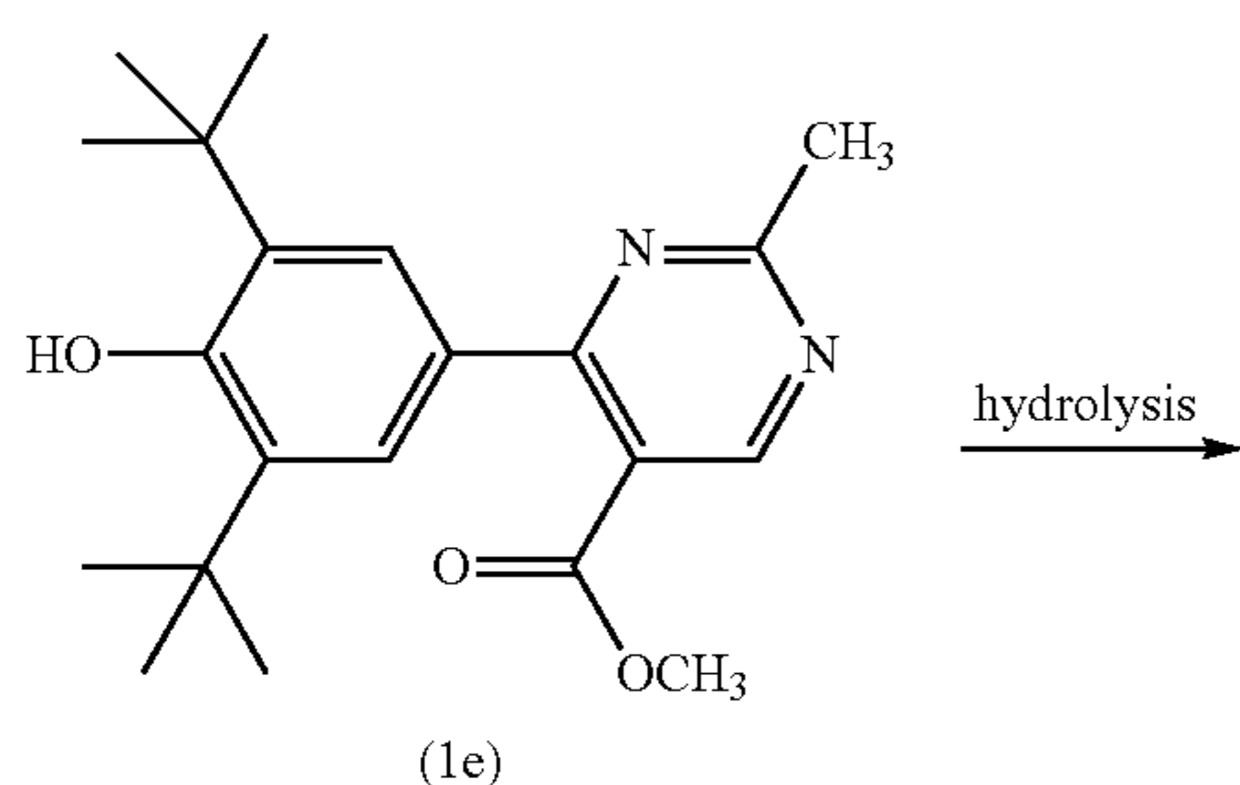
Reaction Scheme IV
