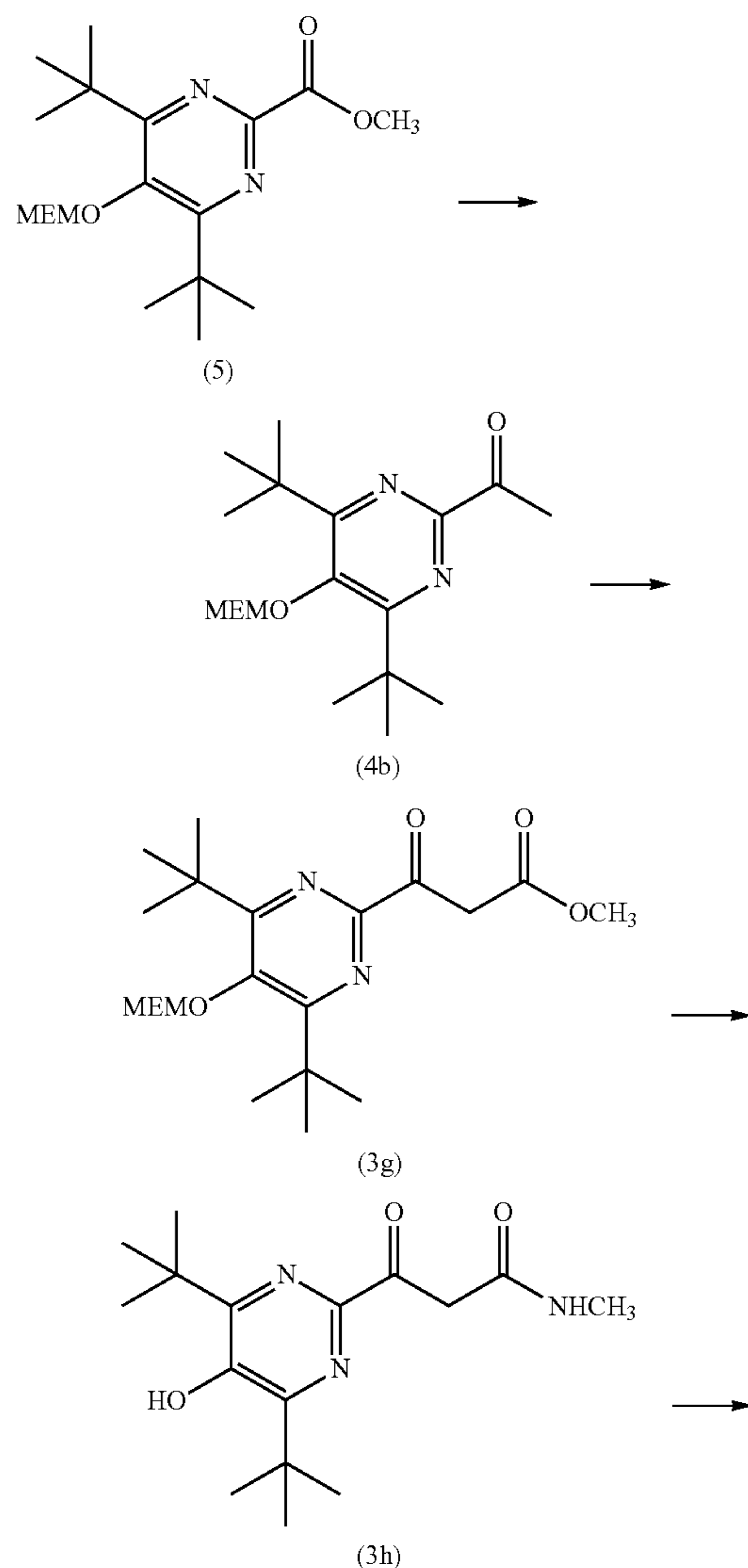
Reaction Scheme VII
