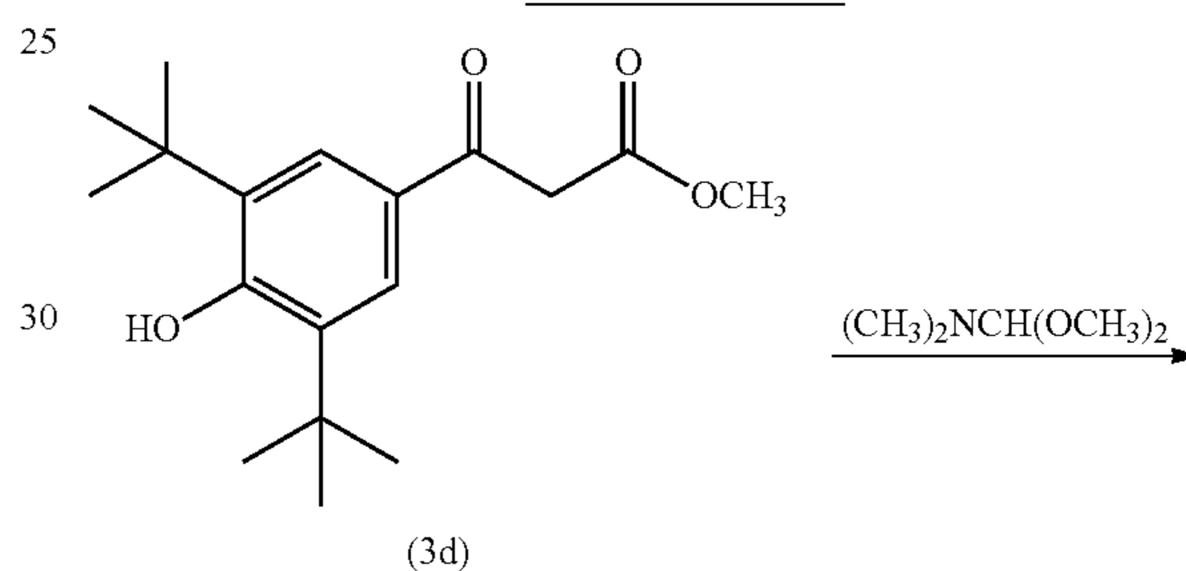
Reaction Scheme III
