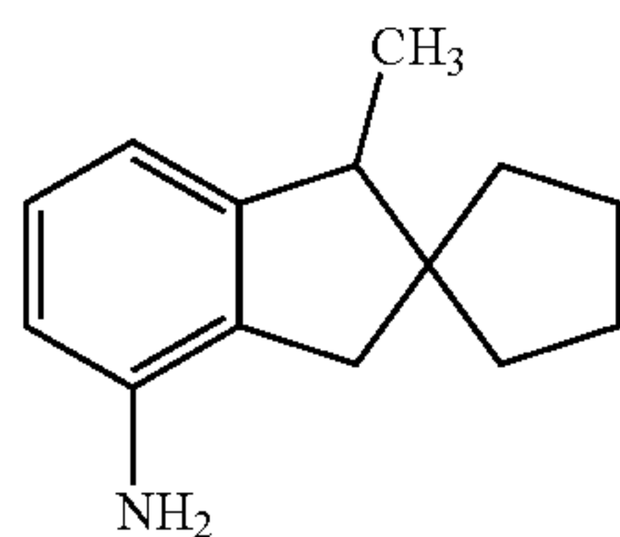
1'-methyl-1',3'-dihydrospiro[cyclopentane-1,2'-inden]-4'-amine
