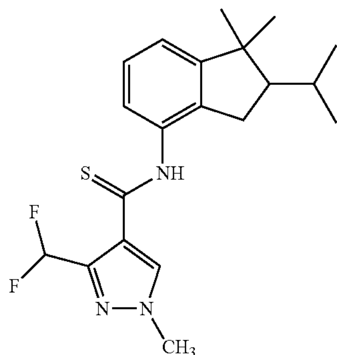
3-(difluoromethyl)-N-(2-isopropyl-1,1-dimethyl-2,3-dihydro-1H-inden-4-yl)-1-methyl-1H-pyrazole-4-carbothioamide
