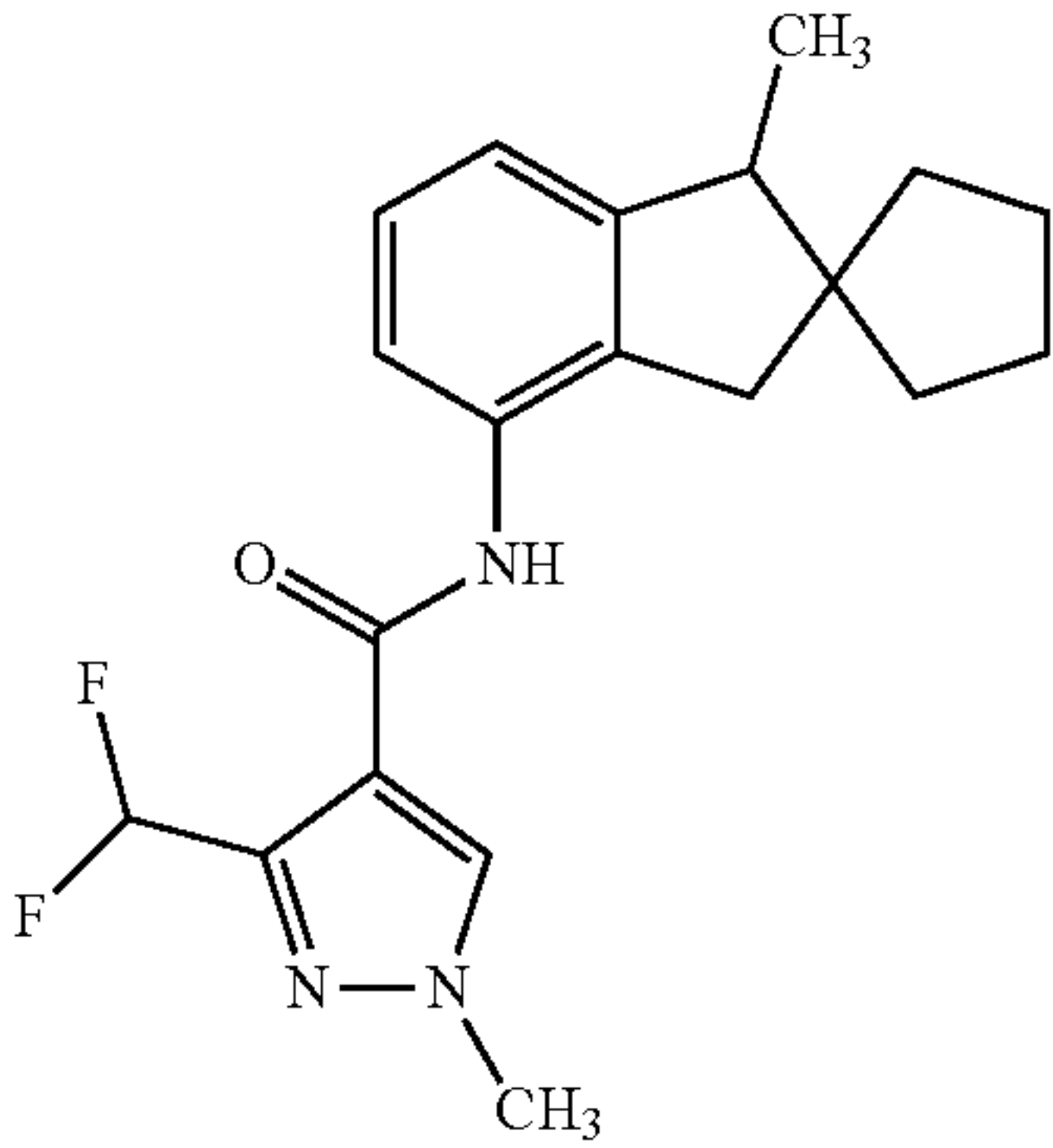
3-(difluoromethyl)-1-methyl-N-(1'-methyl-1',3'-dihydrospiro[cyclopentane-1,2'-inden]-4'-yl)-1H-pyrazole-4-carboxamide
