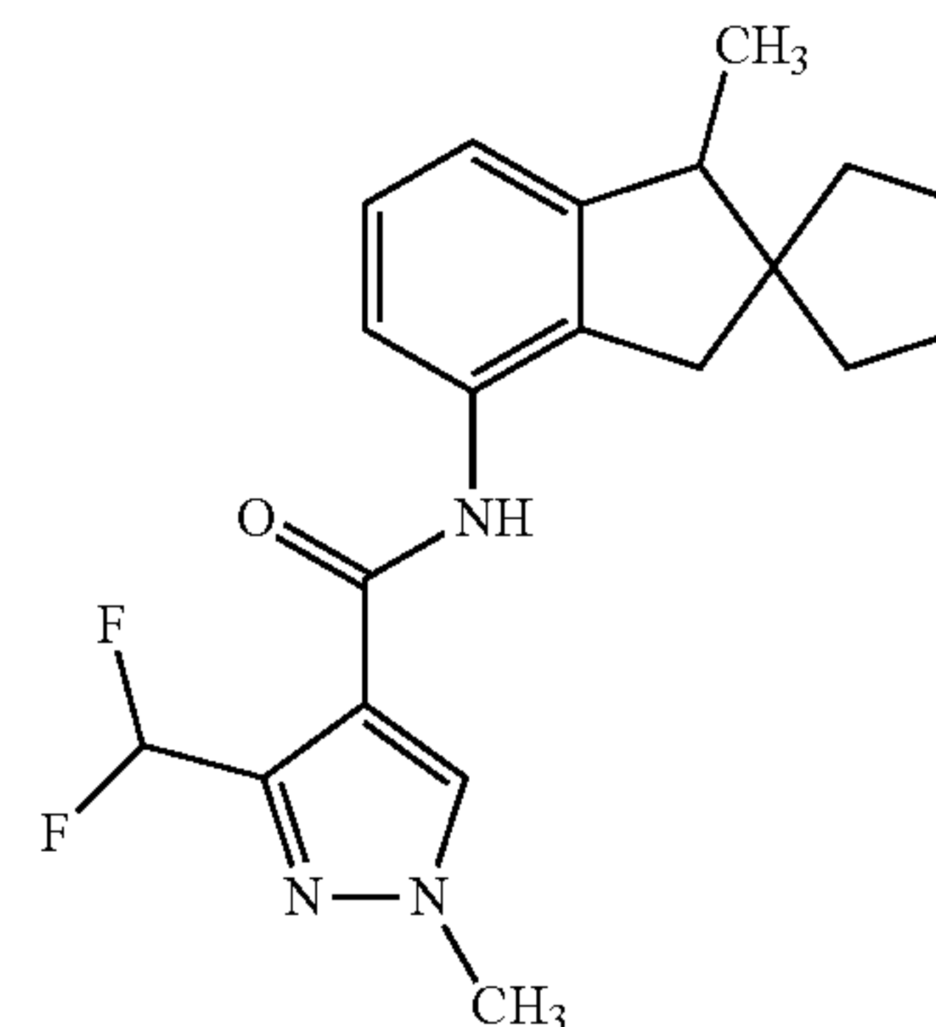
3-(difluoromethyl)-1-methyl-N-(1'-methyl-1',3'-dihydrospiro[cyclopentane-1,2'-inden]-4'-yl)-1H-pyrazole-4-carboxamide
