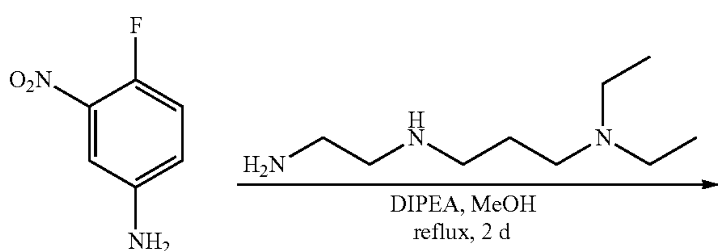
Scheme 7
