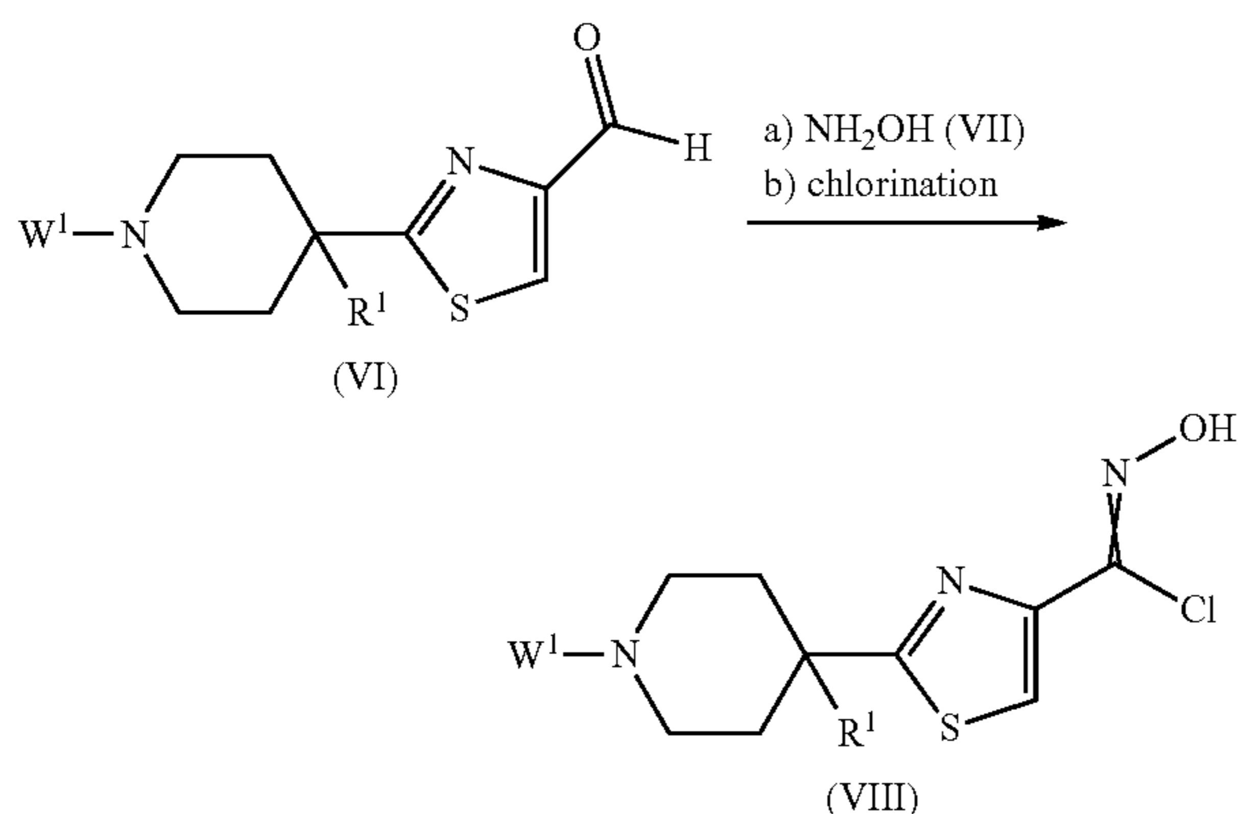
Scheme 4: Process D
