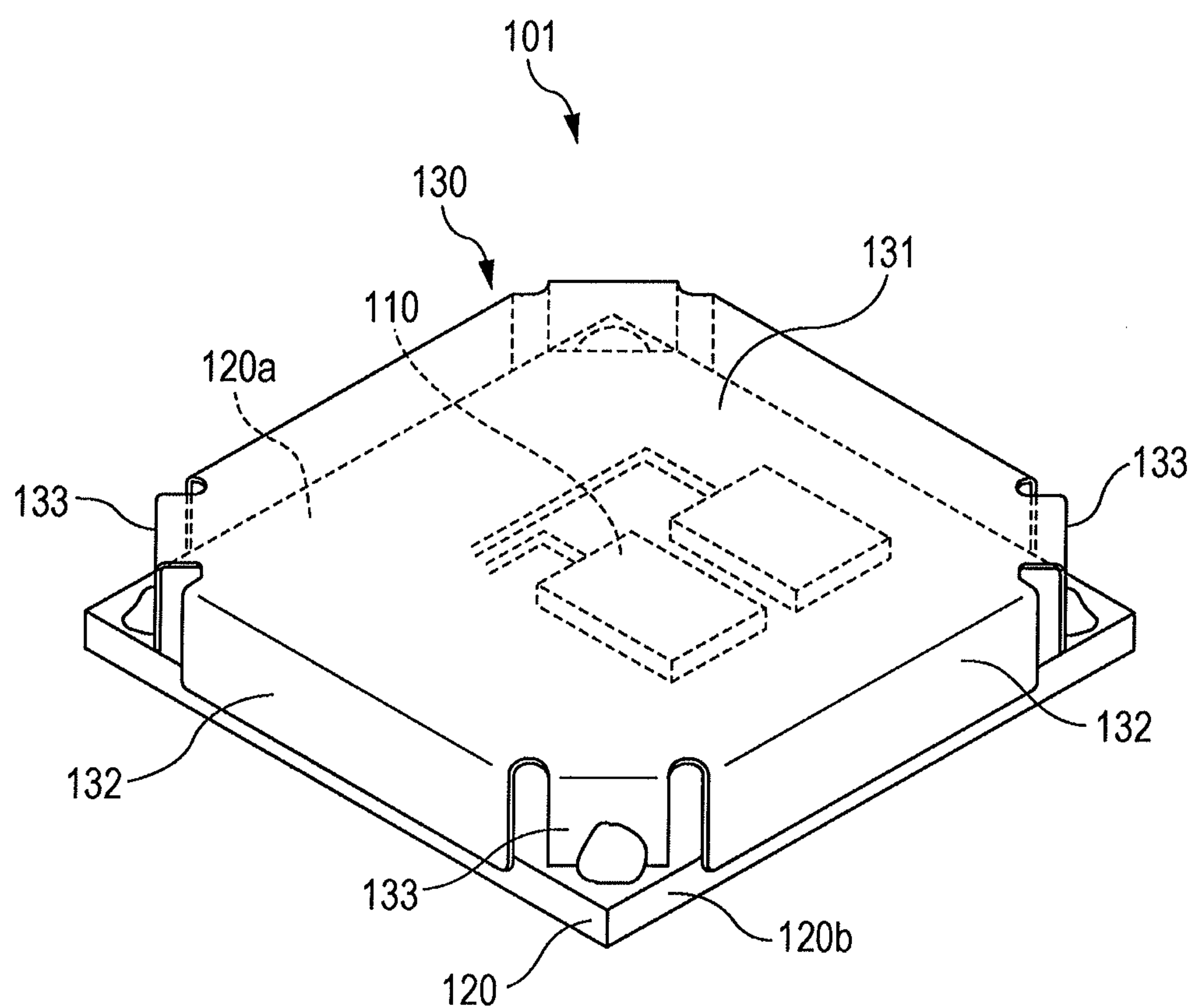
FIG. 9 PRIOR ART
