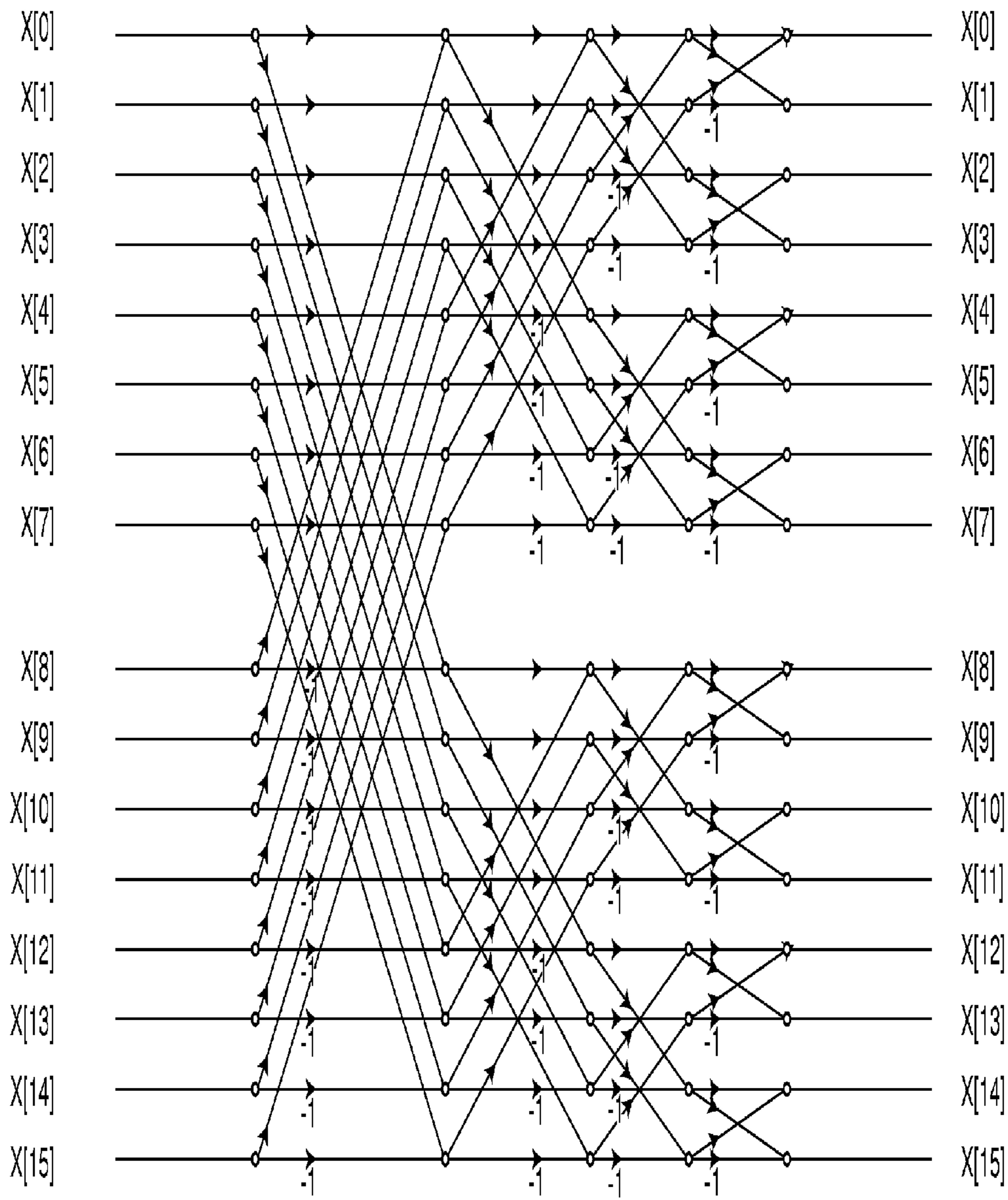
FAST HADAMARD TRANSFORM STRUCTURE
