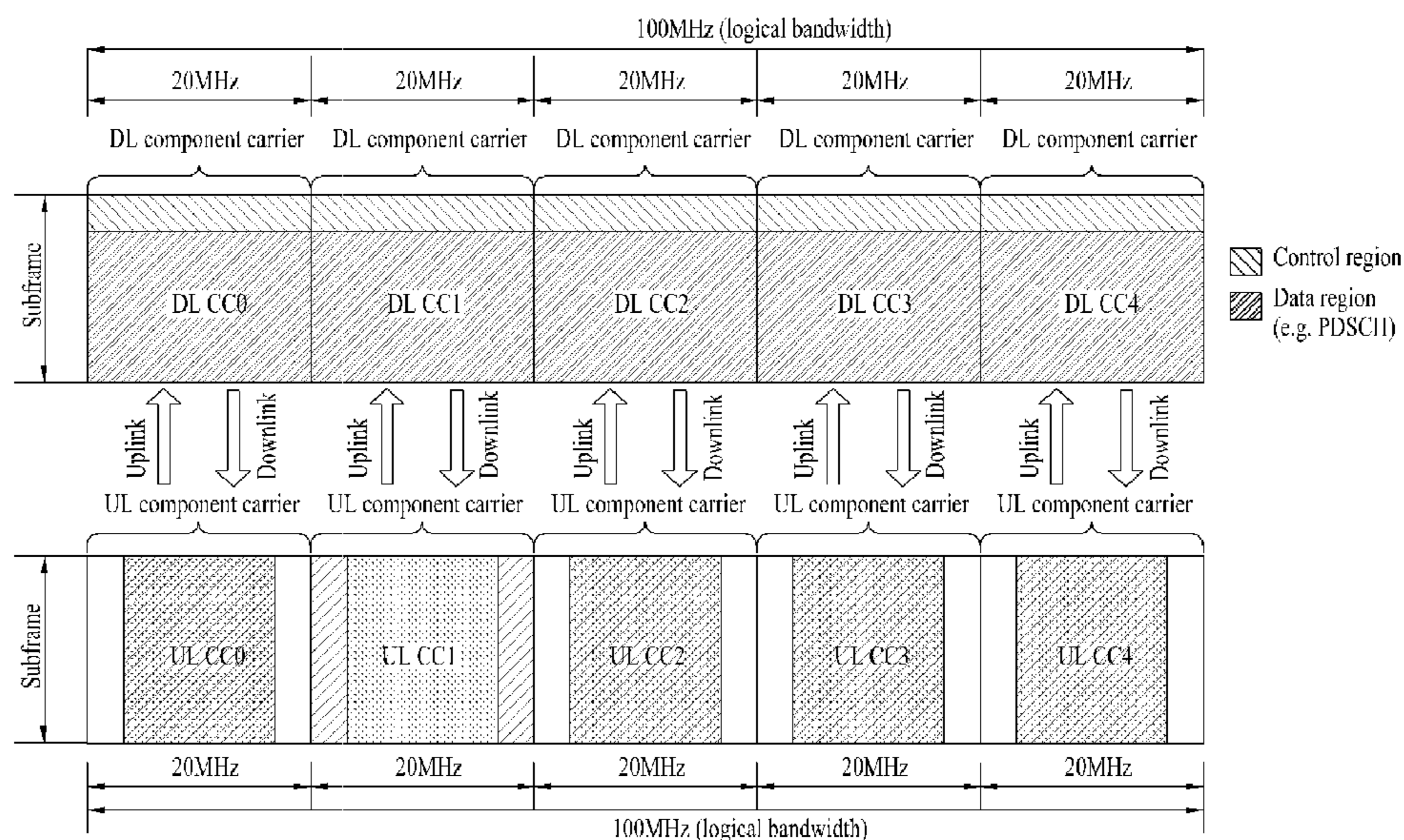
Multi component carriers (e.g. LTE-A system)
