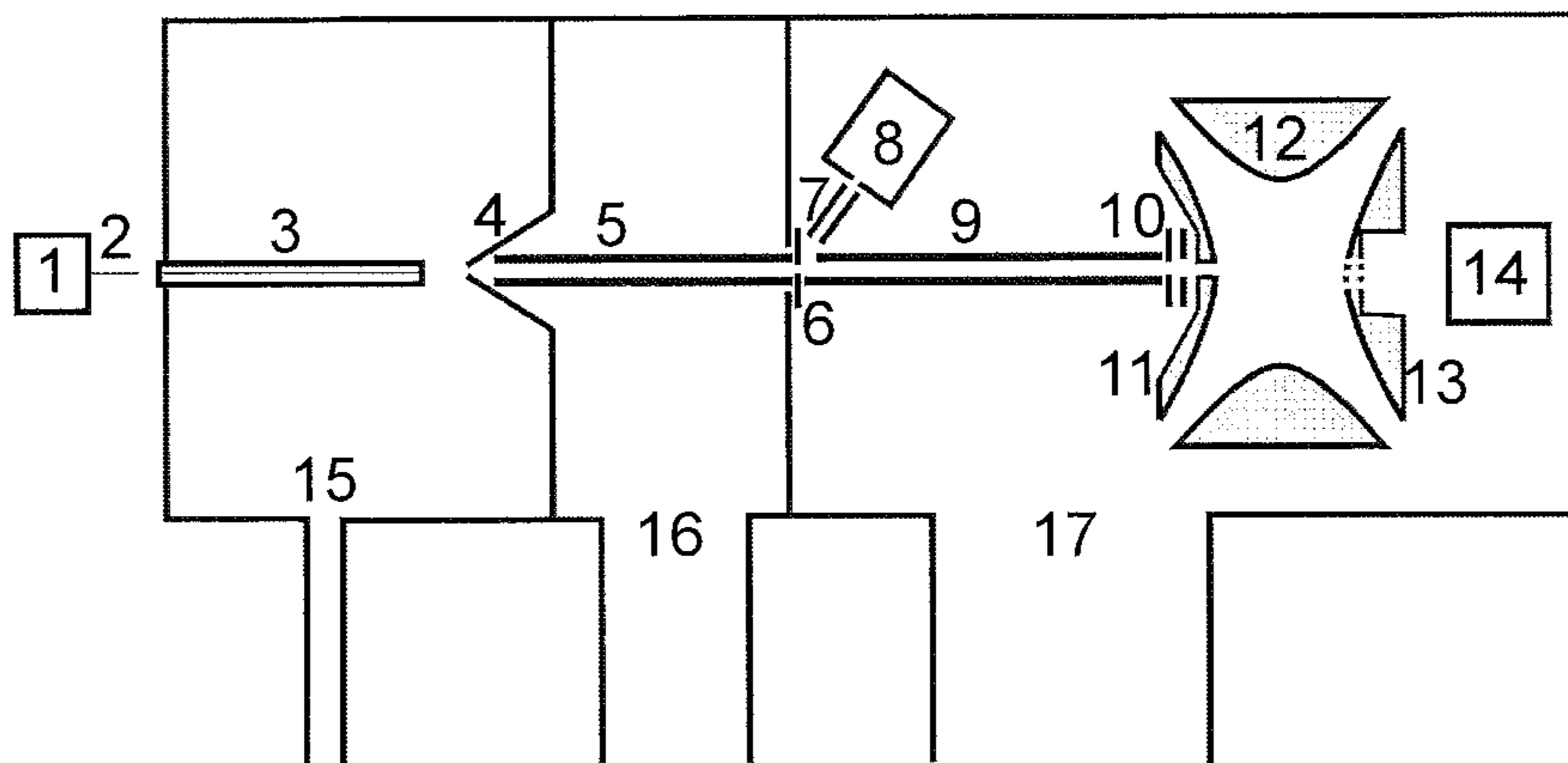
Figure 2 (Prior Art)
