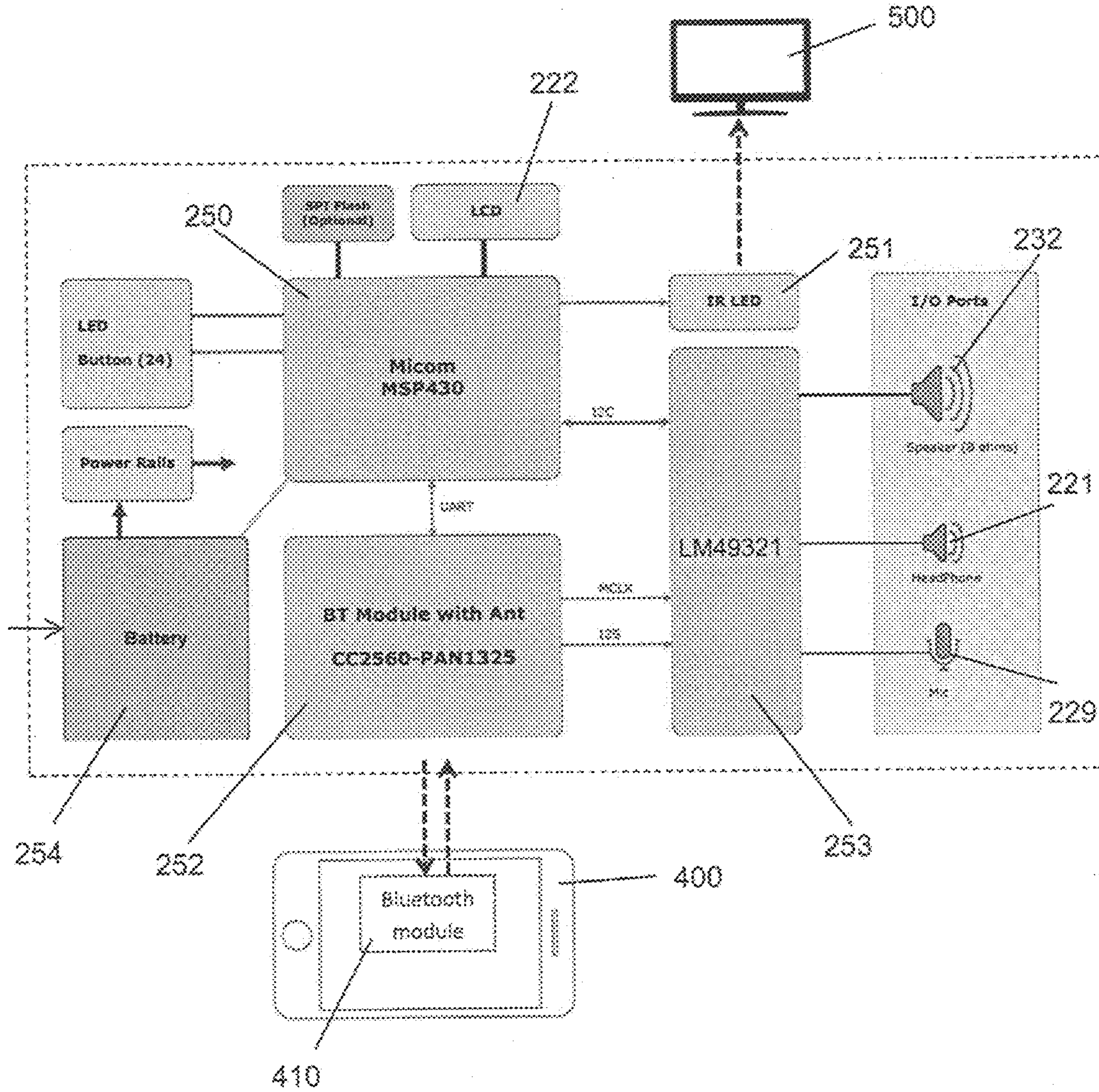
Block Diagram - I: Remote Controller
