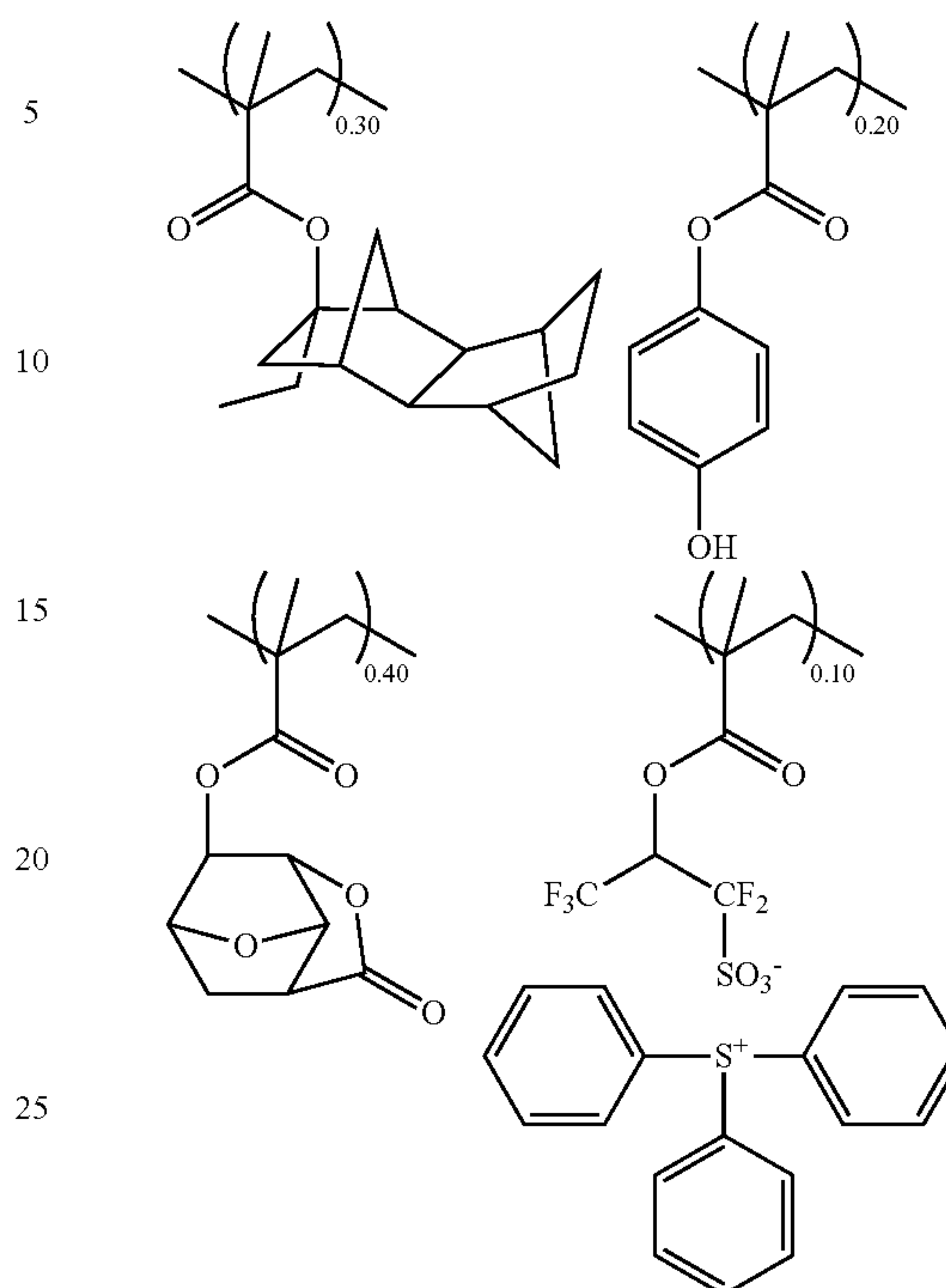
Comparative Polymer 4
