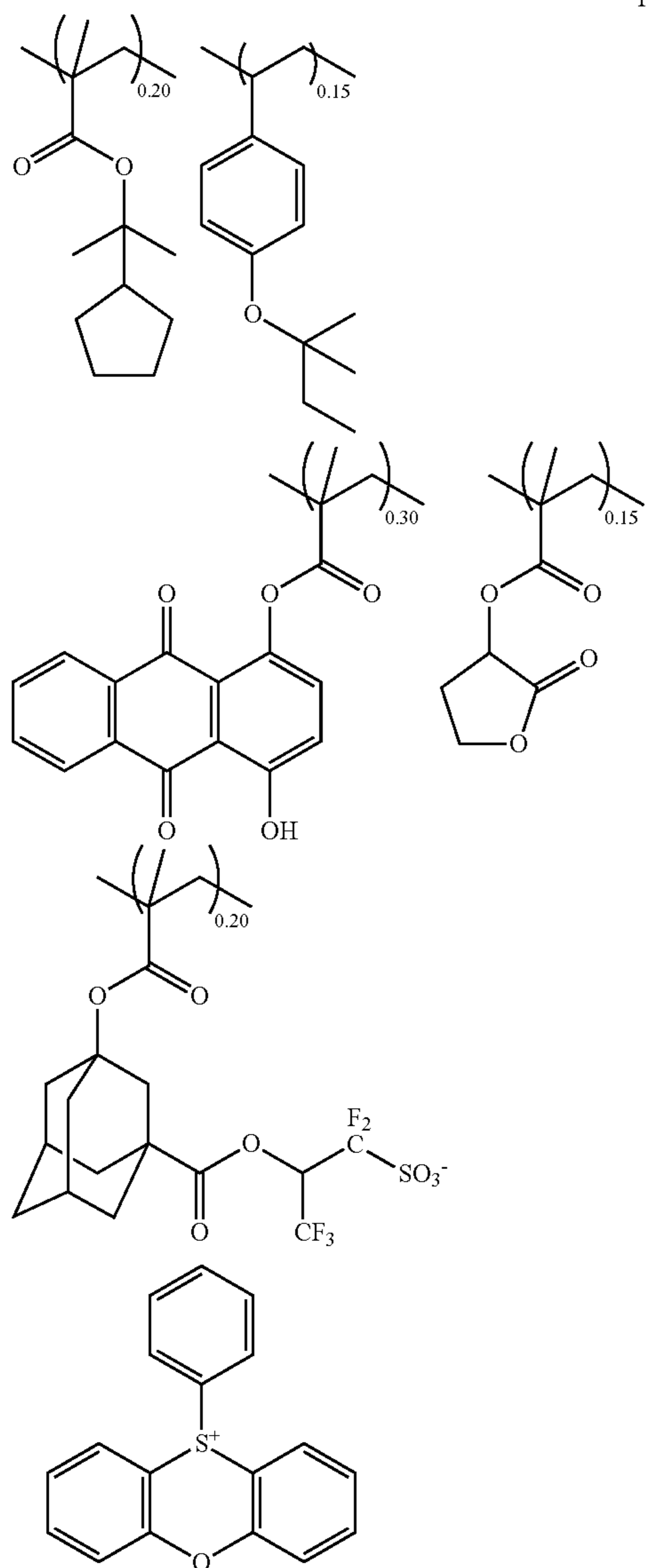
Synthesis Example 8
