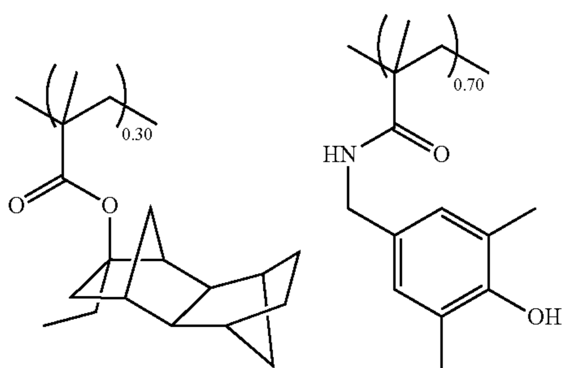
Comparative Polymer 3
