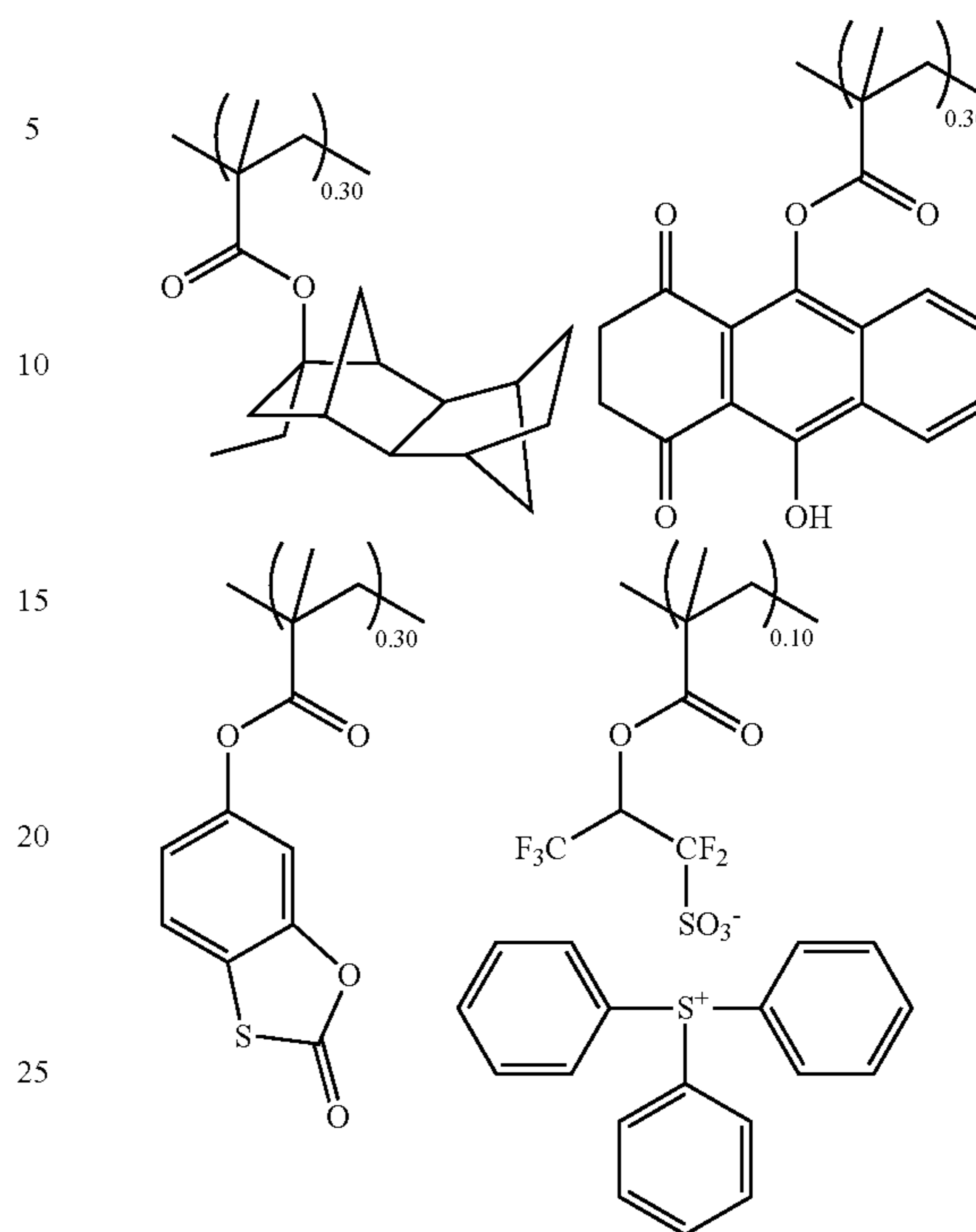
Synthesis Example 5
