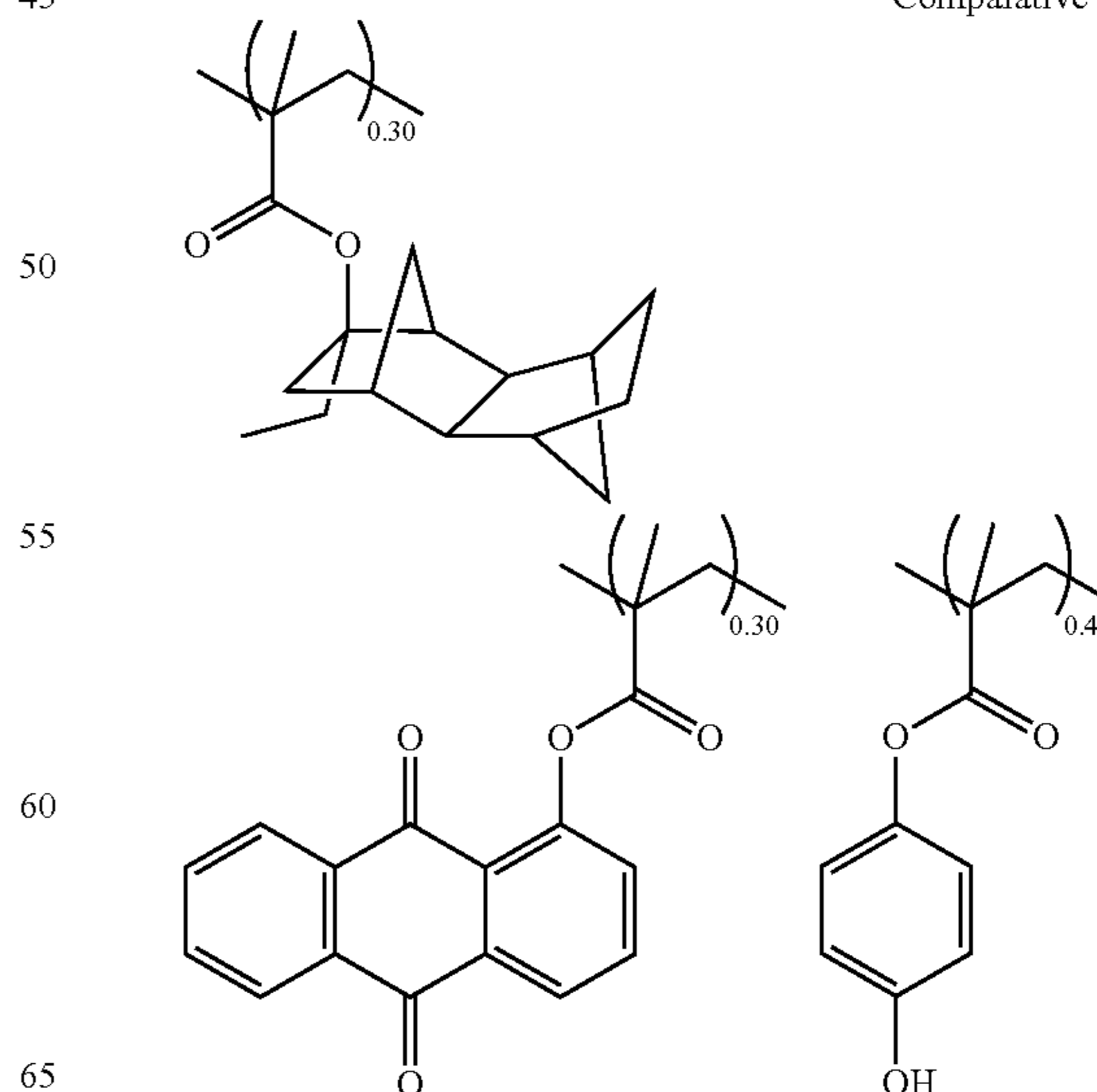
Comparative Polymer 5
