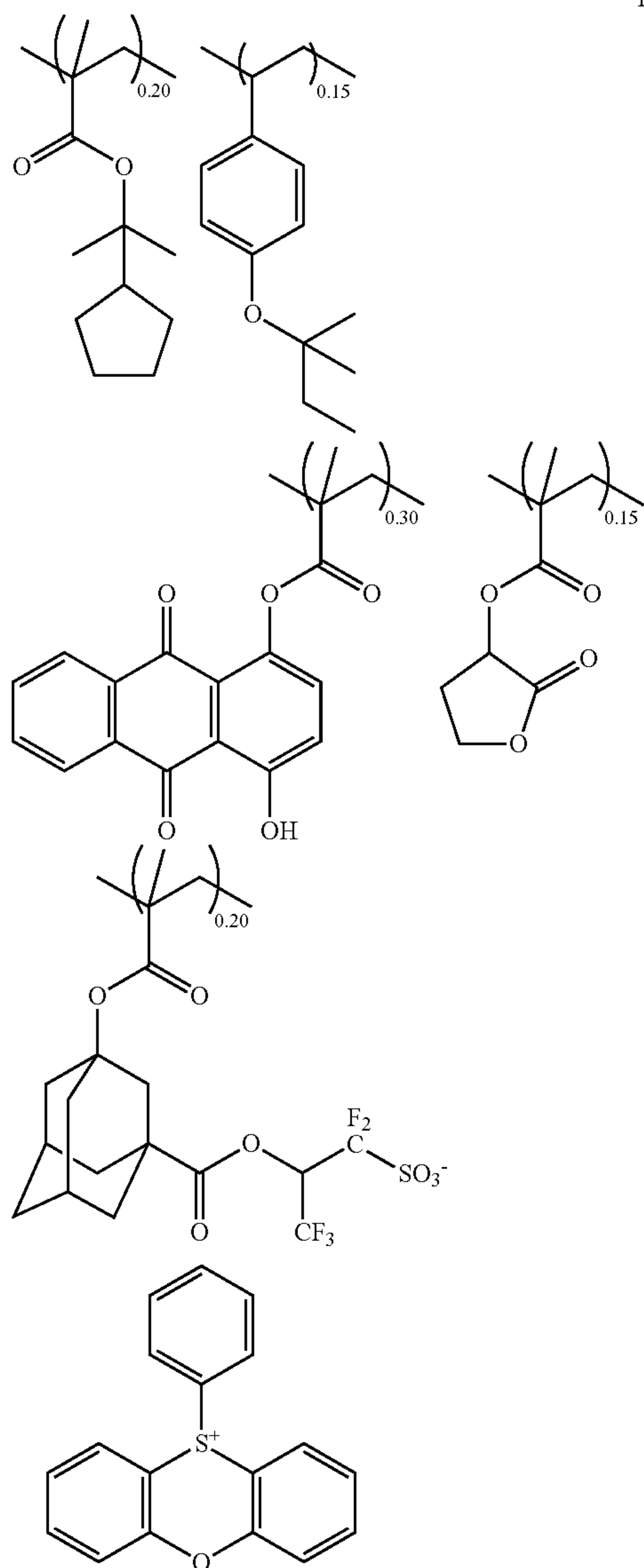
Synthesis Example 8
