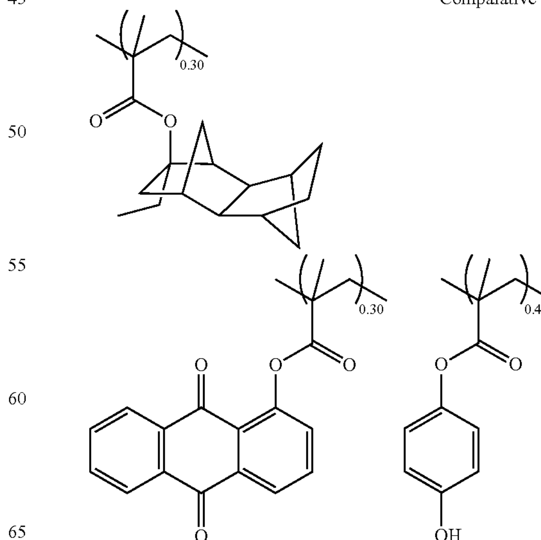
Comparative Polymer 5
