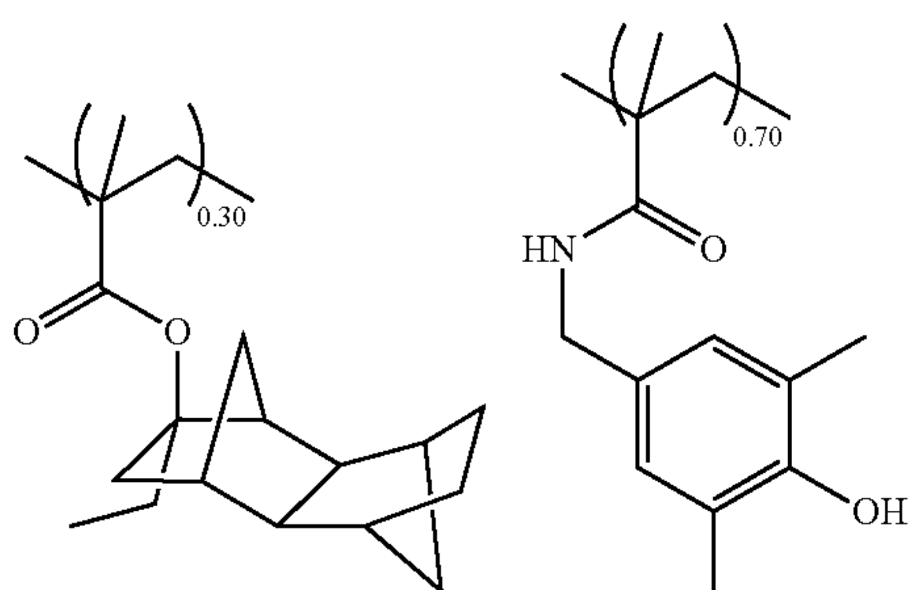
Comparative Polymer 3
