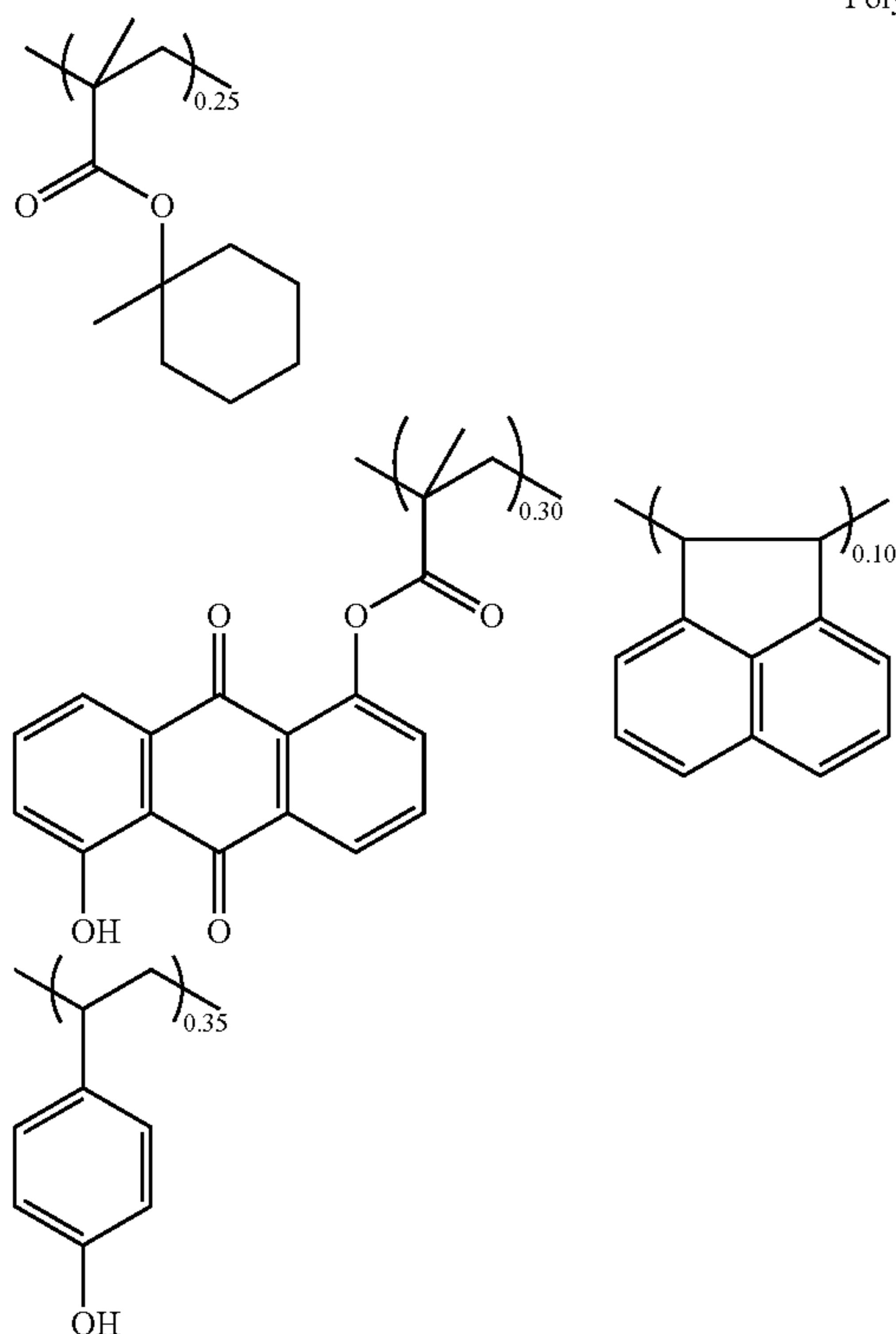
Synthesis Example 4
