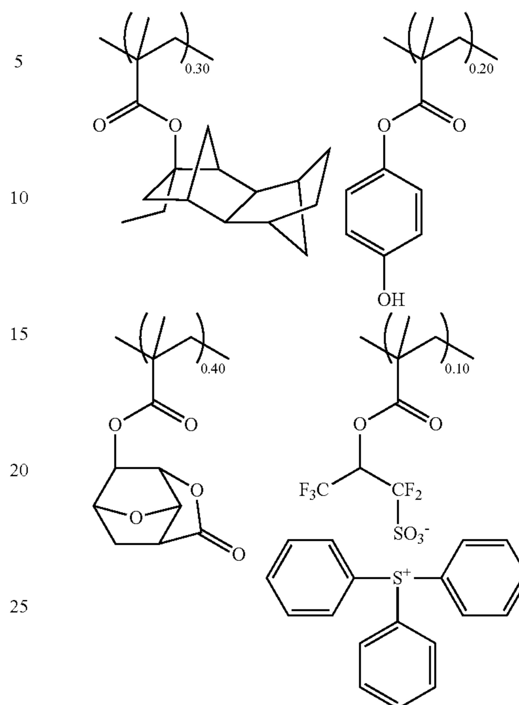
Comparative Polymer 4
