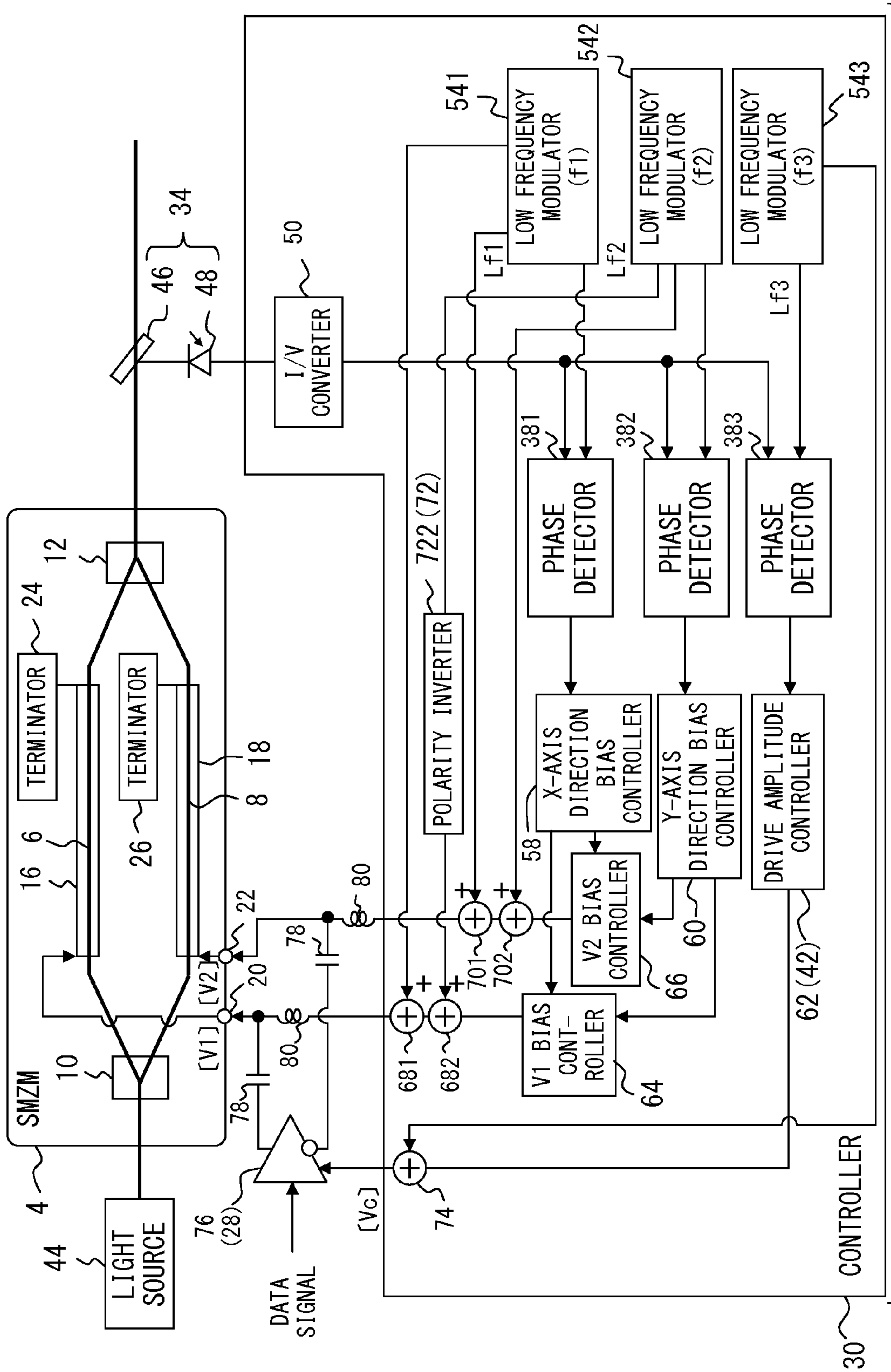
200C OPTICAL TRANSMISSION MODULE
