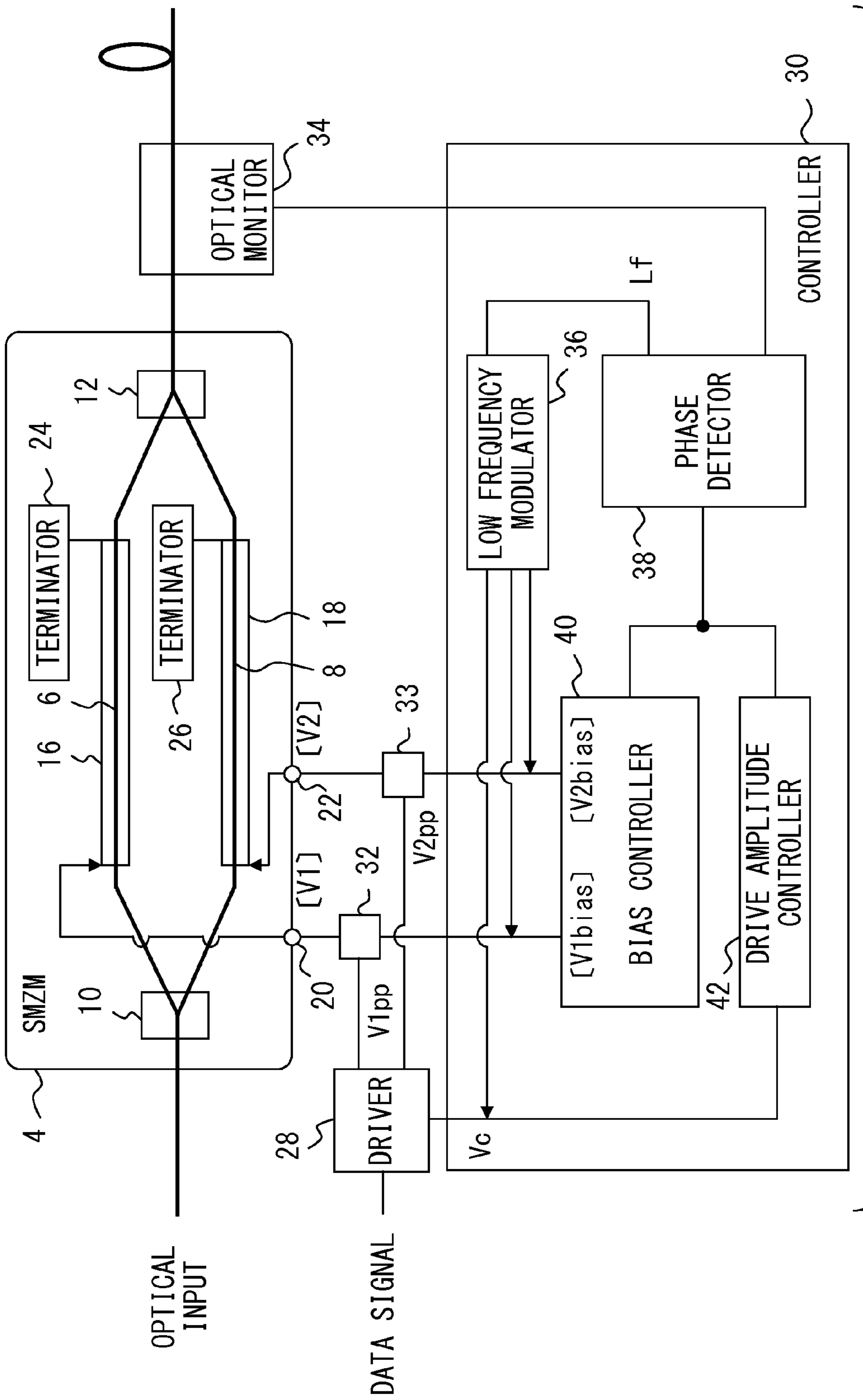
2 OPTICAL MODULATOR
