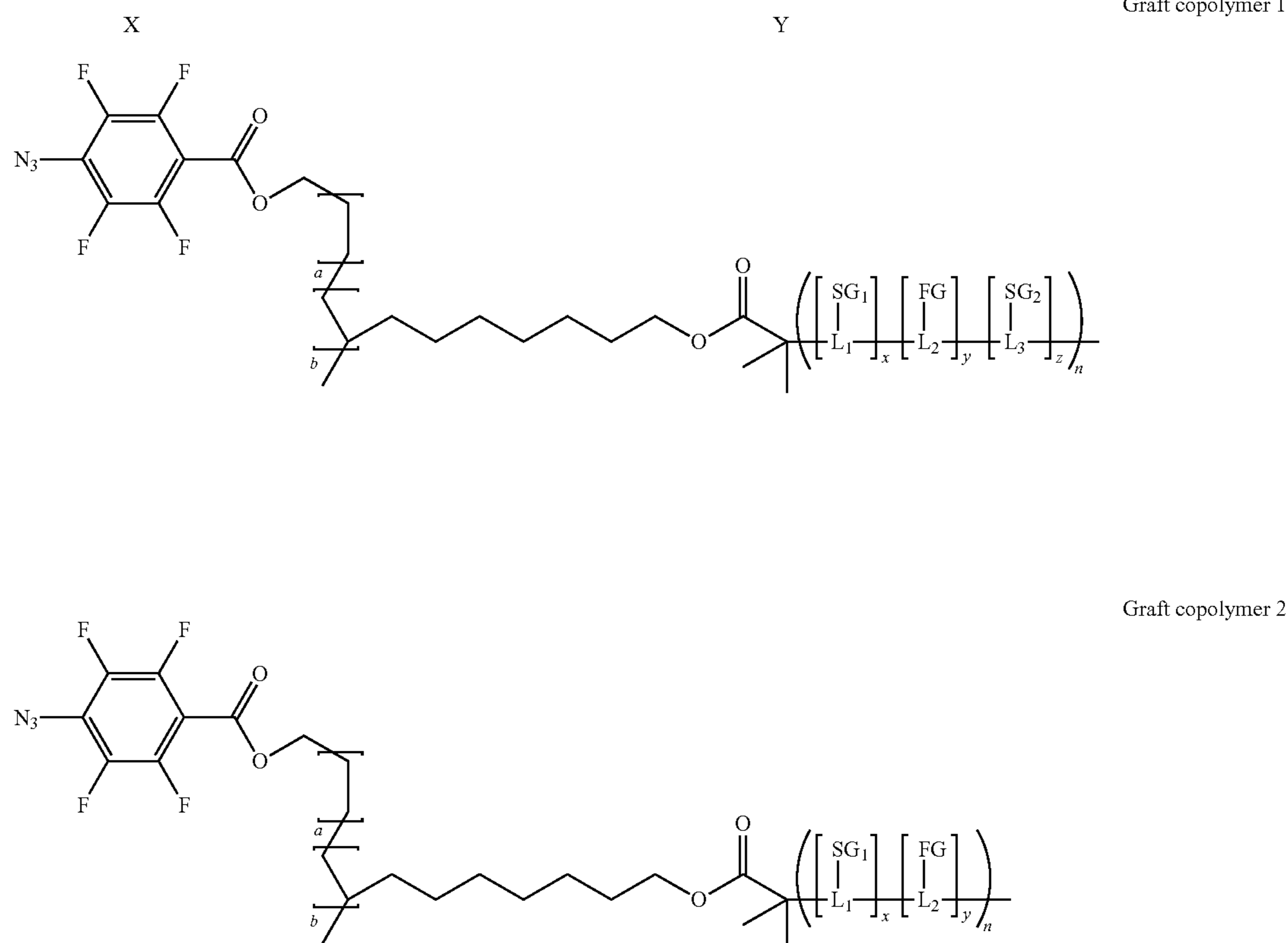
Scheme 1
