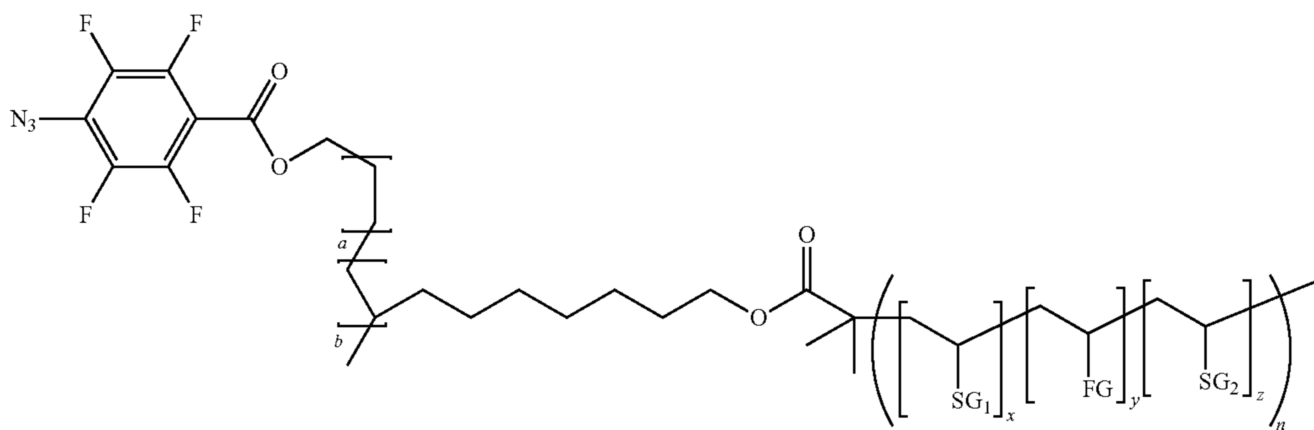
Scheme 2
