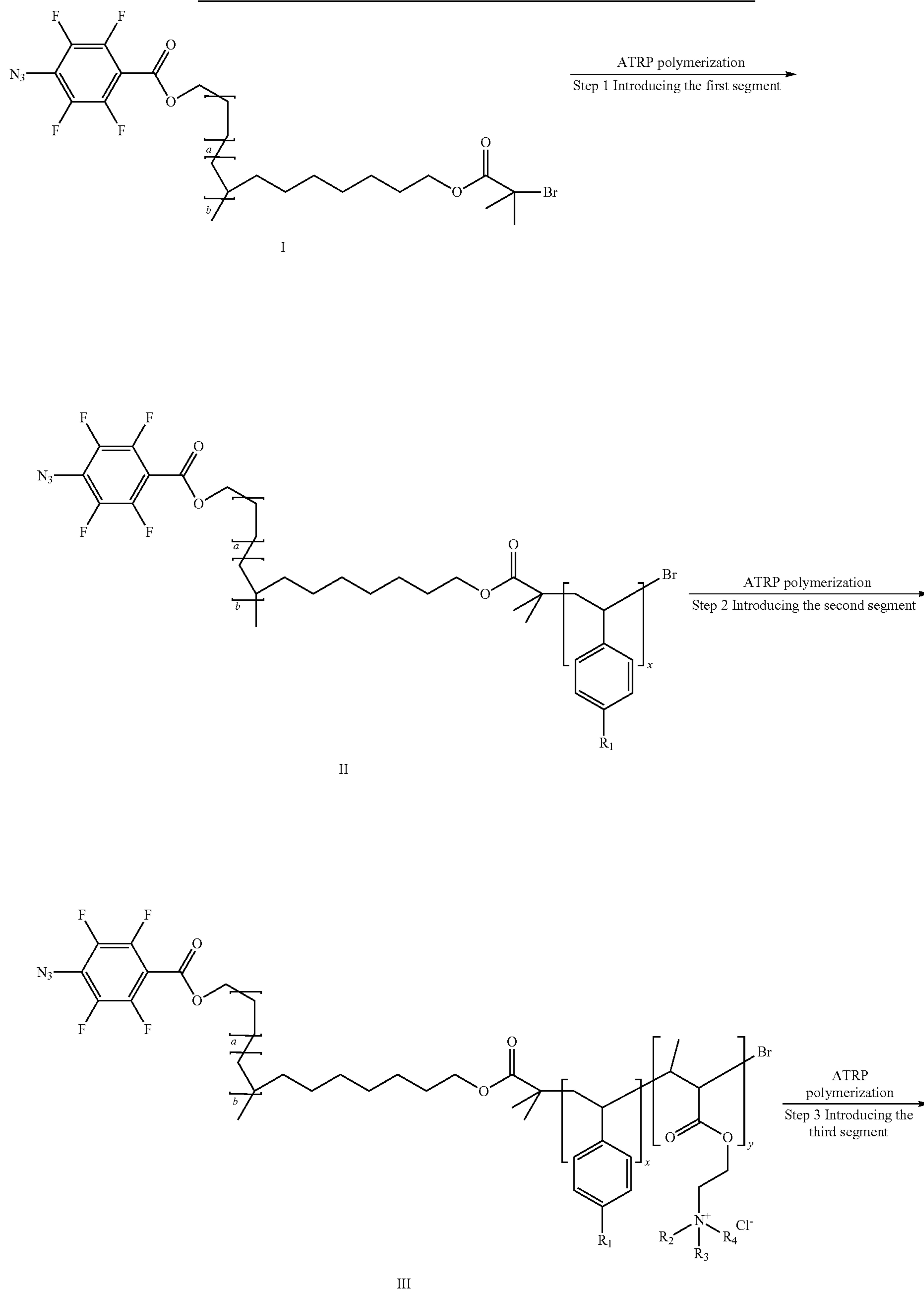
Scheme 8
