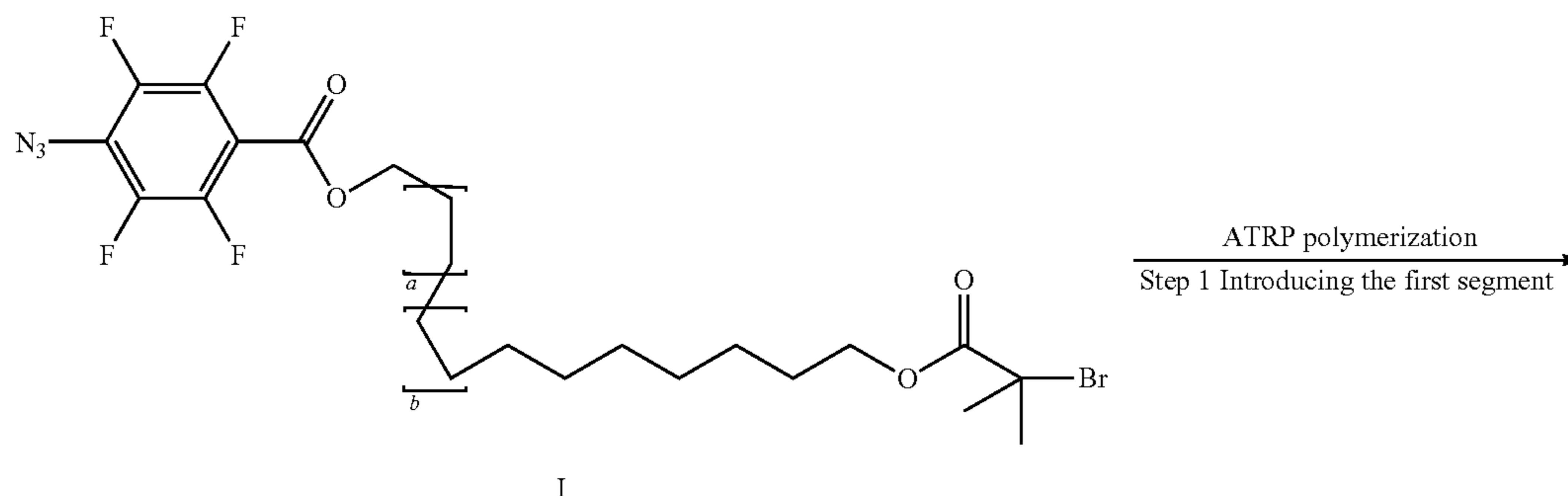
Scheme 7
