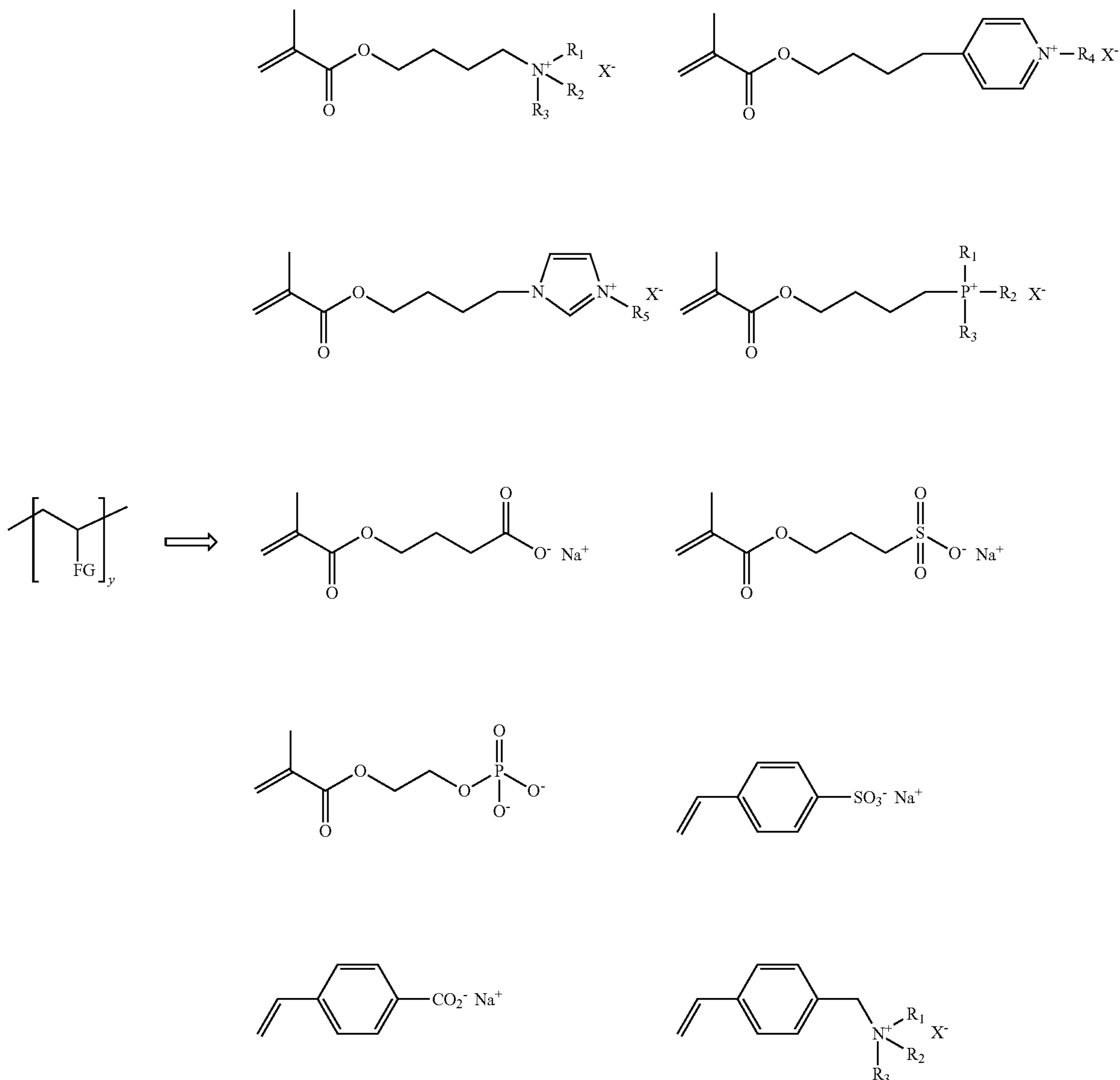
Scheme 4
