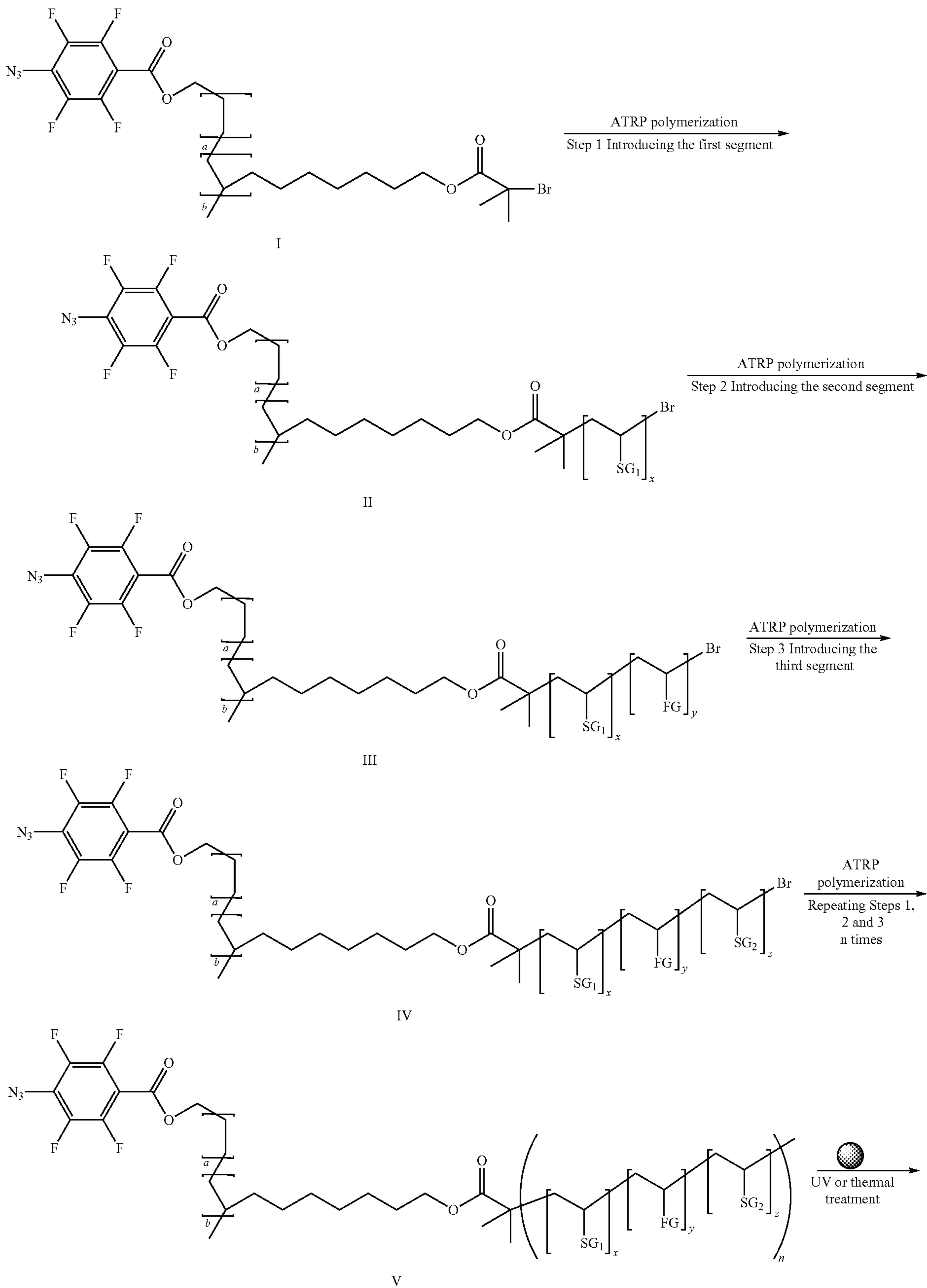
Scheme 6
