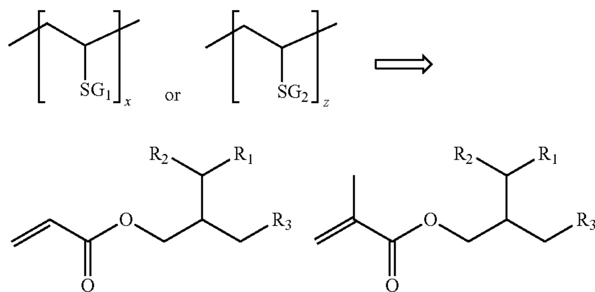
Scheme 3
