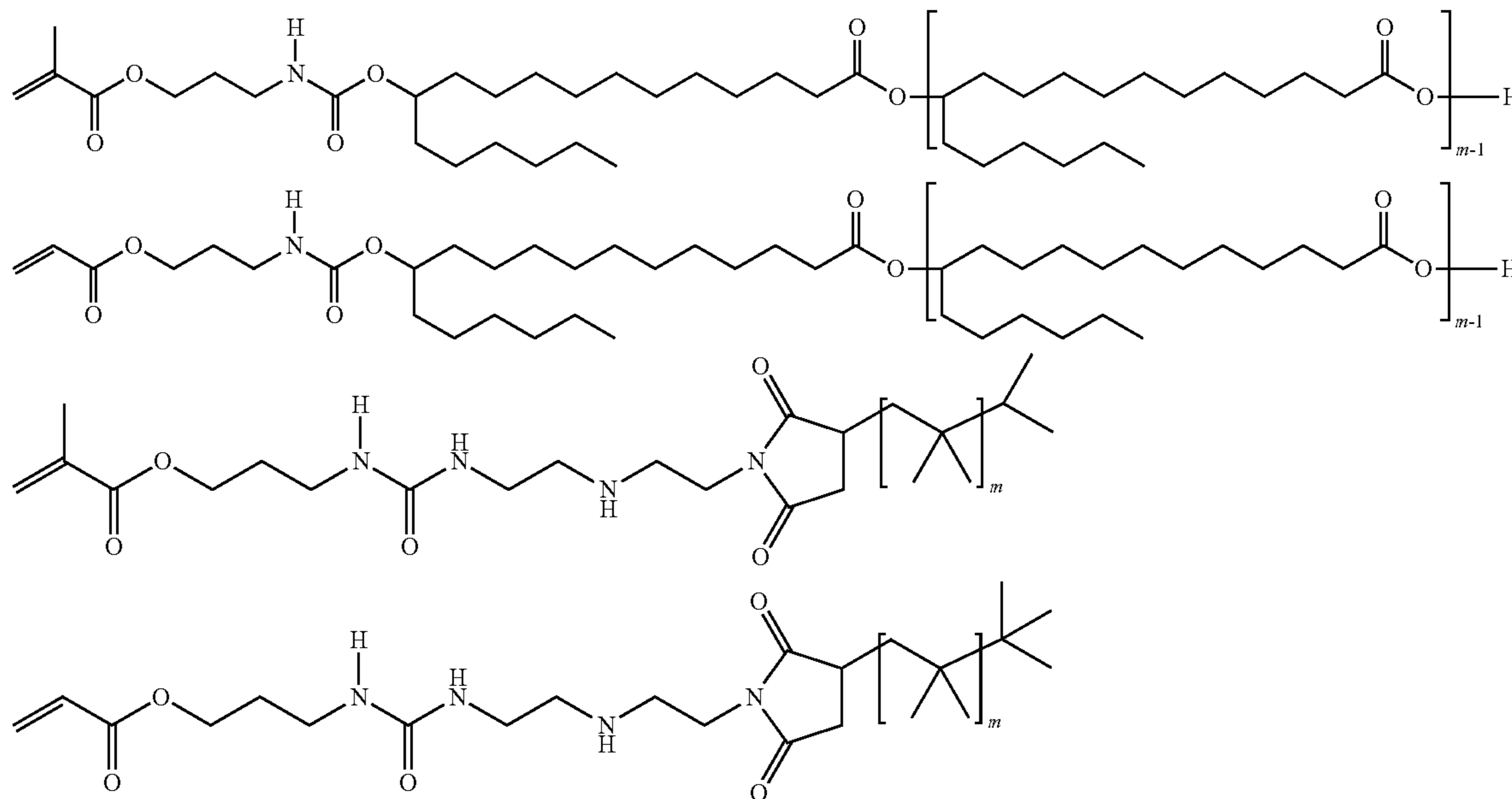
Scheme 3A
