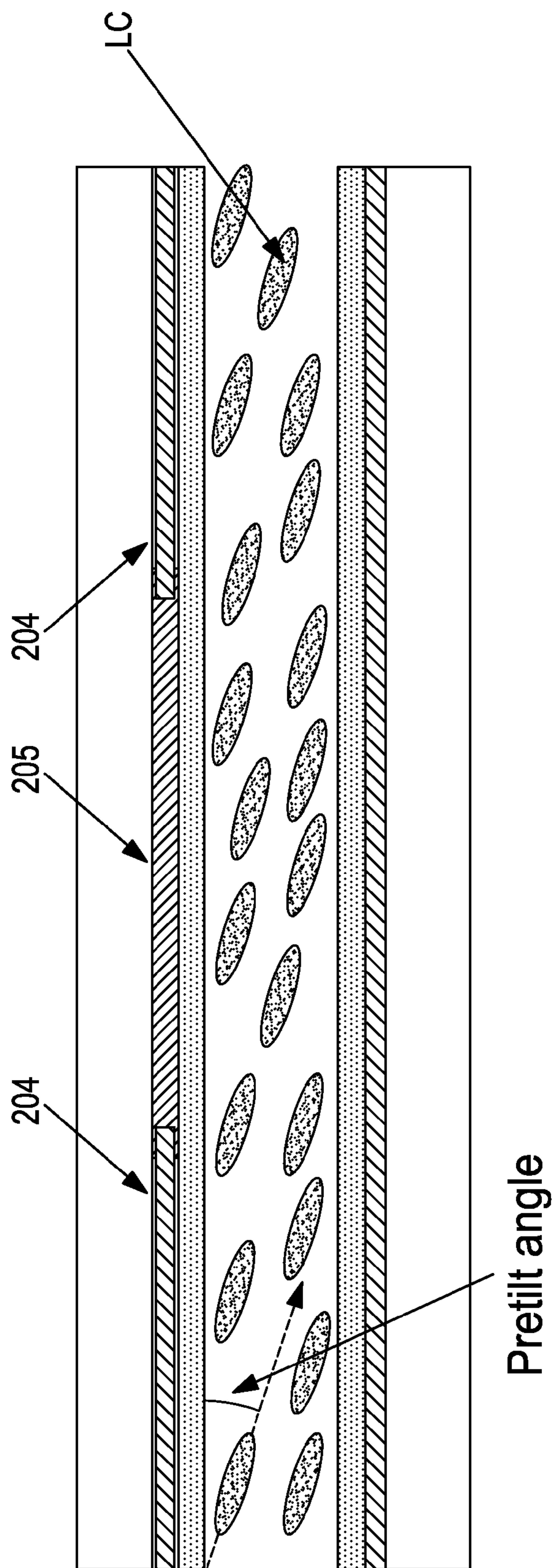
FIGURE 2 (PRIOR ART)
