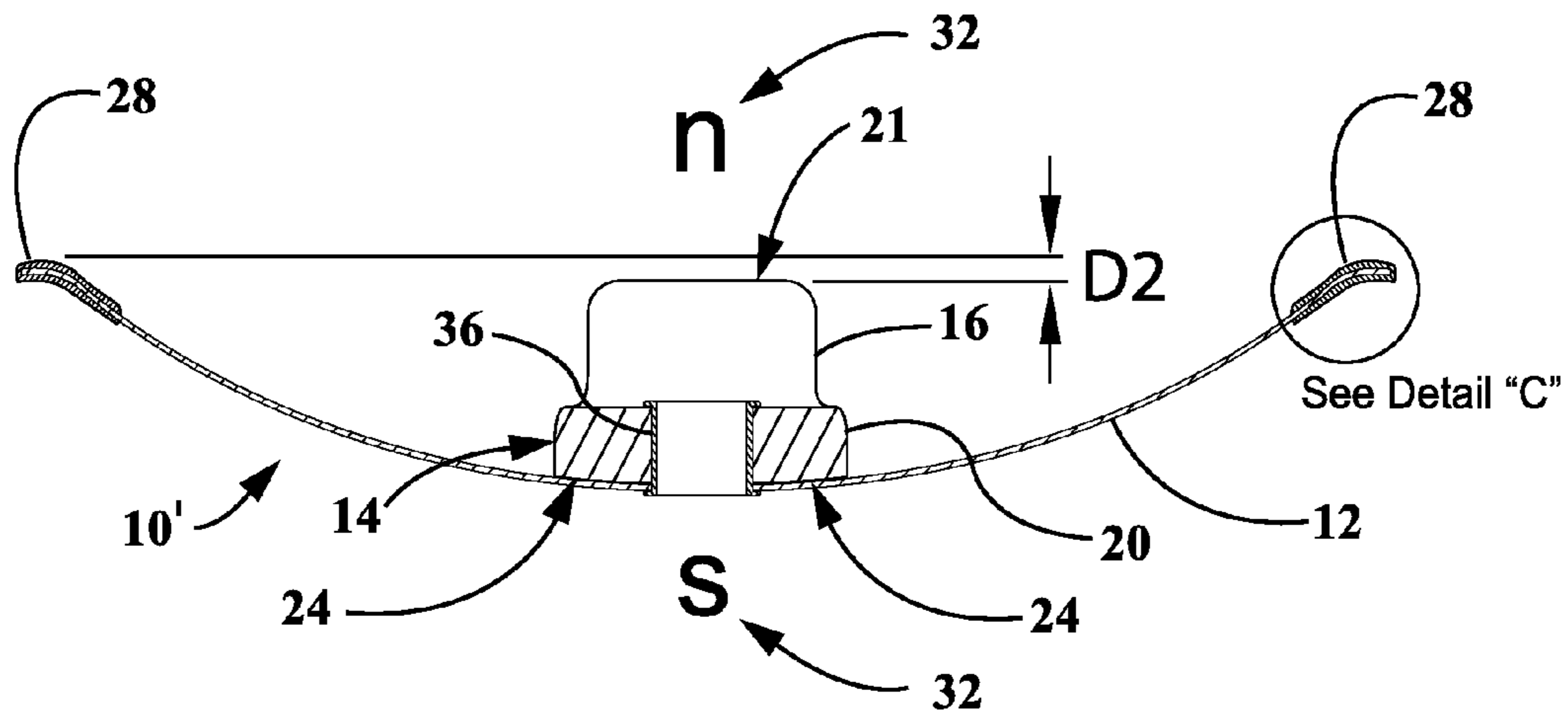
Section B-B
