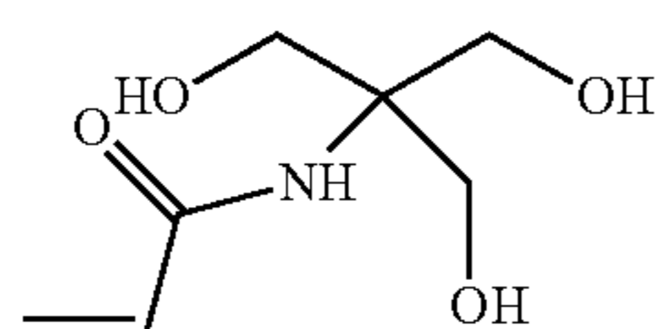
N-[Tris(hydroxymethyl)methyl]acrylamide
