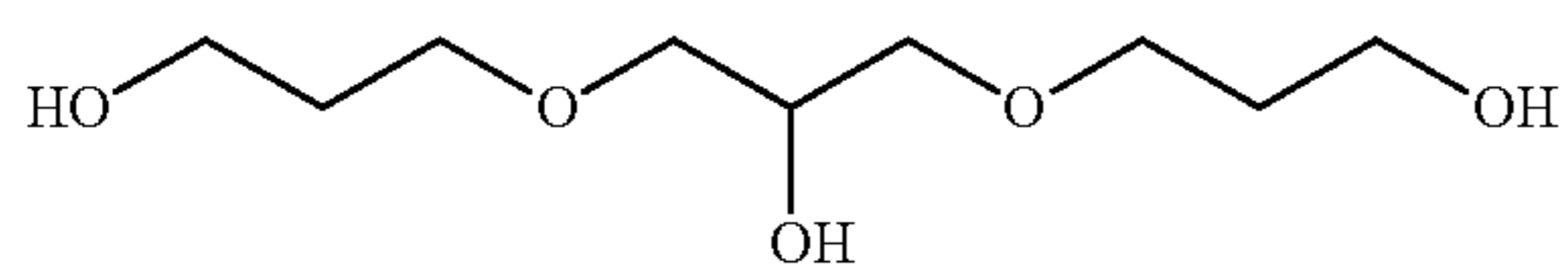
1,3-Di(hydroxypropoxy)-2-hydroxyl-propane
