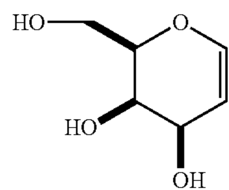
D-Galactool
