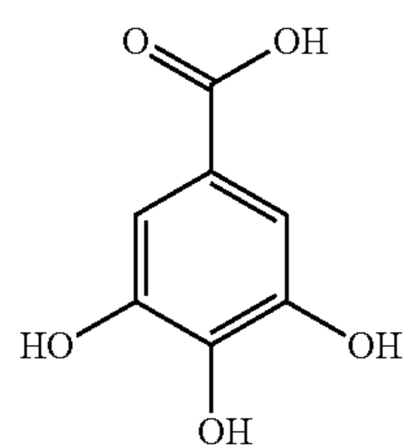
Gallic acid
