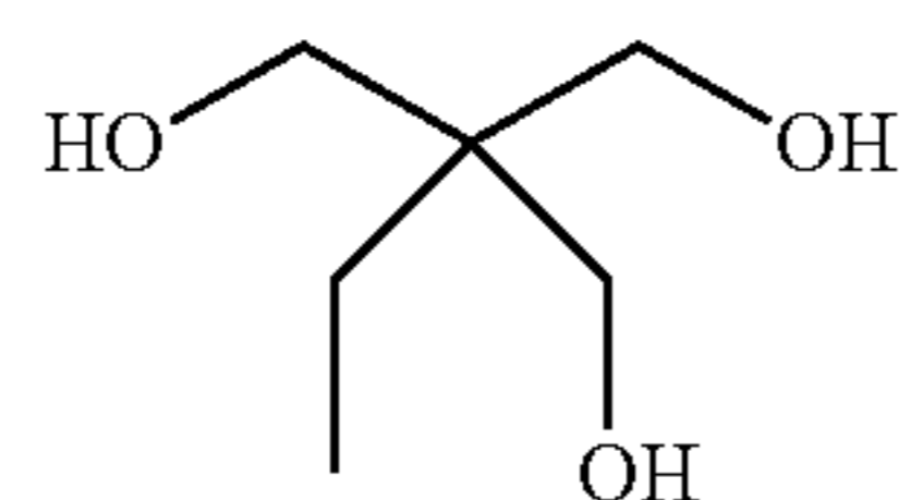
1,1,1-Tris(hydroxymethyl)propane
