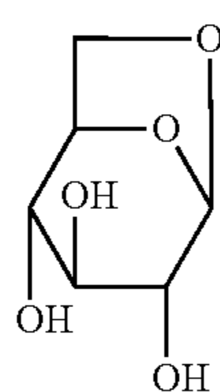
1,6-anhydro-β-D-Glucose
