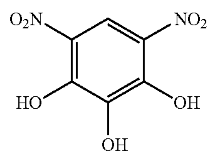
4,6-Nitropyrogallol
