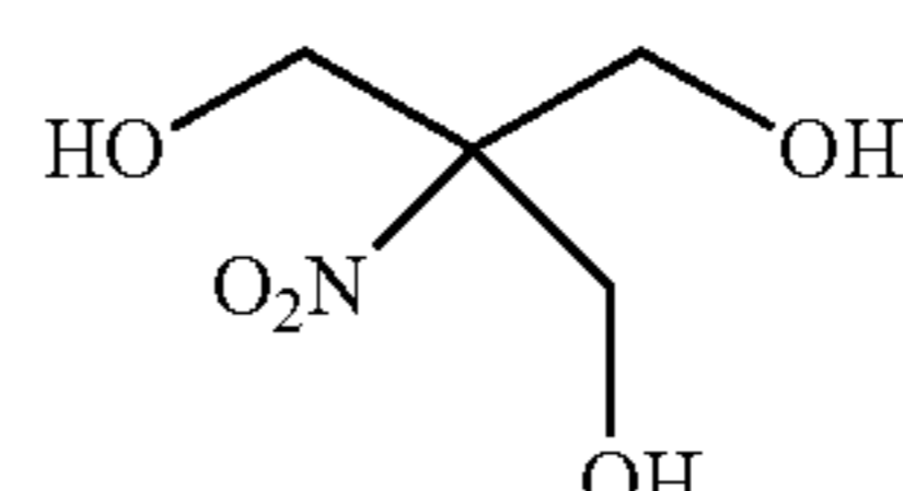
1,1,1-Tris(hydroxymethyl)nitromethane
