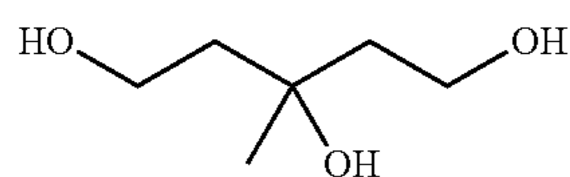
3-Methyl-1,3,5-pentanetriol
