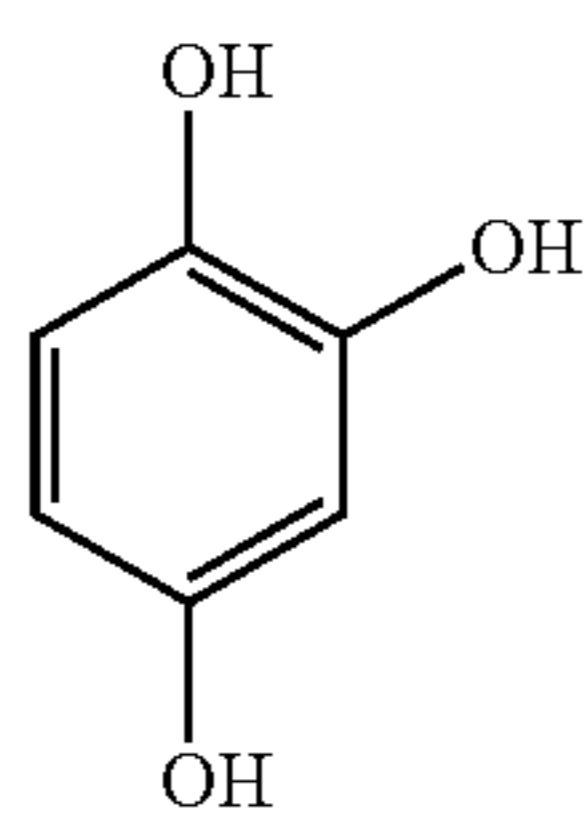
1,2,4,-Trihydroxyl-benzene
