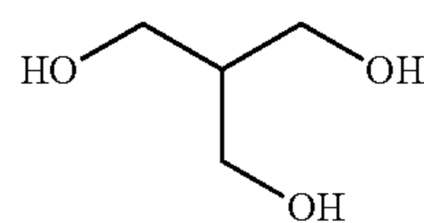
2-(hydroxymethyl)-1,3-propanediol
