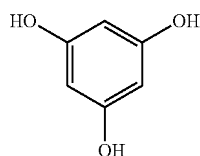
1,3,5-Trihydroxyl-benzene
