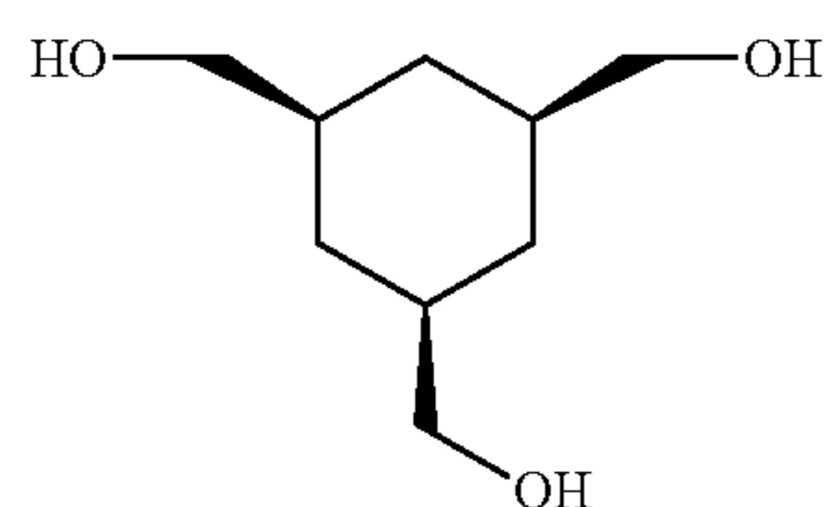
cis-1,3,5-Tri(hydroxymethyl)cyclohexane
