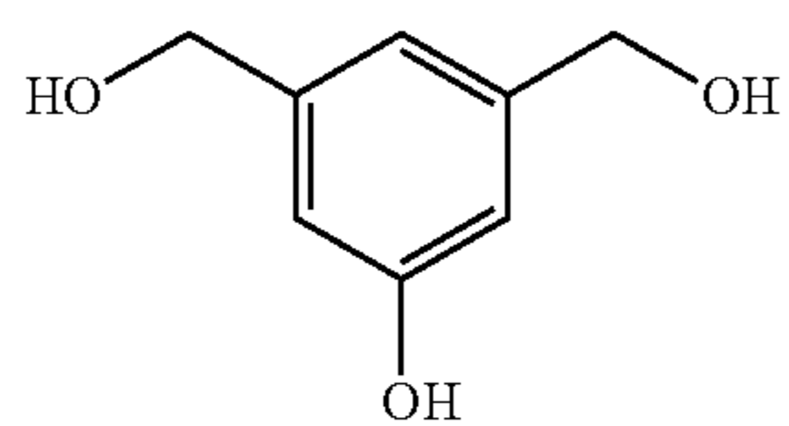
3,5,-Di(hydroxymethyl)phenol
