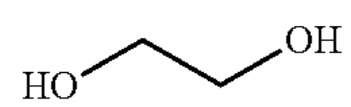
Ethylene glycol
