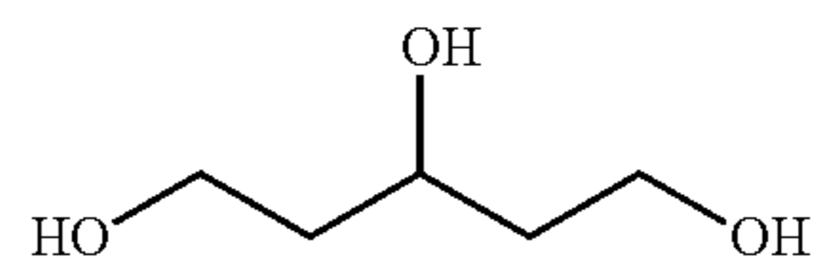
1,3,5-Pentanetriol
