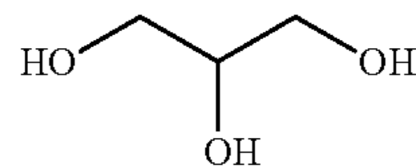
Glycerol (1,2,3-Propanetriol)
