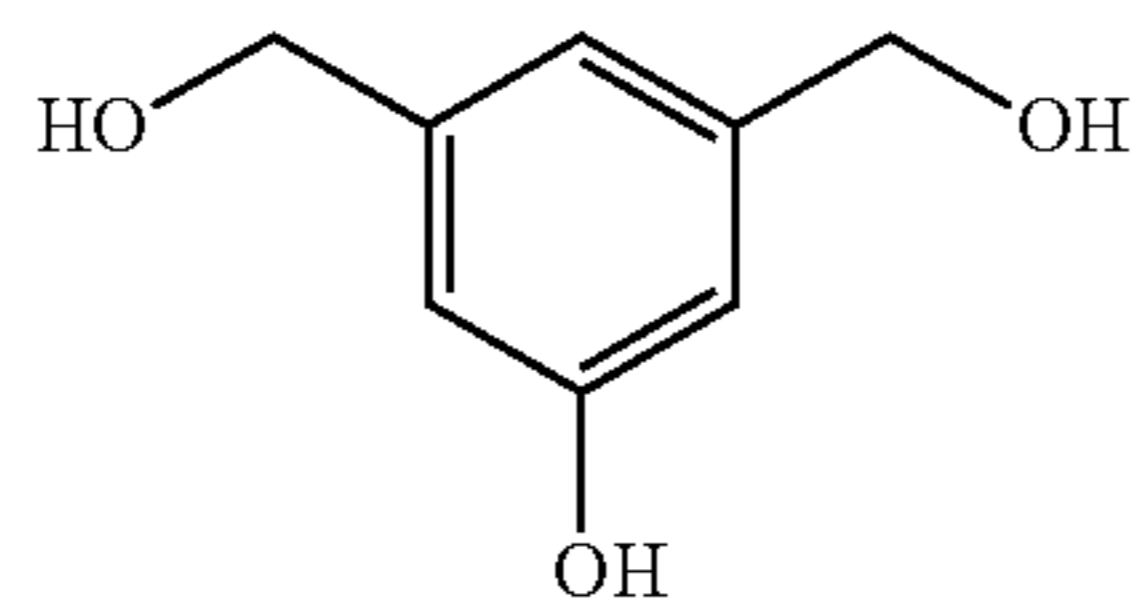
1,3,5,-Tri(hydroxymethyl)benzene
