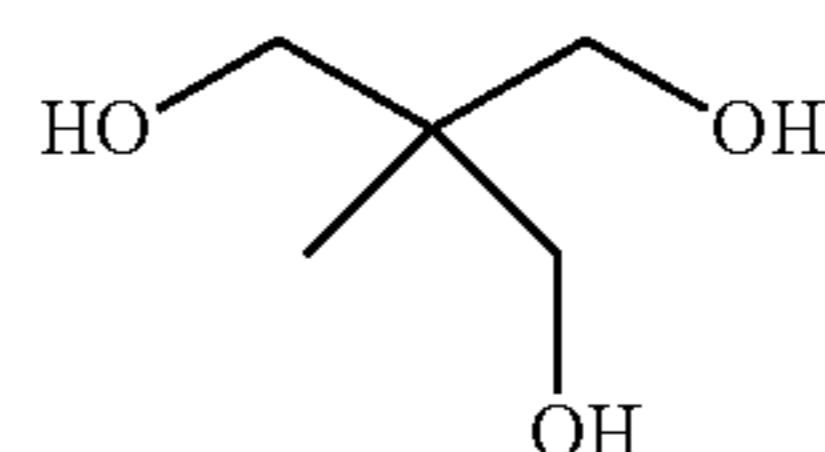
1,1,1-Tris(hydroxymethyl)ethane
