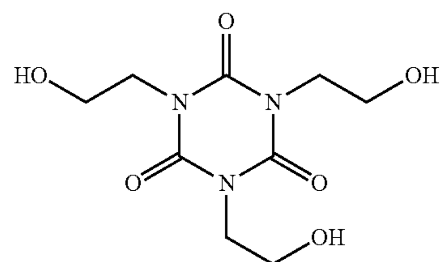
1,3,5-Tris(2-hydroxyethyl)-Cyanuric acid
