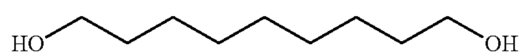
1,9-Nonanediol
