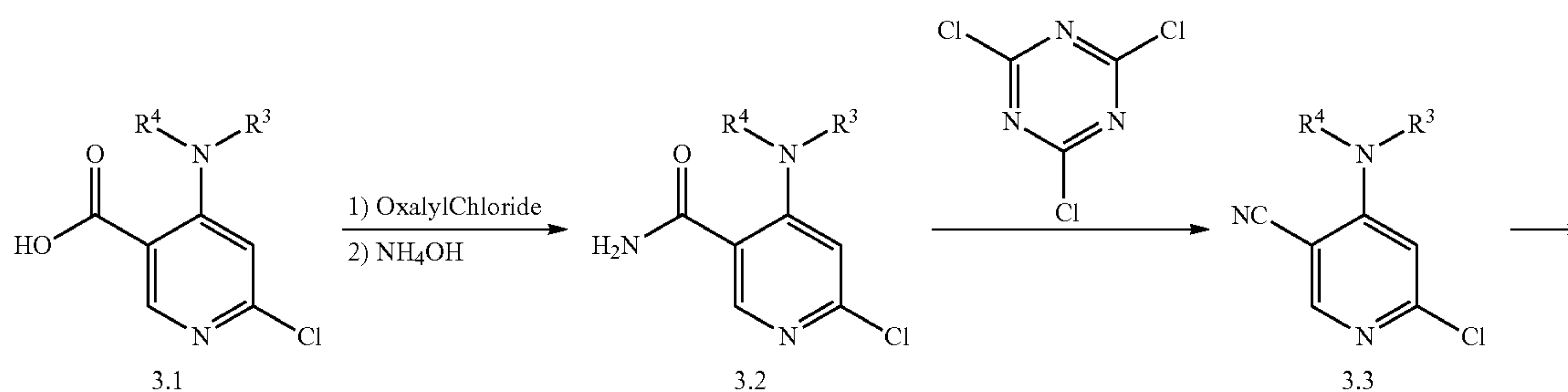
Scheme 3
