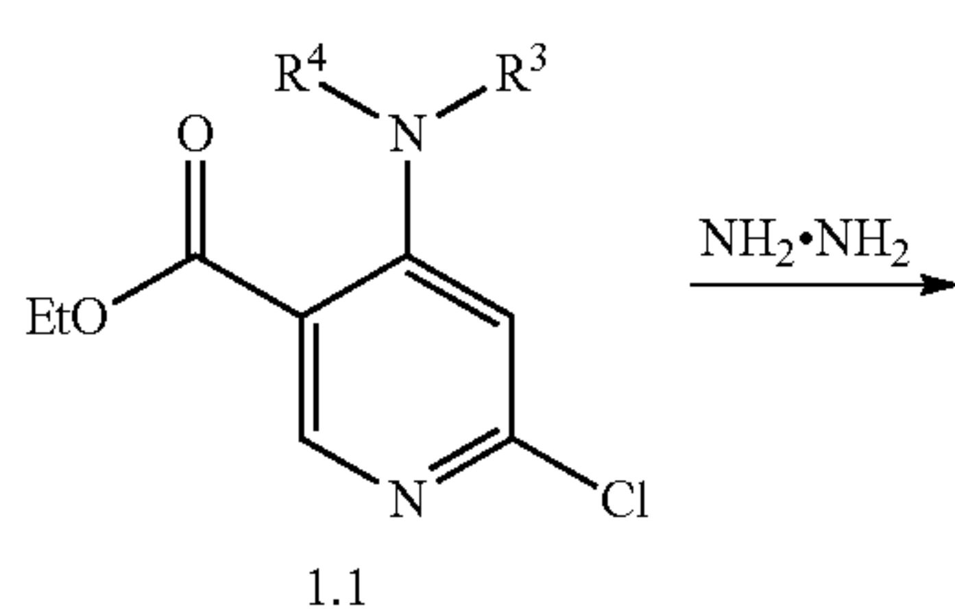
Scheme 2
