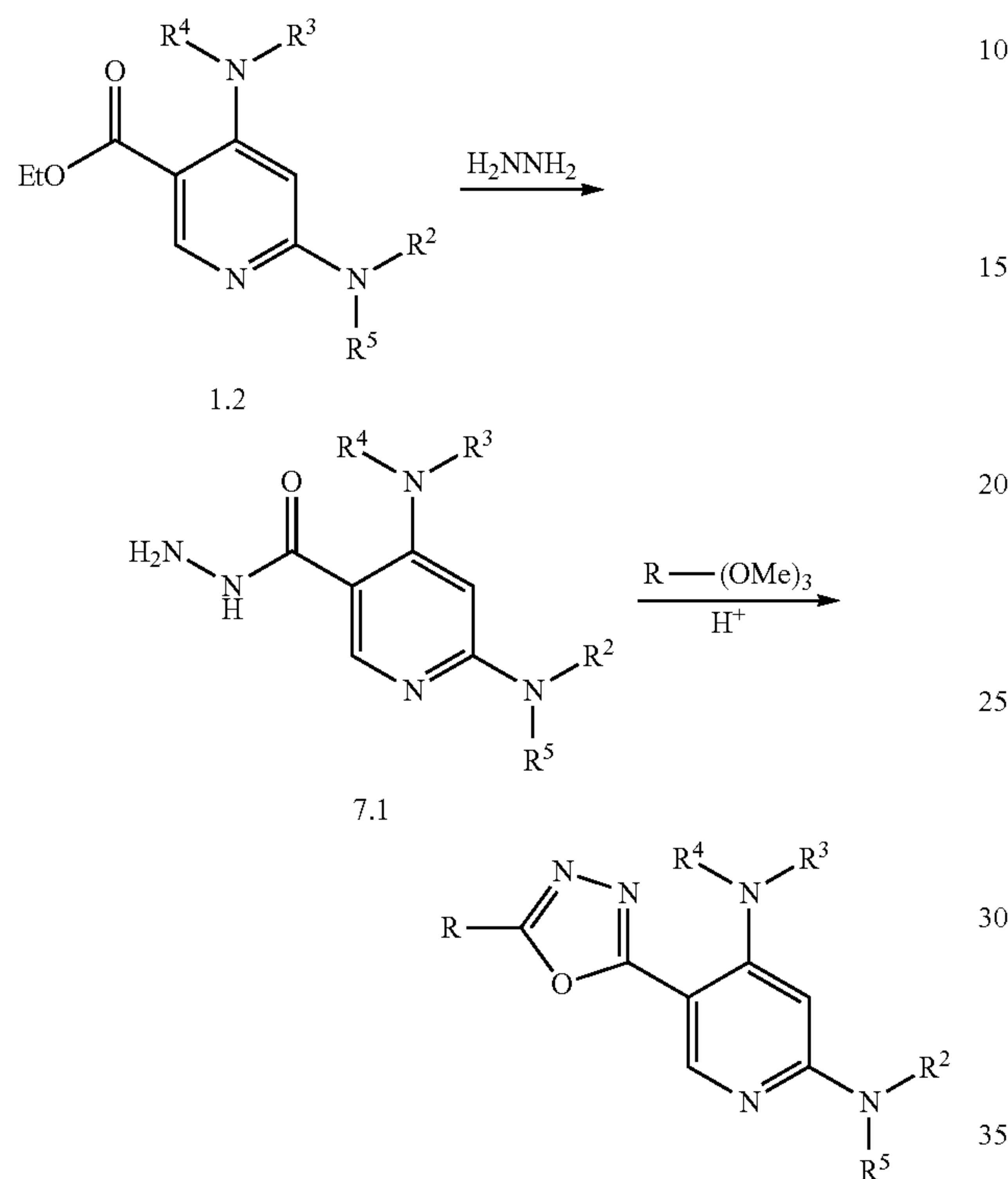
Scheme 7
