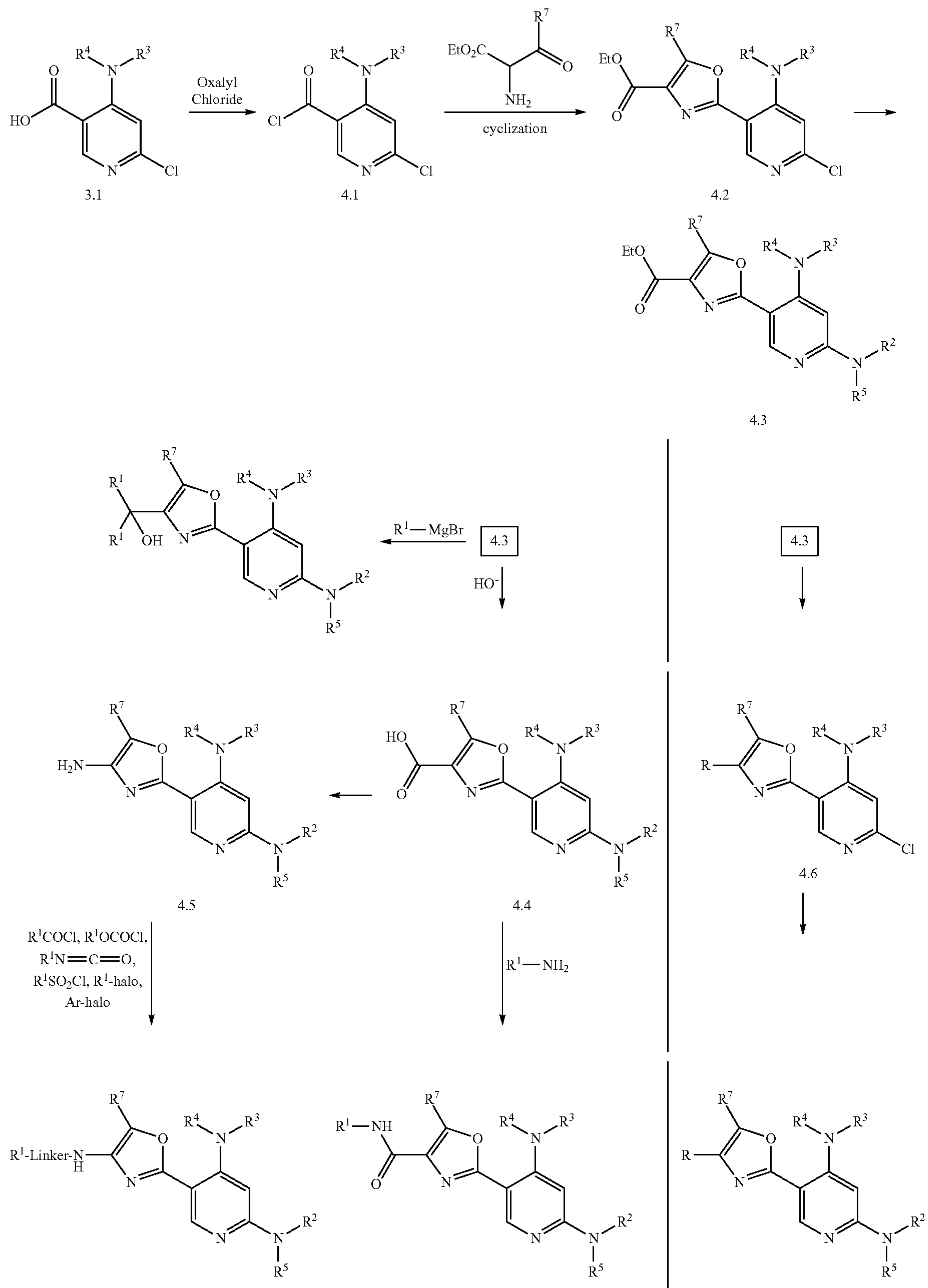
Scheme 4
