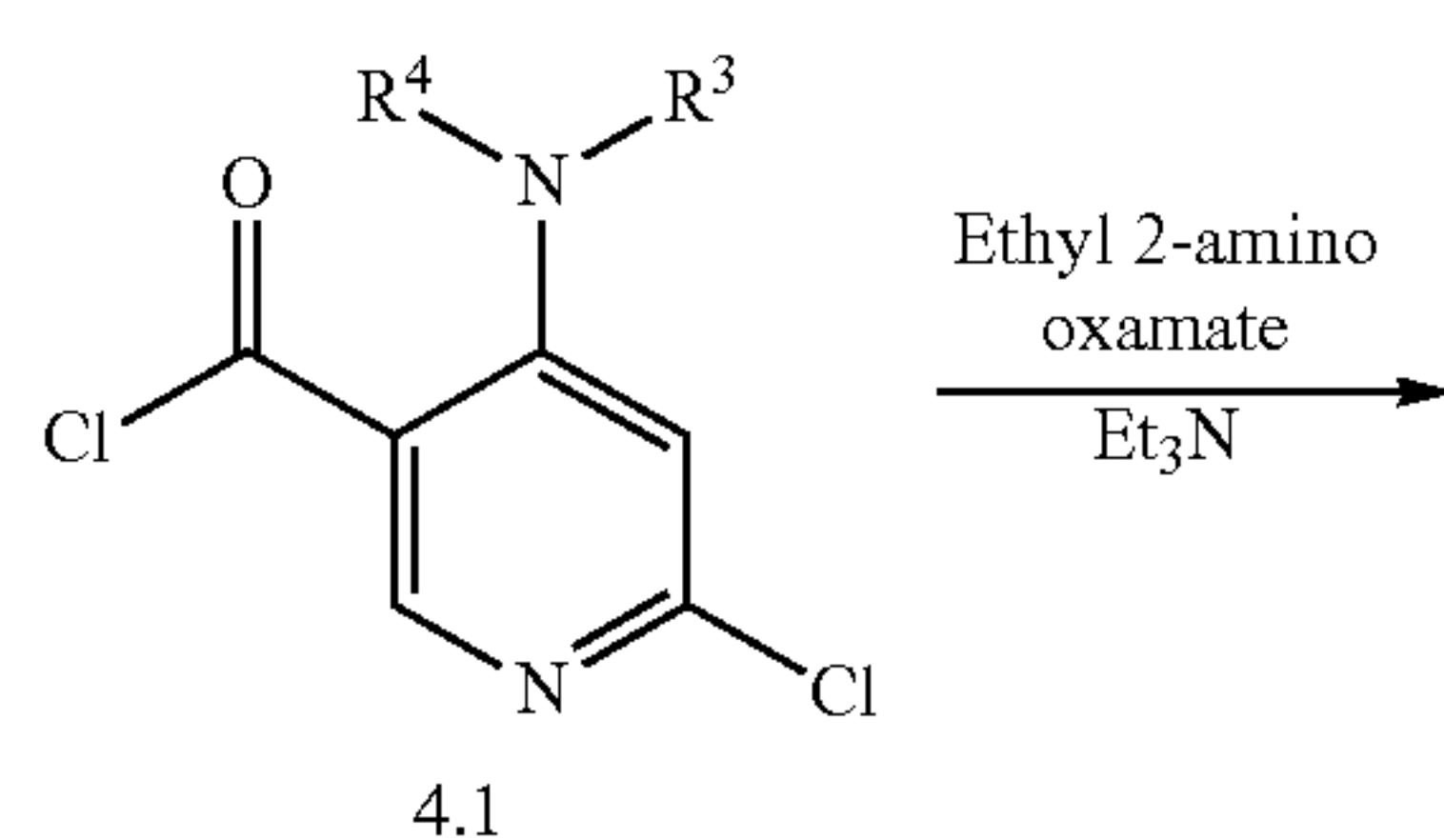
Scheme 8
