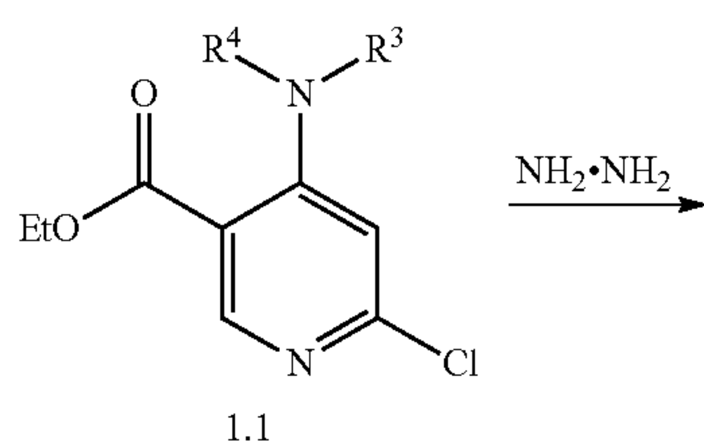
Scheme 2
