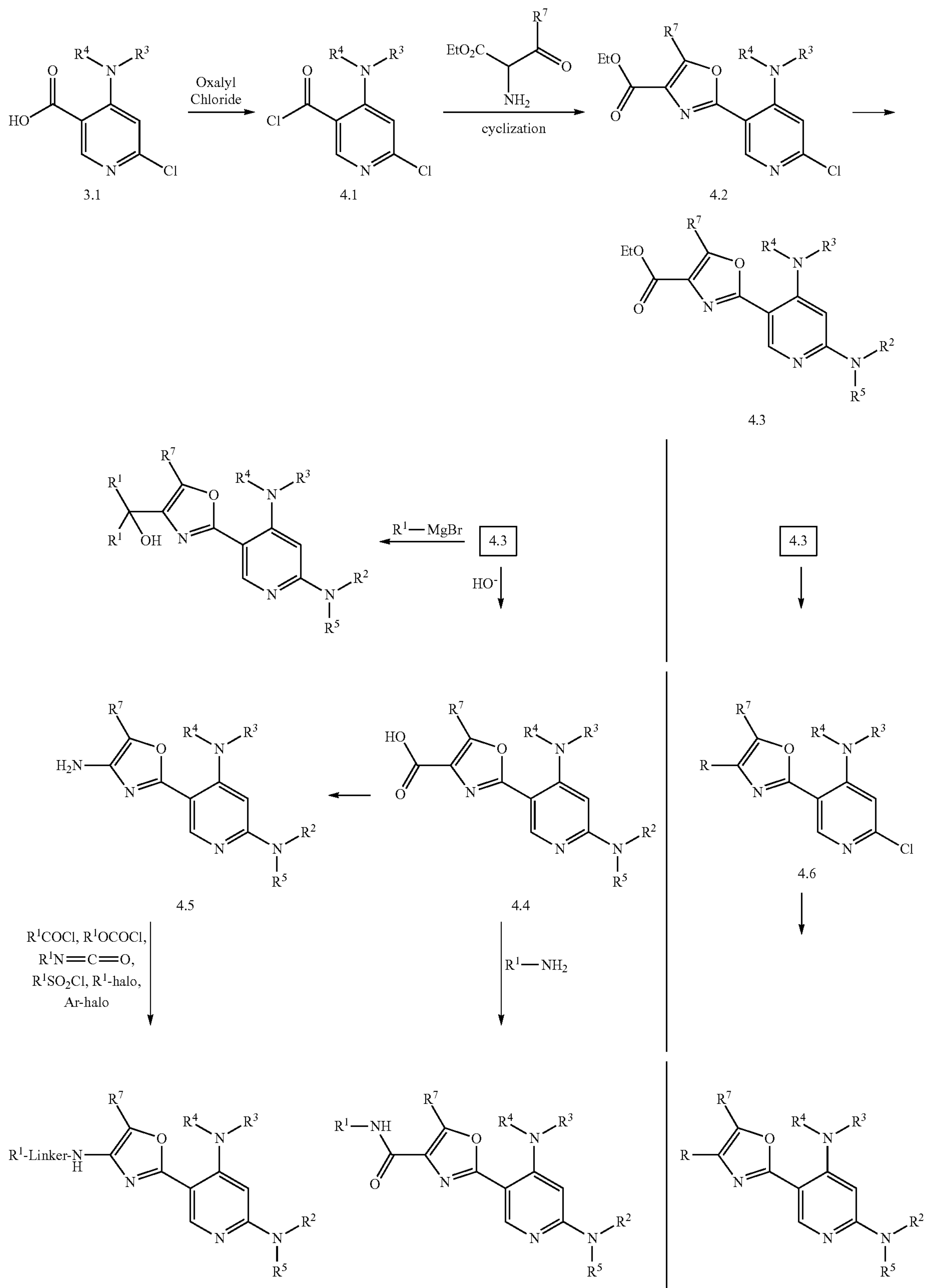
Scheme 4
