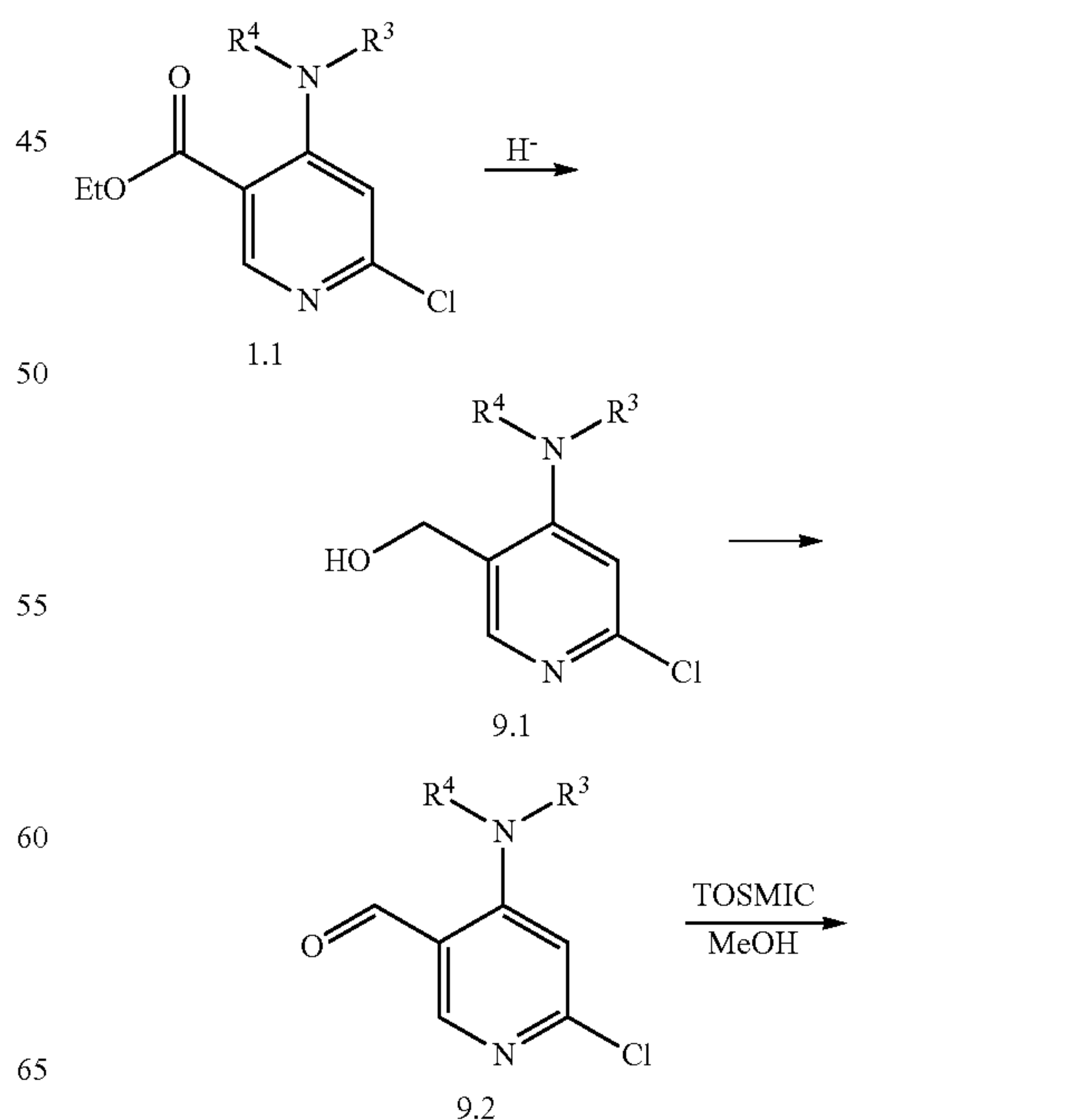
Scheme 9
