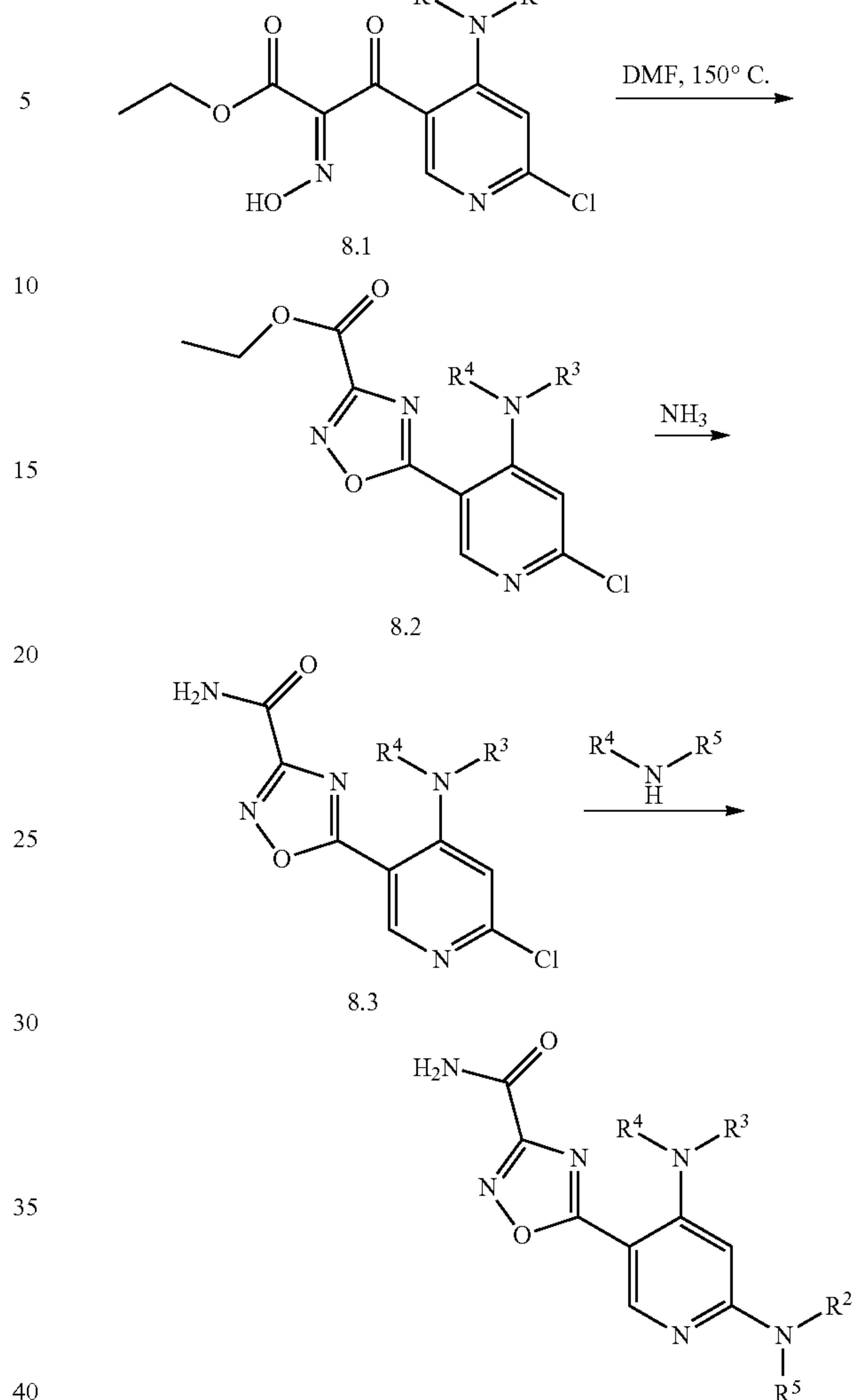
Scheme 9
