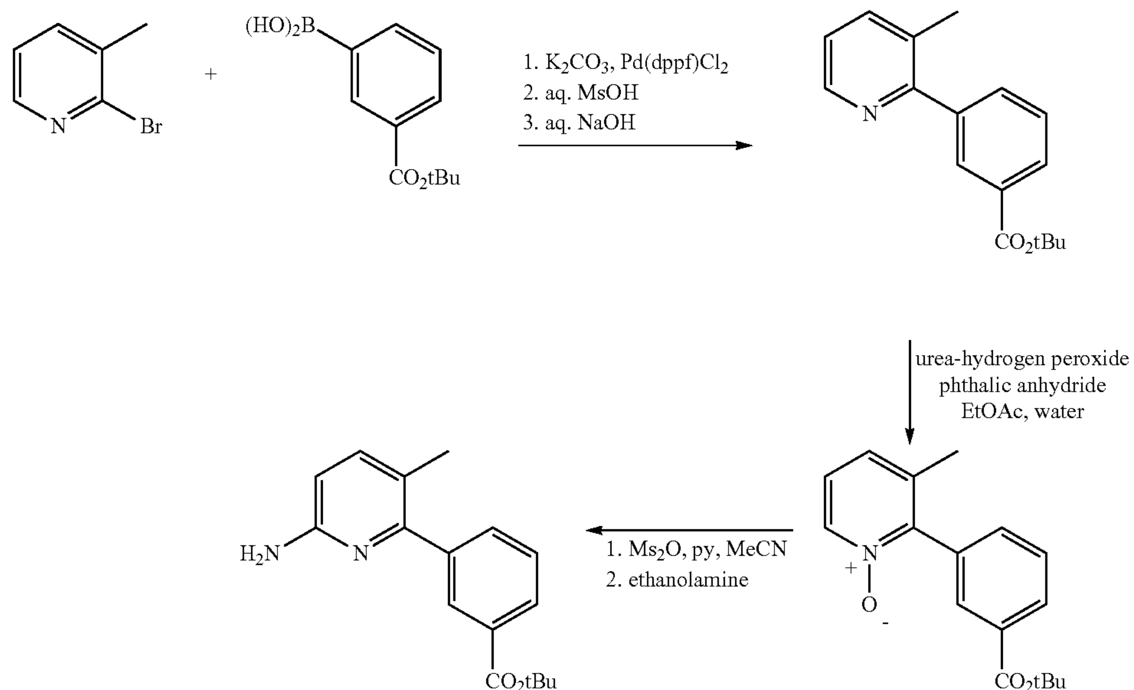
Scheme 3.
