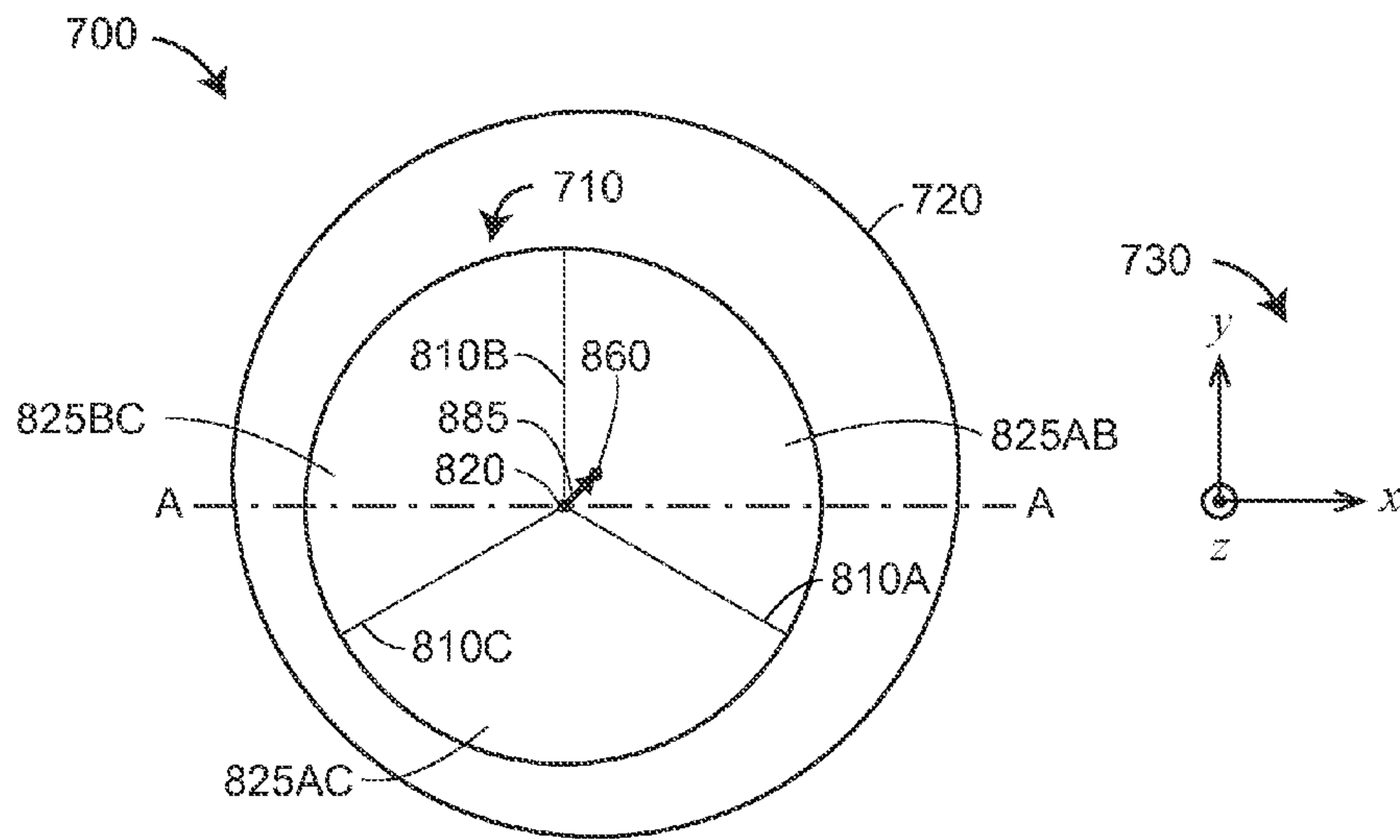
FRONT VIEW FIG. 7A
