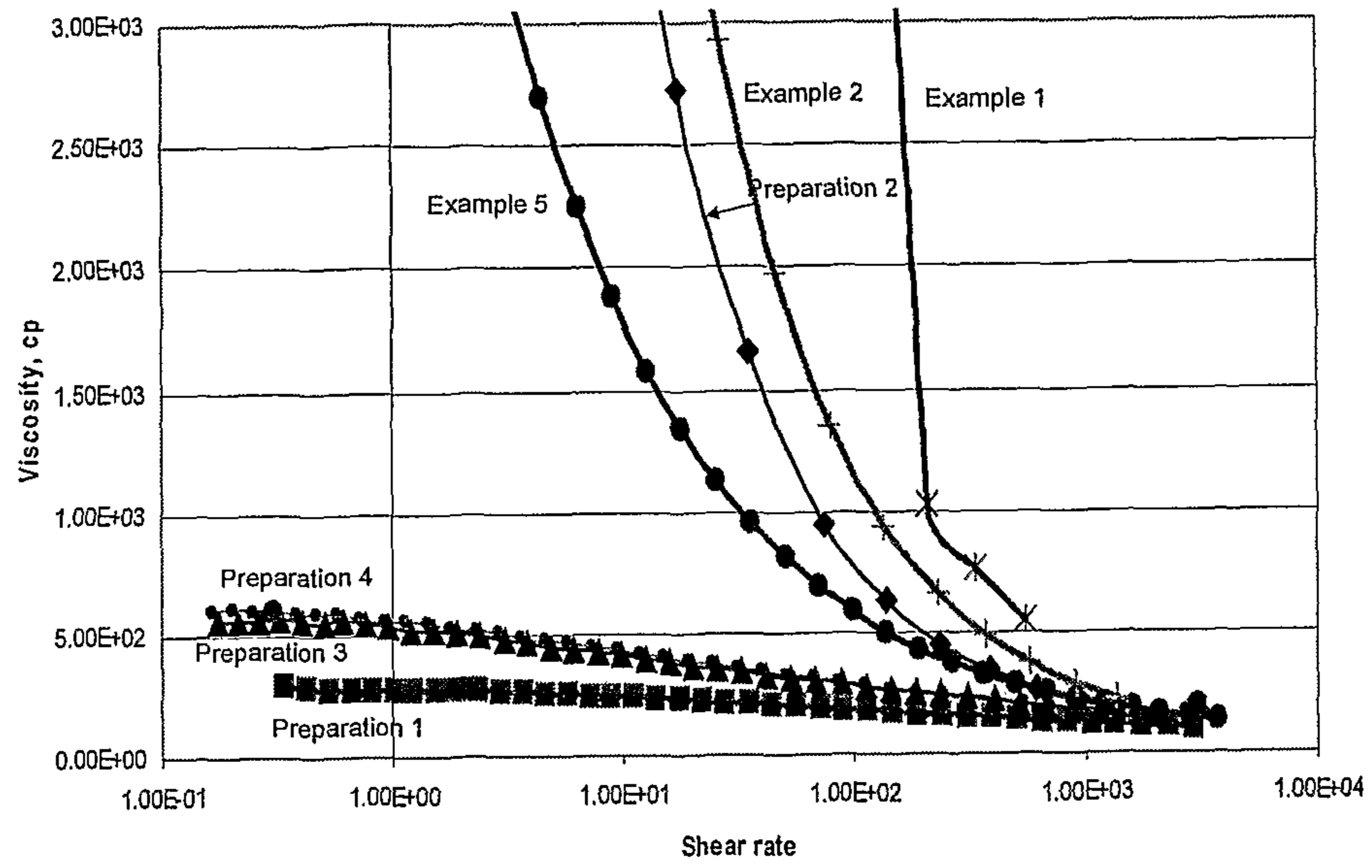
Figure 1: Viscosity Comparison of Various Dispersants in Premix Formulation 1
