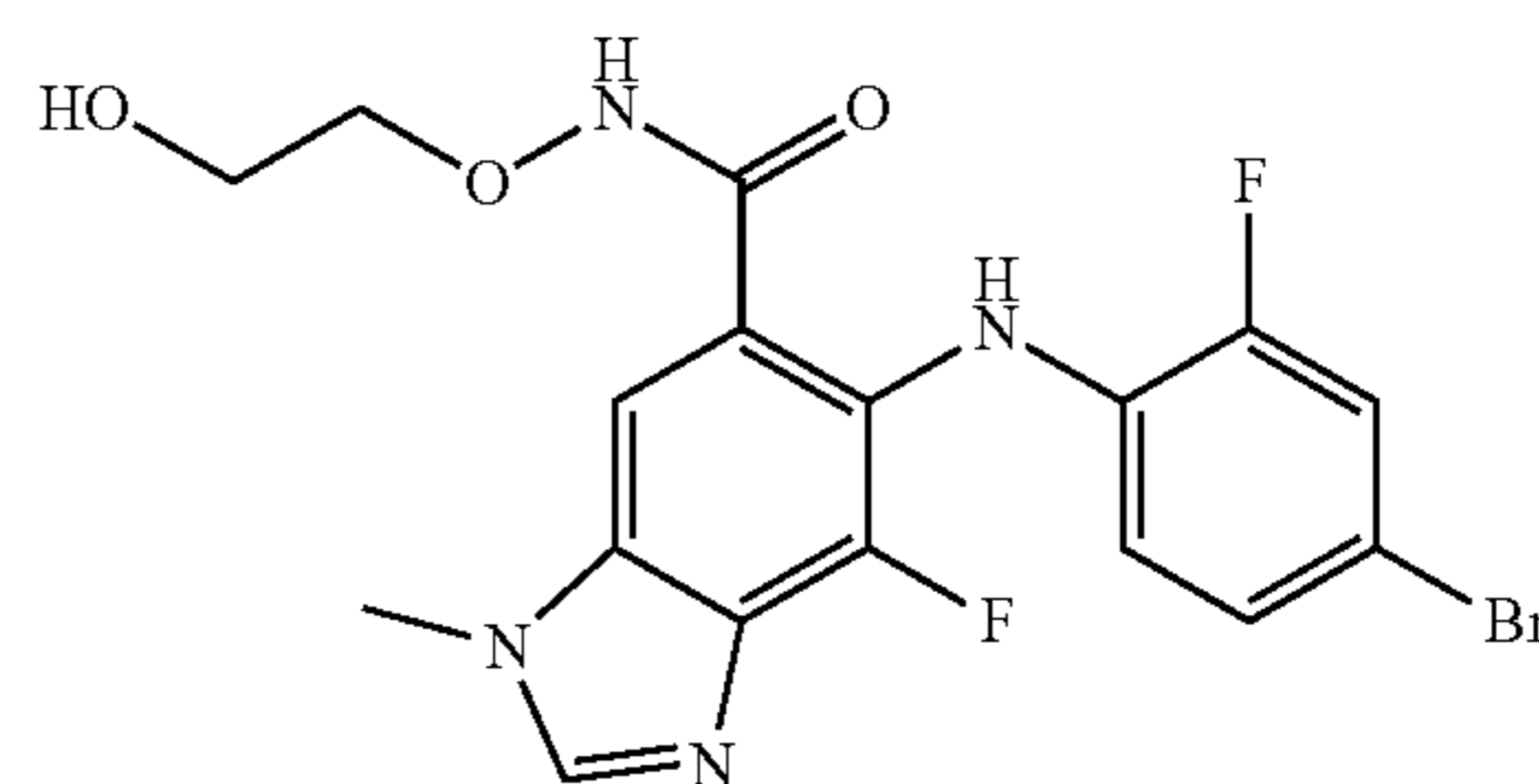
Compound A
