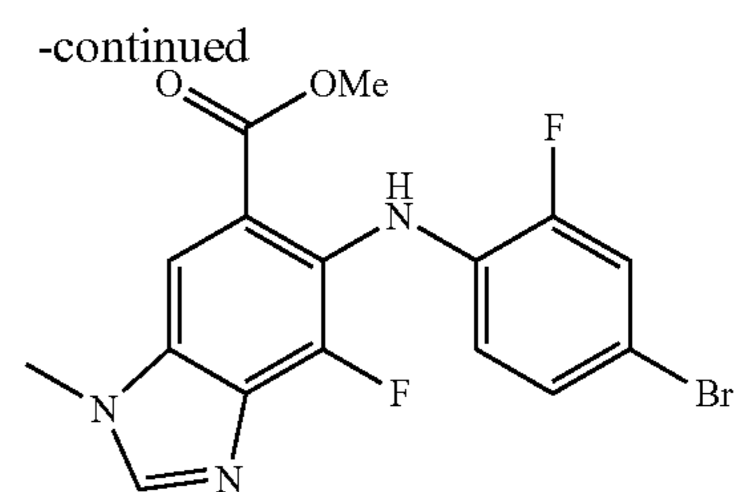
Compound 3
