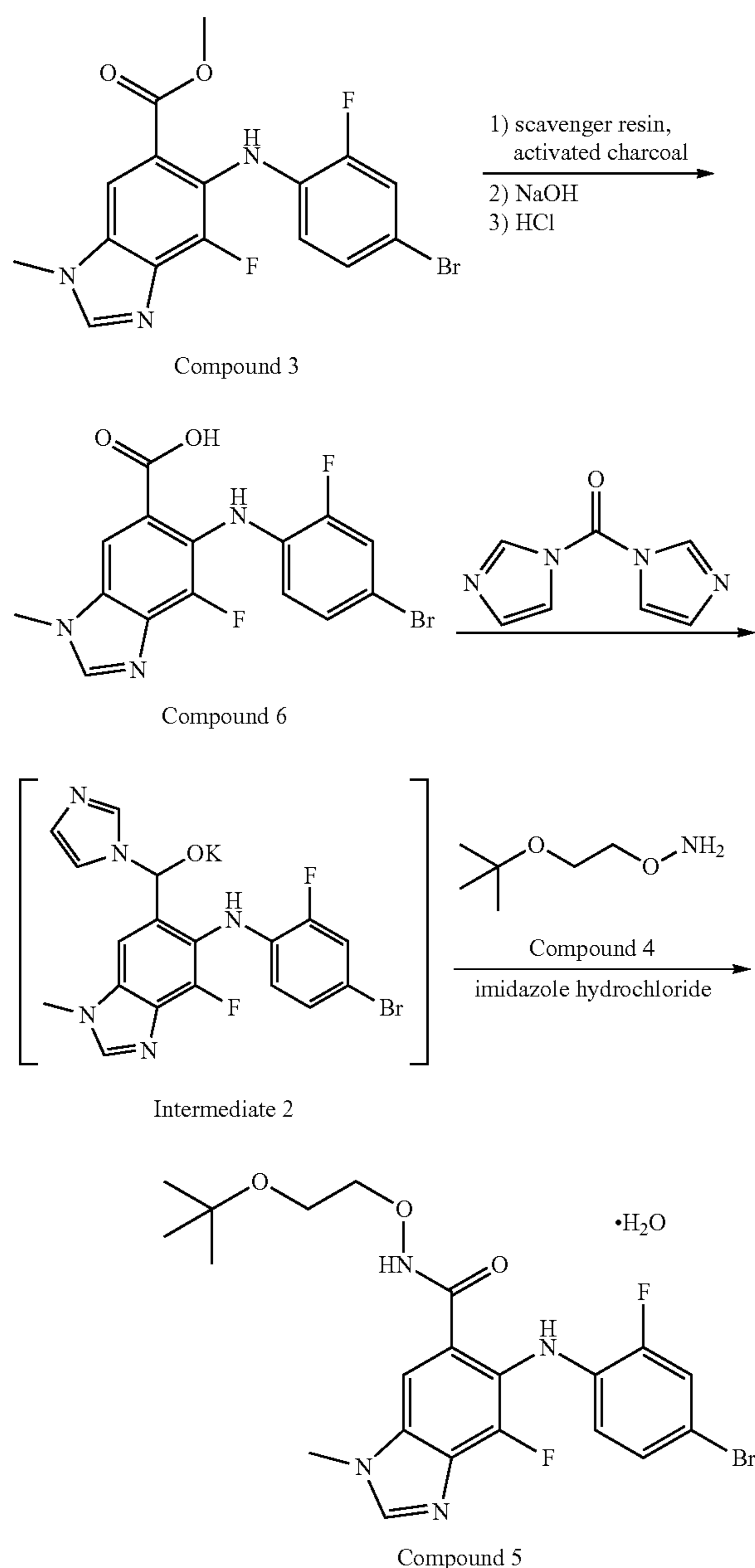
6-(4-Bromo-2-fluorophenylamino)-7-fluoro-3-methyl-3H-benzimidazole-5-carboxylic acid
