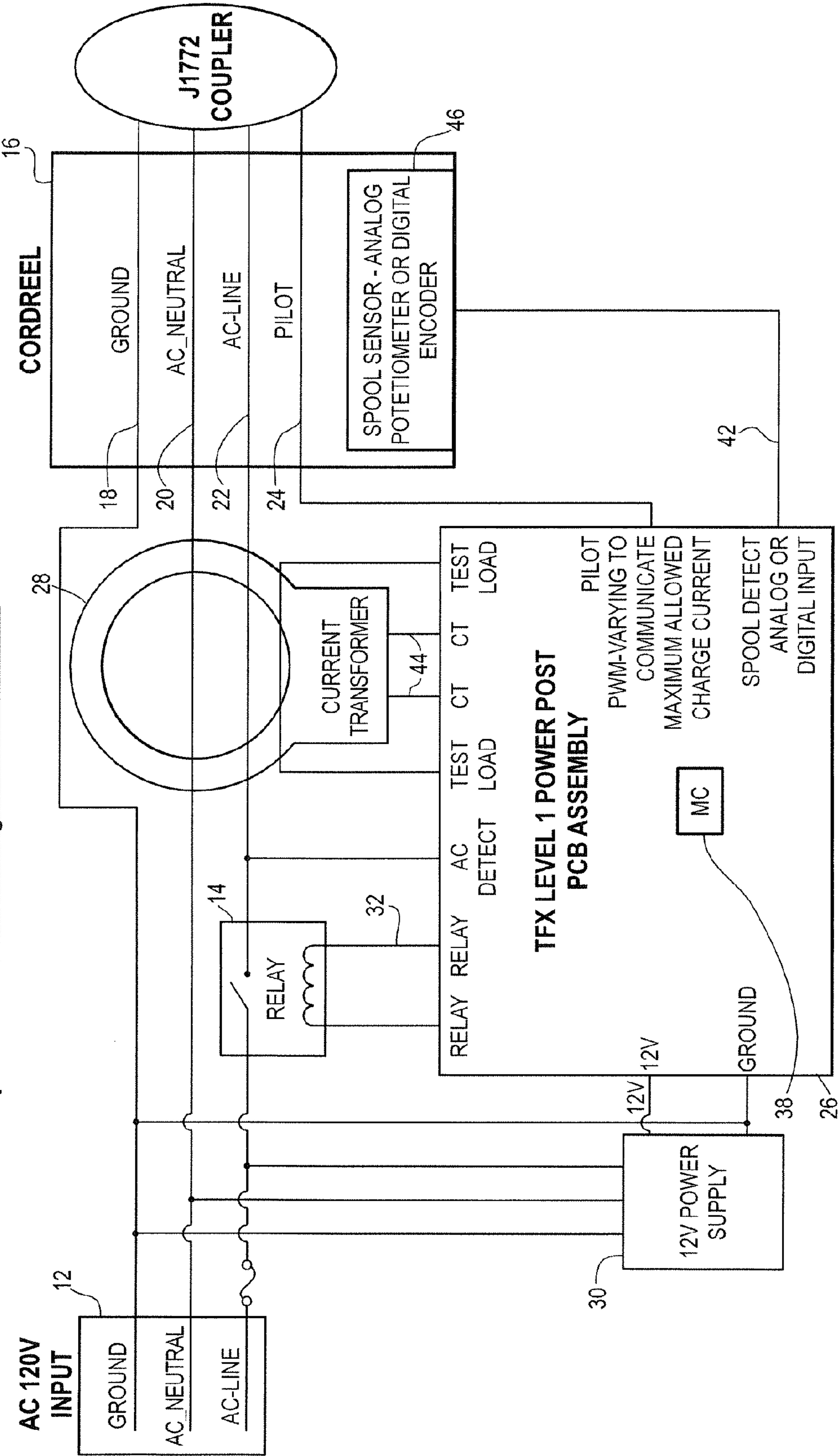
Fig. 1 Telefonix Level 1 Power Post - Electrical Block Diagram Spool Detection / Charge Current control
