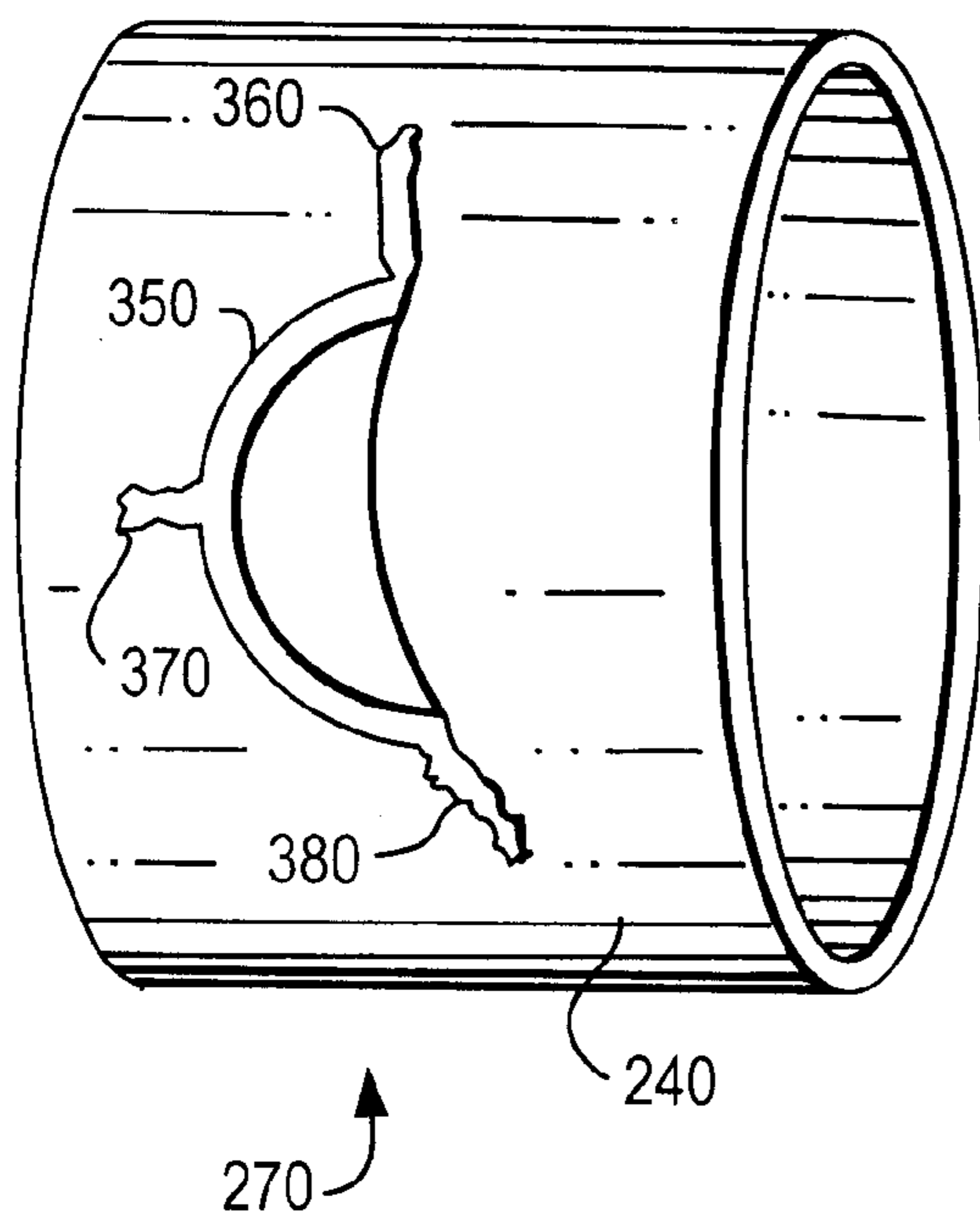
FIG. 3C PRIOR ART
