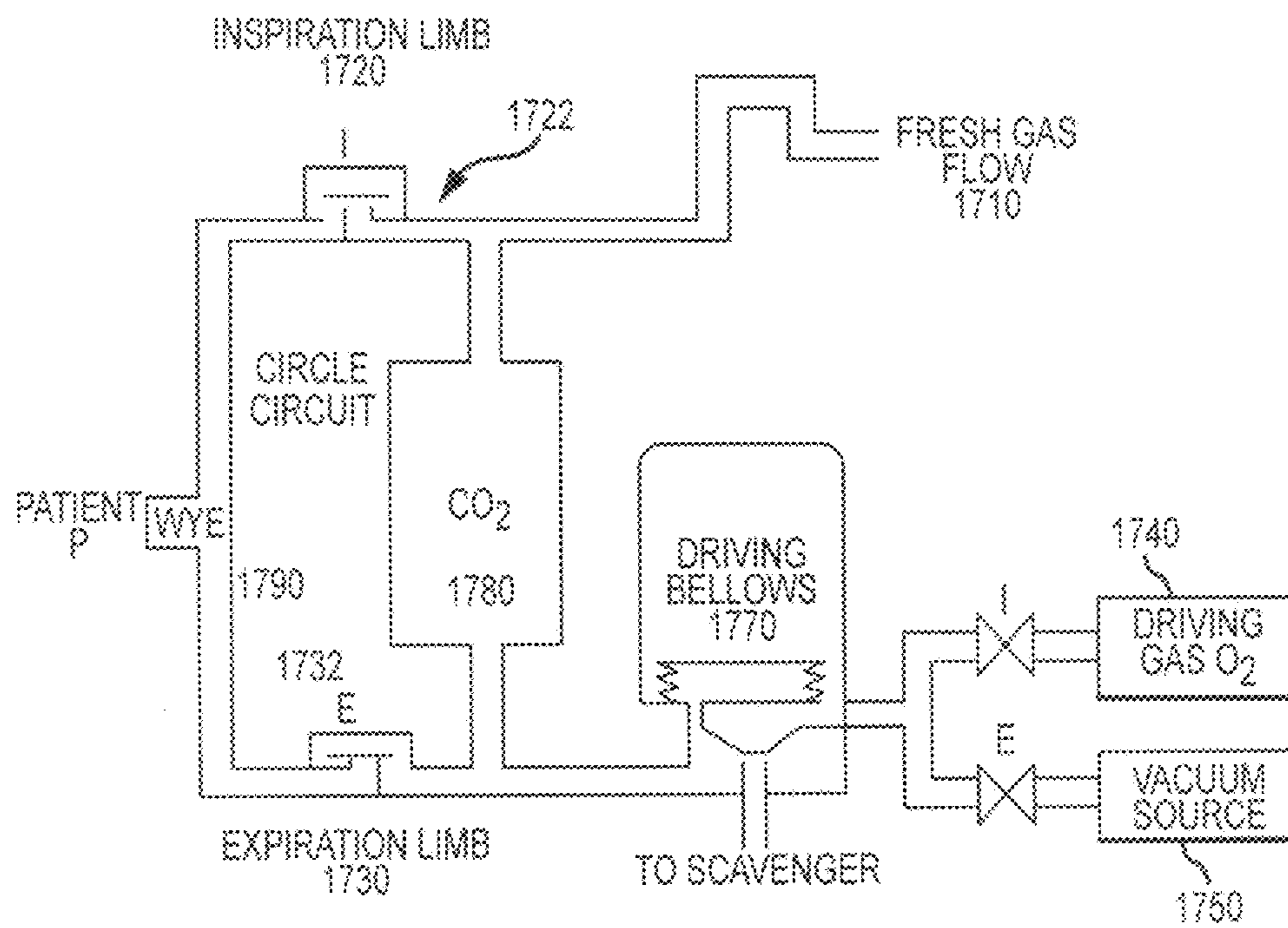
ANESTHESIA MACHINE WITH ACTIVE EXHALATION
