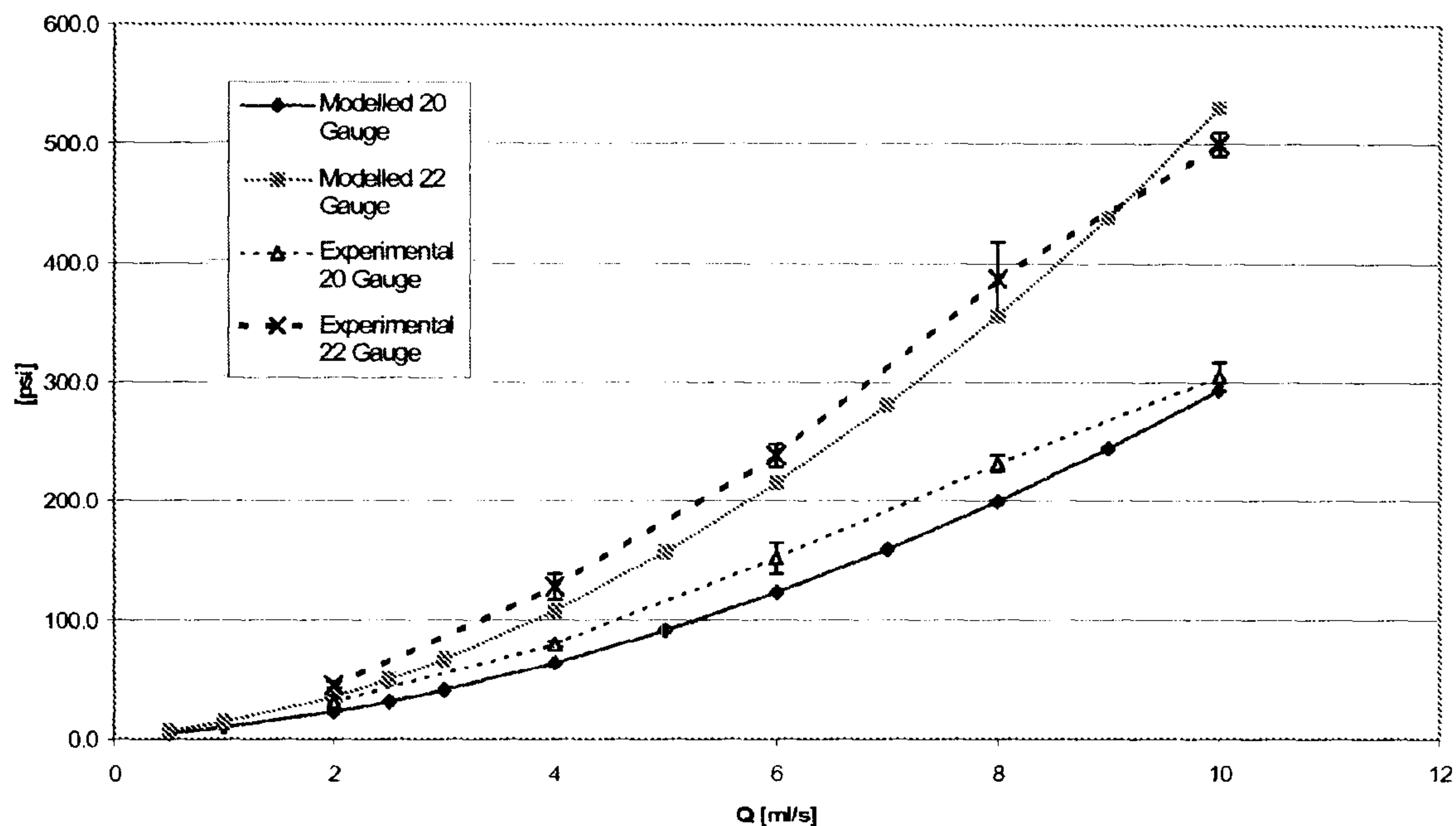
Saline Theoretical and Experimental Press vs Flow (96" LPCT, .075"ID)
