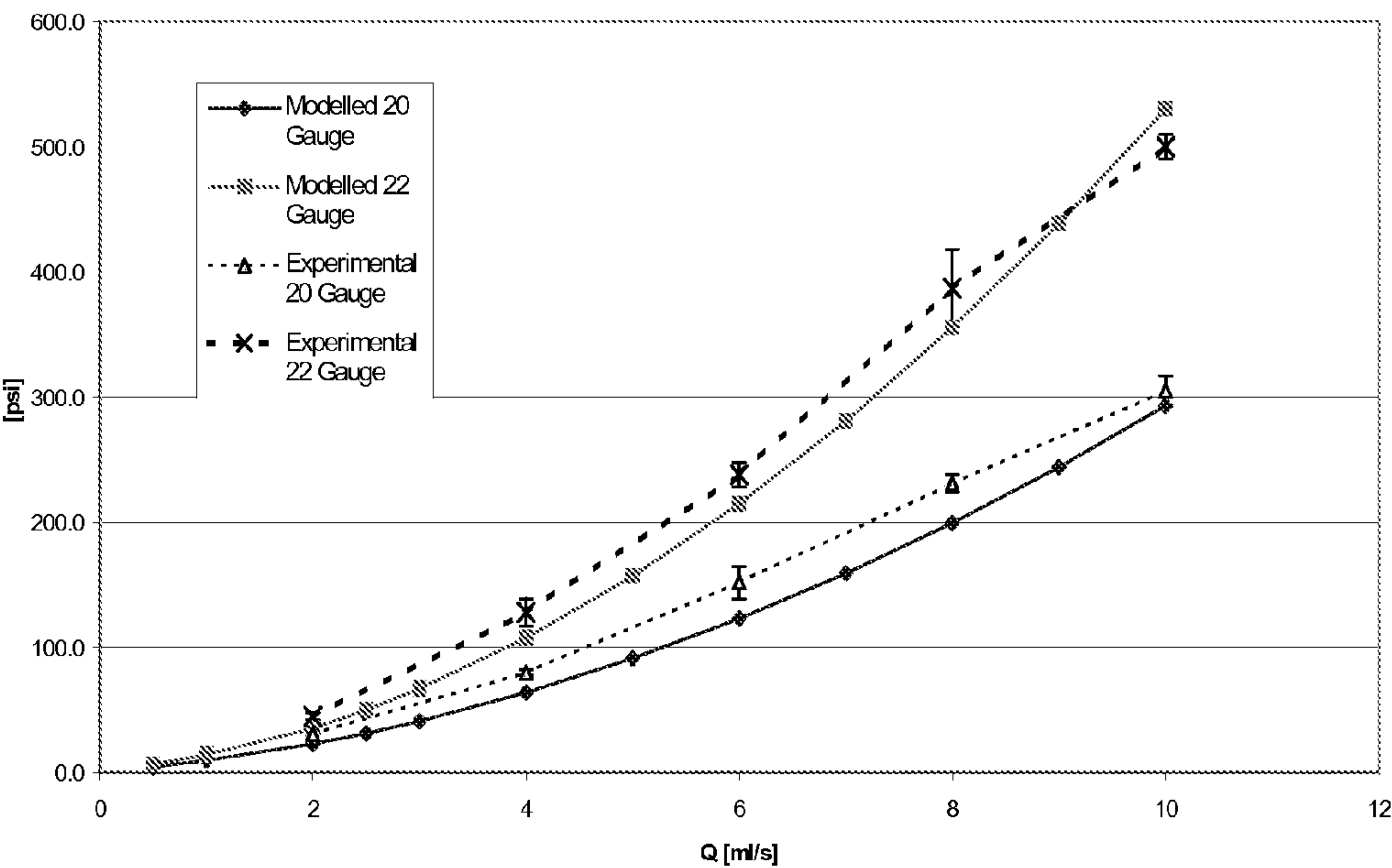
Saline Theoretical and Experimental Press vs Flow (96" LPCT, .075"ID) Error bars = +/-1 sigma
