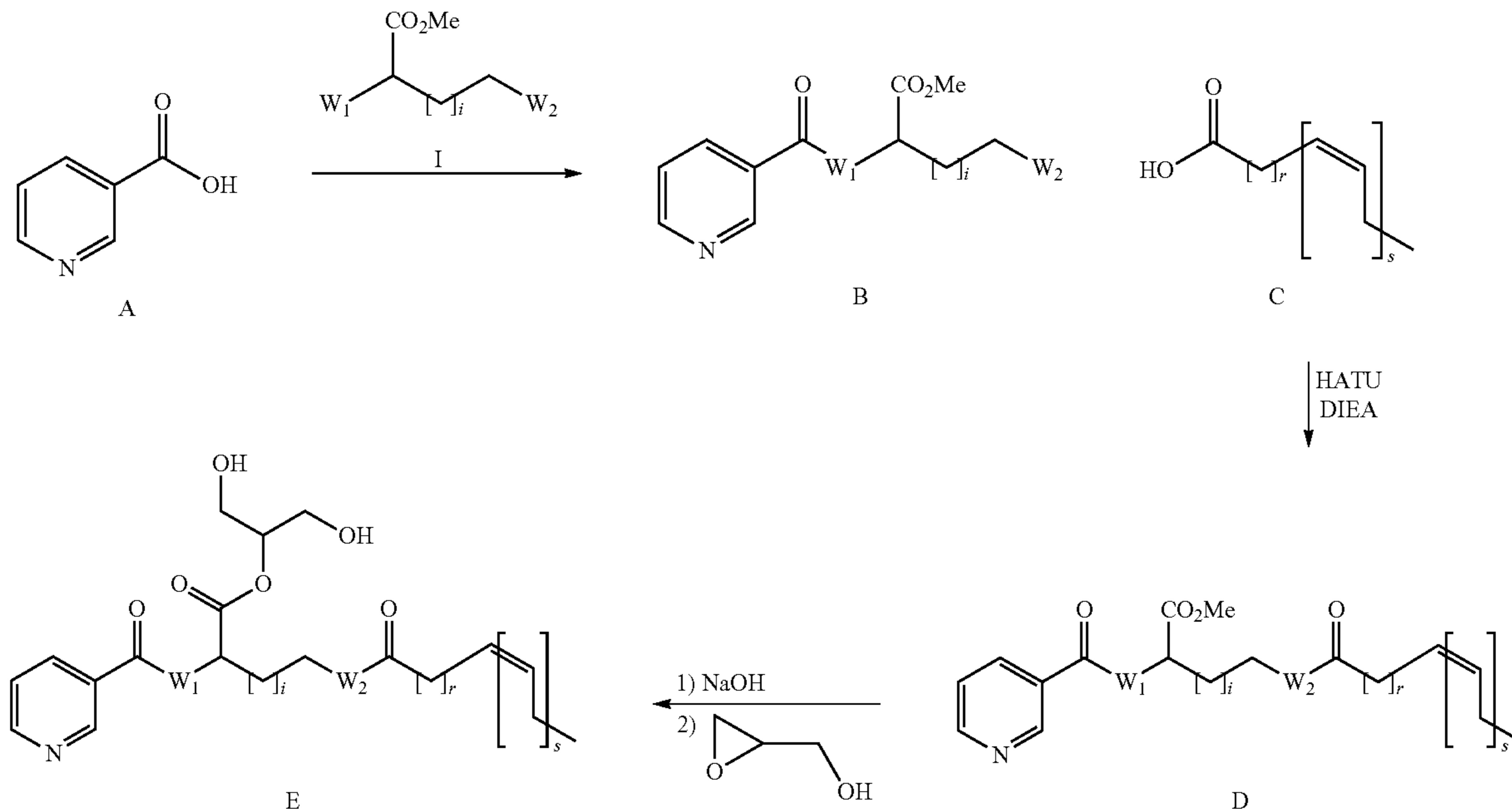
Scheme 11
