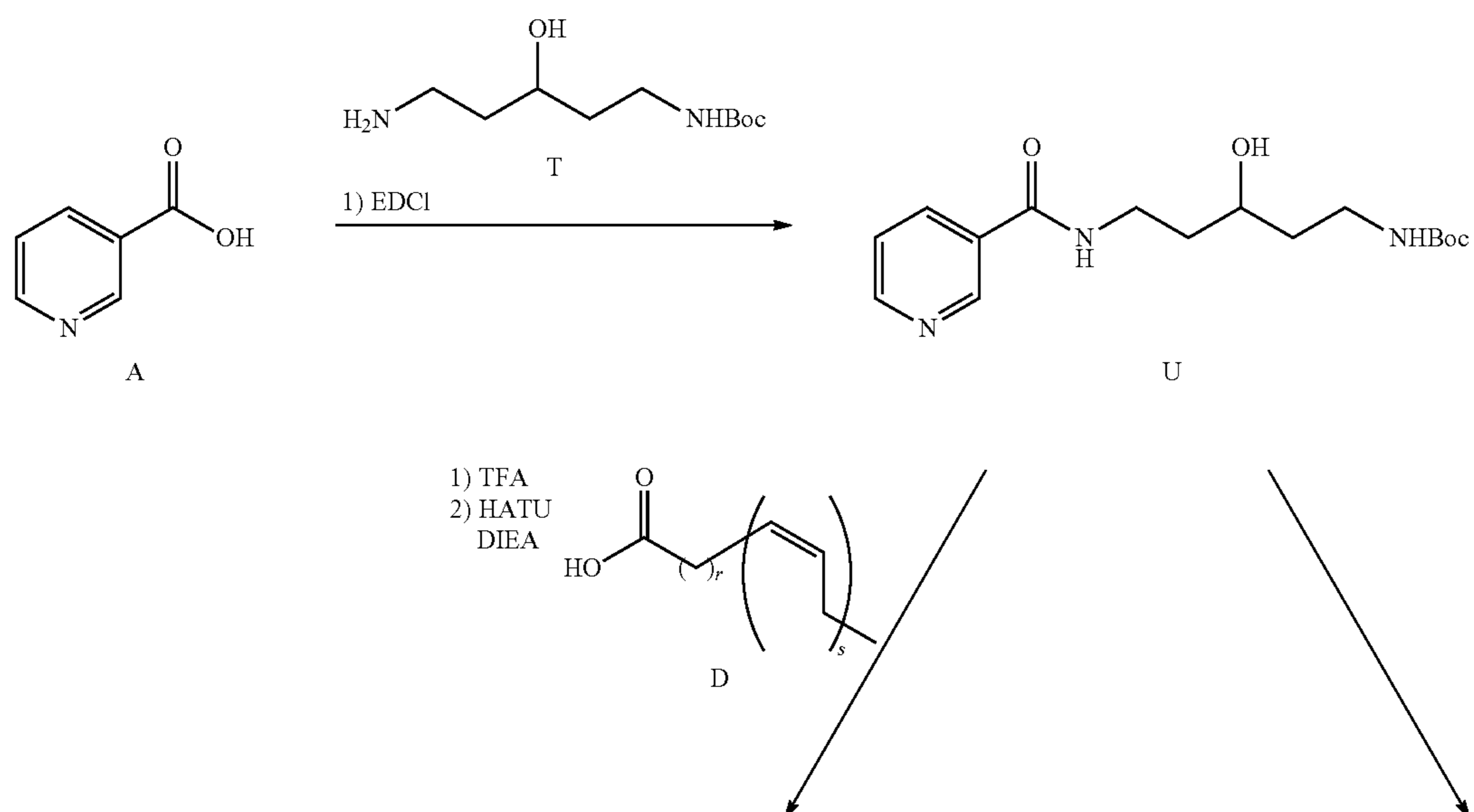
Scheme 6
