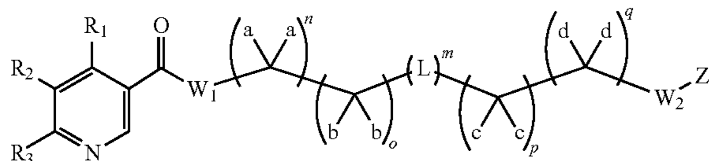
Formula I
