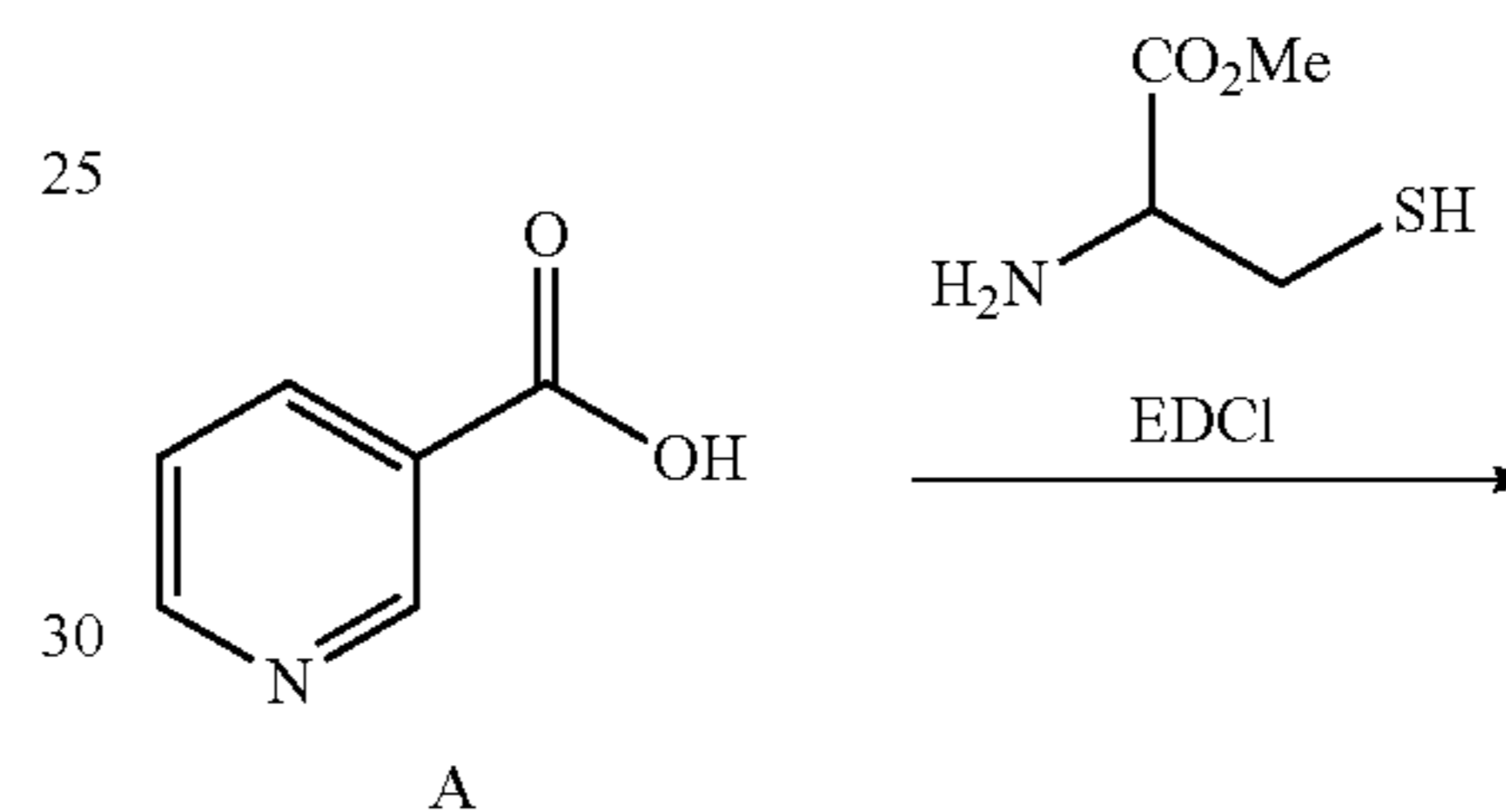
Scheme 8
