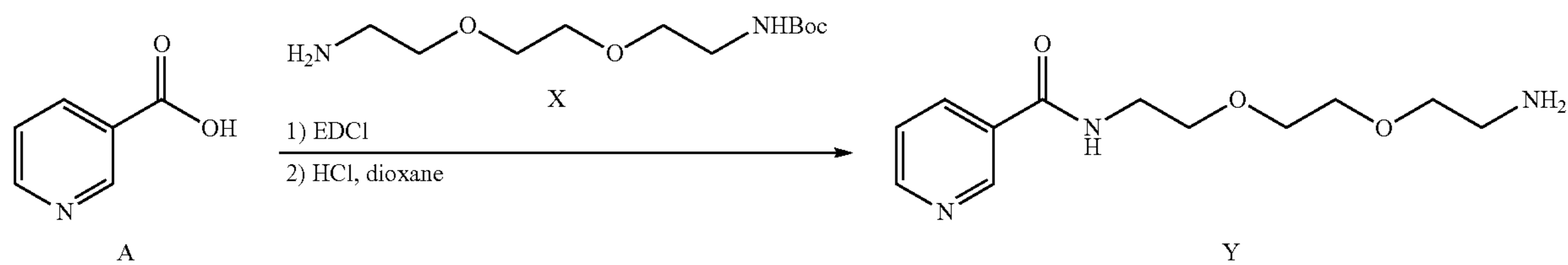
Scheme 7
